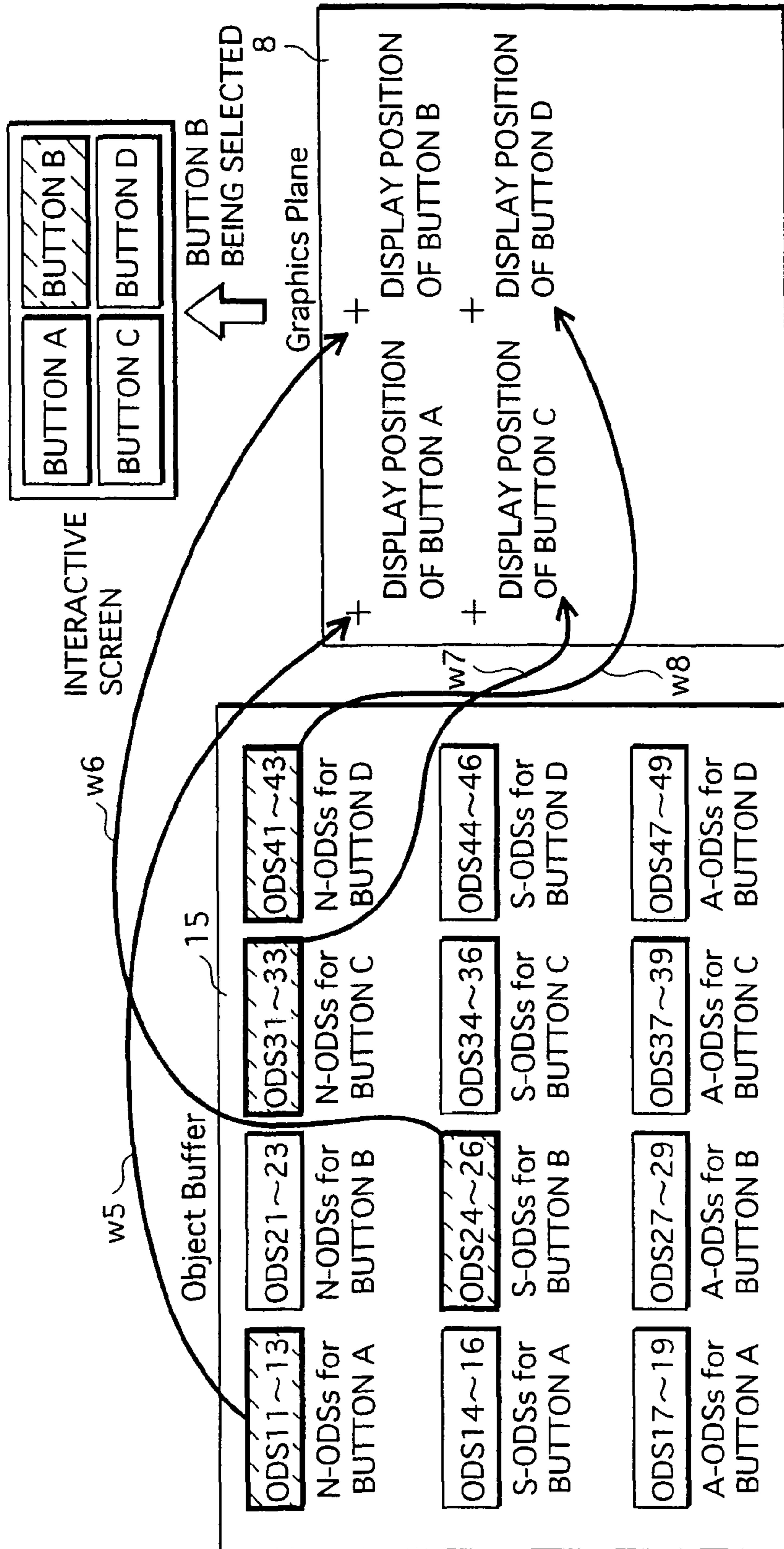
FIG. 30 WRITING OPERATION OF Graphics Controller AT INTERACTIVE SCREEN UPDATE ACCORDING TO 1st User Action(Move Right)
