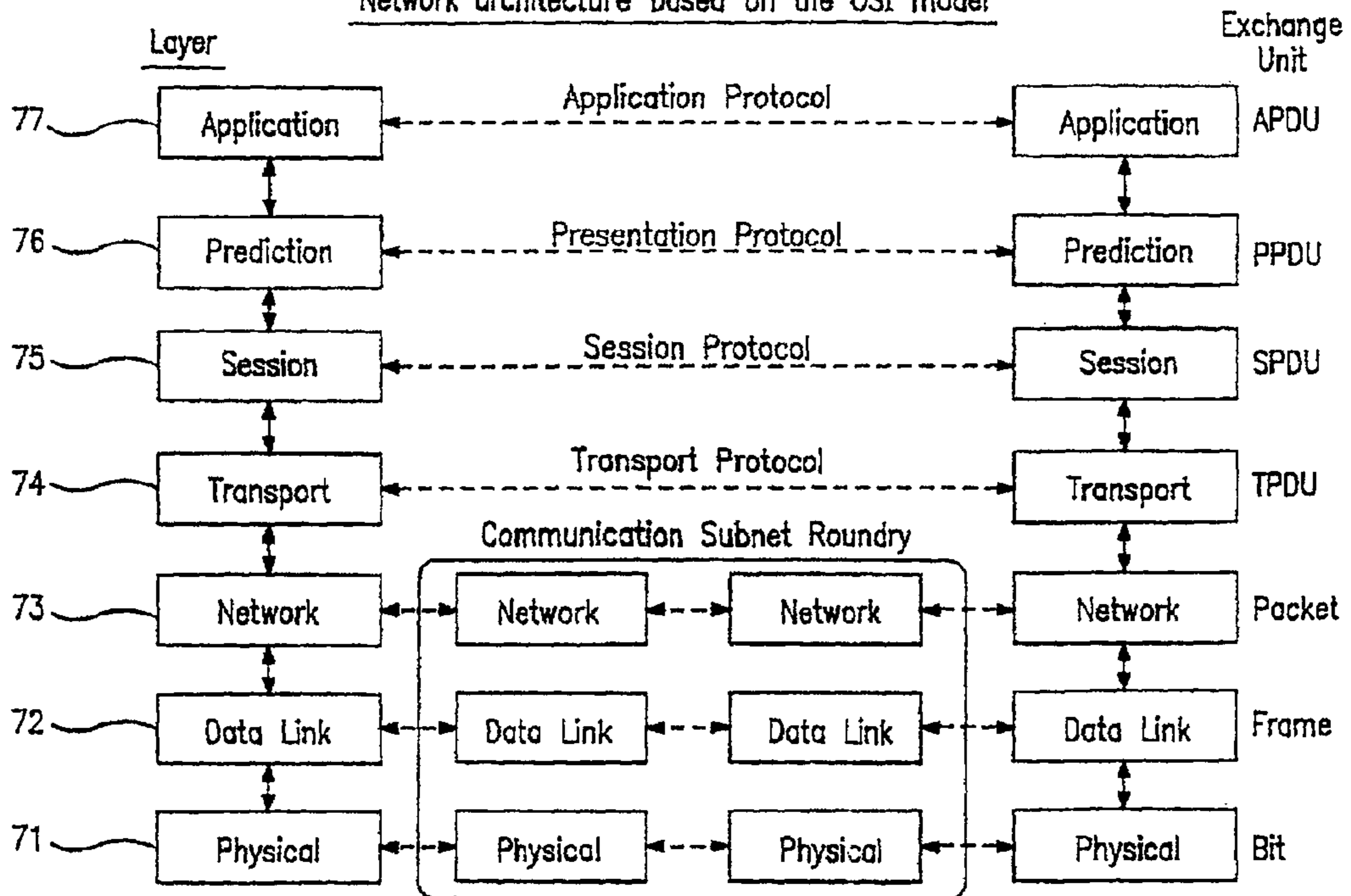
Network architecture based on the OSI model
