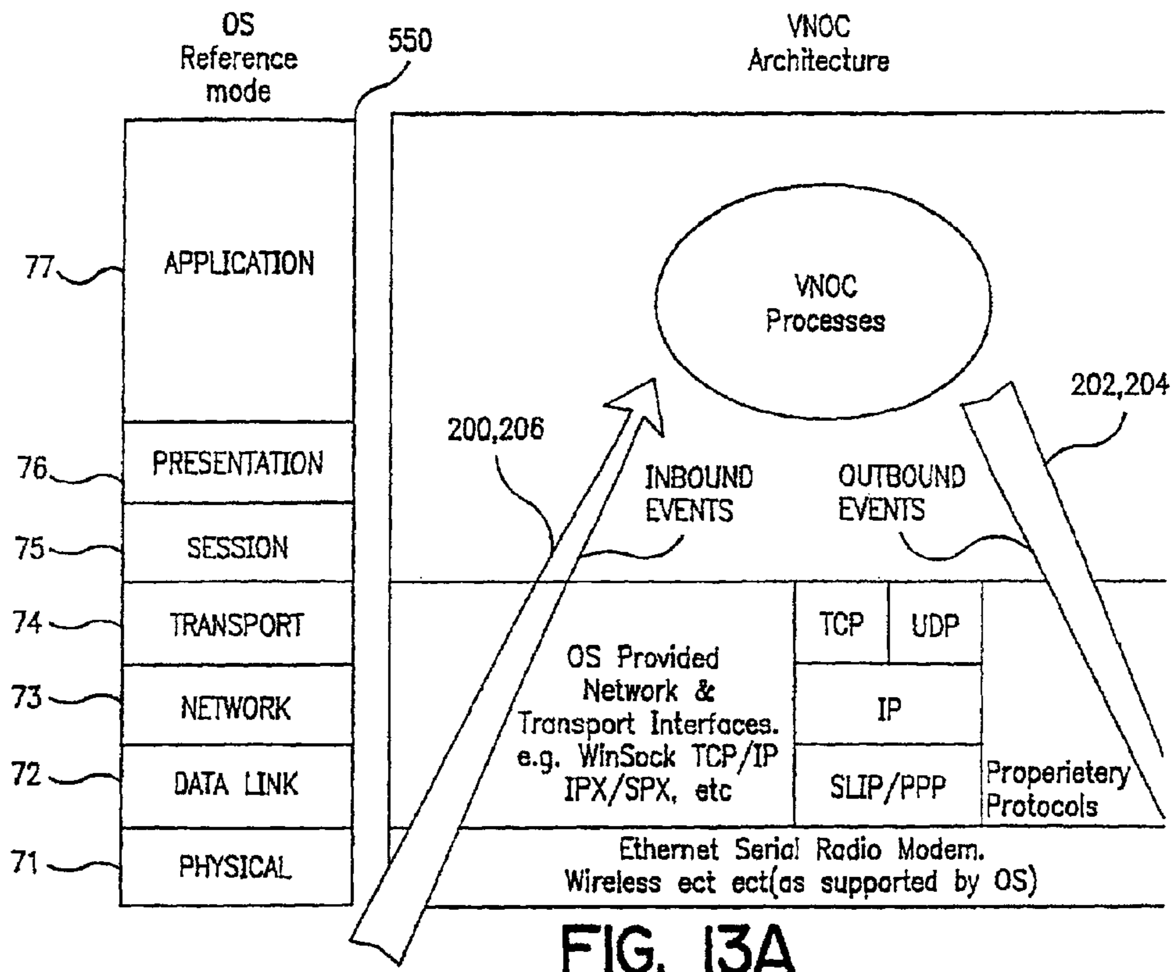
Network architecture based on the OSI model
