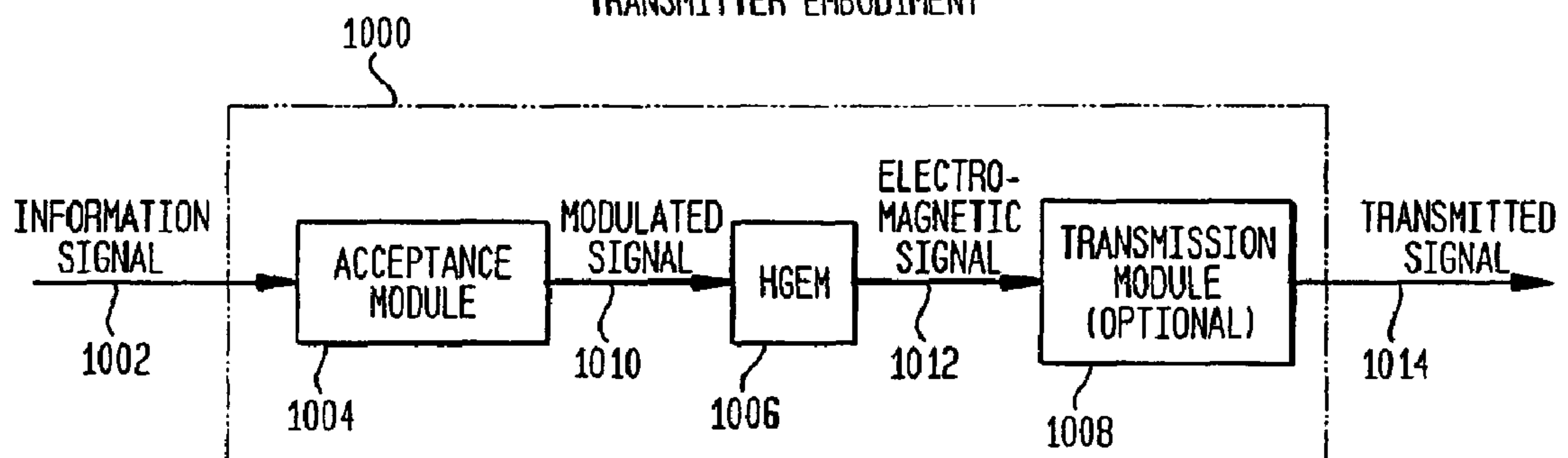
FIG. 10 TRANSMITTER EMBODIMENT
