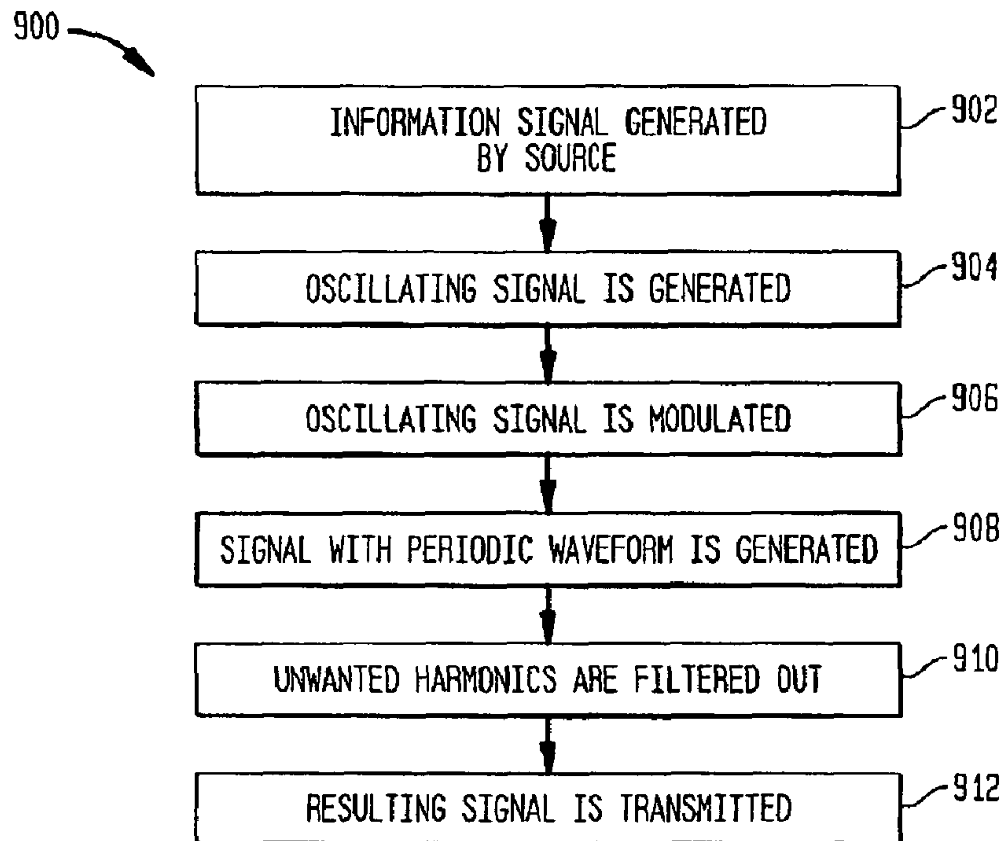
FIG. 9 TRANSMITTER
