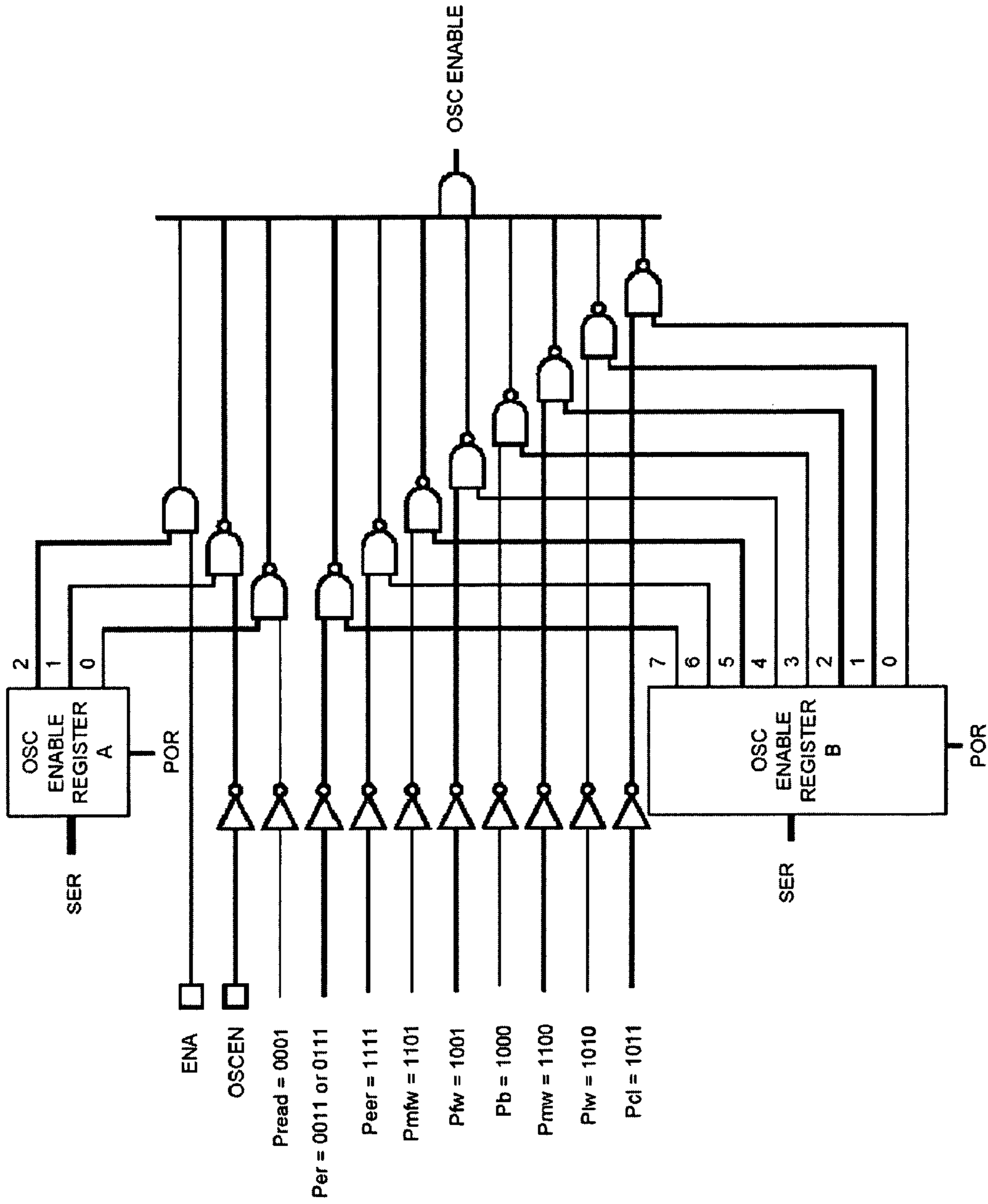
SERIAL CONFIGURABLE OSCILLATOR ENABLE LOGIC
