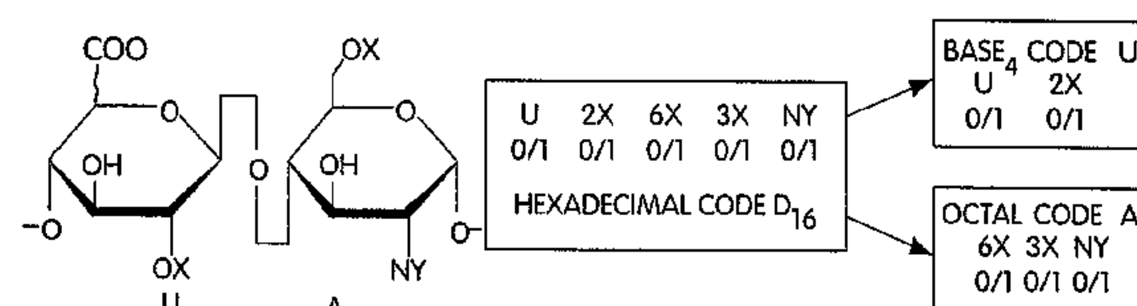
Representation of monosaccharides and linkages using PEN
