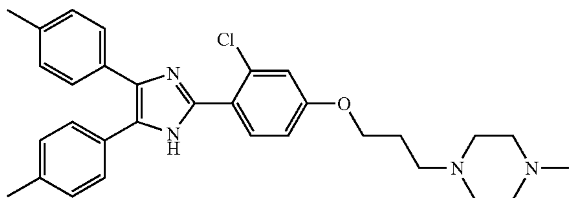
1-{3-[3-Chloro-4-(4,5-di-p-tolyl)-1H-imidazol-2-yl]-phenoxy}-propyl)-4-methyl-piperazine
