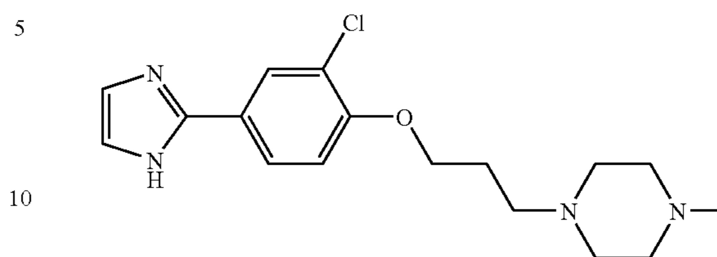
1-{3-[2-Chloro-4-(1H-imidazol-2-yl)-phenoxy]-propyl}-4-methyl-piperazine
