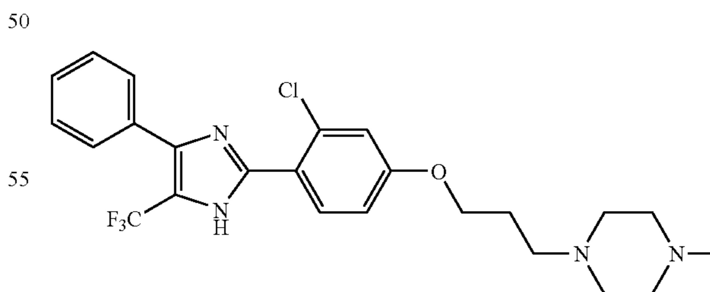
1-{3-[3-Chloro-4-(4-phenyl-5-trifluoromethyl-1H-imidazol-2-yl)-phenoxy]-propyl}-4-methyl-piperazine
