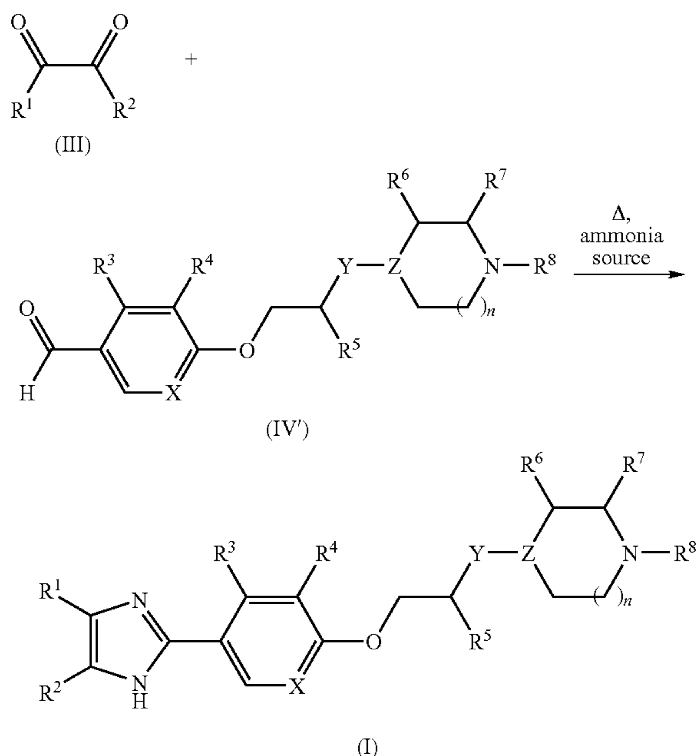
SCHEME 1
