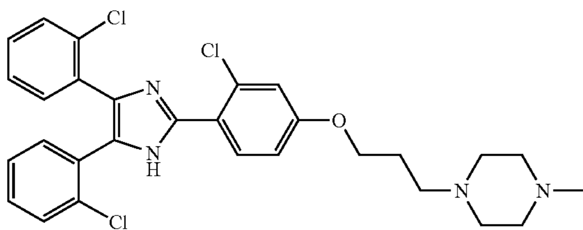
1-(3-{4-[4,5-Bis-(2-chloro-phenyl)-1H-imidazol-2-yl]-3-chloro-phenoxy}-propyl)-4-methyl-piperazine
