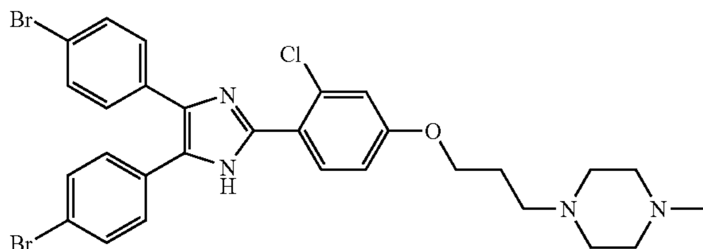
1-(3-{4-[4,5-Bis-(4-bromo-phenyl)-1H-imidazol-2-yl]-3-chloro-phenoxy}-propyl)-4-methyl-piperazine
