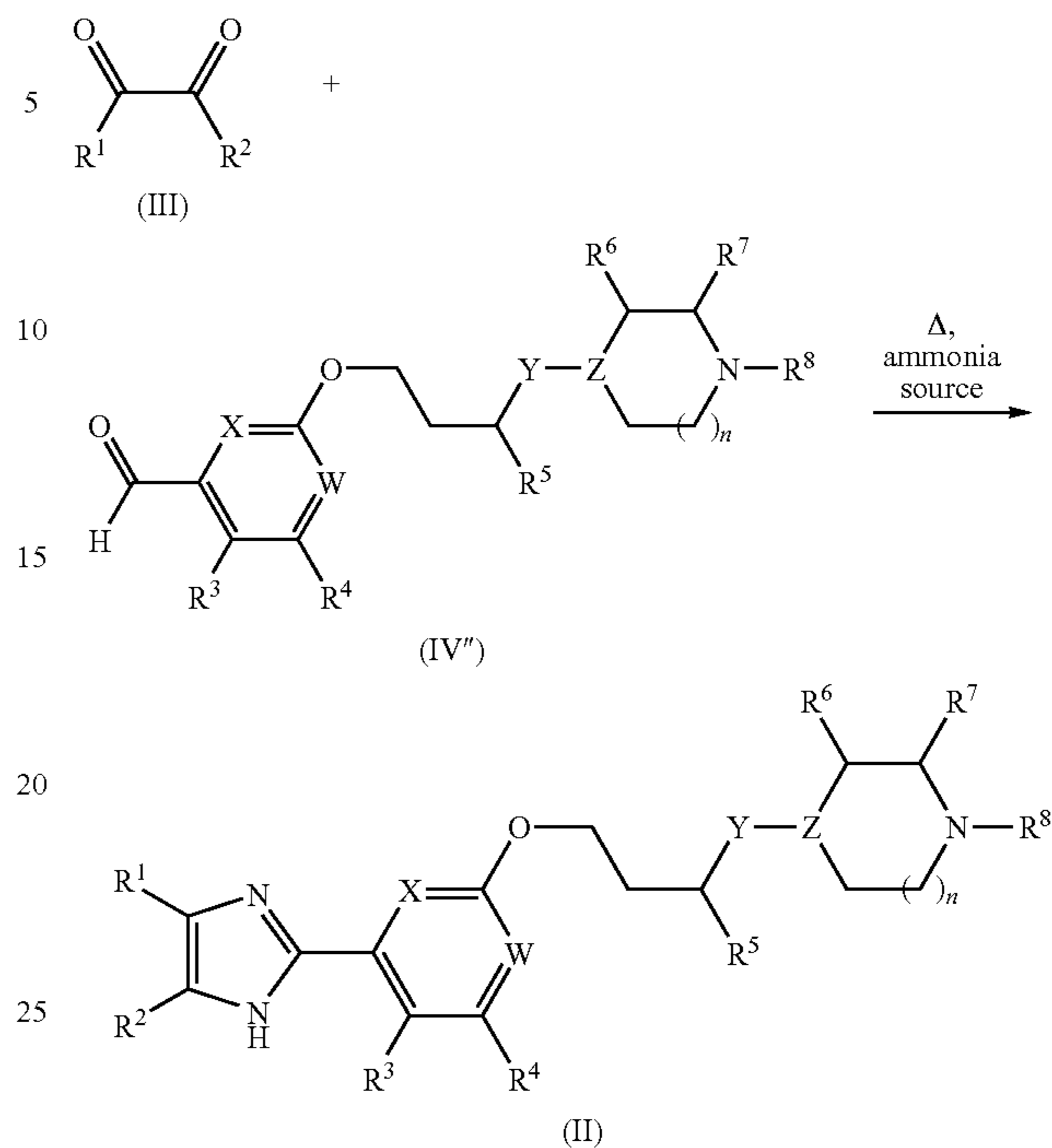
SCHEME 2
