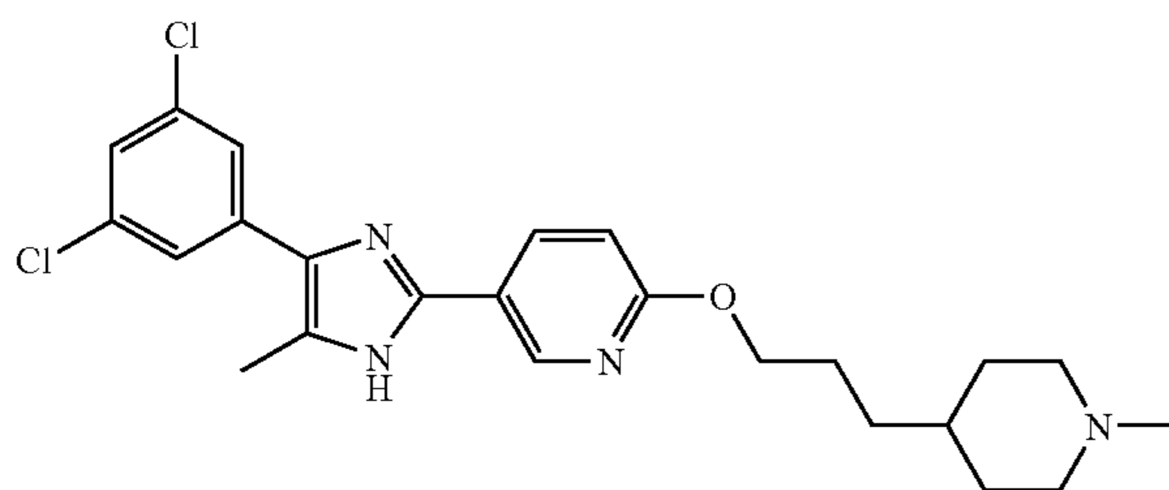
5-[4-(3,5-Dichloro-phenyl)-5-methyl-1H-imidazol-2-yl]-2-[3-(1-methyl-piperidin-4-yl)-propoxy]-pyridine
