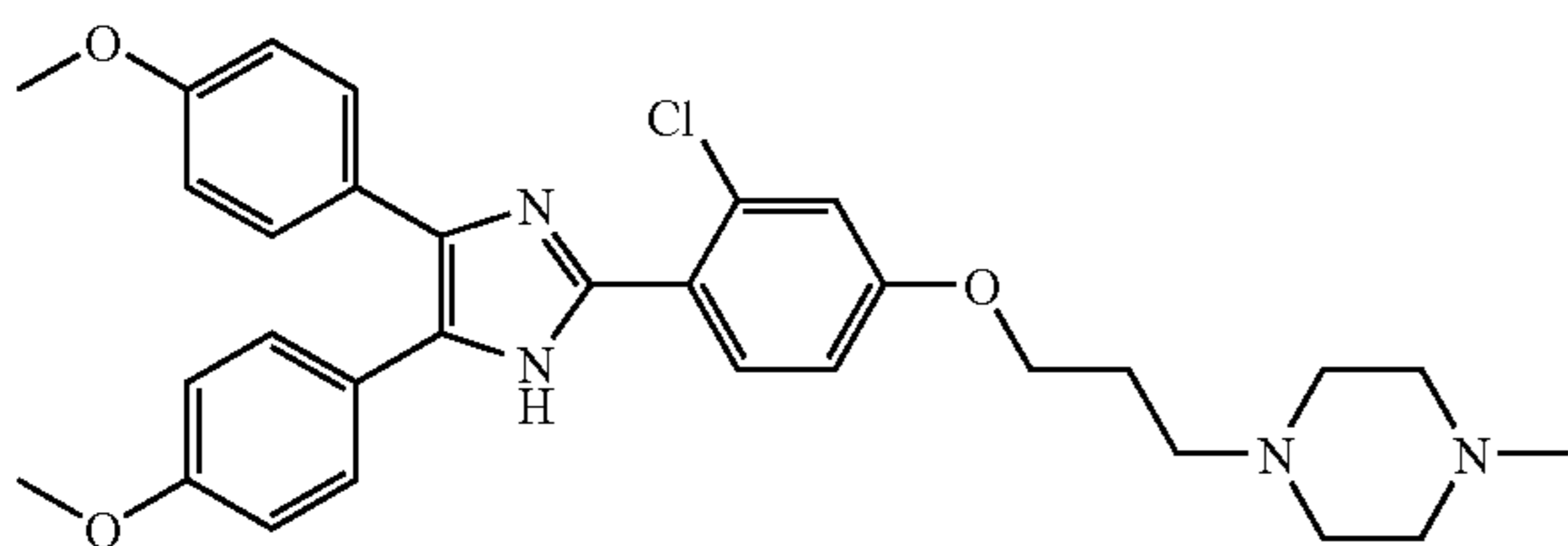
1-(3-{4-[4,5-Bis-(4-methoxy-phenyl)-1H-imidazol-2-yl]-3-chloro-phenoxy}-propyl)-4-methyl-piperazine
