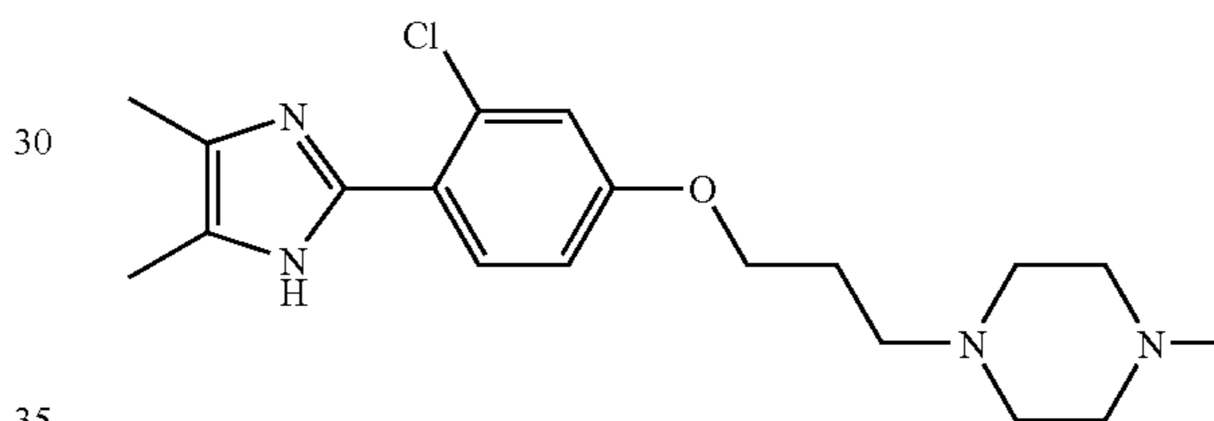
1-{3-[3-Chloro-4-(4,5-dimethyl-1H-imidazol-2-yl)-phenoxy]-propyl}-4-methyl-piperazine
