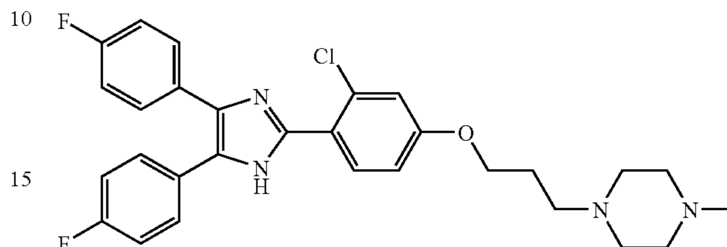
1-(3-{4-[4,5-Bis-(4-fluoro-phenyl)-1H-imidazol-2-yl]-3-chloro-phenoxy}-propyl)-4-methyl-piperazine
