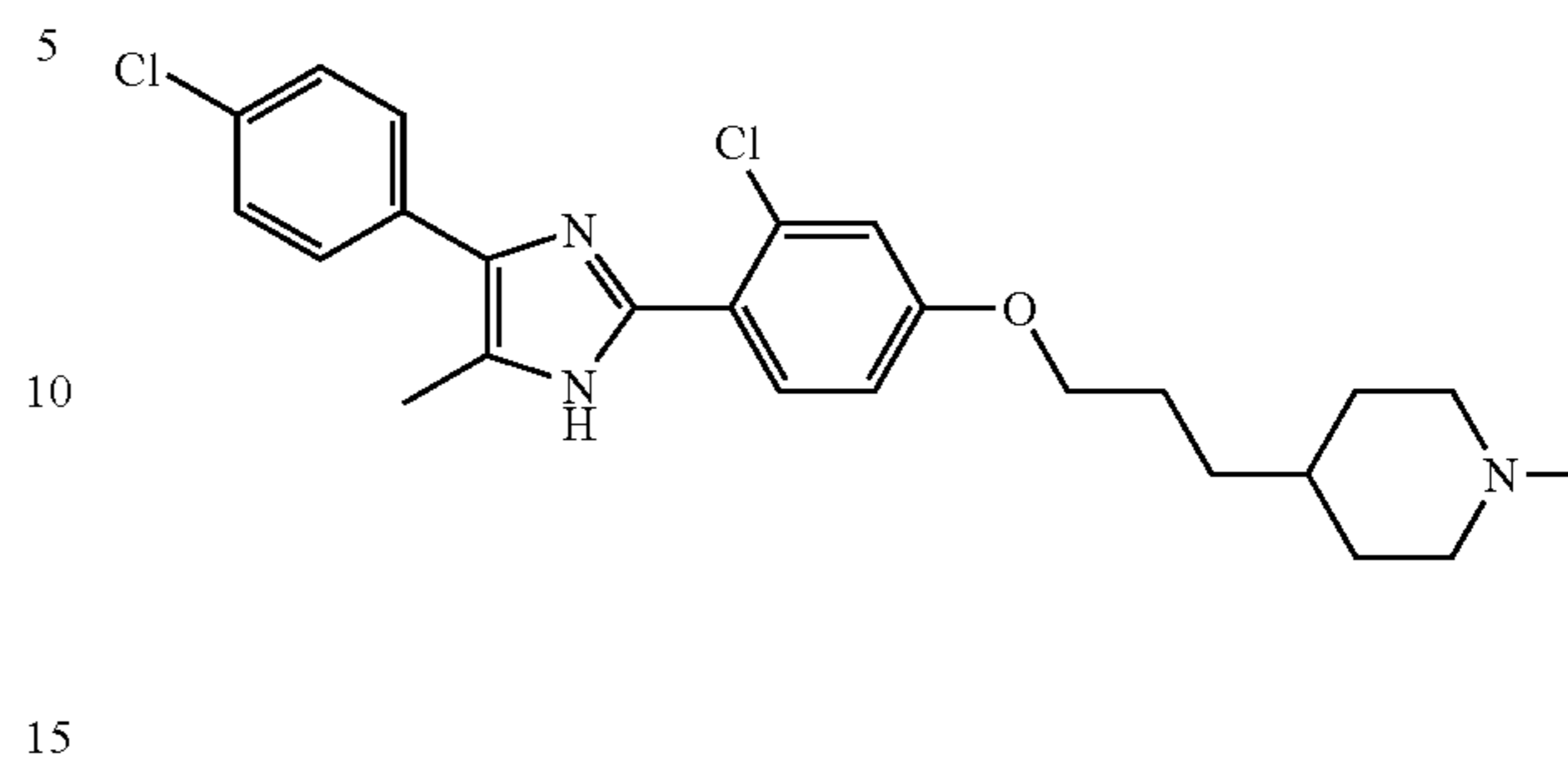
4-(3-{3-Chloro-4-[4-(4-chloro-phenyl)-5-methyl-1H-imidazol-2-yl]-phenoxy}-propyl)-1-methyl-piperidine
