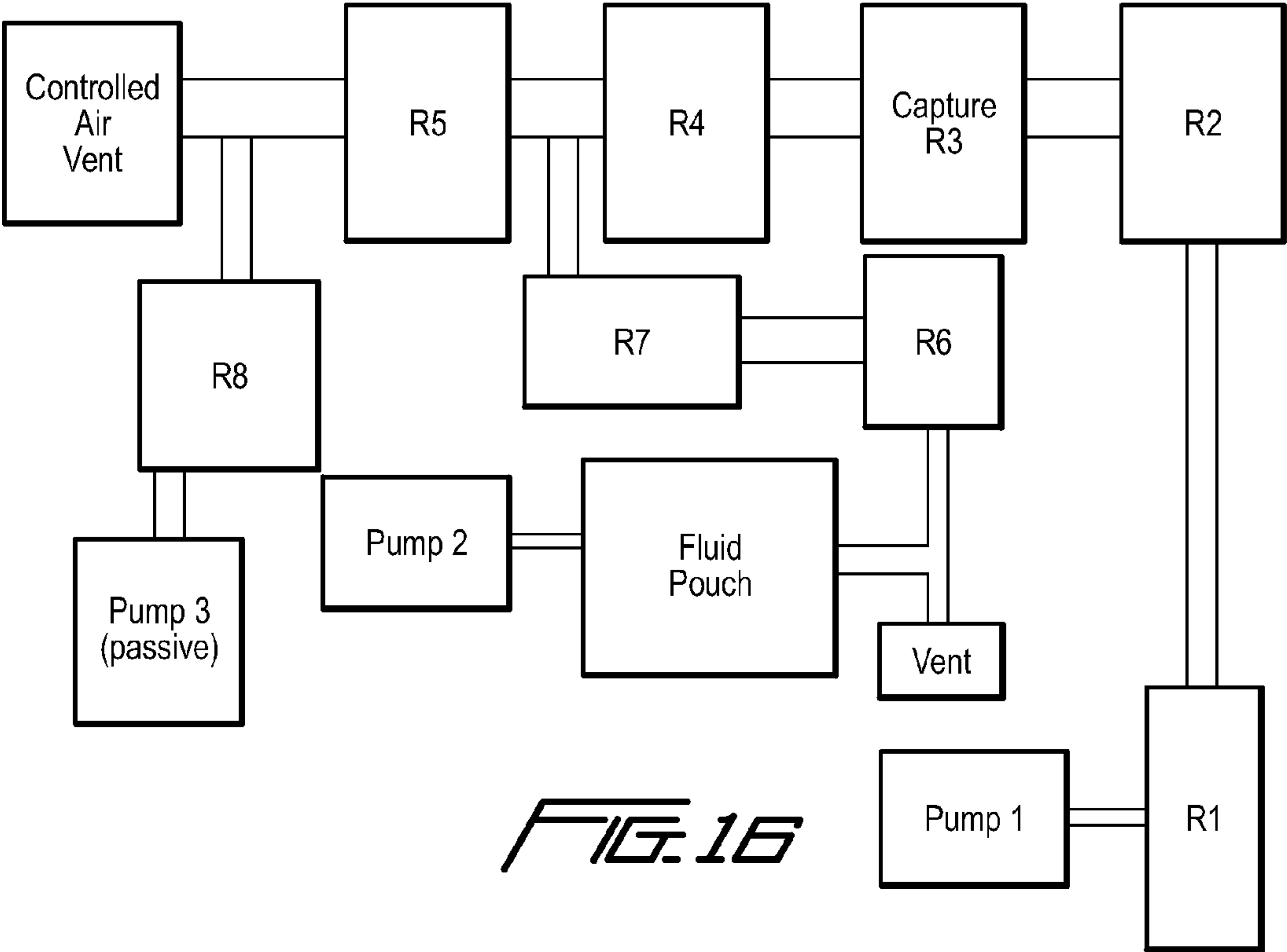
Fluidic Schematic for i-STAT immunocartridge
