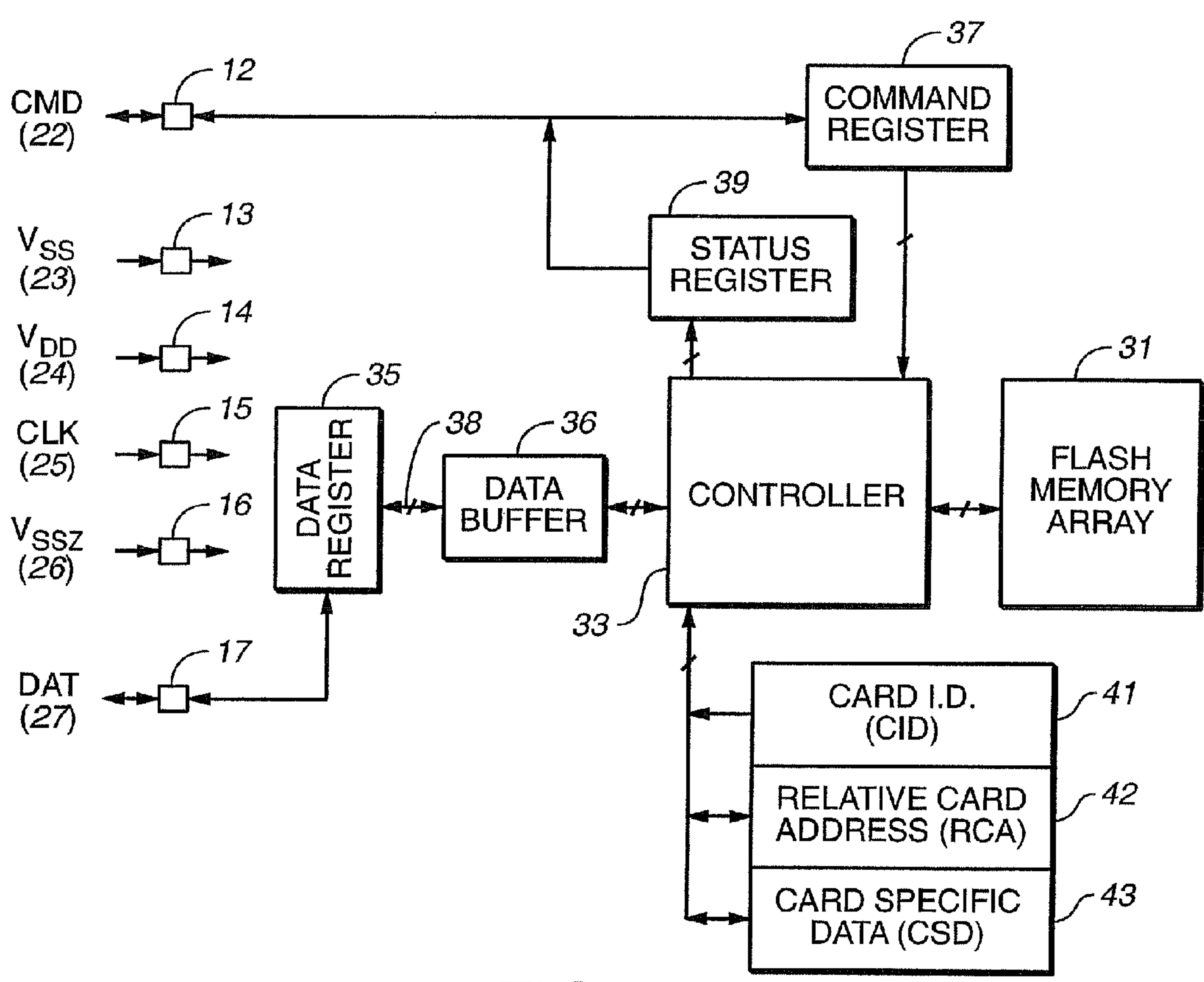
FIG. 2 (PRIOR ART)
