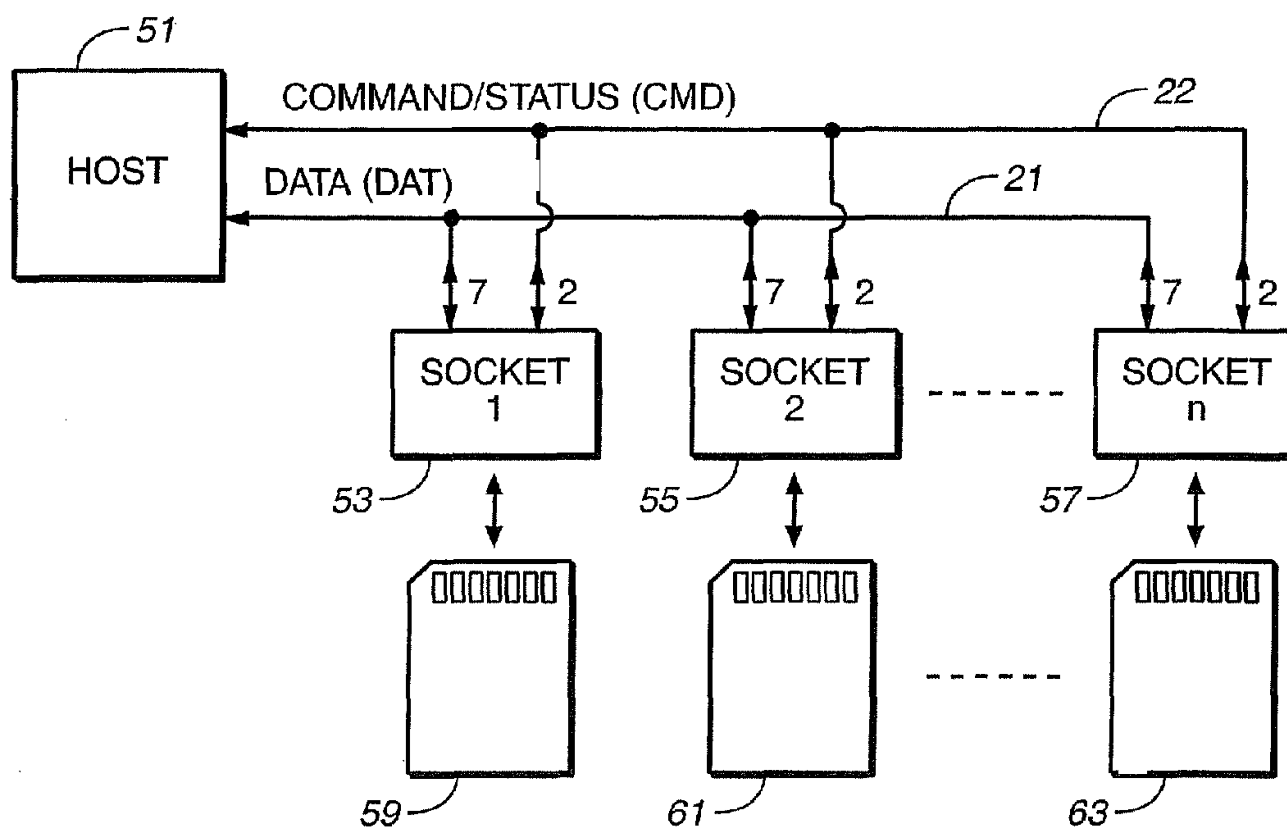
FIG. 3 (PRIOR ART)
