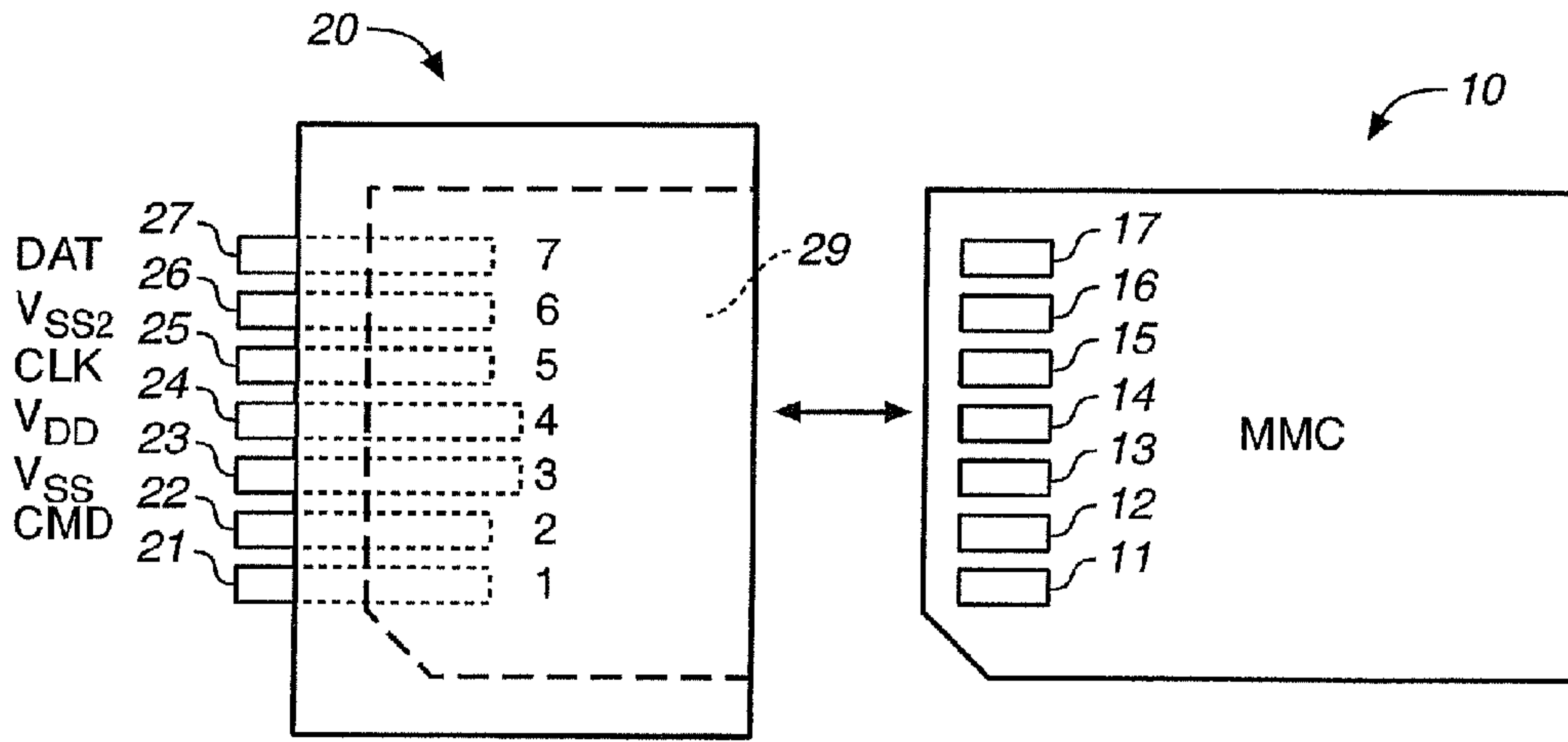
FIG. 1 (PRIOR ART)
