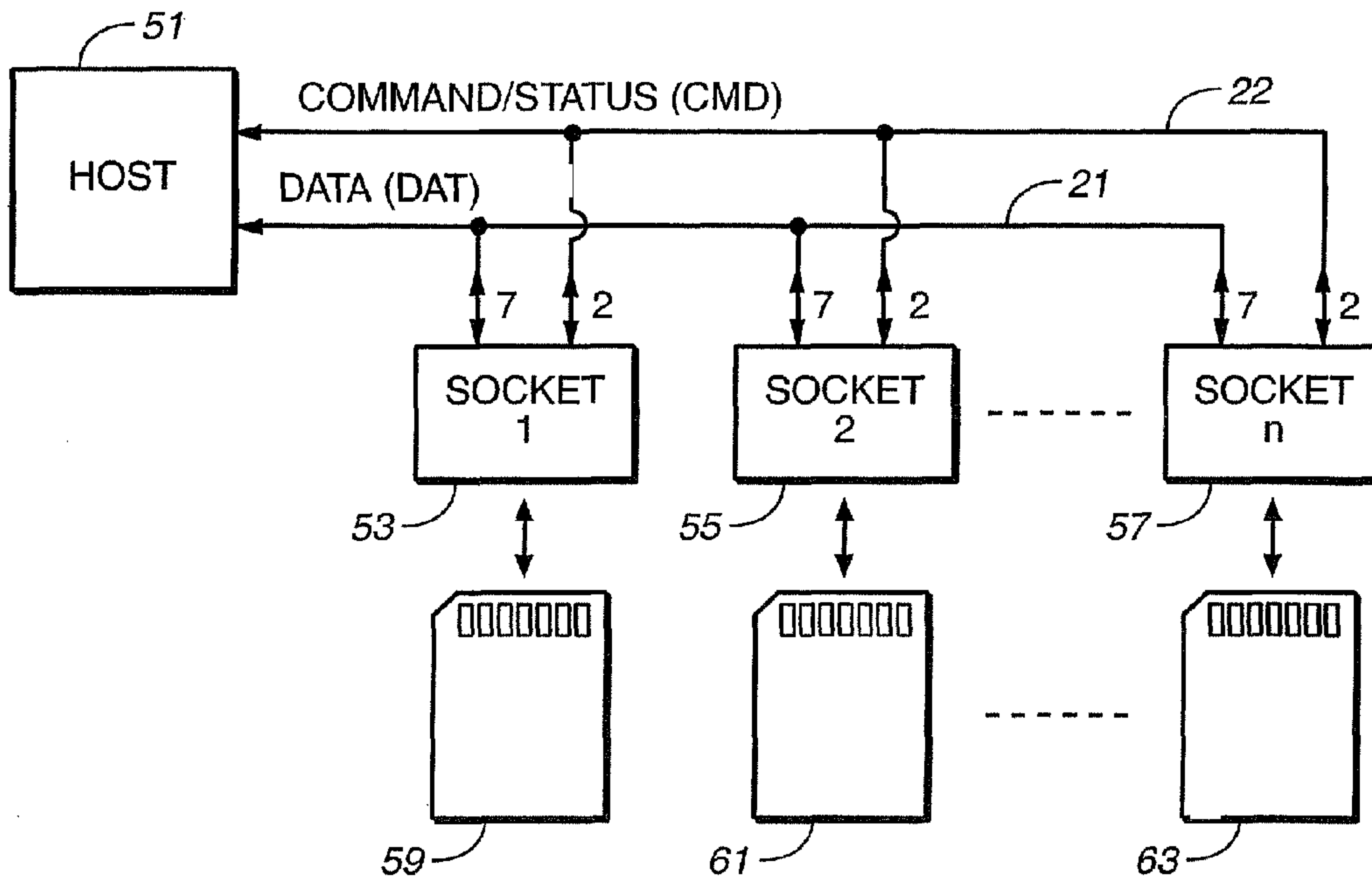
FIG. 3 (PRIOR ART)
