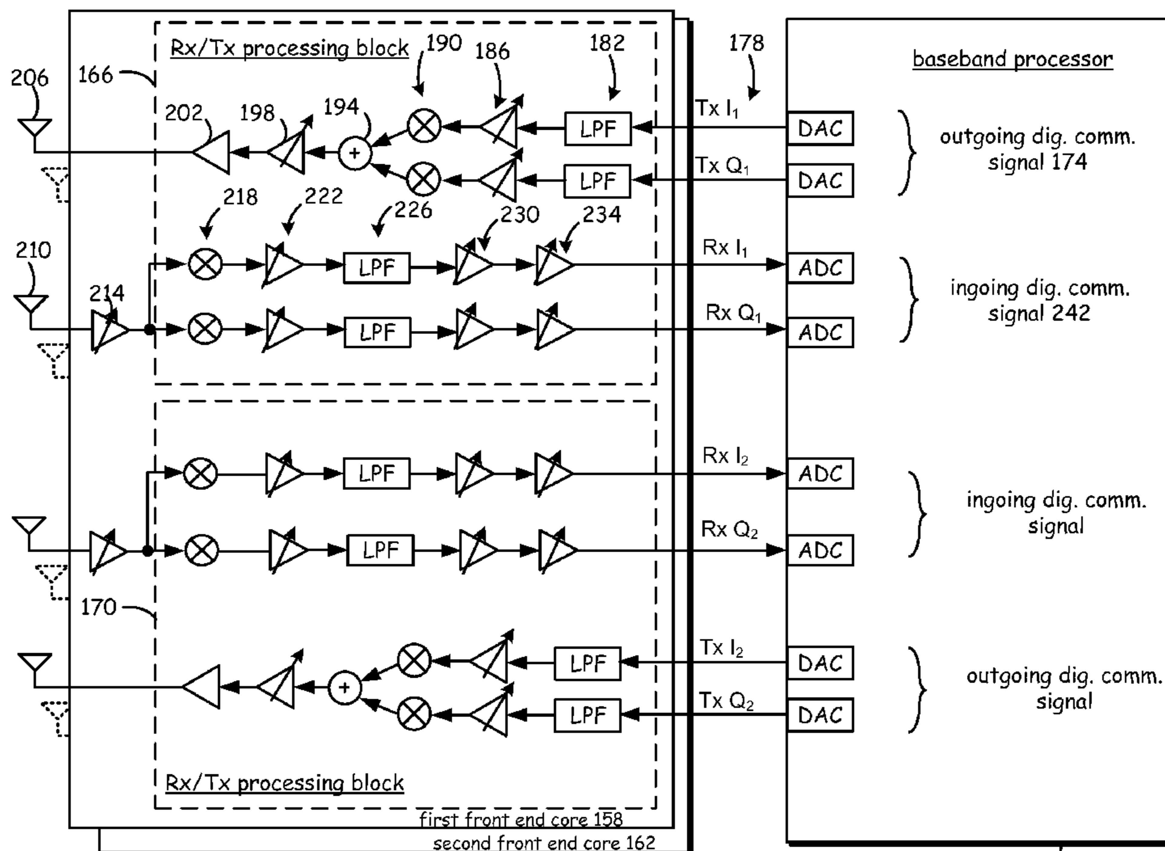
MIMO transceiver 150
