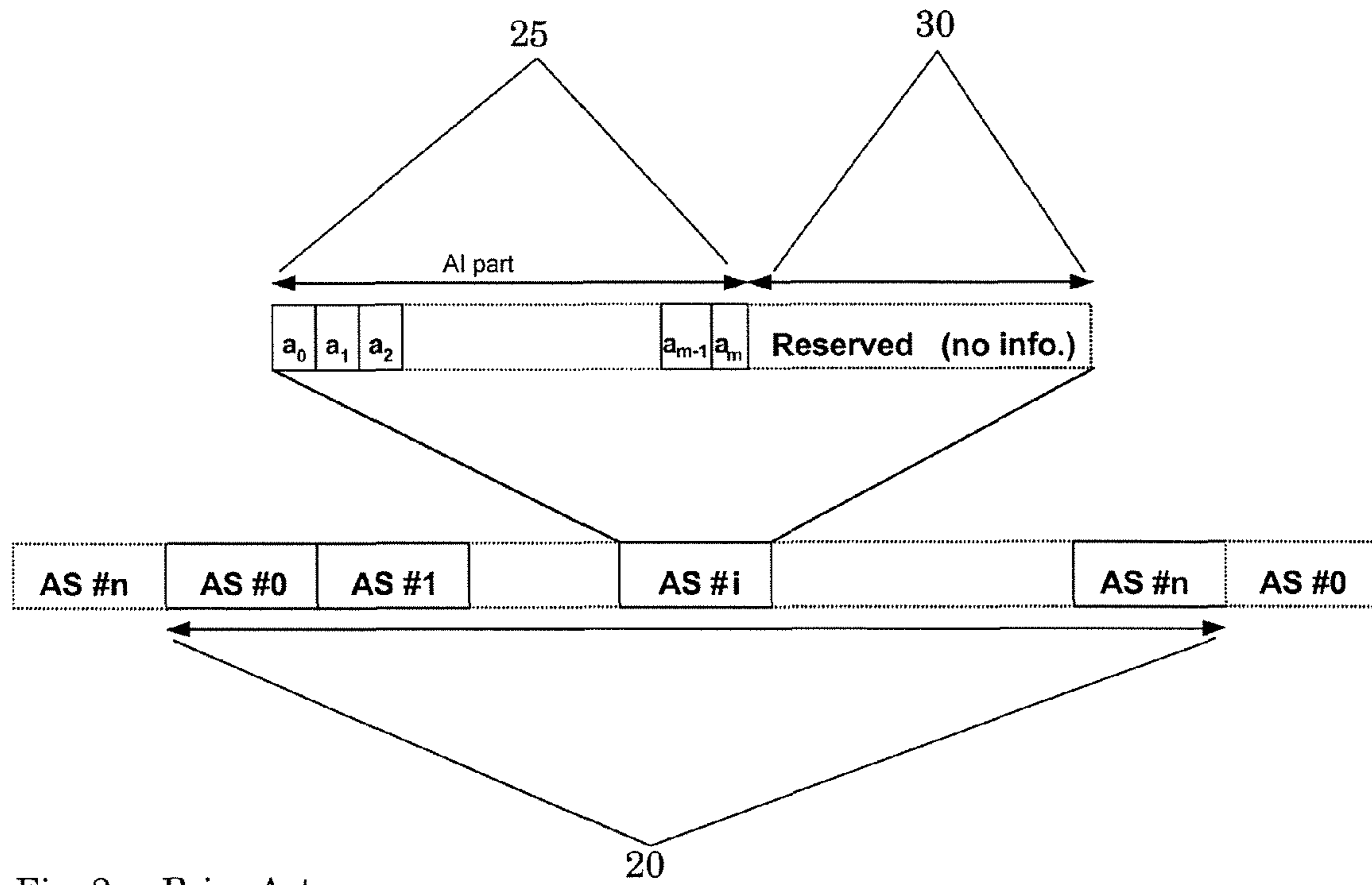
Fig. 2 Prior Art
