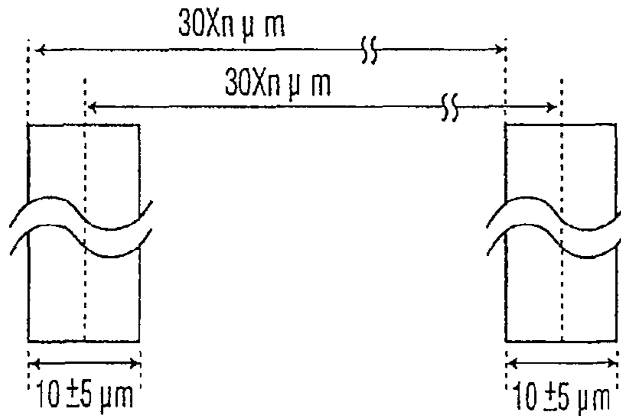
DIMENSIONAL ACCURACY OF SLIT (AT r=22.2\text{mm} )
