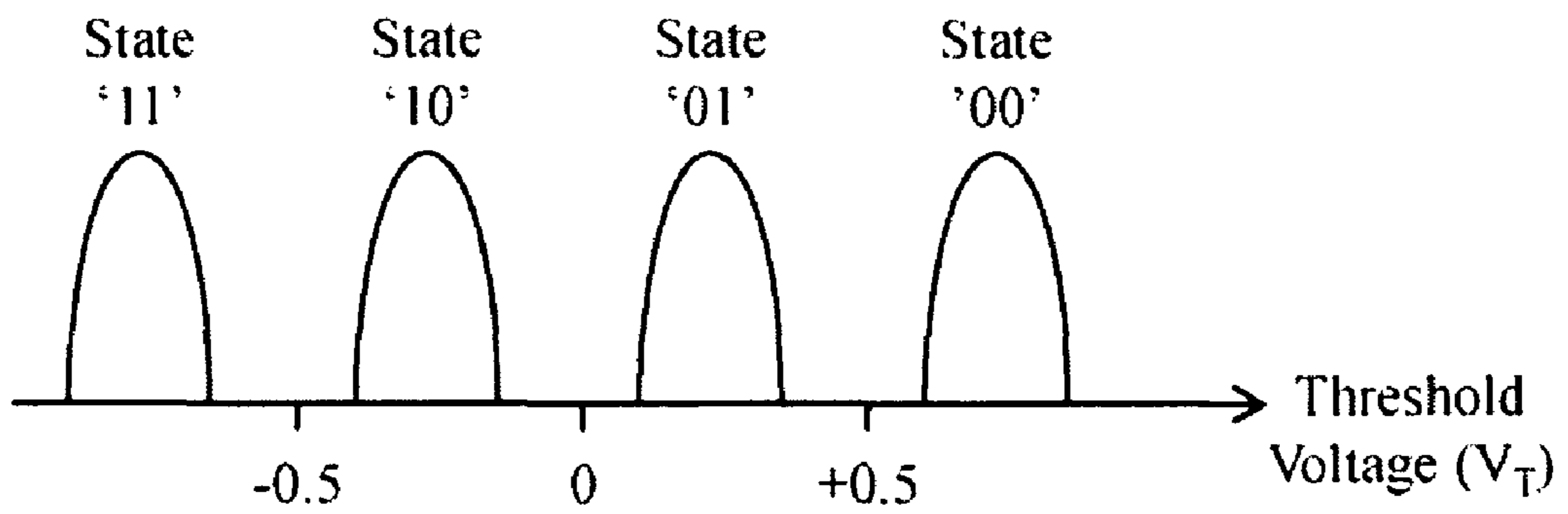
Multi-Level Cell
