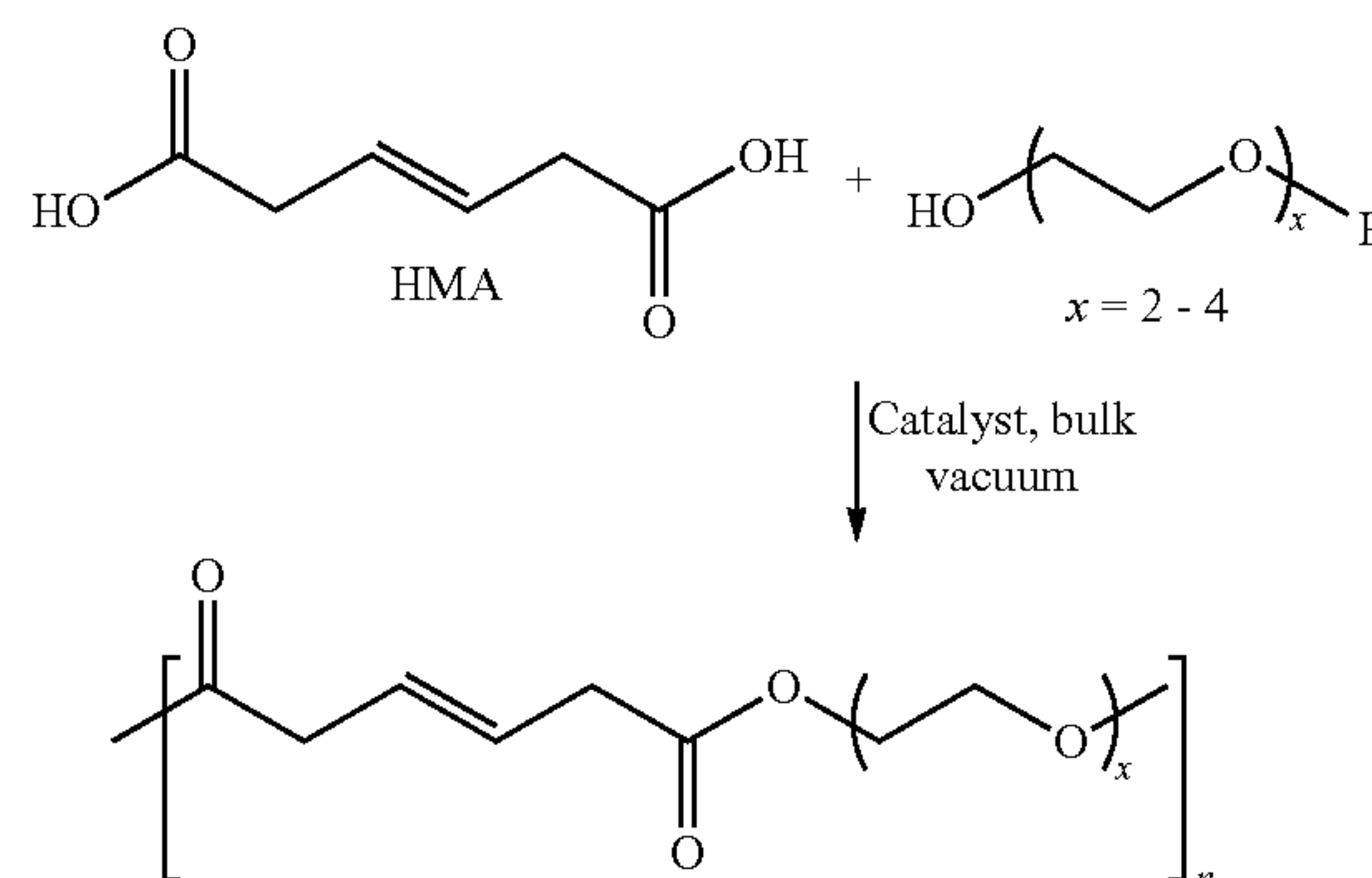
Scheme 1. Synthesis of unsaturated poly(ester-ether) prepolymers
