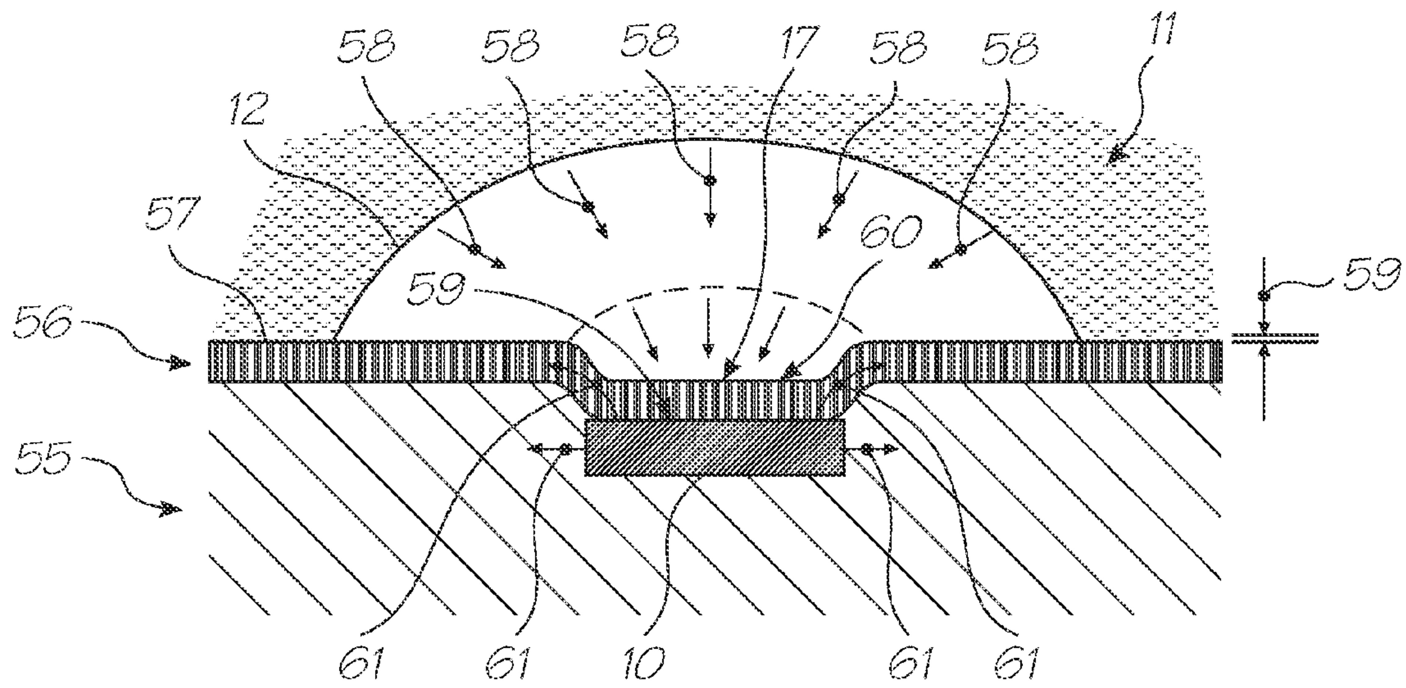
FIG. 47 (PRIOR ART)
