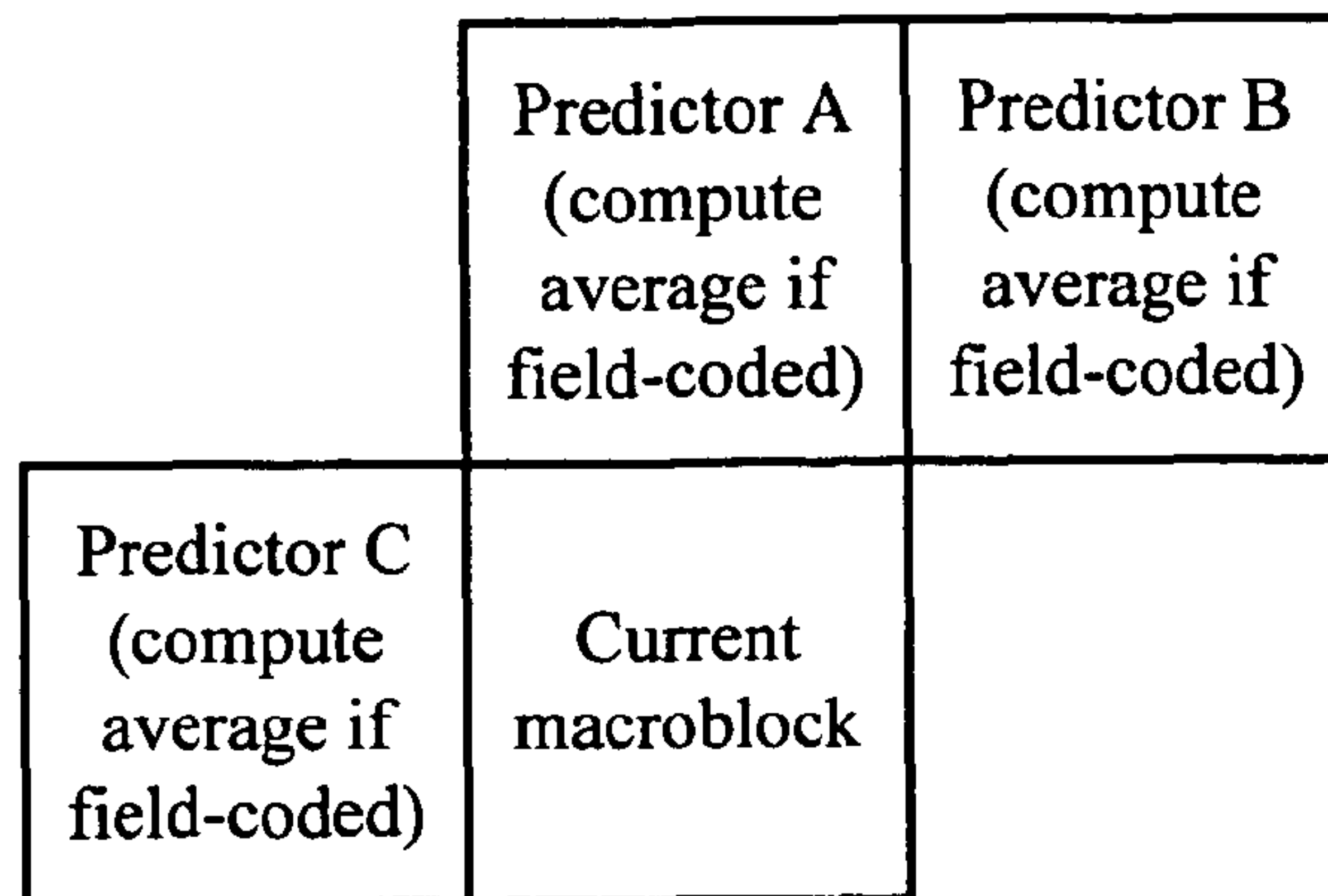
Figure 11, prior art
