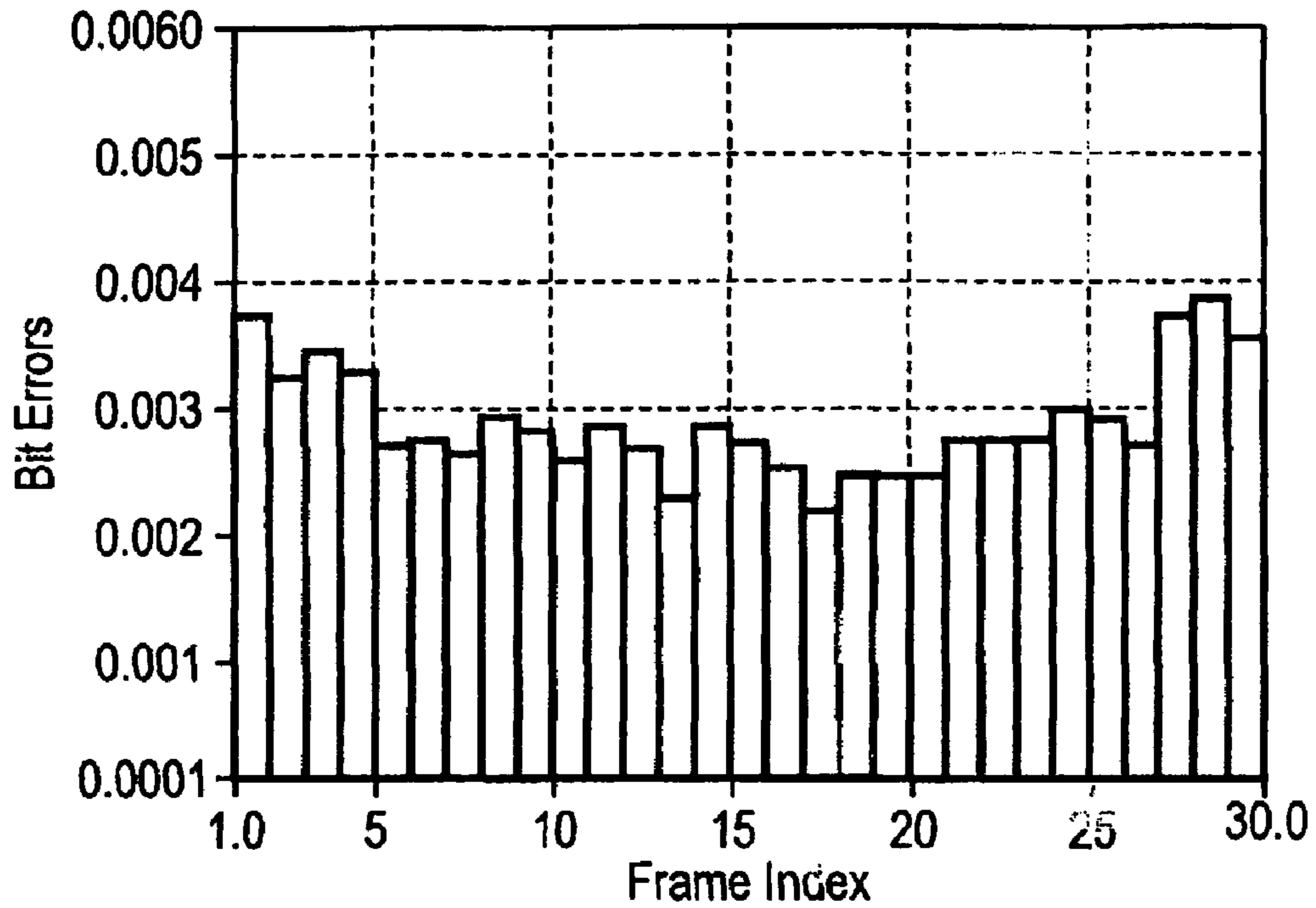
HS-SCCH, Part 2, Pattern 19, FER=1.1×E-02 Error Histogram
