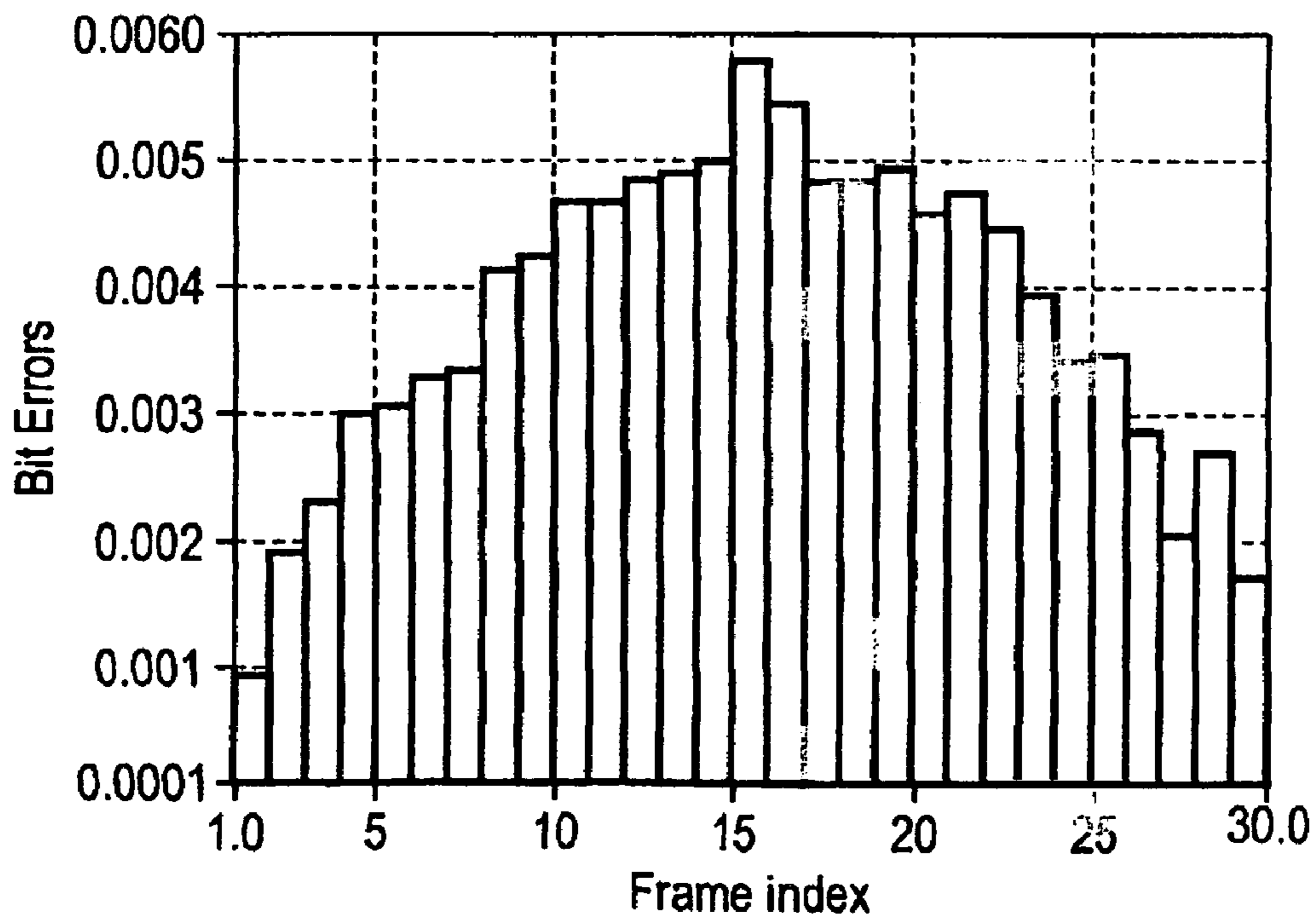
HS-SCCH, Part 2, Pattern 0, FER=1.6×E-02 Error Histogram
