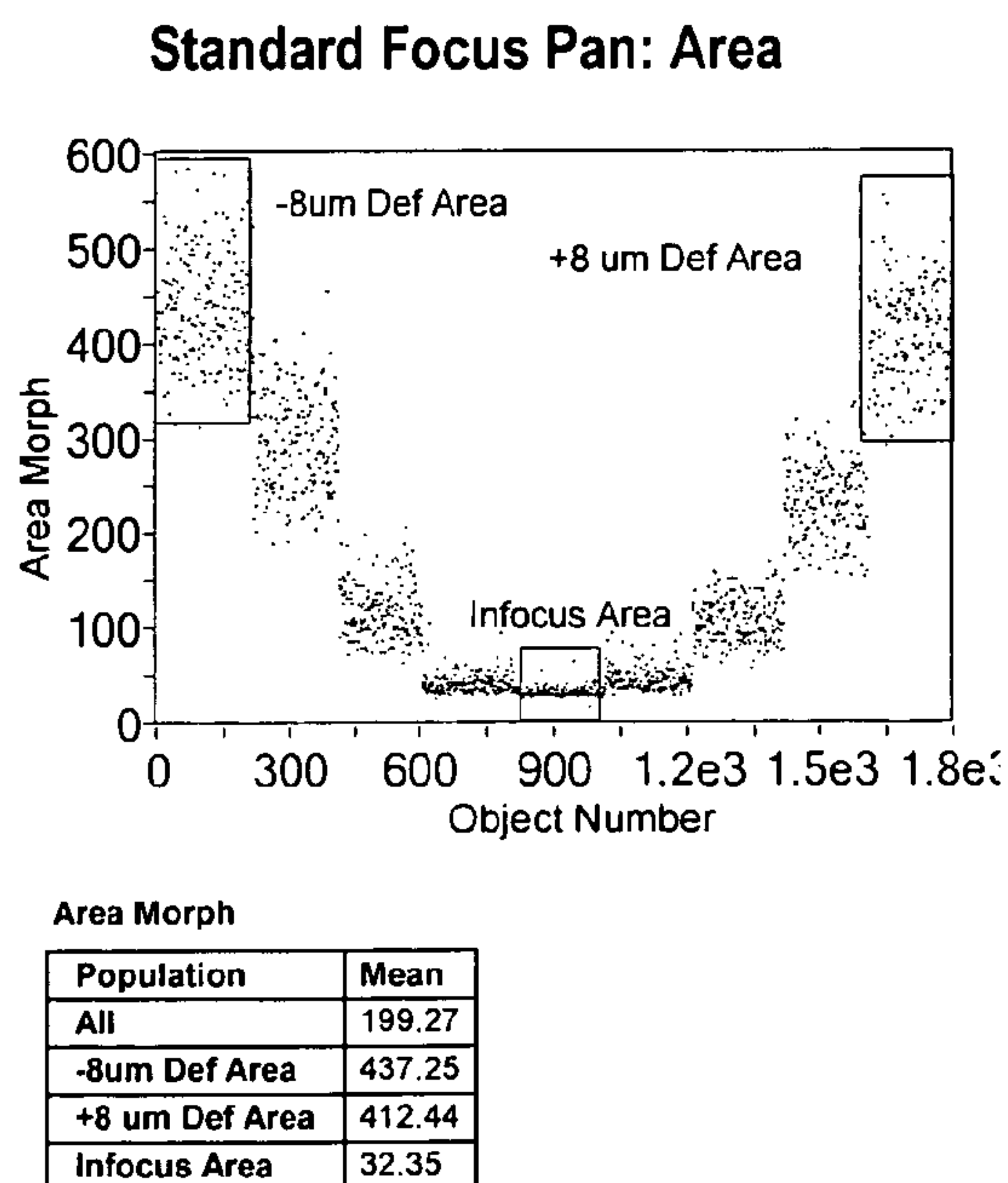
FIG. 15A – PRIOR ART
