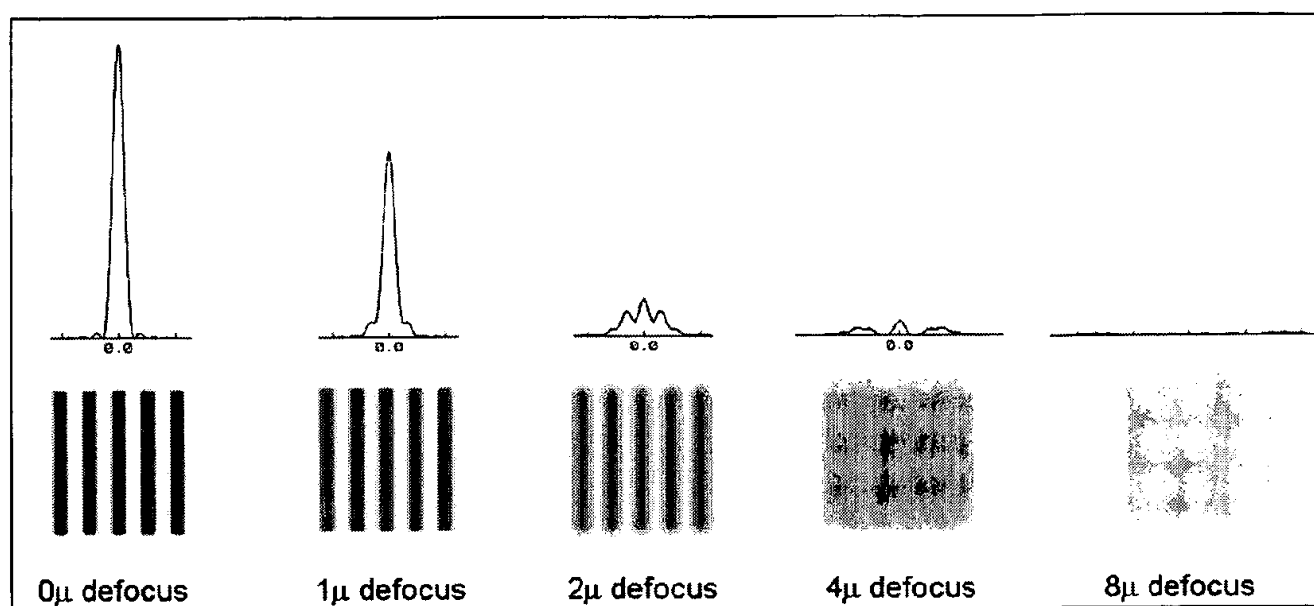
FIG. 9 (PRIOR ART)
