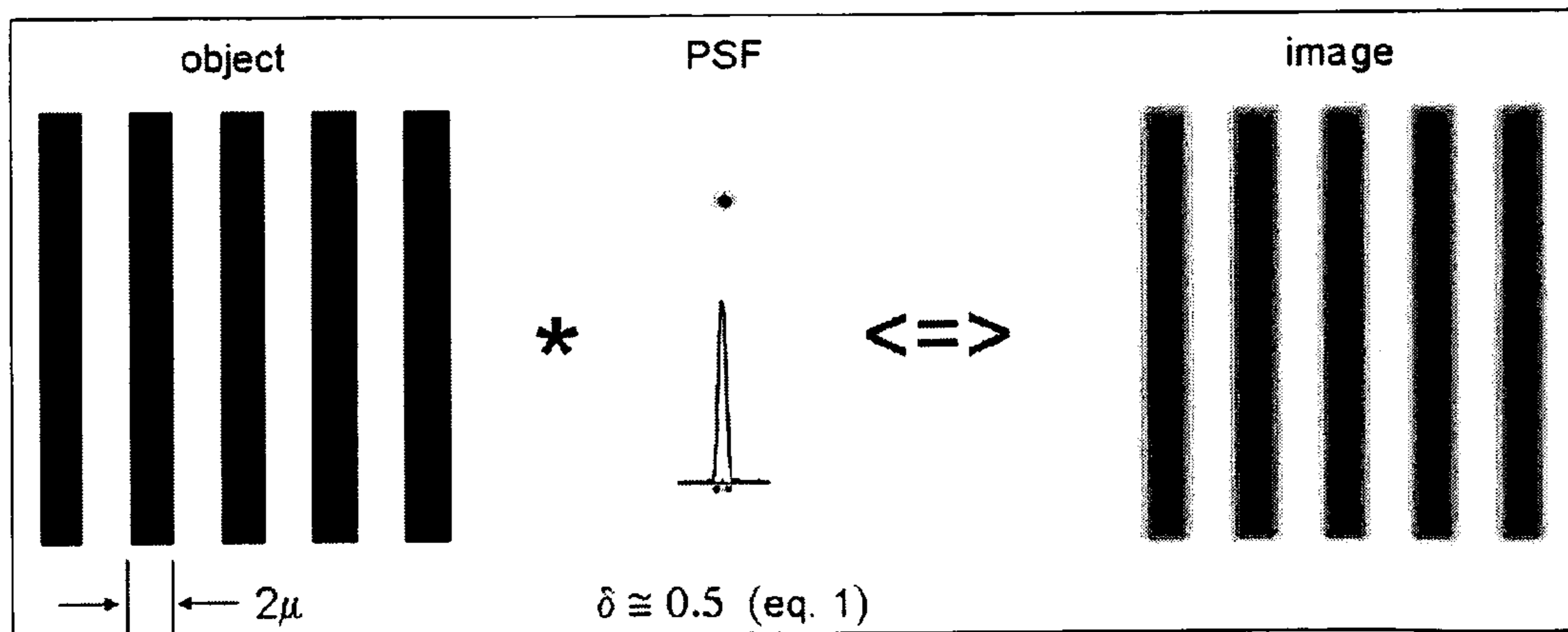
FIG. 8 (PRIOR ART)
