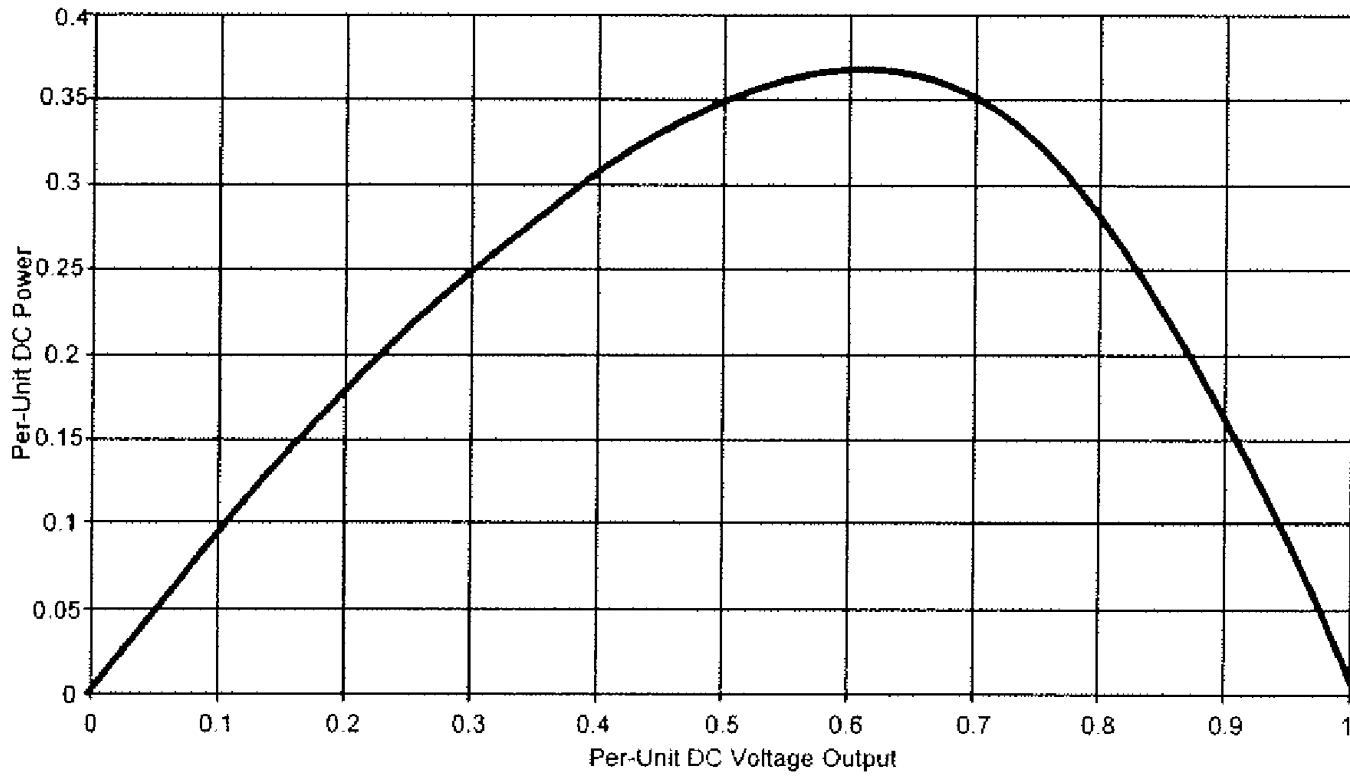
The Power Available from a 3-Phase Diode Rectifier, with Capacitors in Series with the AC Source.
