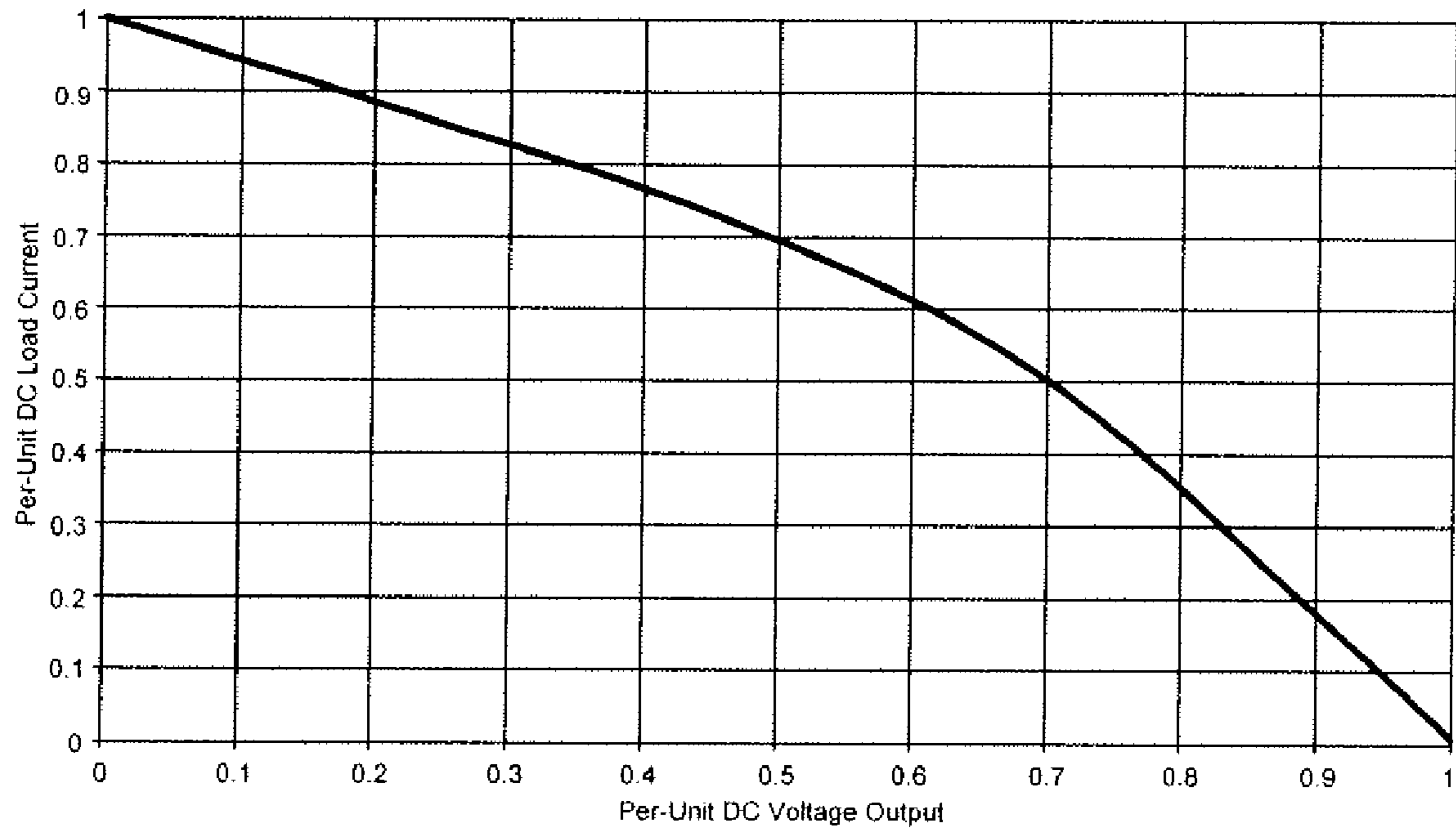
The Current Available from a 3-Phase Diode Rectifier, with Capacitors in Series with the AC Source.
