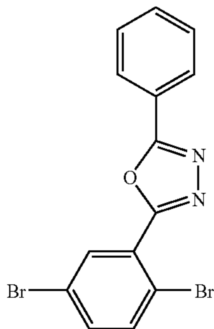
2-(2,5-Dibromo-phenyl)-5-phenyl-[1,3,4]oxadiazole,
