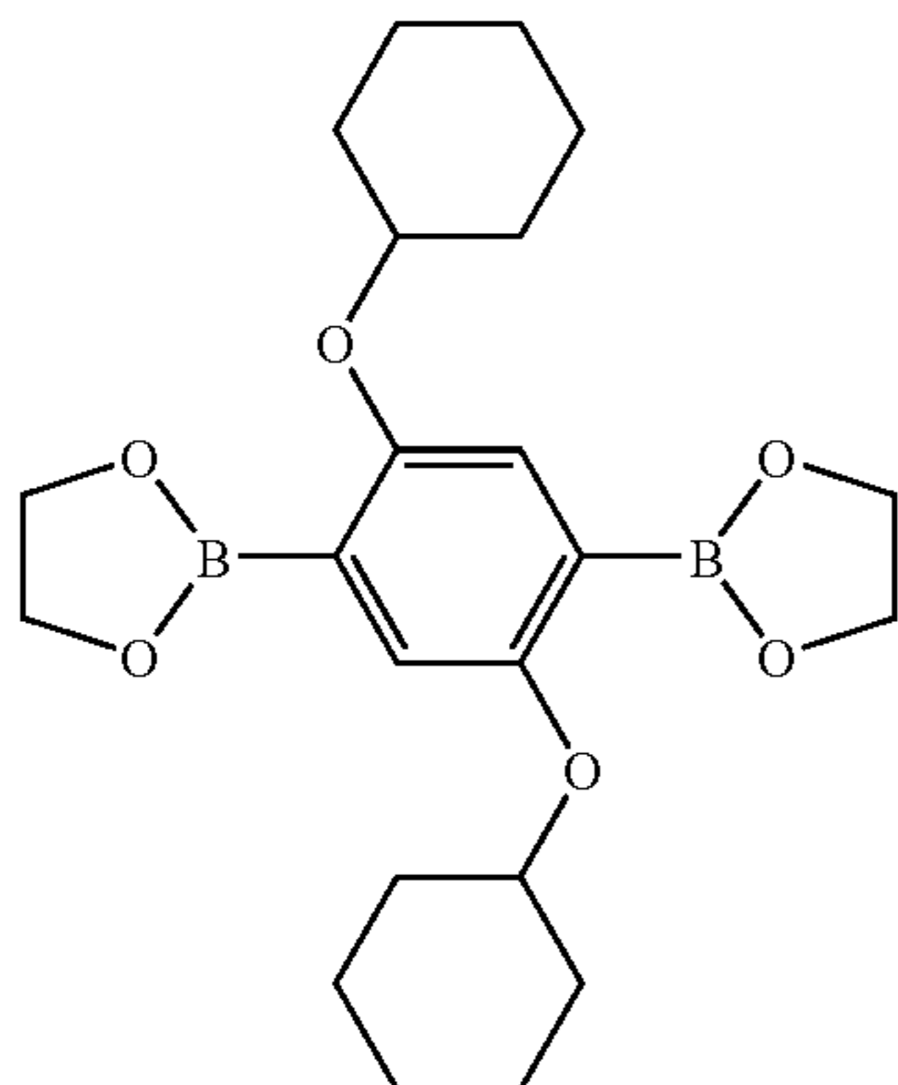
2-(4-[1,3,2]Dioxaborolan-2-yl)-2,5-dicyclohexyloxy-phenyl-[1,3,2]dioxaborolane
