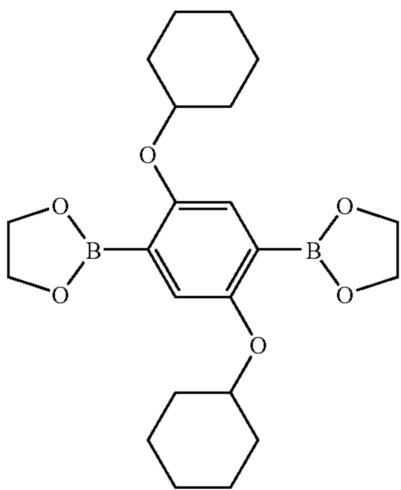
2-(4-[1,3,2]Dioxaborolan-2-yl)-2,5-dicyclohexyloxy-phenyl-[1,3,2]dioxaborolane
