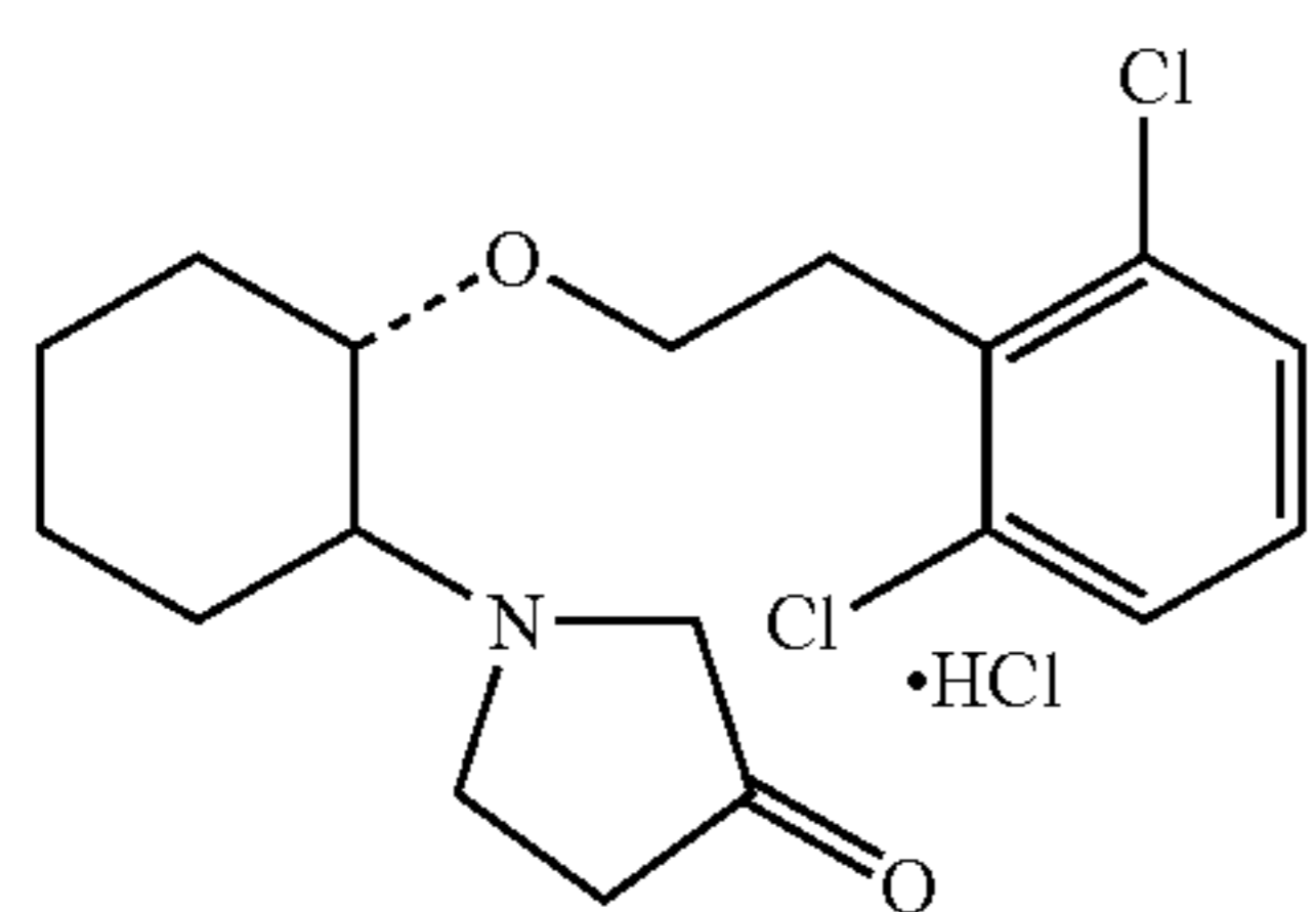
(1R,2R)/(1S,2S)-2-(3-ketopyrrolidinyl)-1-(2,6-dichlorophenethoxy)cyclohexane
