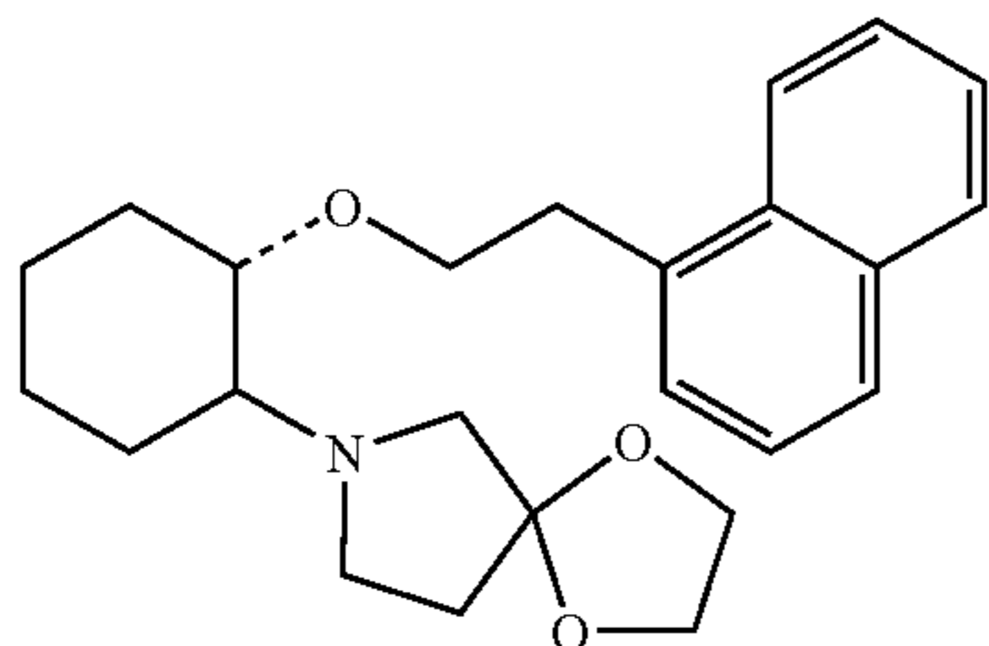
(1R,2R)/(1S,2S)-2-[1,4-dioxo-7-azaspiro[4.4]non-7-yl]-1-(1-naphthenethoxy)cyclohexane
