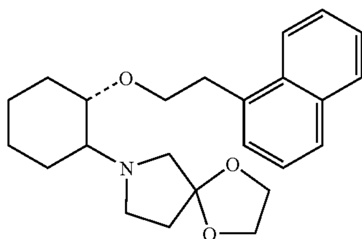
(1R,2R)/(1S,2S)-2-[1,4-dioxo-7-azaspiro[4.4]non-7-yl]-1-(1-naphthenethoxy)cyclohexane
