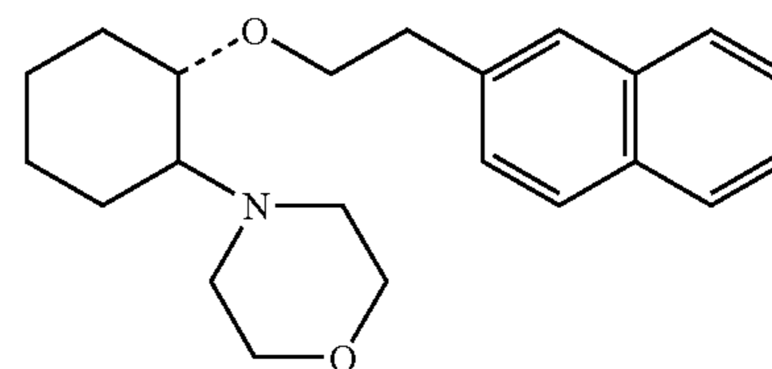
(1R,2R)/(1S,2S)-[2-(4-morpholinyl)-1-(2-naphthenethoxy)]cyclohexane
