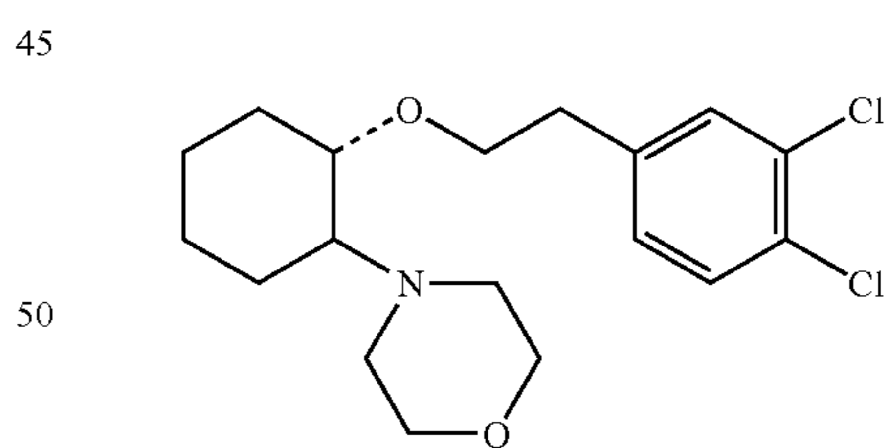
(1R,2R)/(1S,2S)-2-(4-morpholinyl)-1-(3,4-dichlorophenethoxy)cyclohexane
