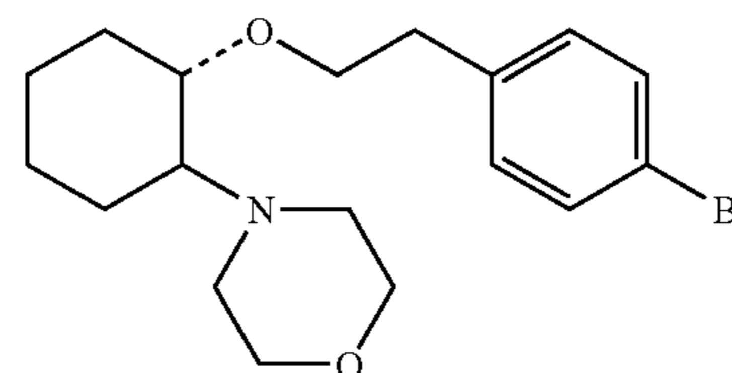
(1R,2R)/(1S,2S)-[2-(4-morpholinyl)-1-(4-bromophenethoxy)]cyclohexane
