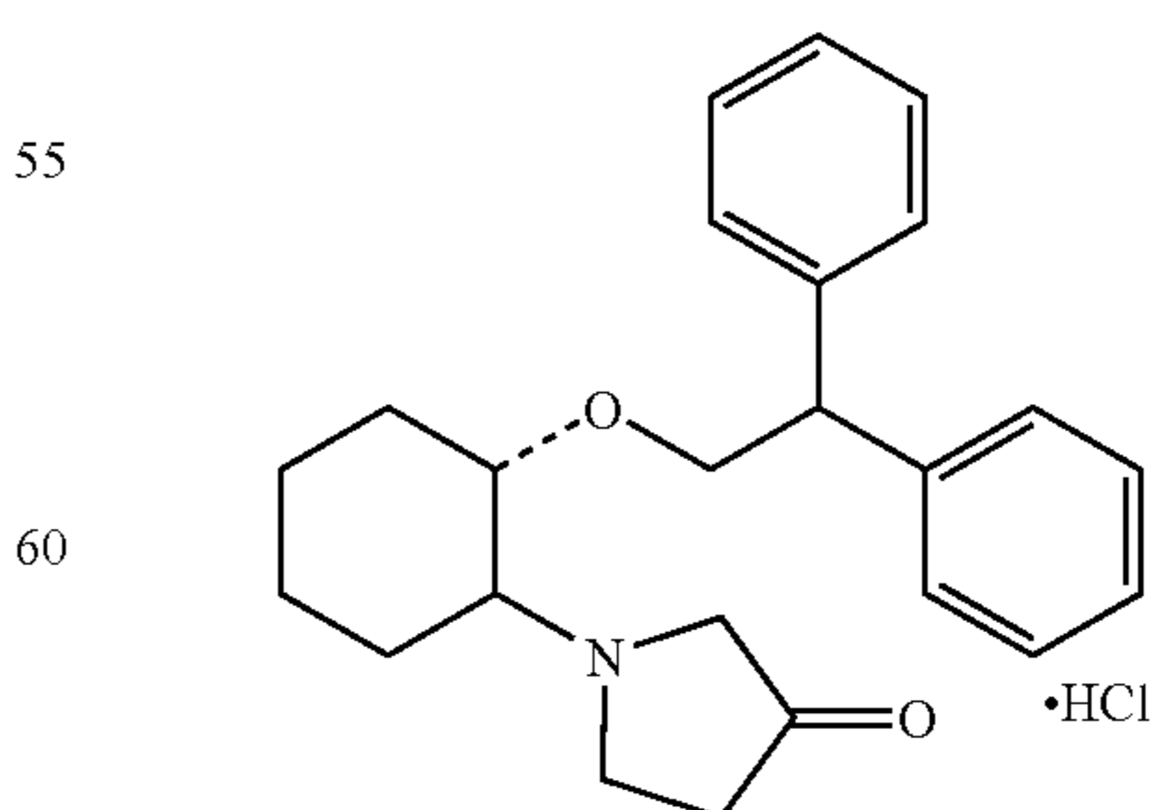
(1R,2R)/(1S,2S)-2-(3-ketopyrrolidinyl)-1-(2,2-diphenylethoxy)cyclohexane monohydrochloride
