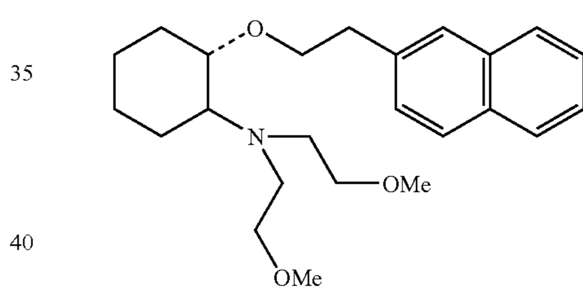
(1R,2R)/(1S,2S)-[2-[bis(2-methoxyethyl)aminyl]-1-(2-naphthenethoxy)]cyclohexane
