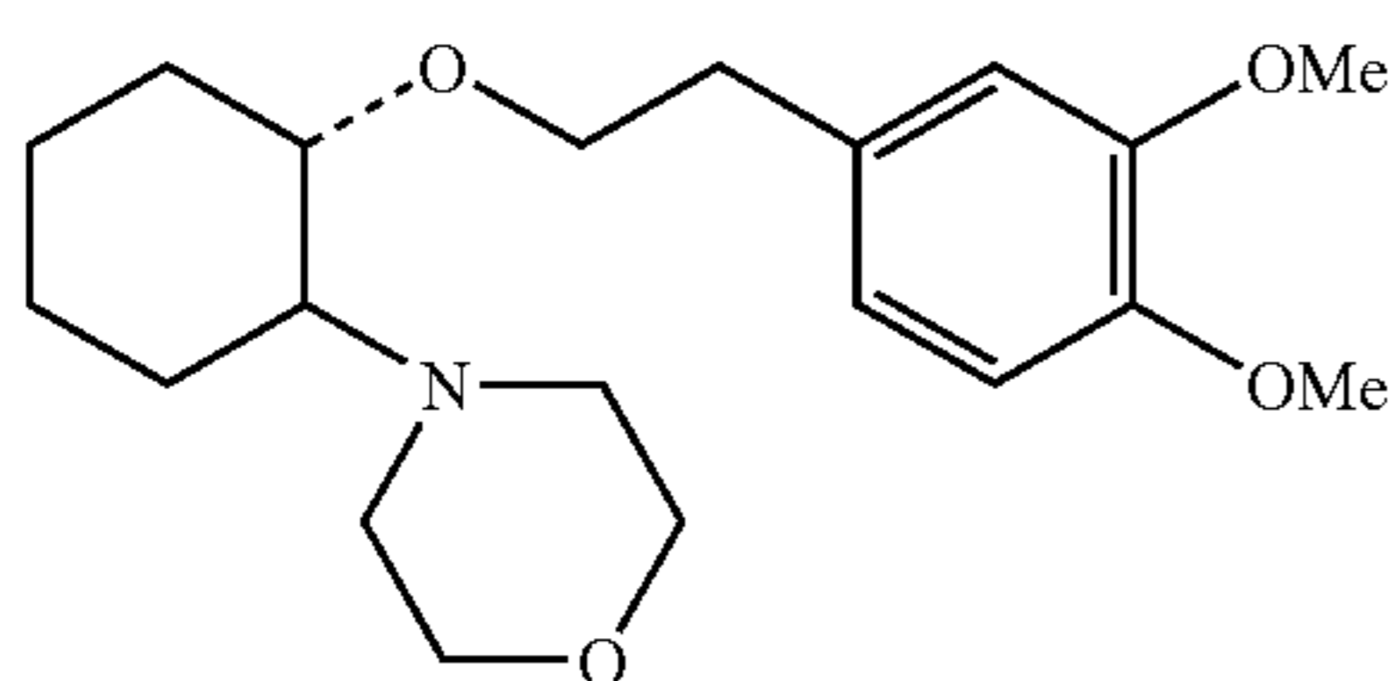
(1R,2R)/(1S,2S)-[2-(4-morpholinyl)-1-(3,4-dimethoxyphenethoxy)]cyclohexane
