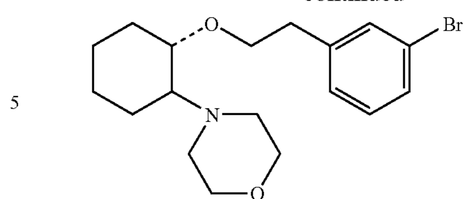
(1R,2R)/(1S,2S)-[2-(4-morpholinyl)-1-(3-bromophenethoxy)]cyclohexane
