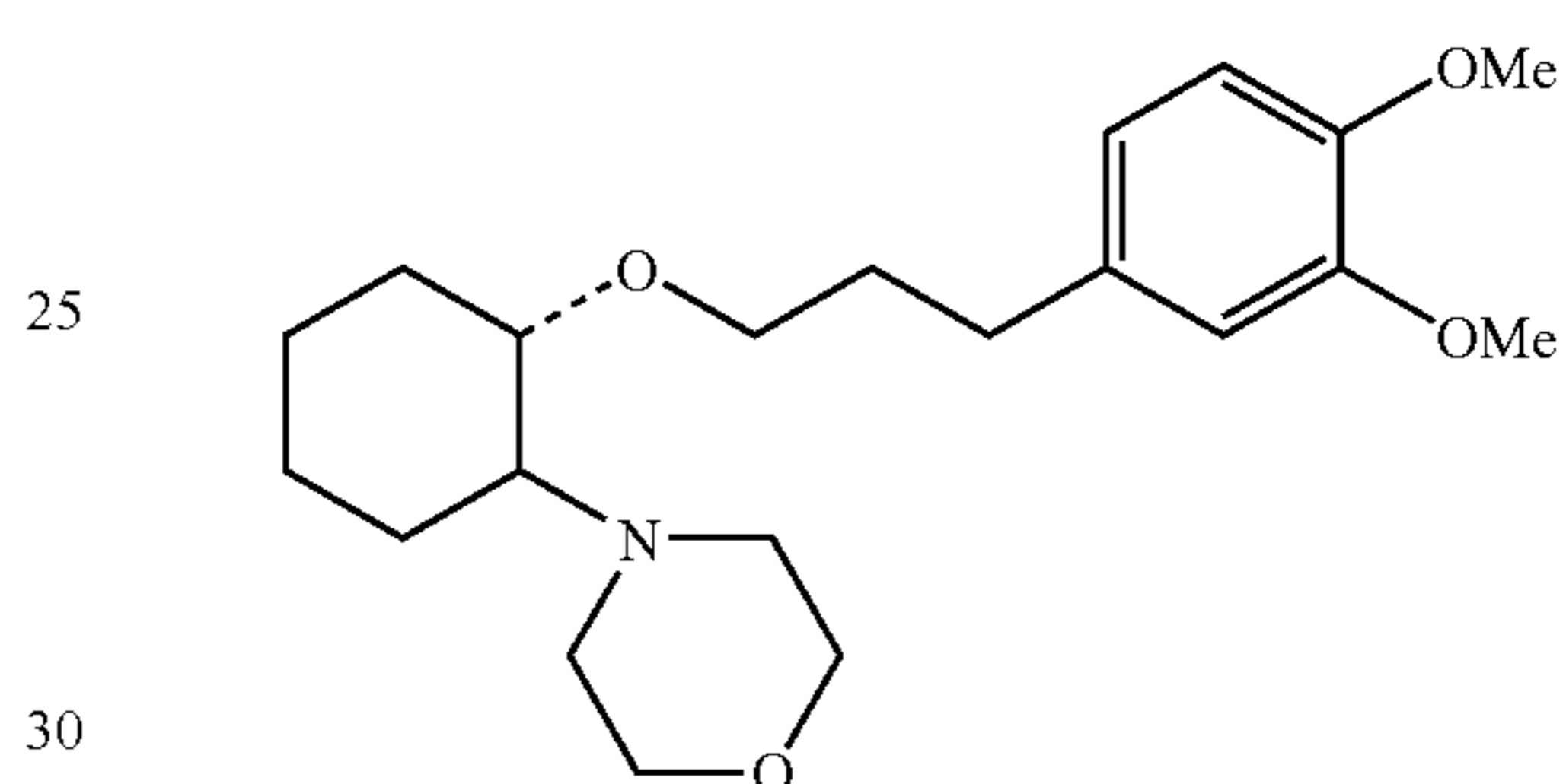
(1R,2R)/(1S,2S)-[2-(4-morpholinyl)-1-(3-(3,4-dimethoxyphenyl)propoxy)]cyclohexane
