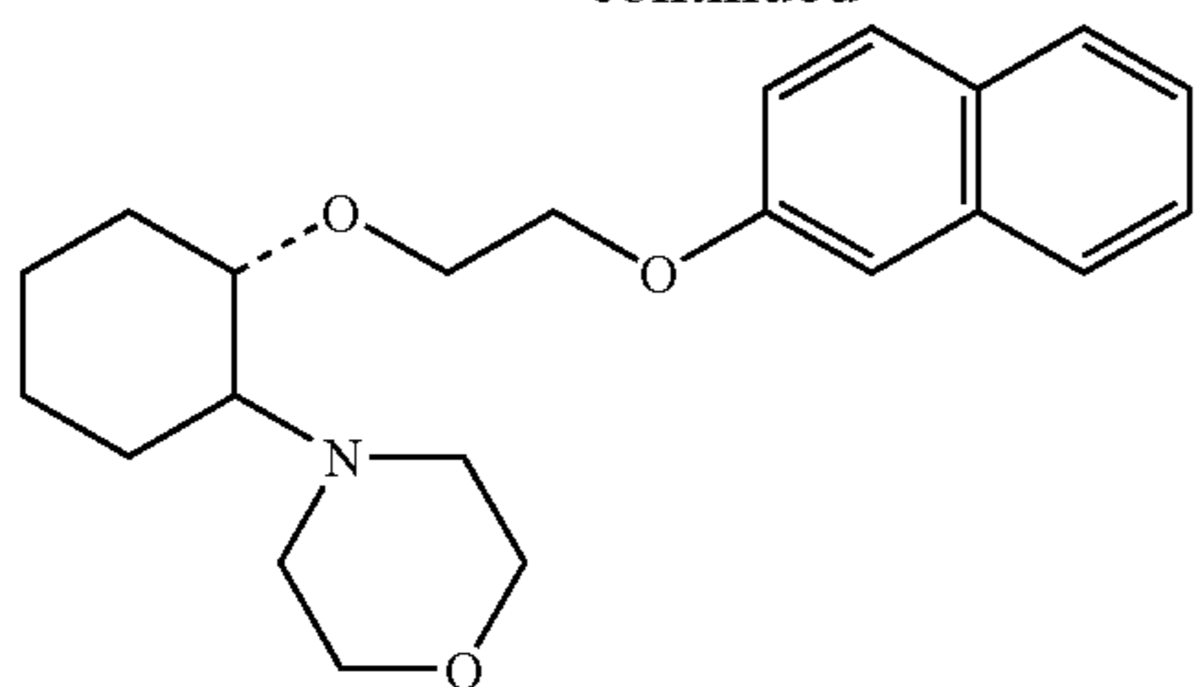
(1R,2R)/(1S,2S)-[2-(4-morpholinyl)-1-[2-(2-naphthoxy)ethoxy]]cyclohexane
