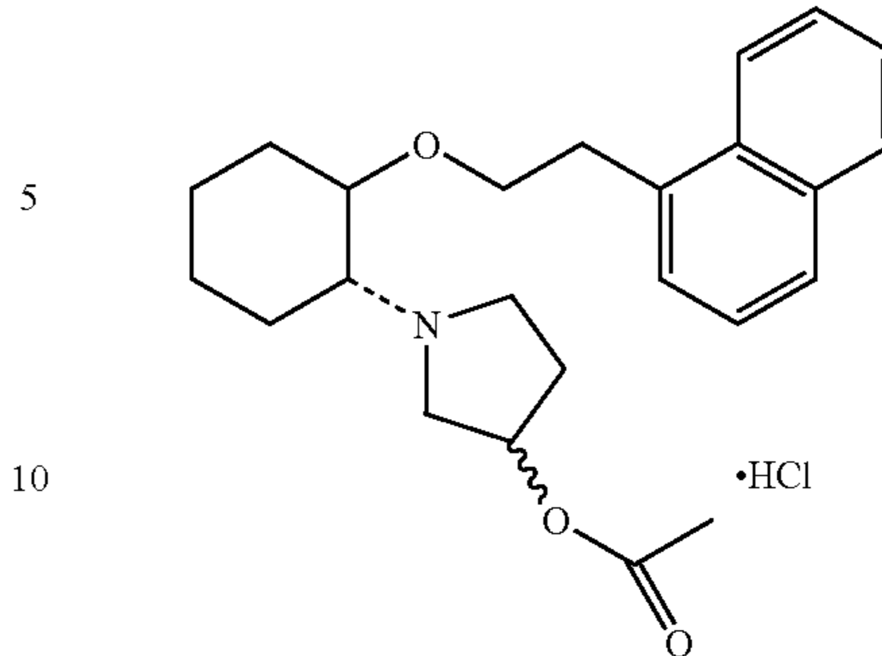
(1R,2R)/(1S,2S)-2-(3-acetoxypyrrolidinyl)-1-(1-naphthenethoxy)cyclohexane monohydrochloride
