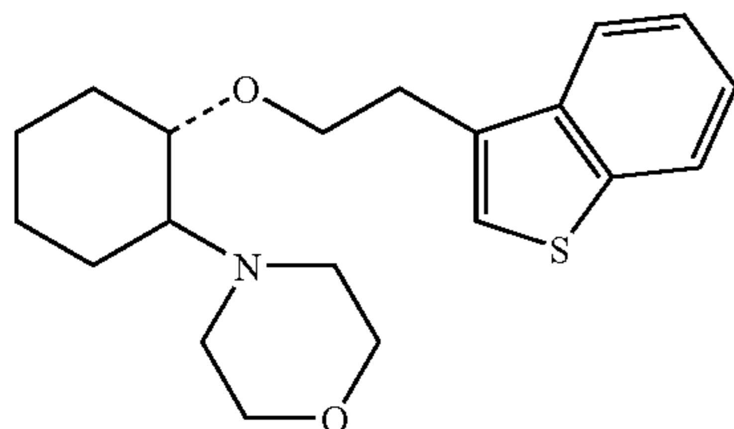
(1R,2R)/(1S,2S)-[2-(4-morpholinyl)-1-(2-benzo[b]thiophen-3-yl)]cyclohexane
