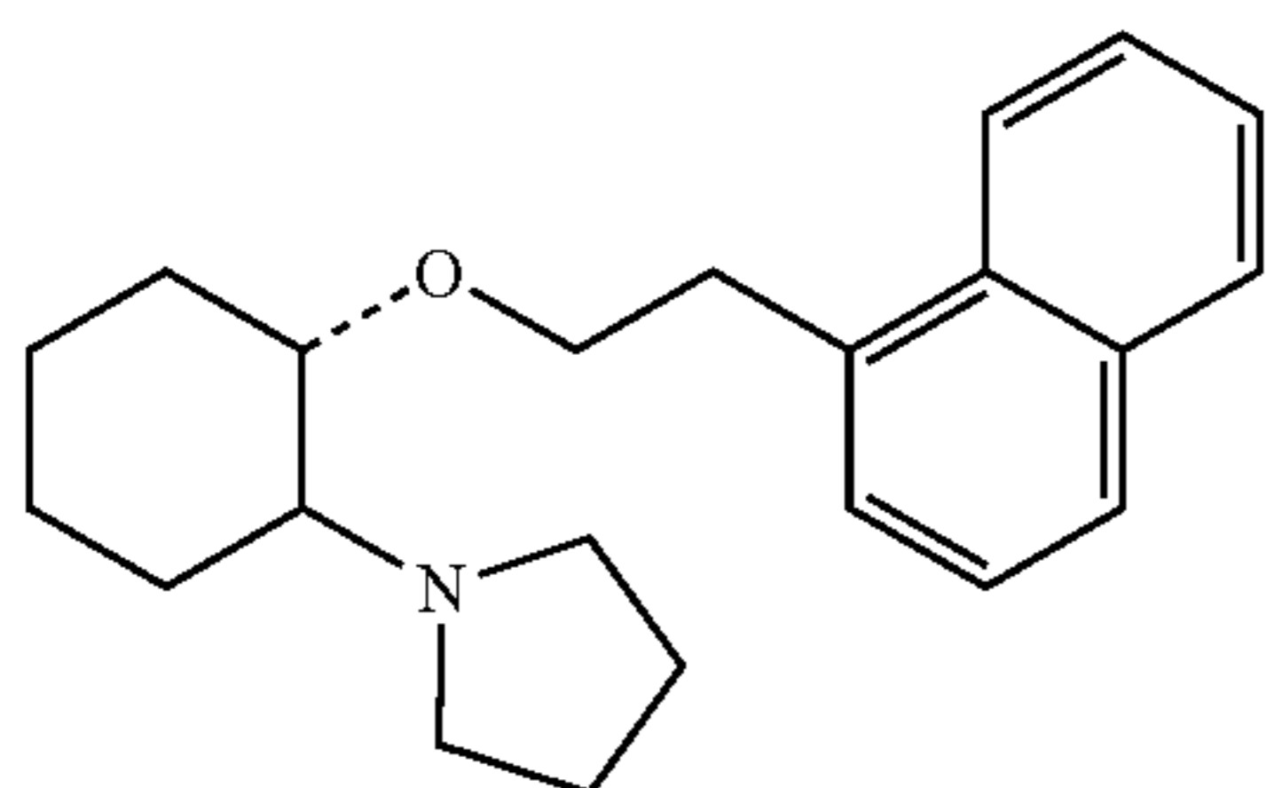
(1R,2R)/(1S,2S)-[2-(1-pyrrolidinyl)-1-(1-naphthenethoxy)]cyclohexane
