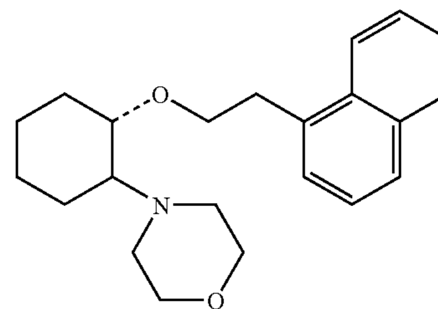
(1R,2R)/(1S,2S)-[2-(4-morpholinyl)-1-(1-naphthenethoxy)]cyclohexane
