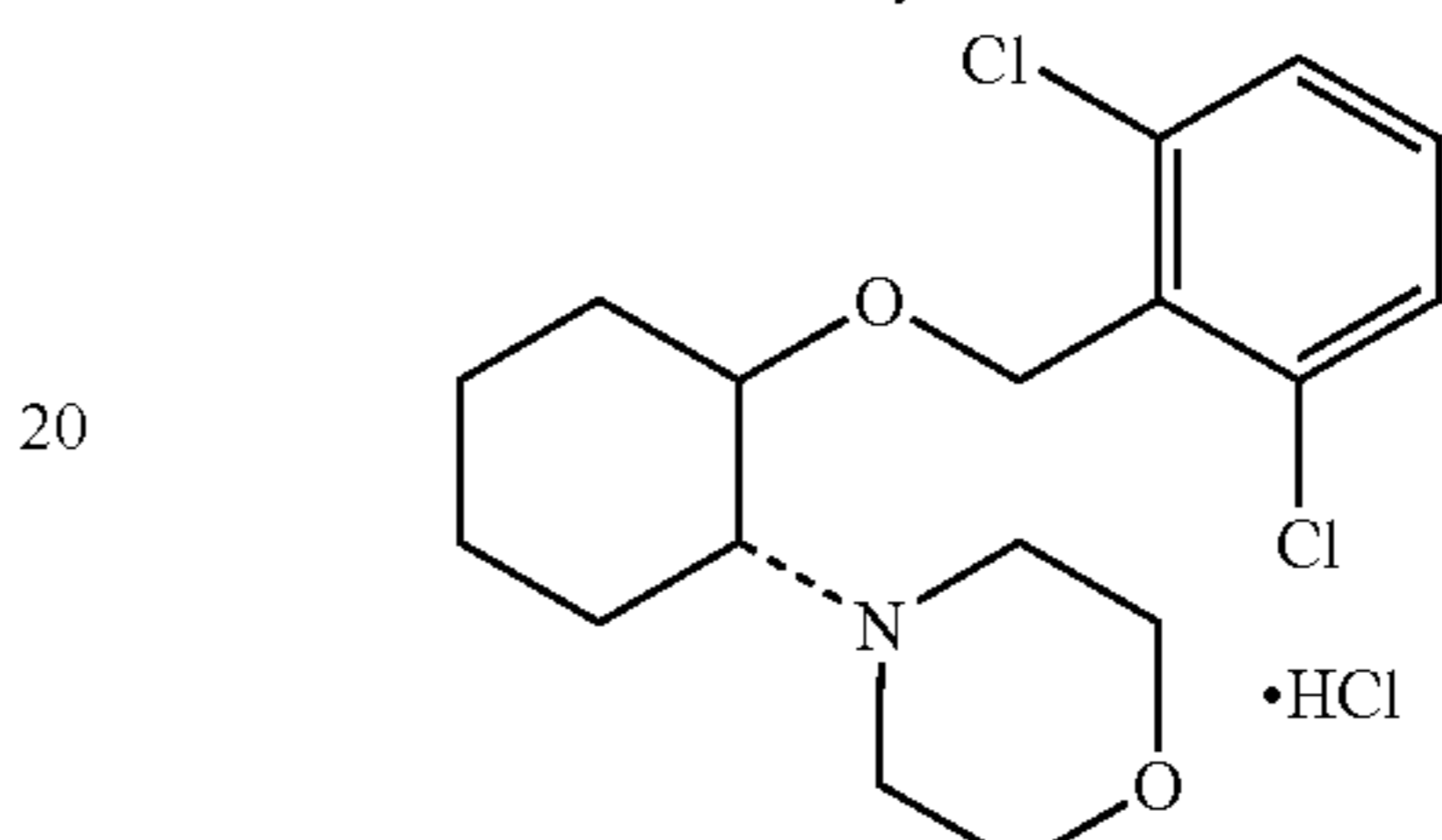
(1R,2R)/(1S,2S)-2-(4-morpholinyl)-1-[(2,6-dichlorophenyl)methoxy]cyclohexane monohydrochloride
