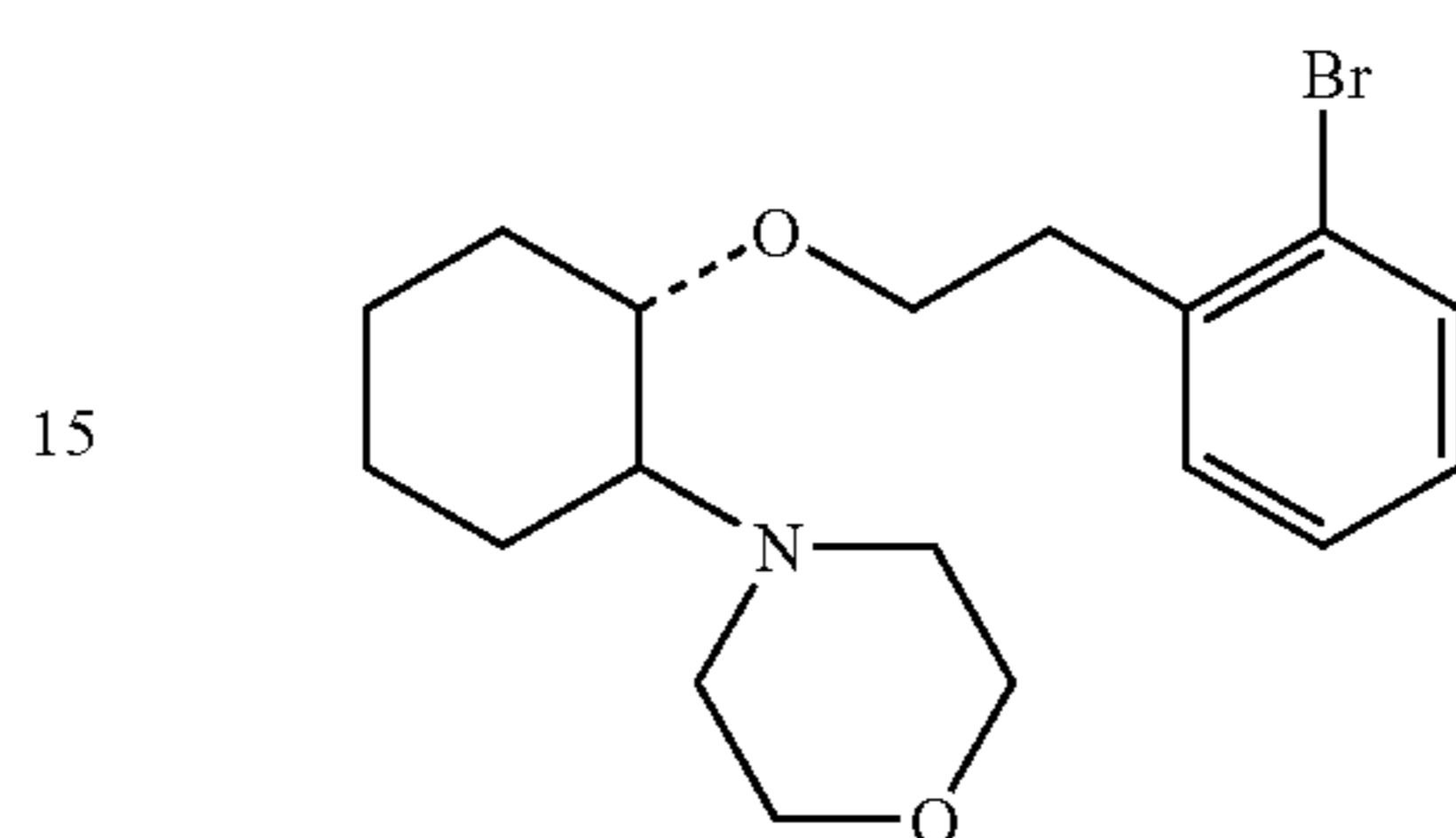
(1R,2R)/(1S,2S)-[2-(4-morpholinyl)-1-(2-bromophenethoxy)]cyclohexane
