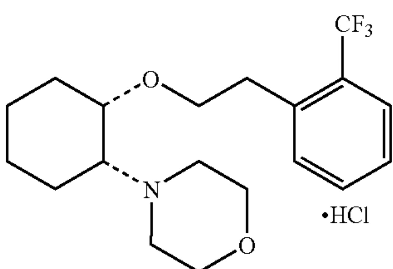
(1R,2S)/(1S,2R)-2-(4-morpholinyl)-1-[2-(trifluoromethyl)phenethoxy]cyclohexane monohydrochloride
