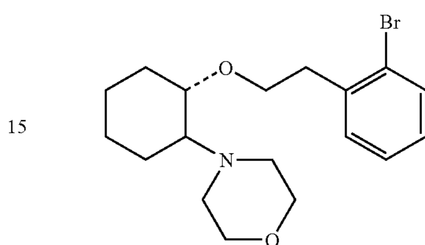
(1R,2R)/(1S,2S)-[2-(4-morpholinyl)-1-(2-bromophenethoxy)]cyclohexane
