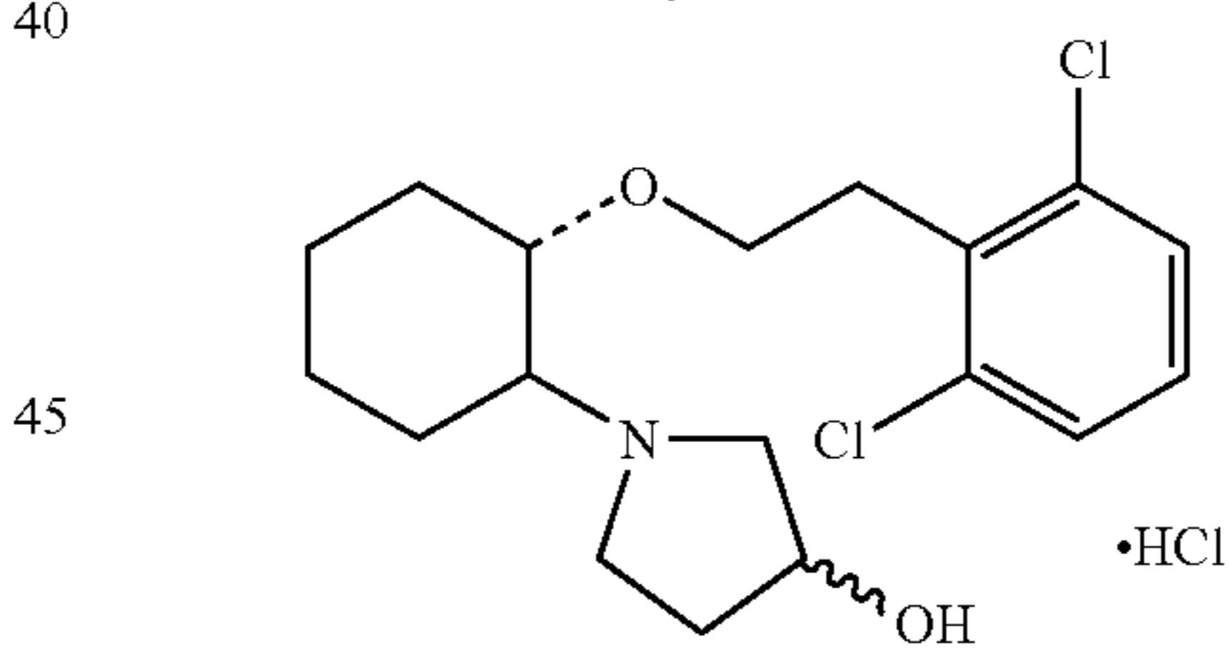
(1R,2R)/(1S,2S)-2-(3-hydroxypyrrolidinyl)-1-(2,6-dichlorophenethoxy)cyclohexane monohydrochloride
