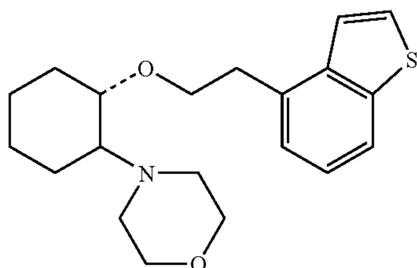
(1R,2R)/(1S,2S)-[2-(4-morpholinyl)-1-(2-benzo[b]thiophen-4-yl)]cyclohexane
