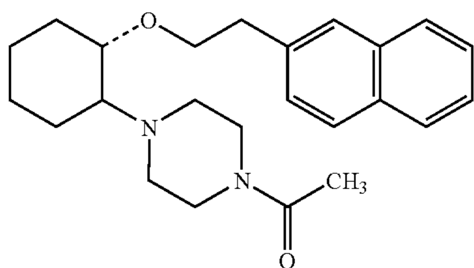
(1R,2R)/(1S,2S)-2-(1-acetylpiperazinyl)-1-(2-naphthenethoxy)cyclohexane
