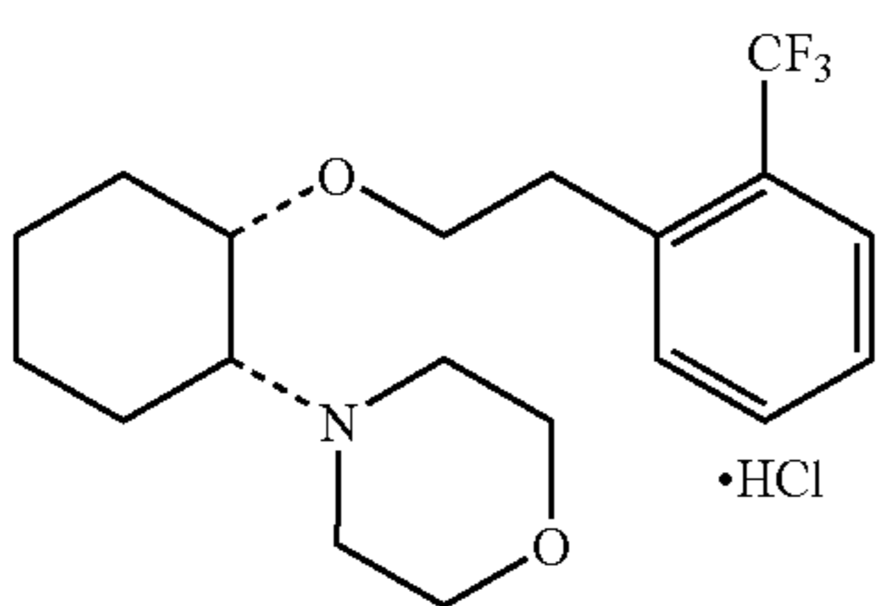
(1R,2S)/(1S,2R)-2-(4-morpholinyl)-1-[2-(trifluoromethyl)phenethoxy]cyclohexane monohydrochloride
