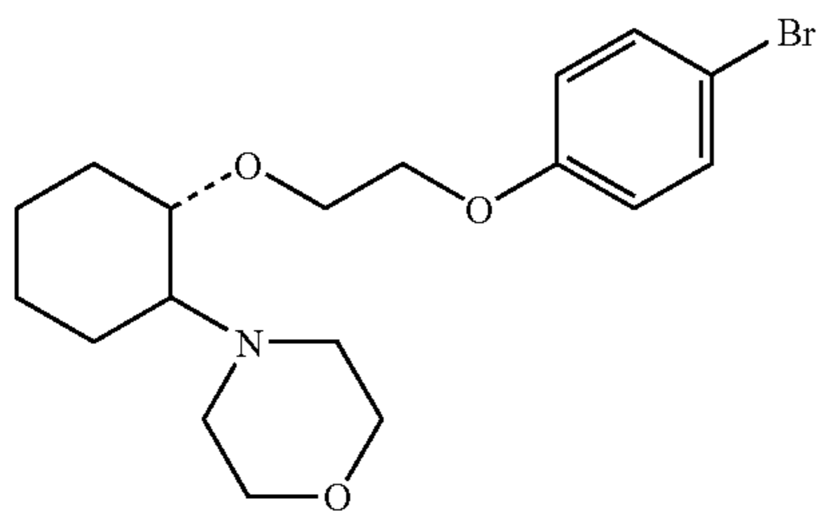
(1R,2R)/(1S,2S)-[2-(4-morpholinyl)-1-[2-(4-bromophenoxy)ethoxy]]cyclohexane
