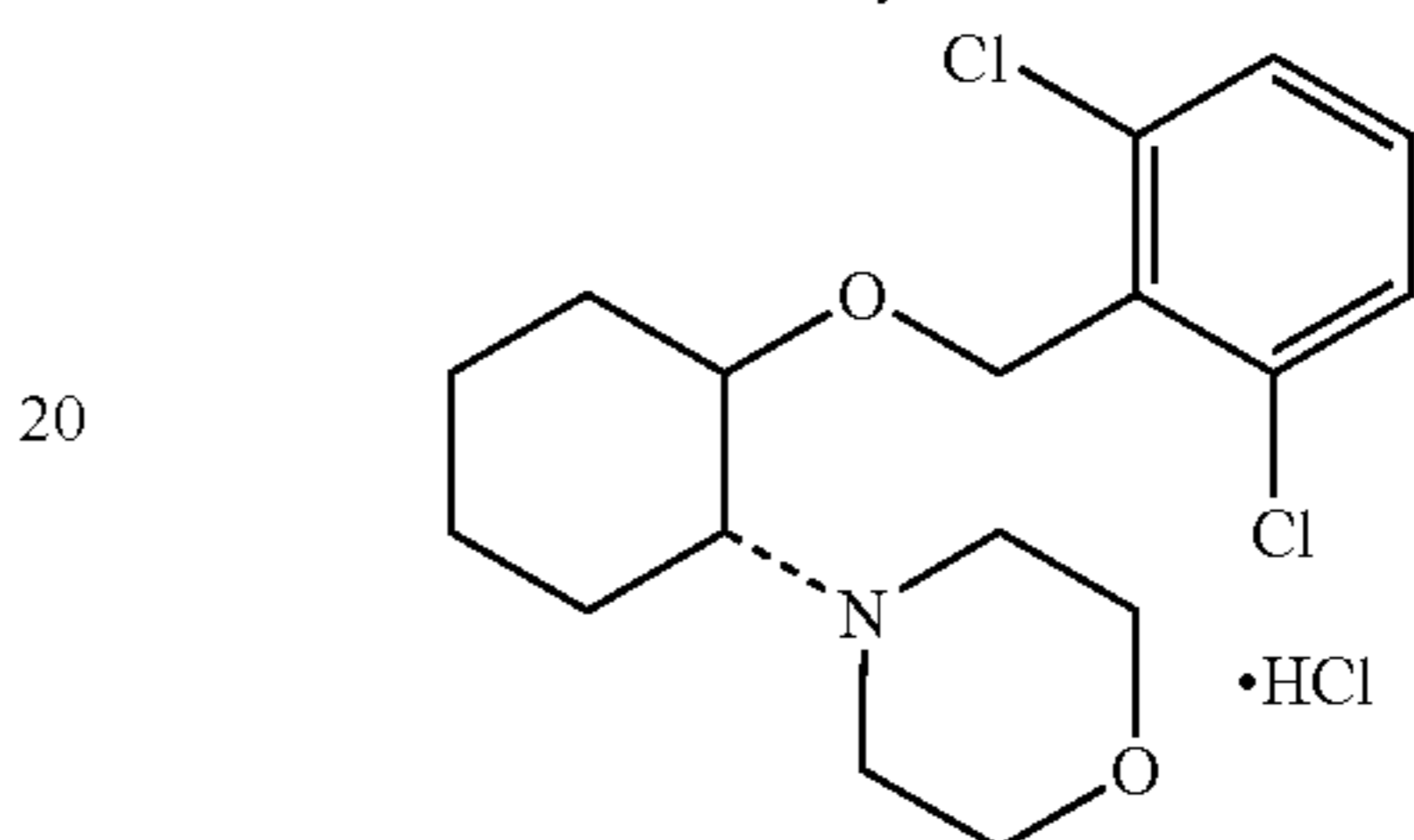
(1R,2R)/(1S,2S)-2-(4-morpholinyl)-1-[(2,6-dichlorophenyl)methoxy]cyclohexane monohydrochloride
