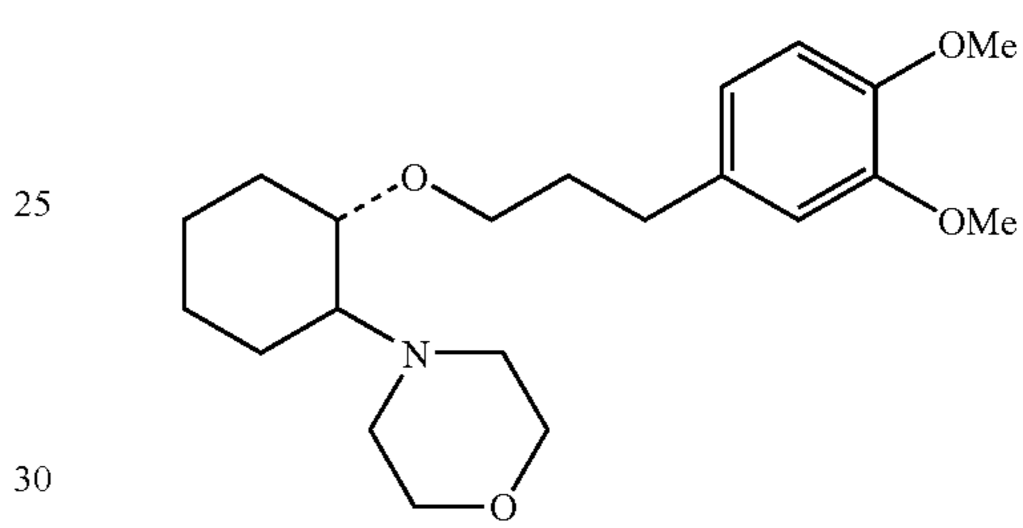
(1R,2R)/(1S,2S)-[2-(4-morpholinyl)-1-(3-(3,4-dimethoxyphenyl)propoxy)]cyclohexane
