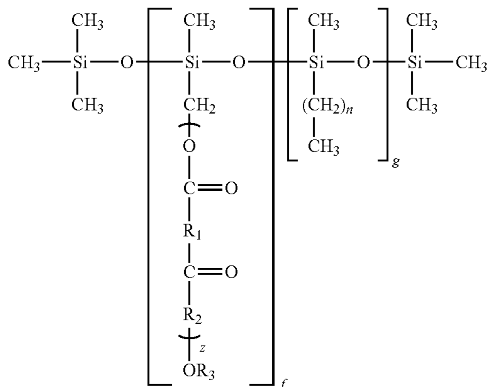
FORMULA (4)
