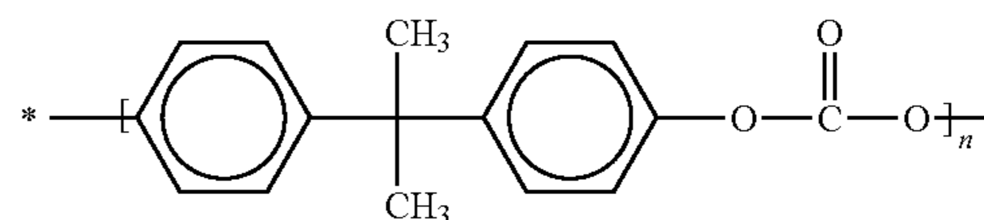
Formula (A)
