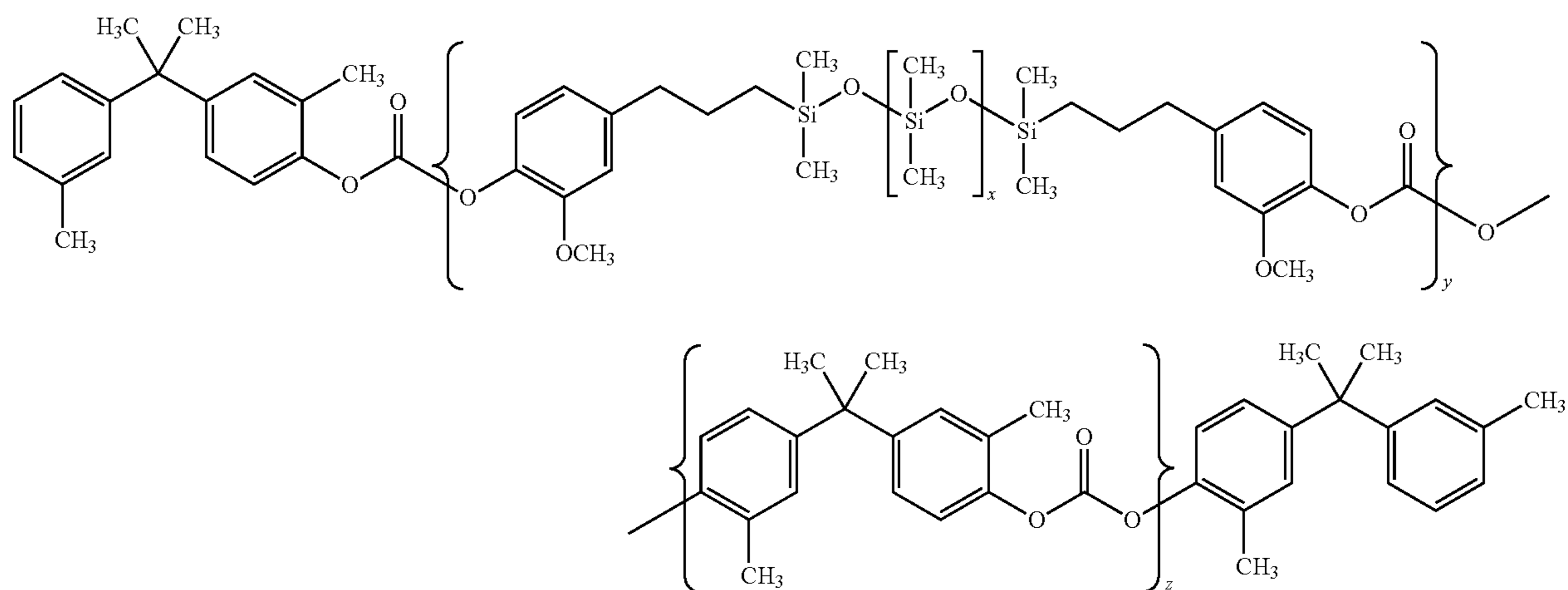
Formula (III)
