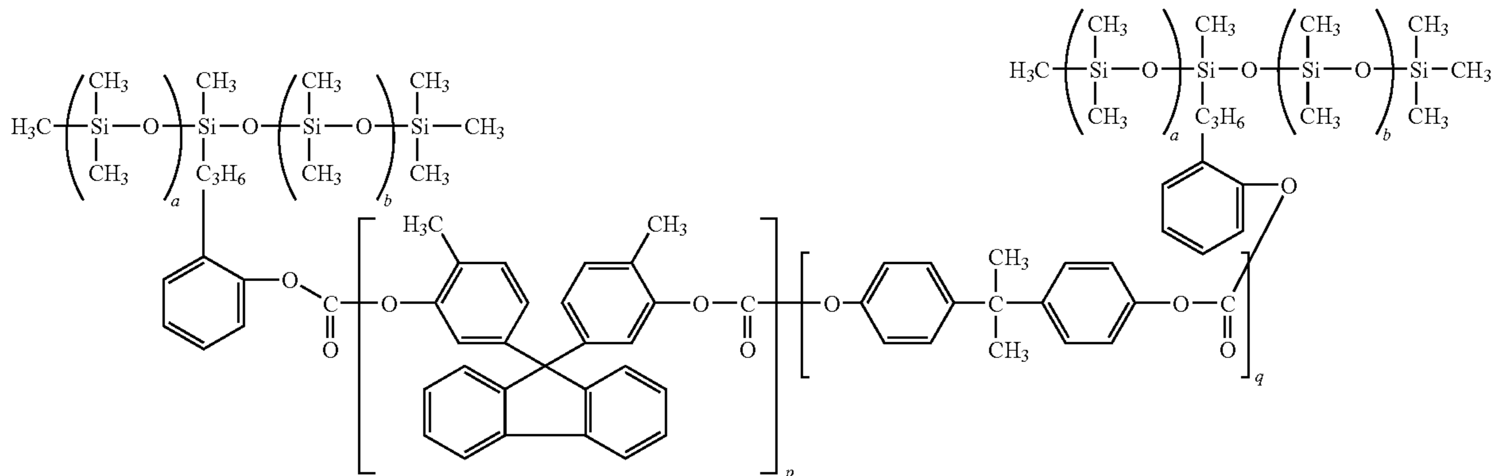
Formula (V)
