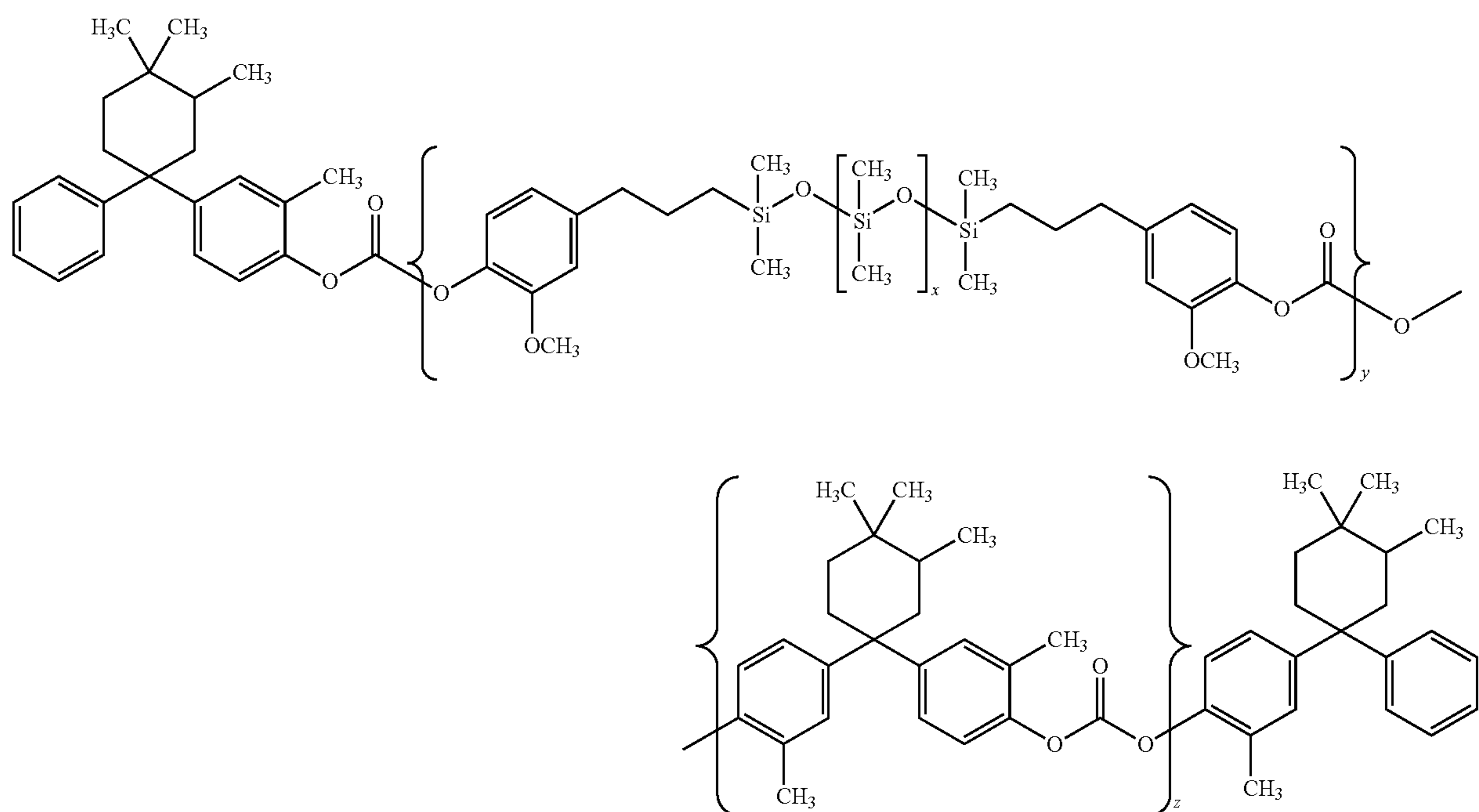
Formula (IV)
