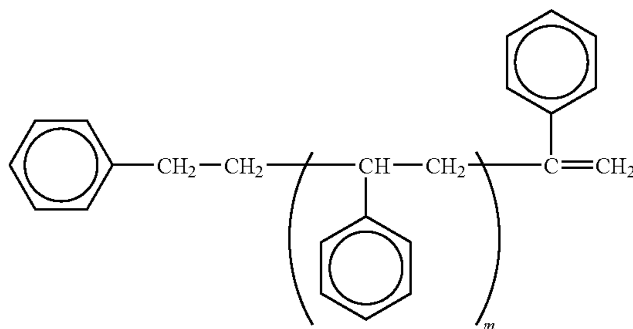
Formula (3)
