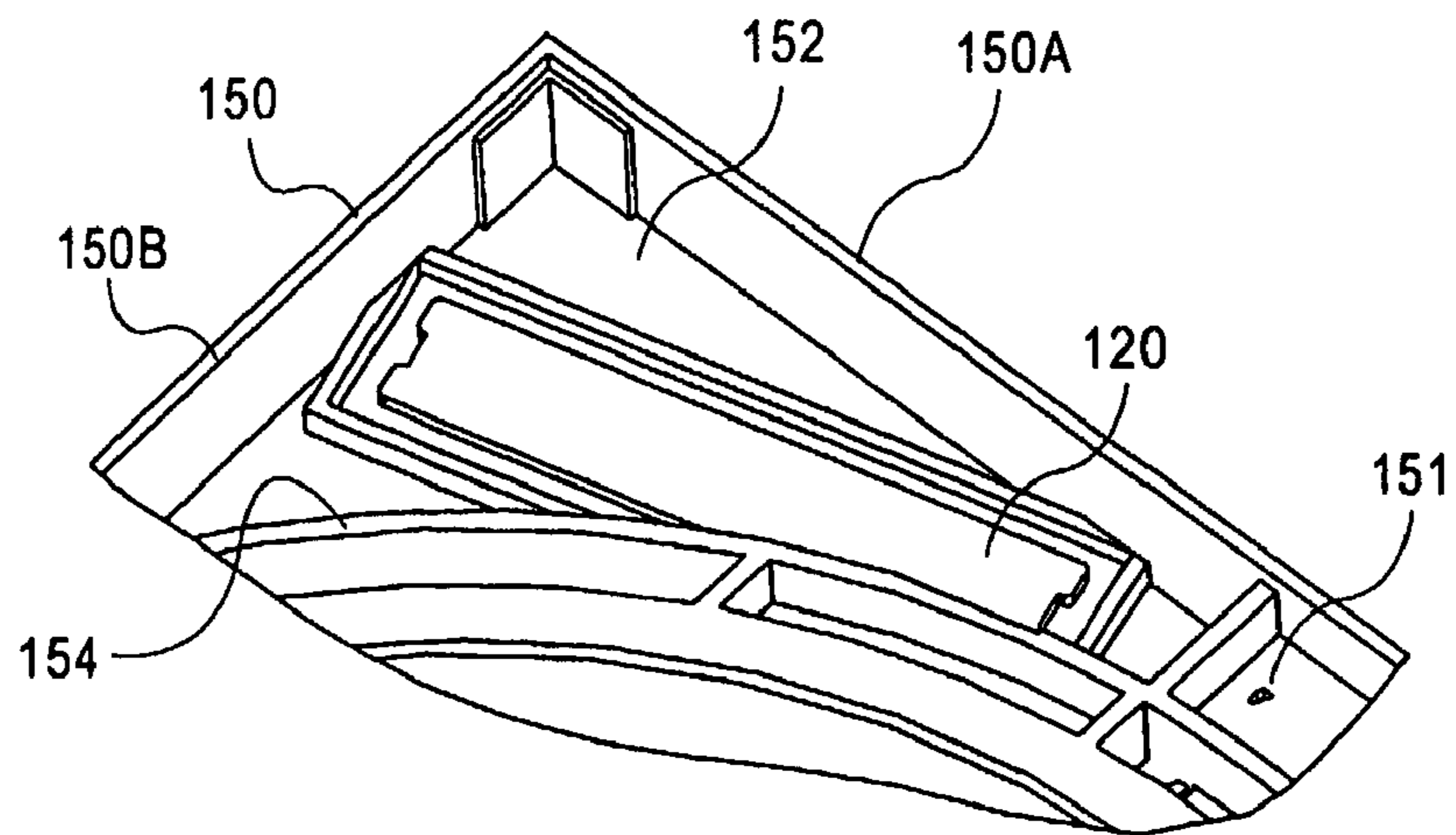
DETAIL A
