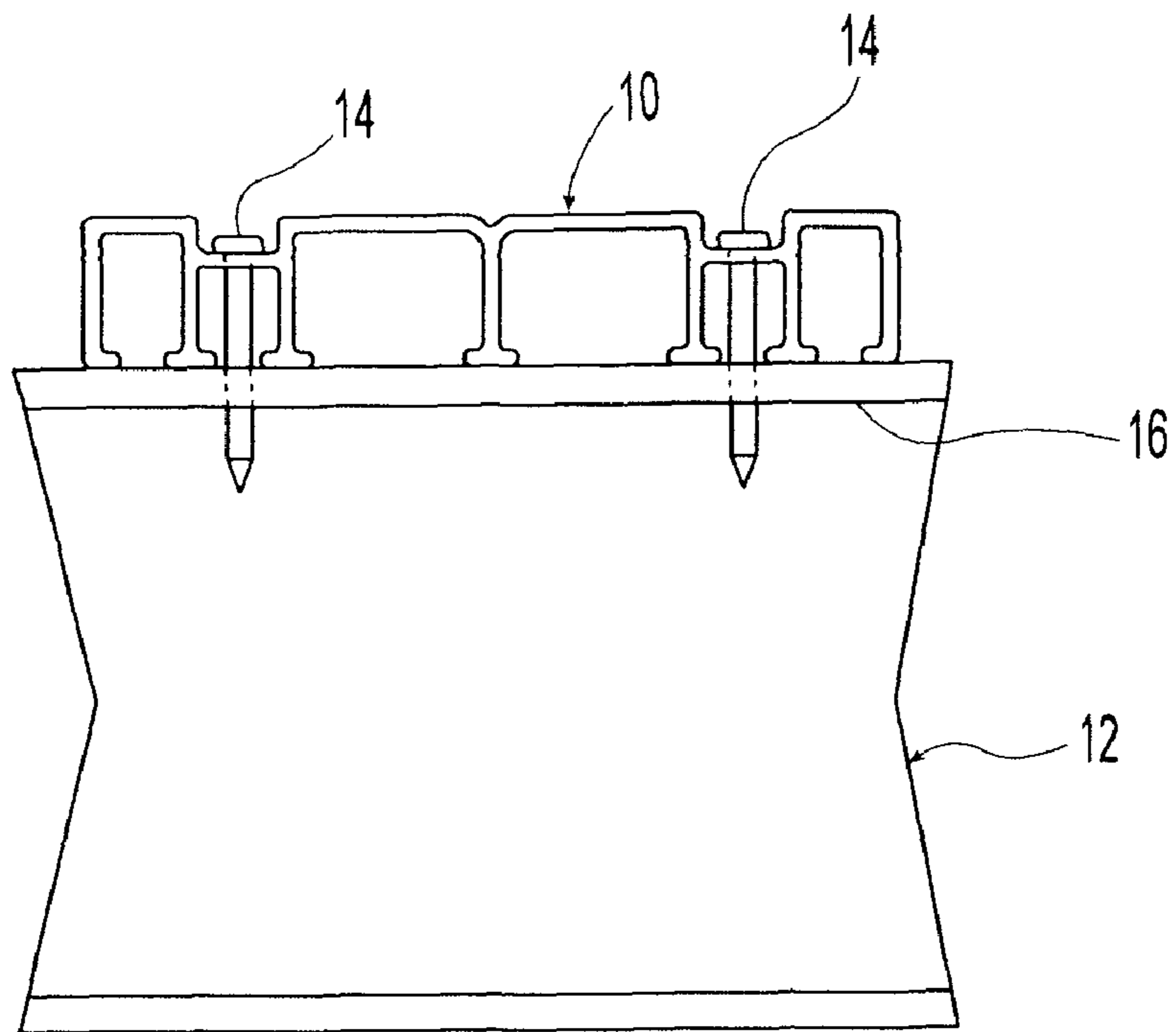
Fig. 1 (Prior Art)
