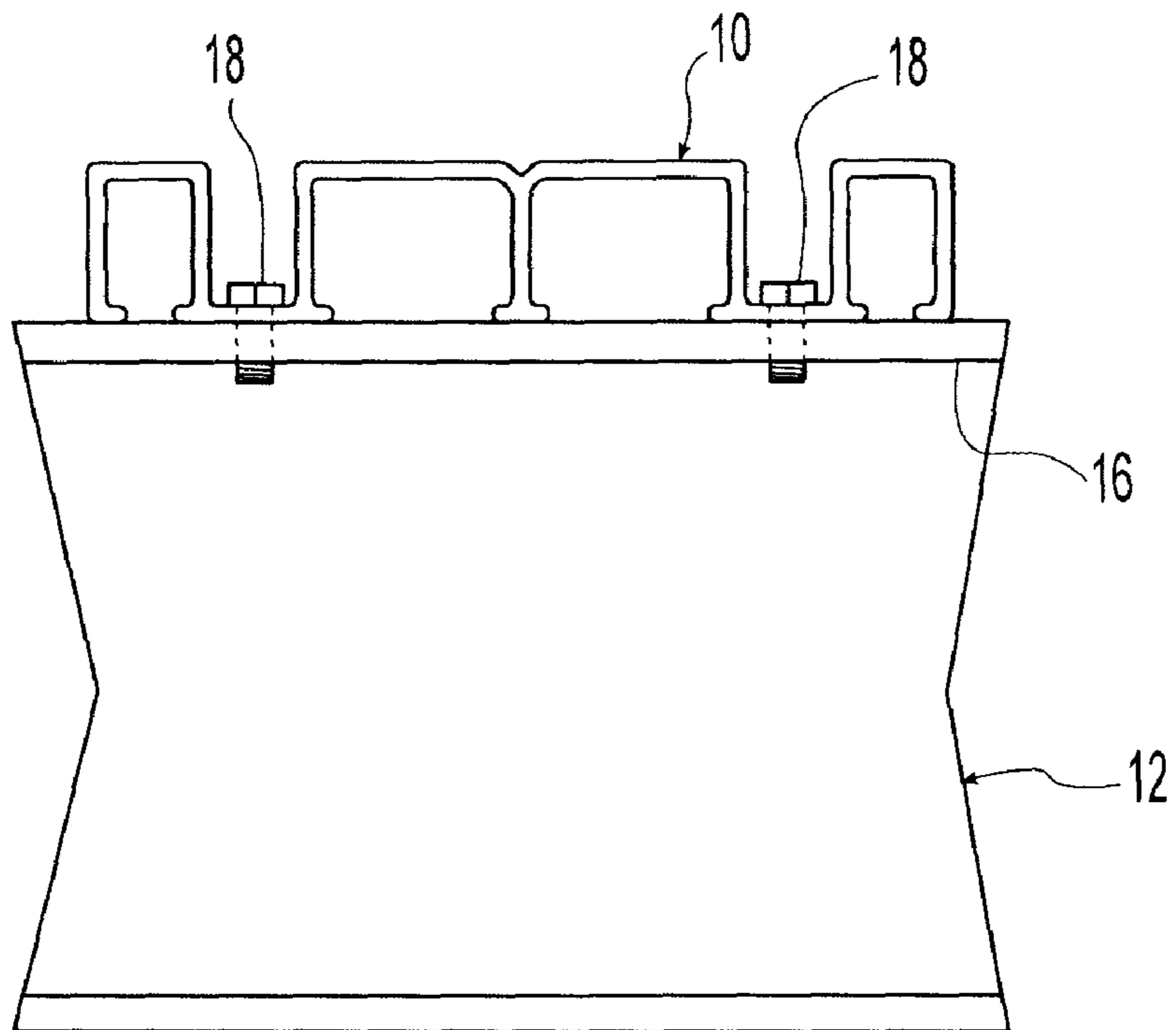
Fig. 3 (Prior Art)
