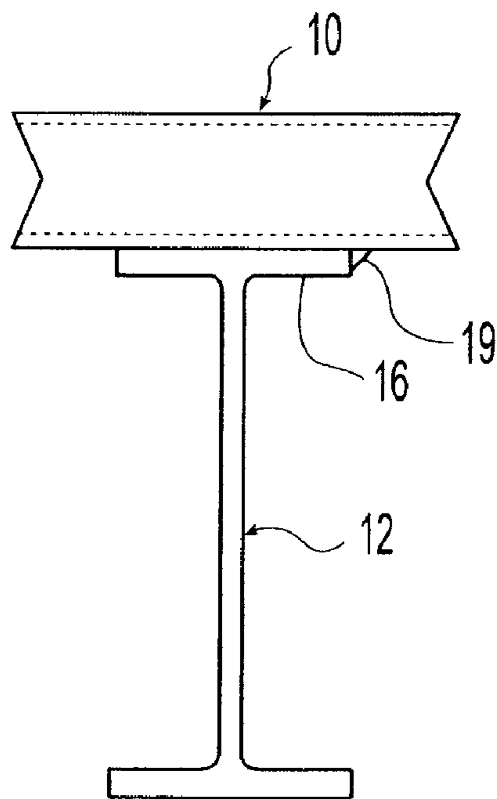
Fig. 5 (Prior Art)
