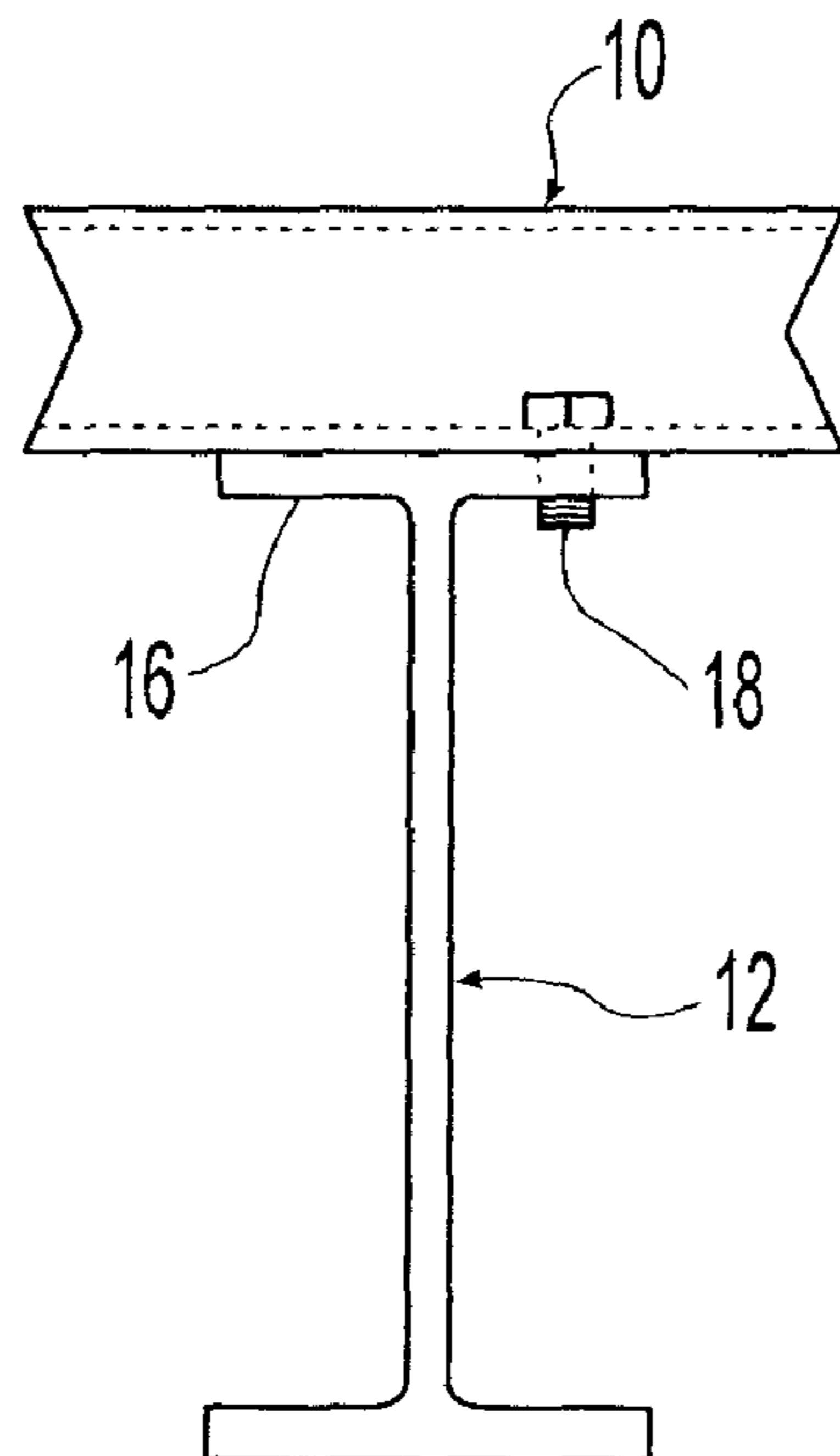
Fig. 4 (Prior Art)
