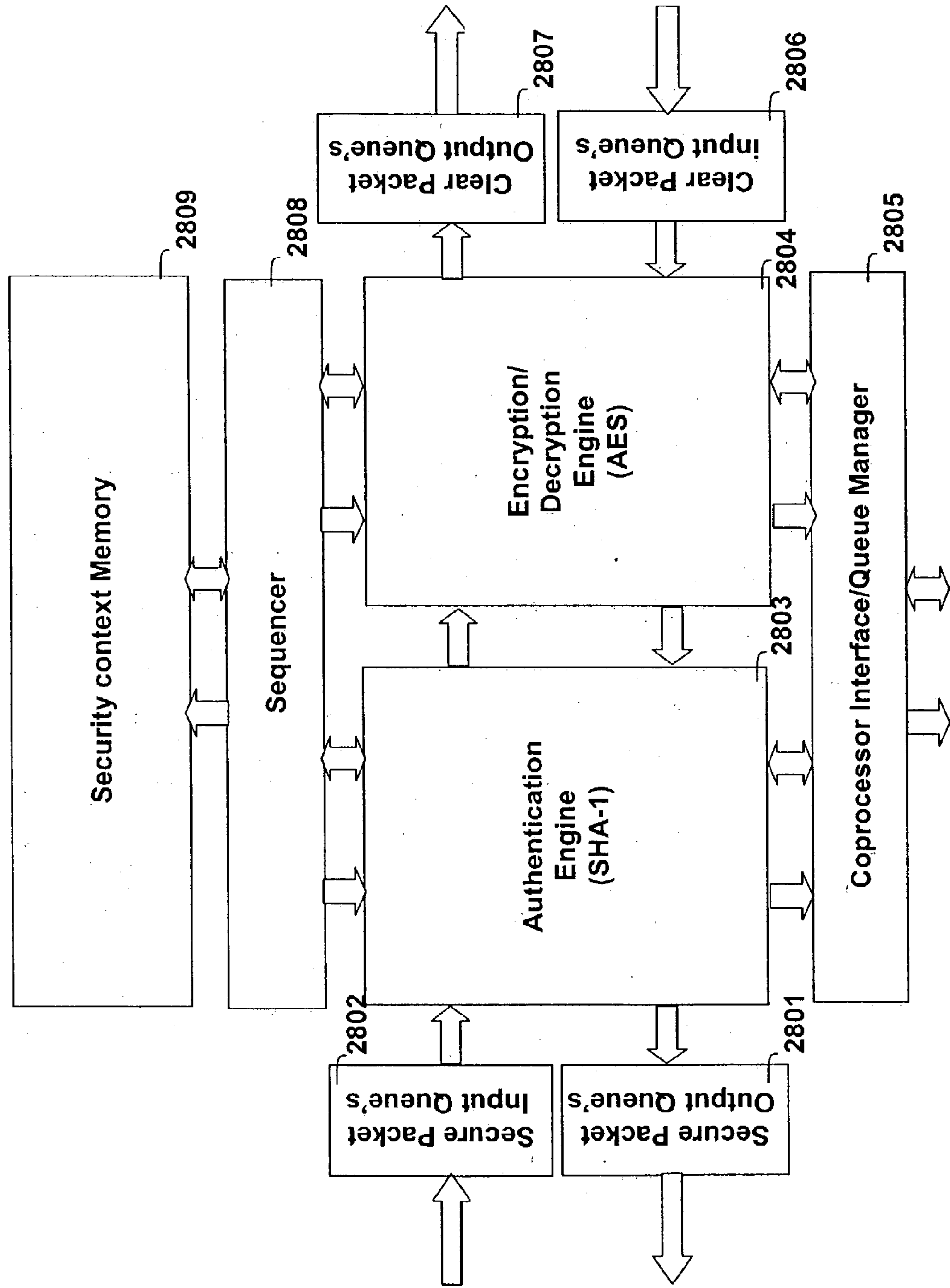
Fig. 28 Security Engine
