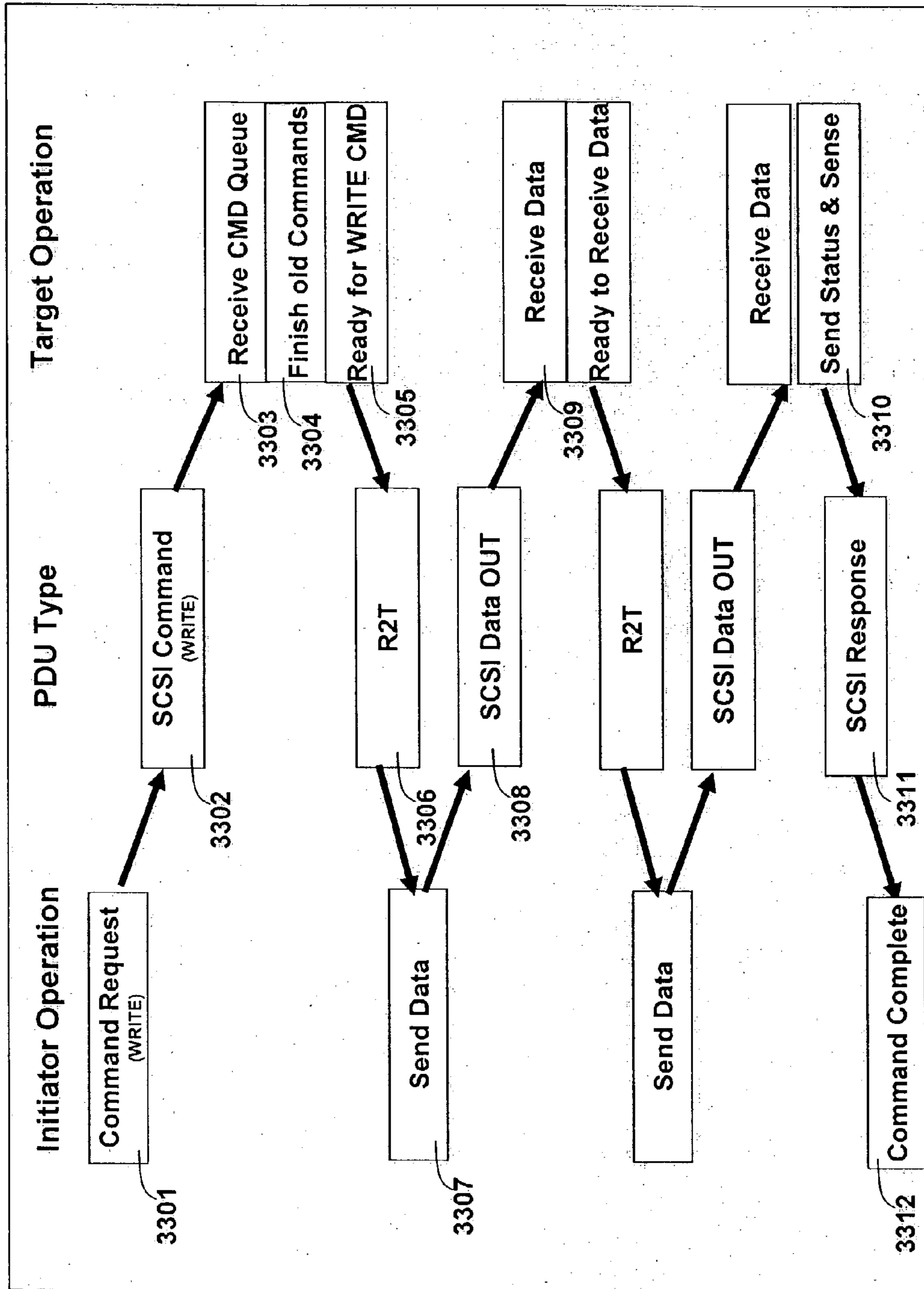
Fig. 33 Write Operation
