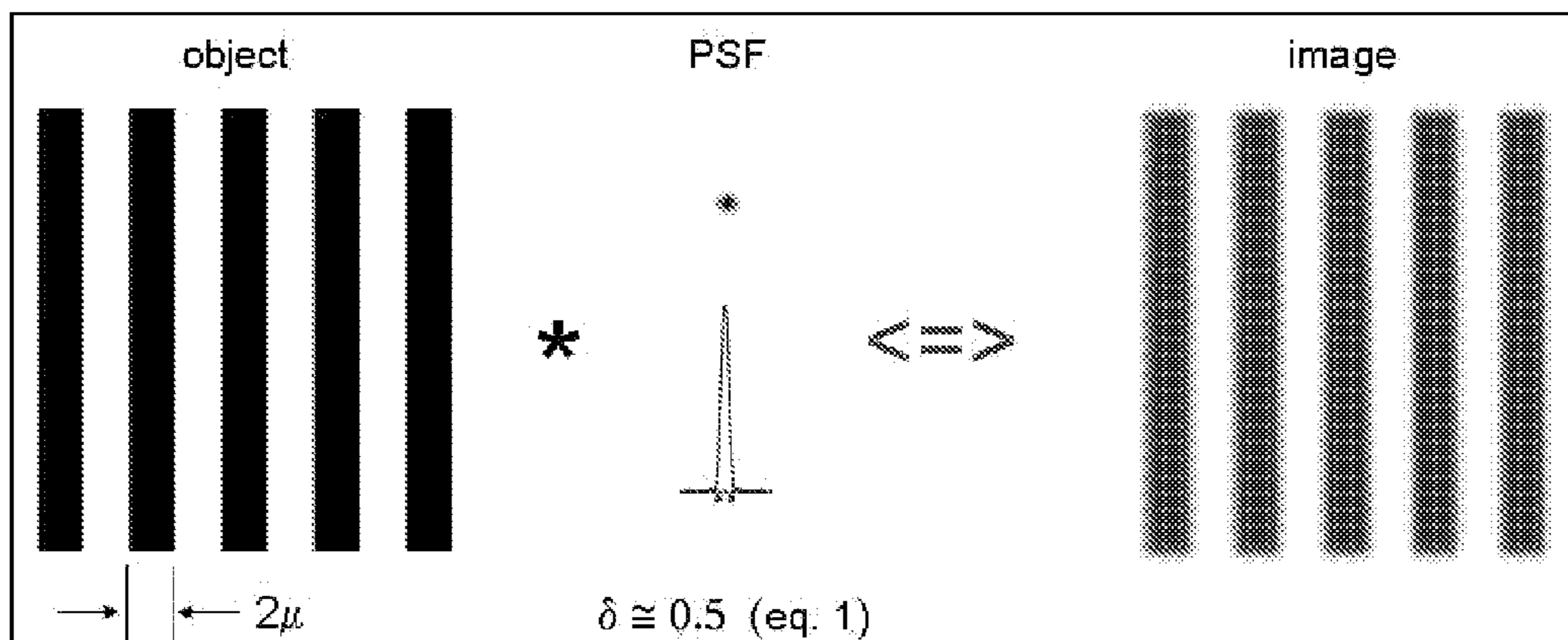
FIG. 8 (PRIOR ART)
