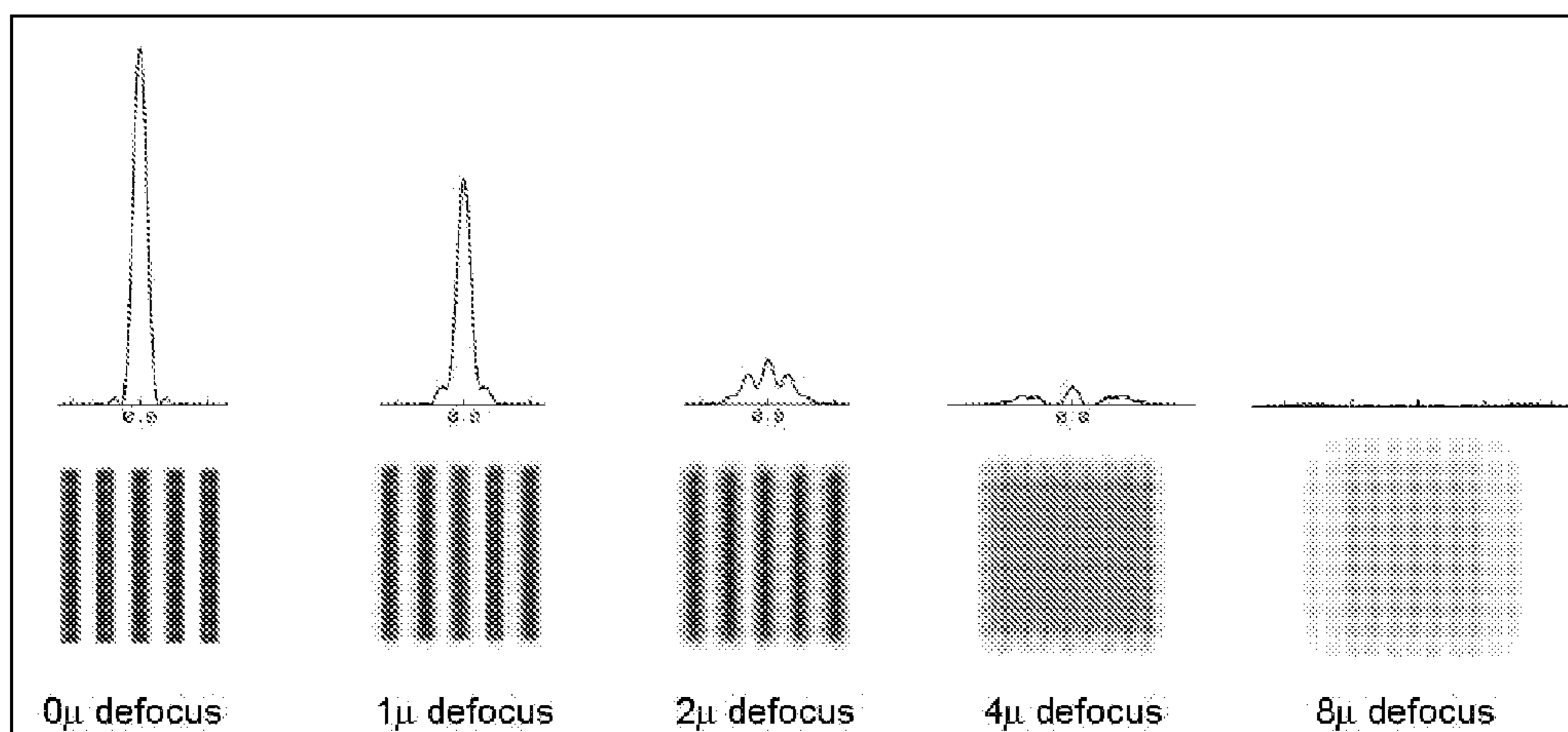
FIG. 9 (PRIOR ART)
