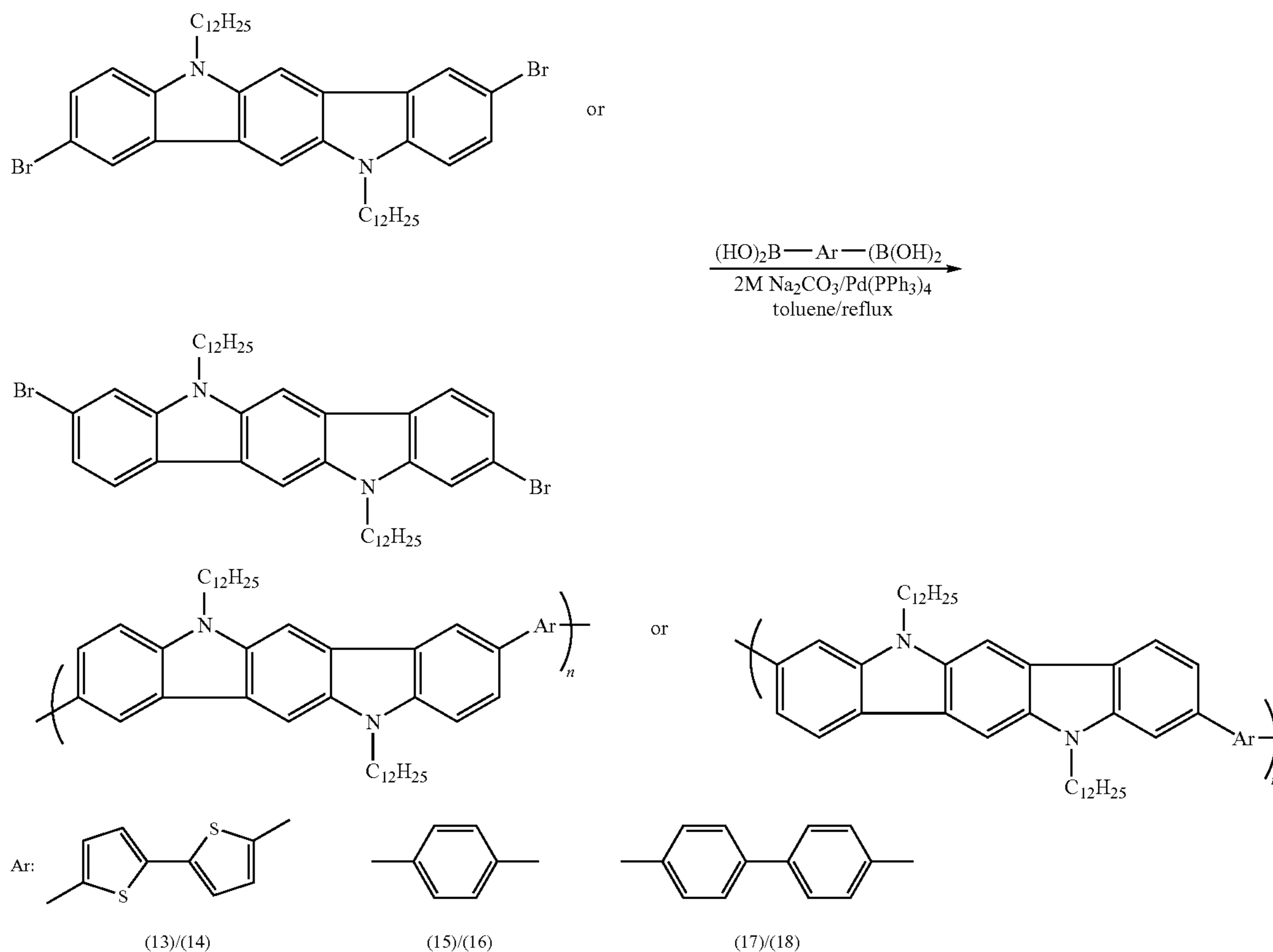
Scheme 2. Synthesis of polymer (13) through (18).
