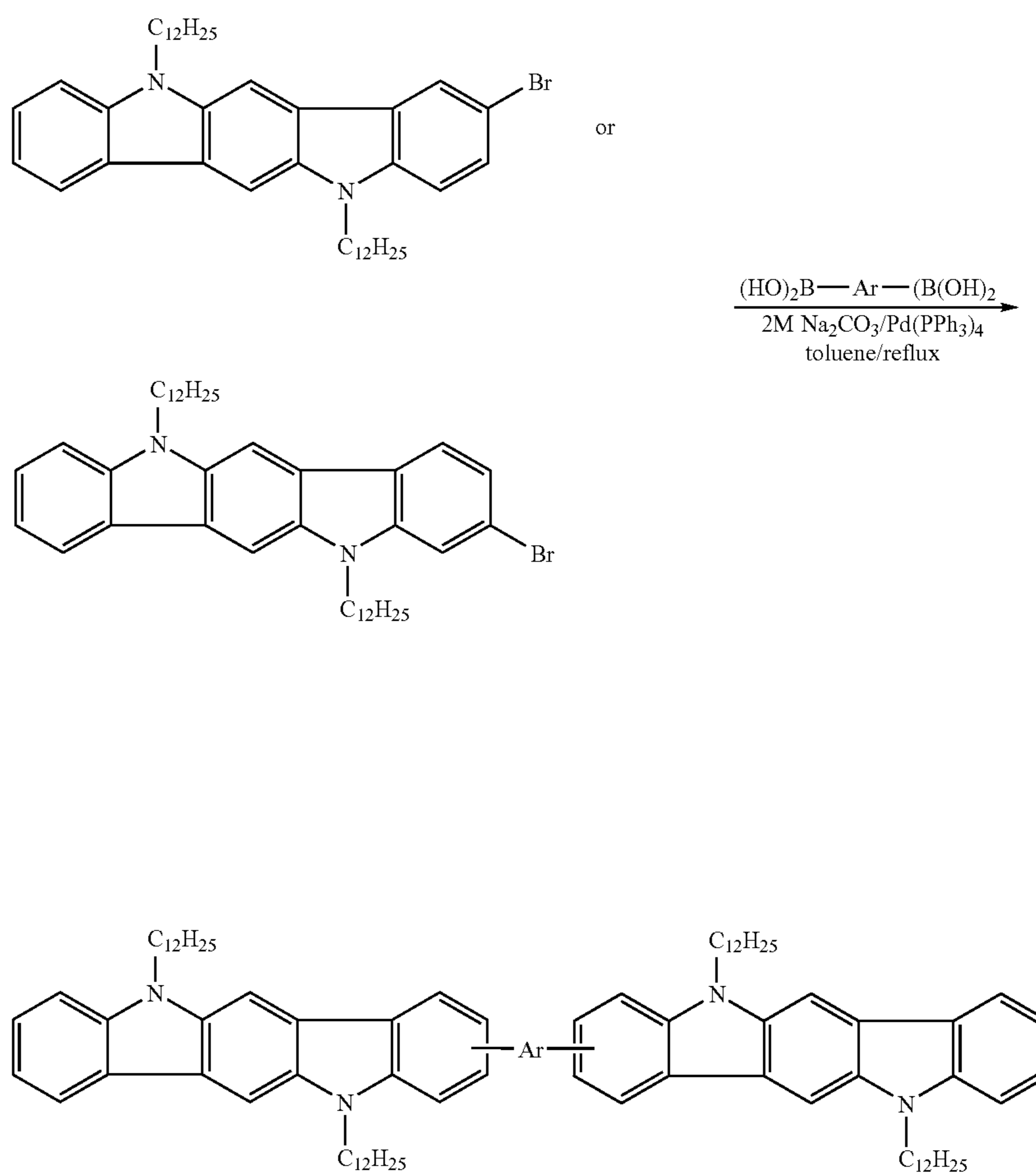
Scheme 1. Synthesis of Compound (1), (2), and (9) through (12).
