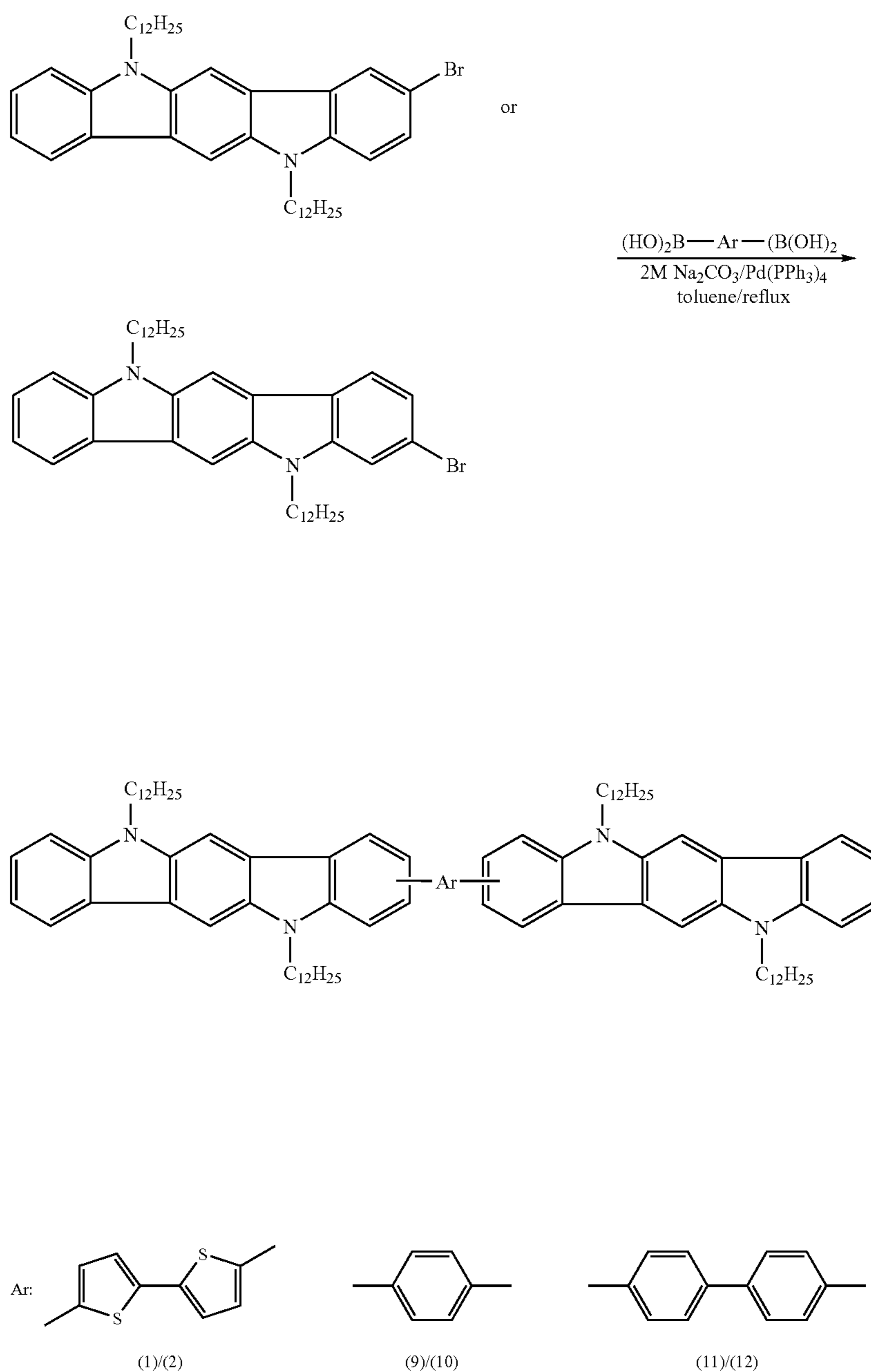
Scheme 1. Synthesis of Compound (1), (2), and (9) through (12).
