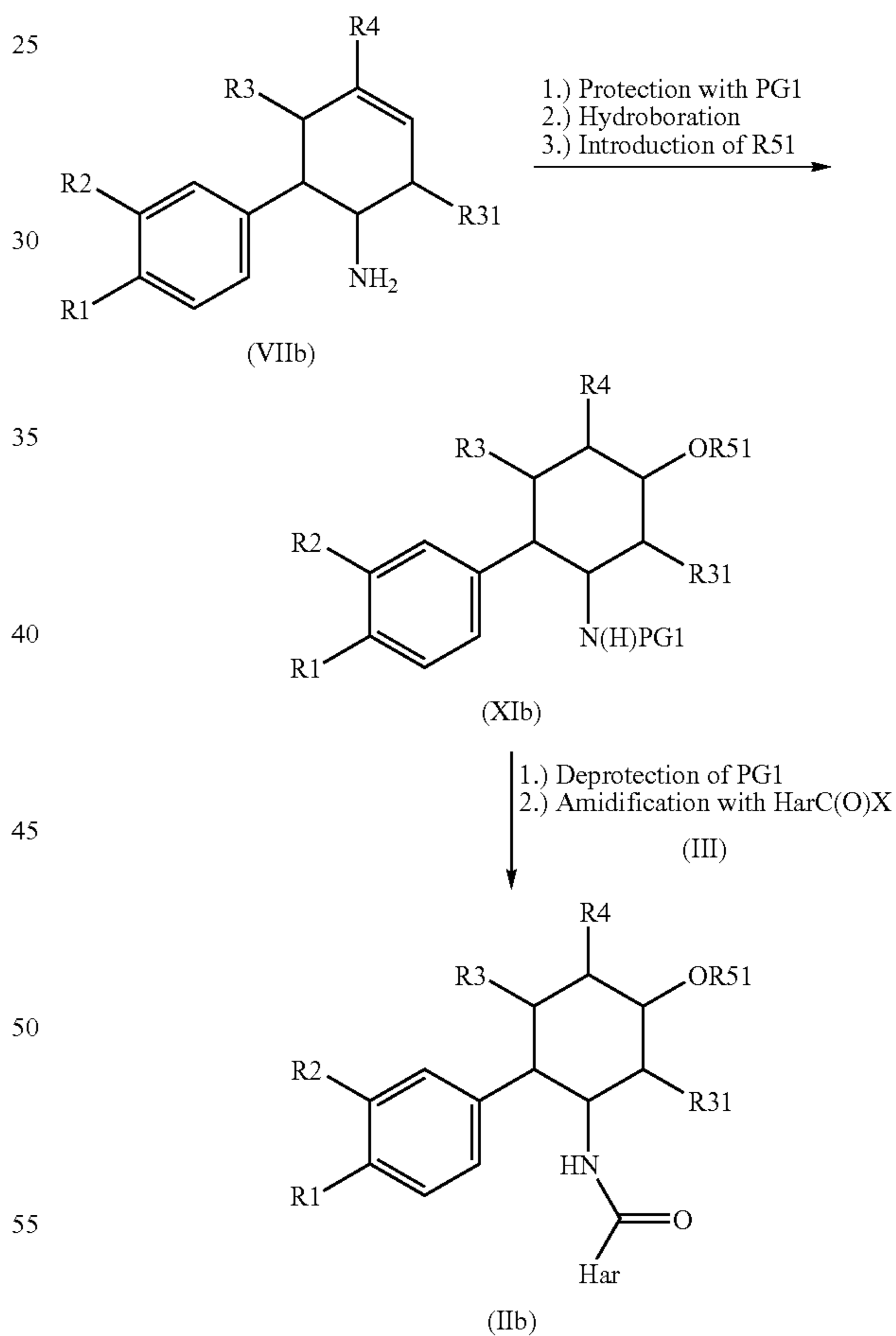
Reaction scheme 6:
