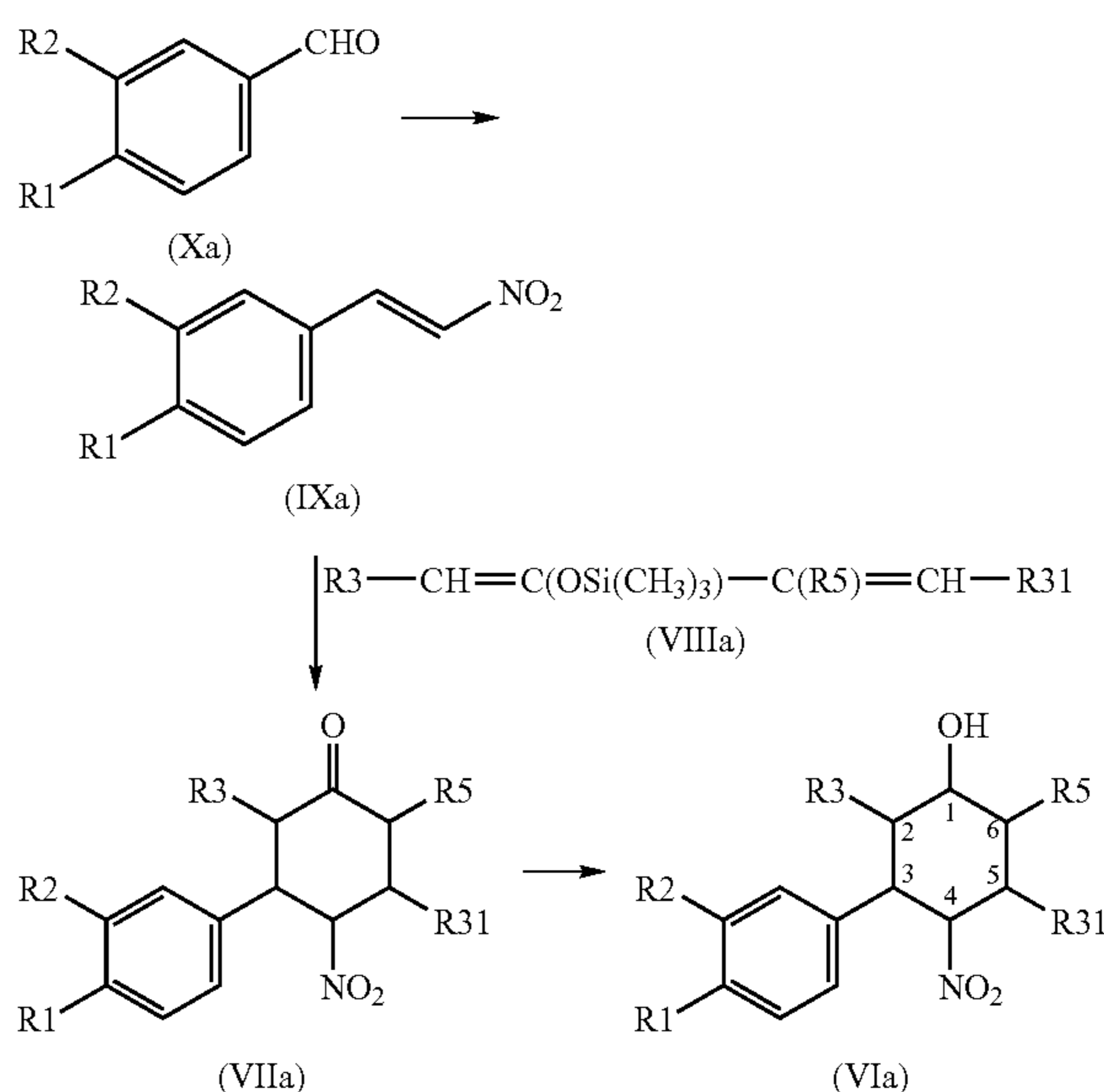
Reaction Scheme 2:
