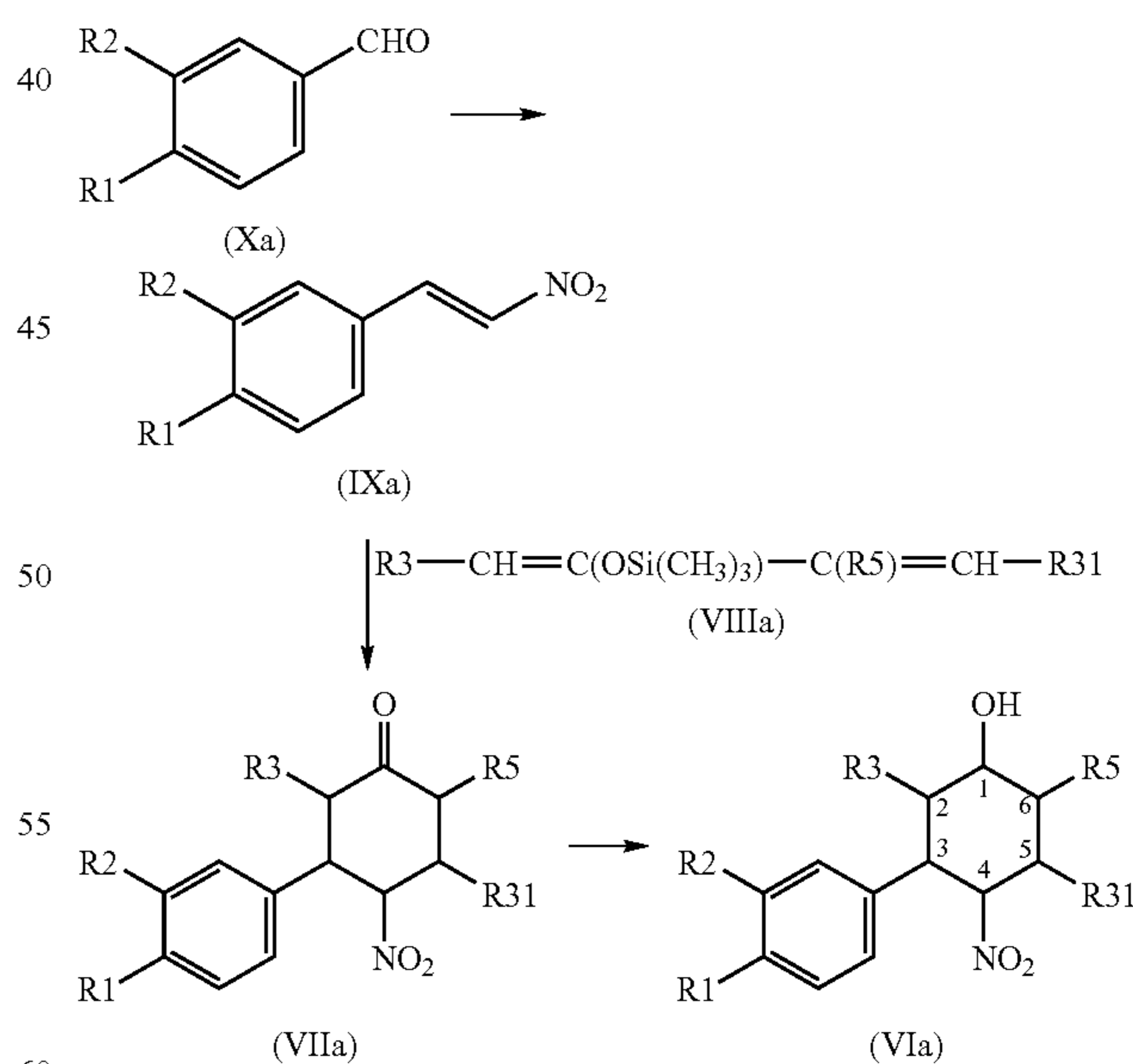
Reaction Scheme 2:
