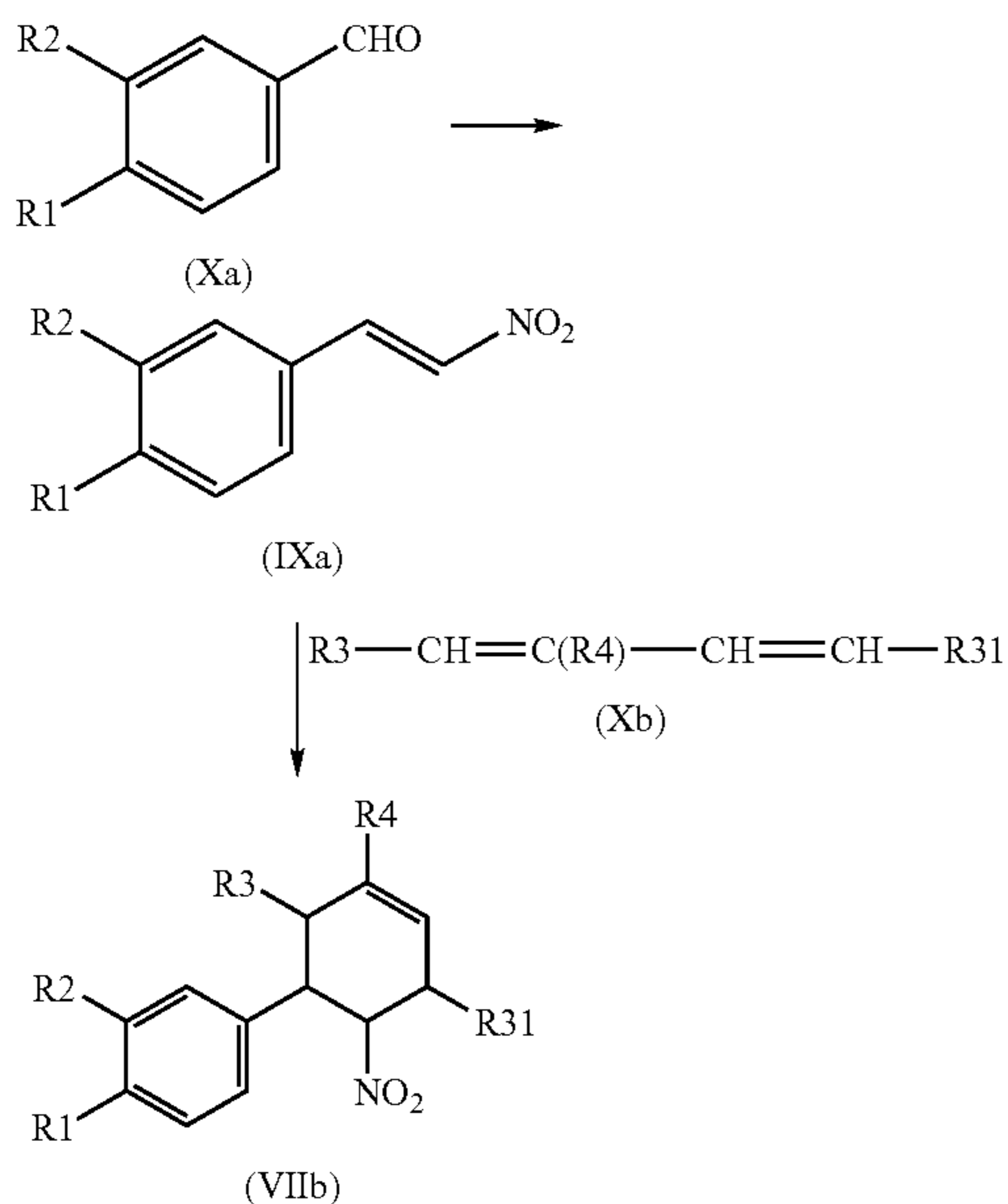
Reaction Scheme 5:
