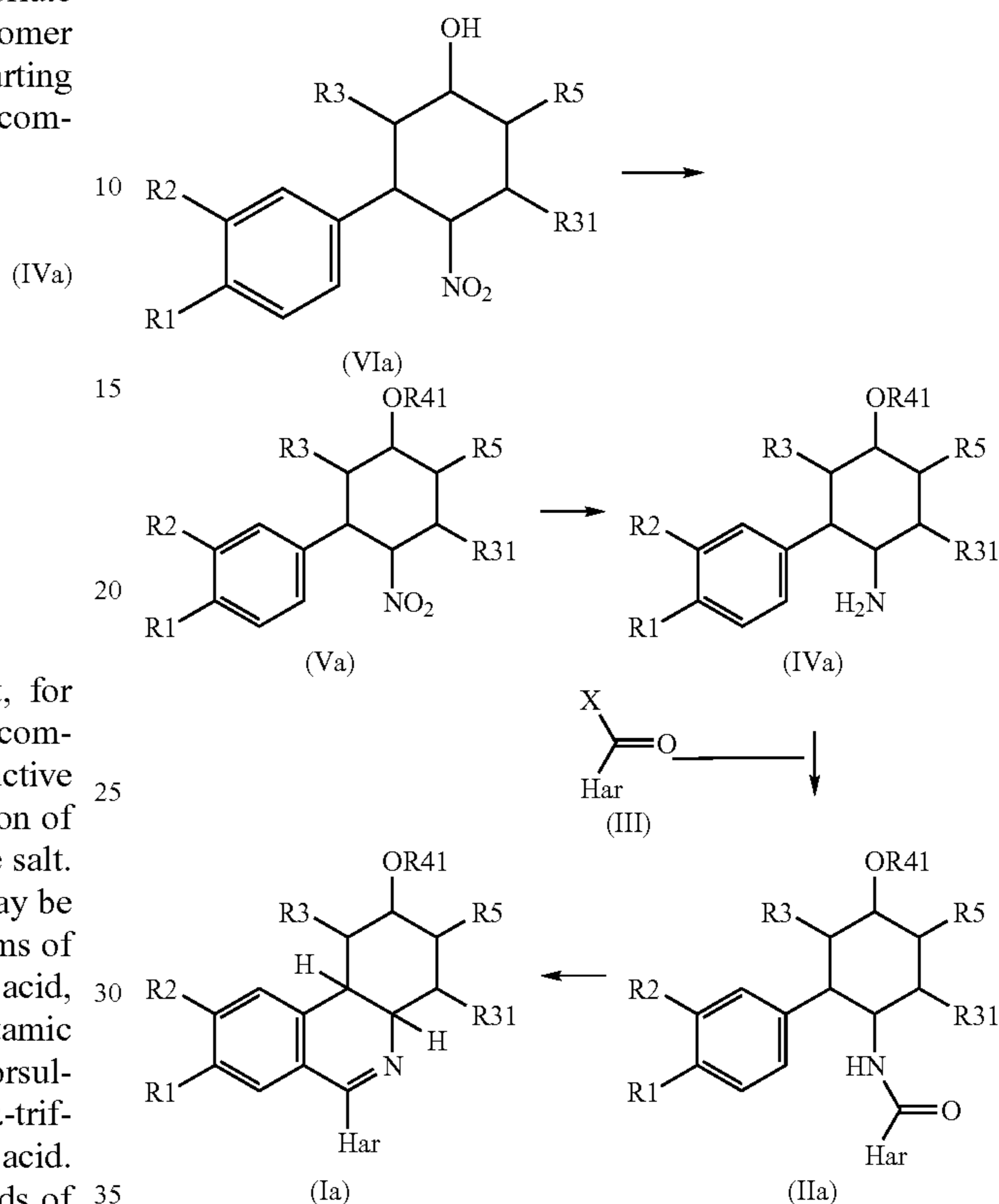
5 Reaction Scheme 1:
