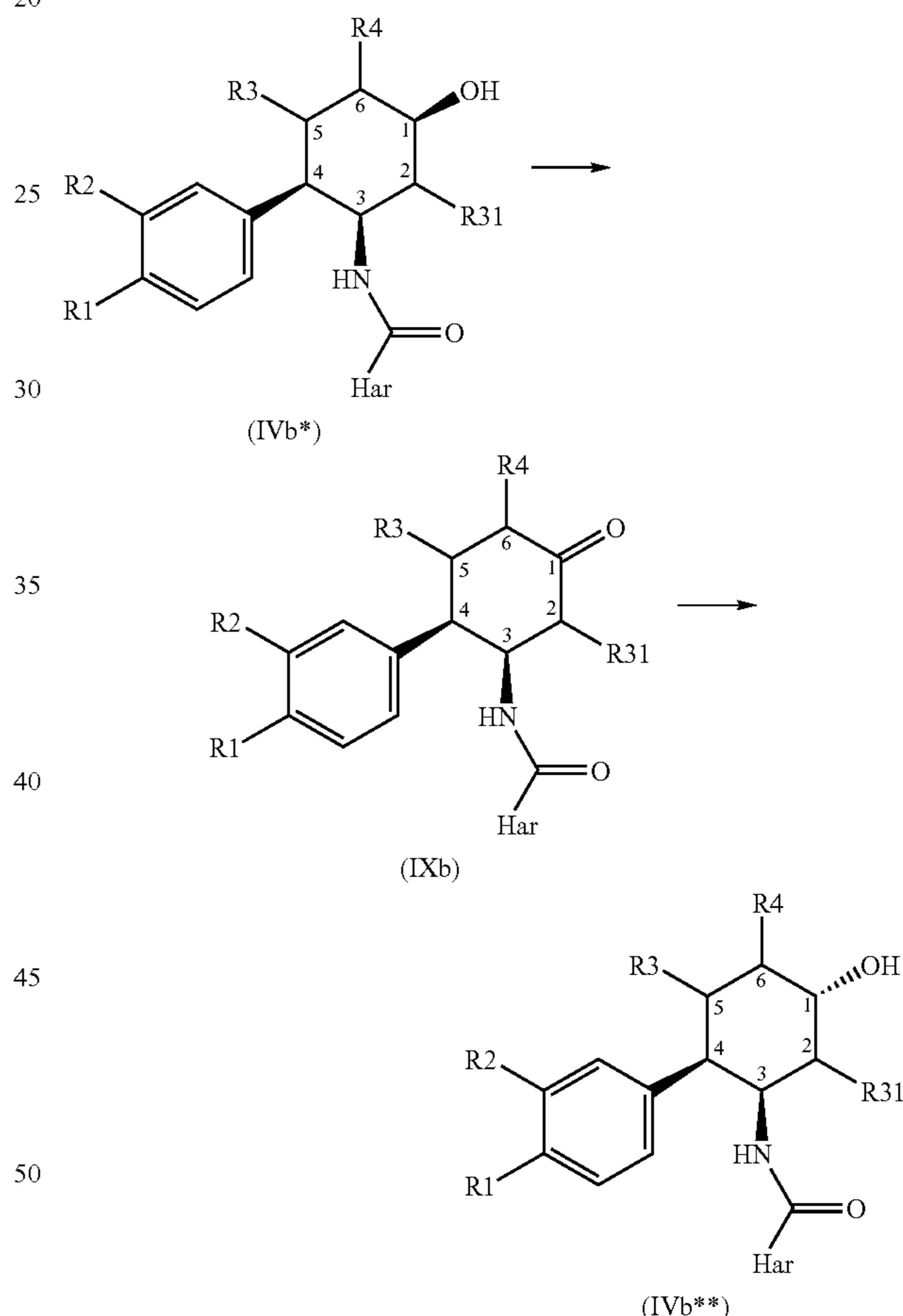
Reaction scheme 4:
