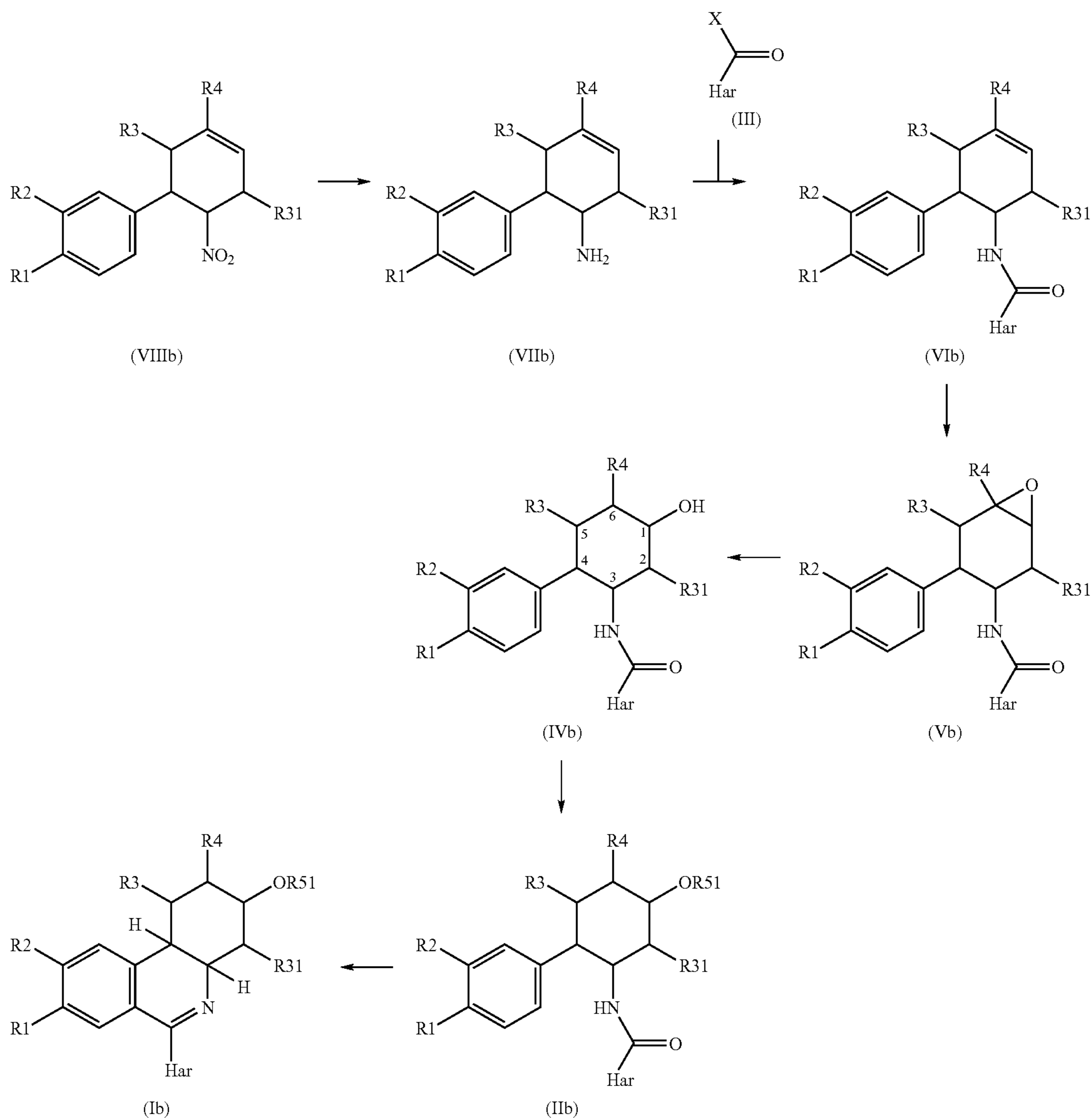
Reaction scheme 3:
