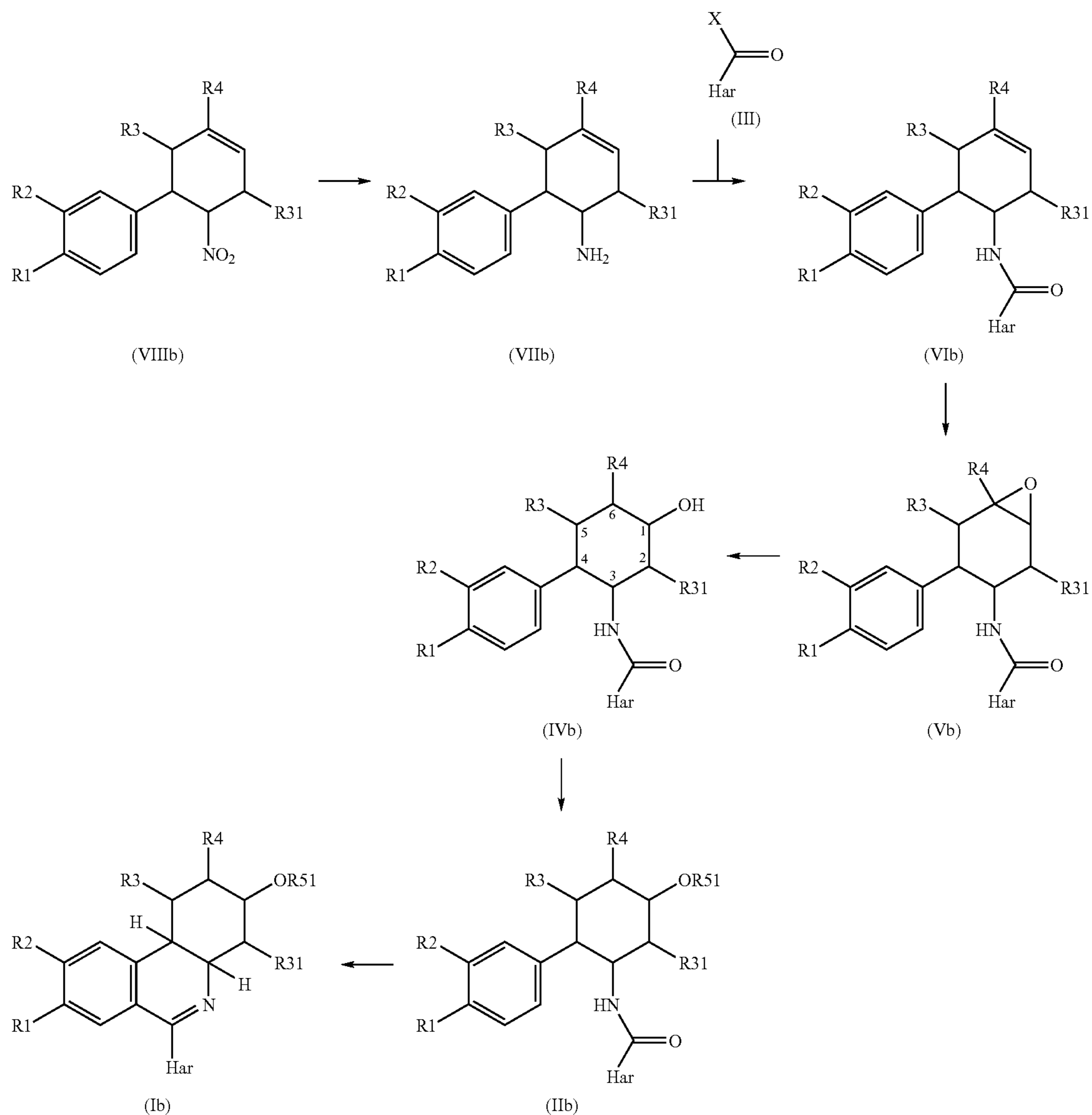
Reaction scheme 3:
