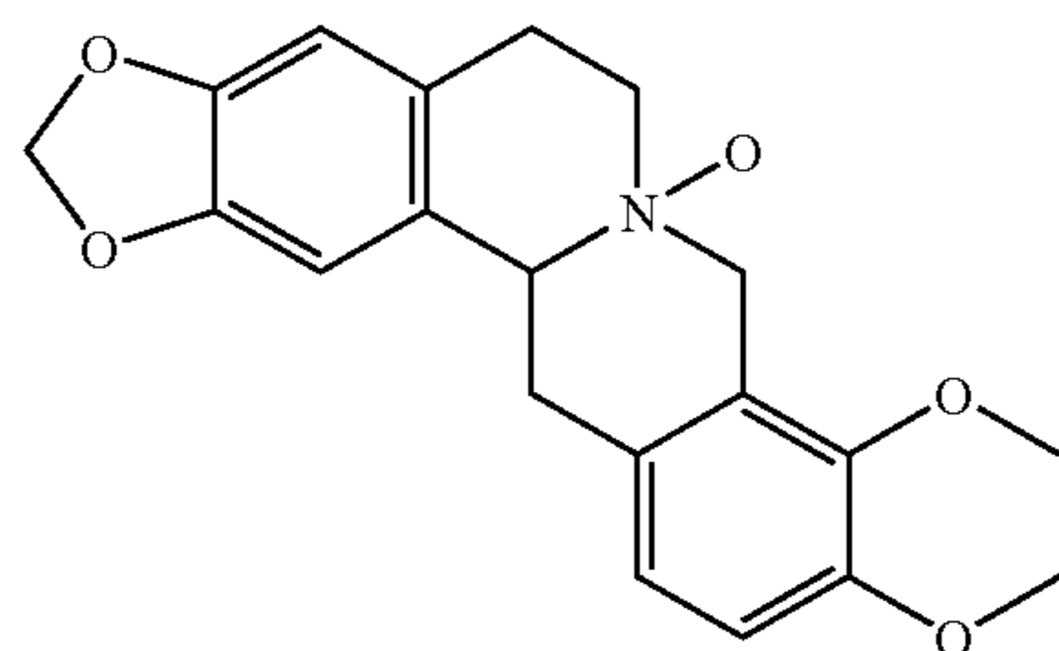
Compound 35
