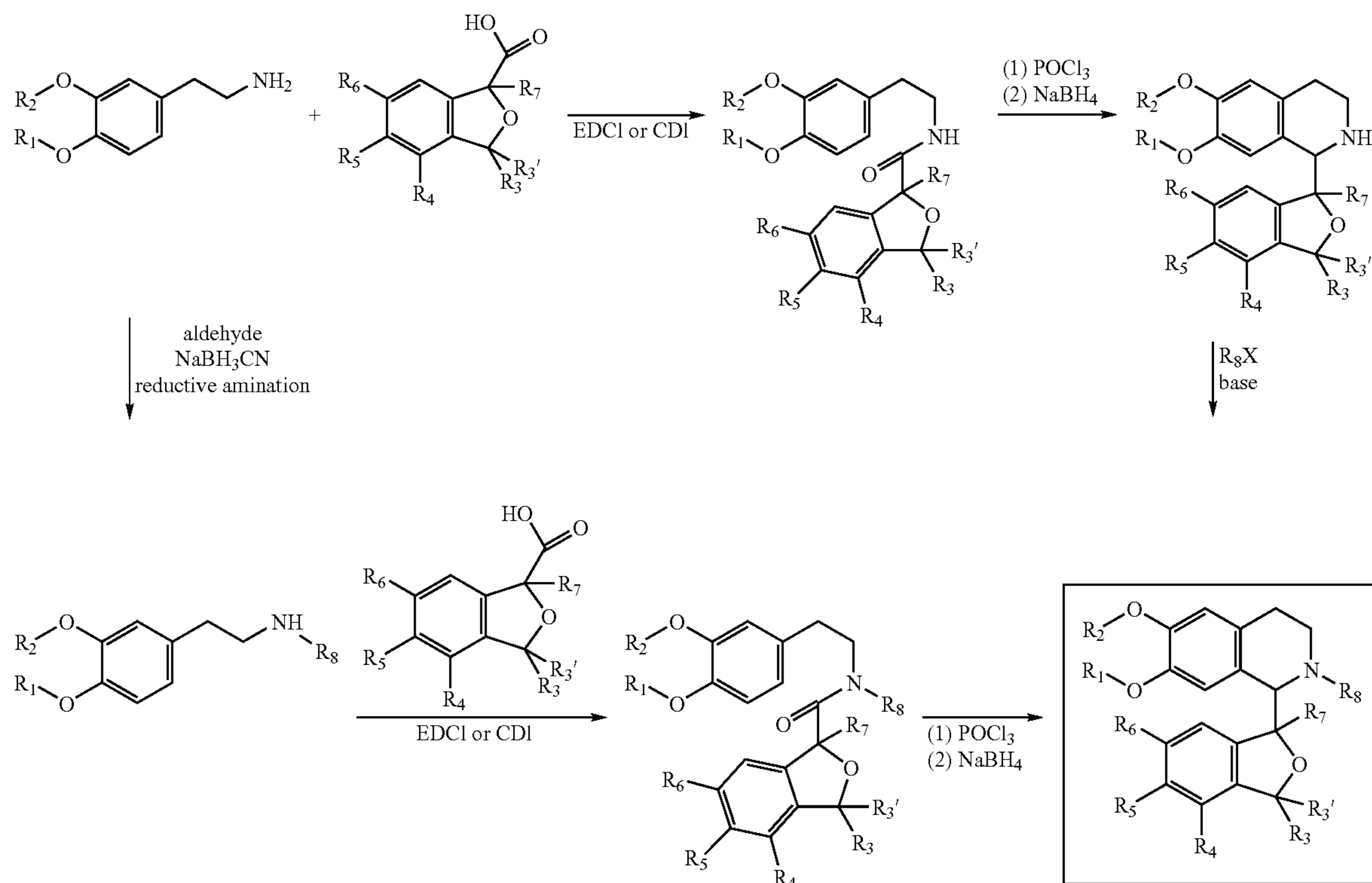
Scheme 10
