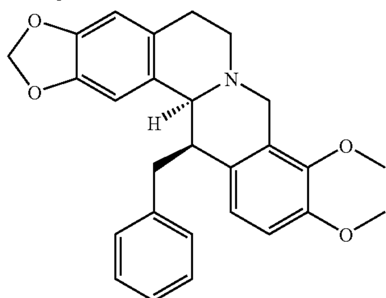
Compound 32
