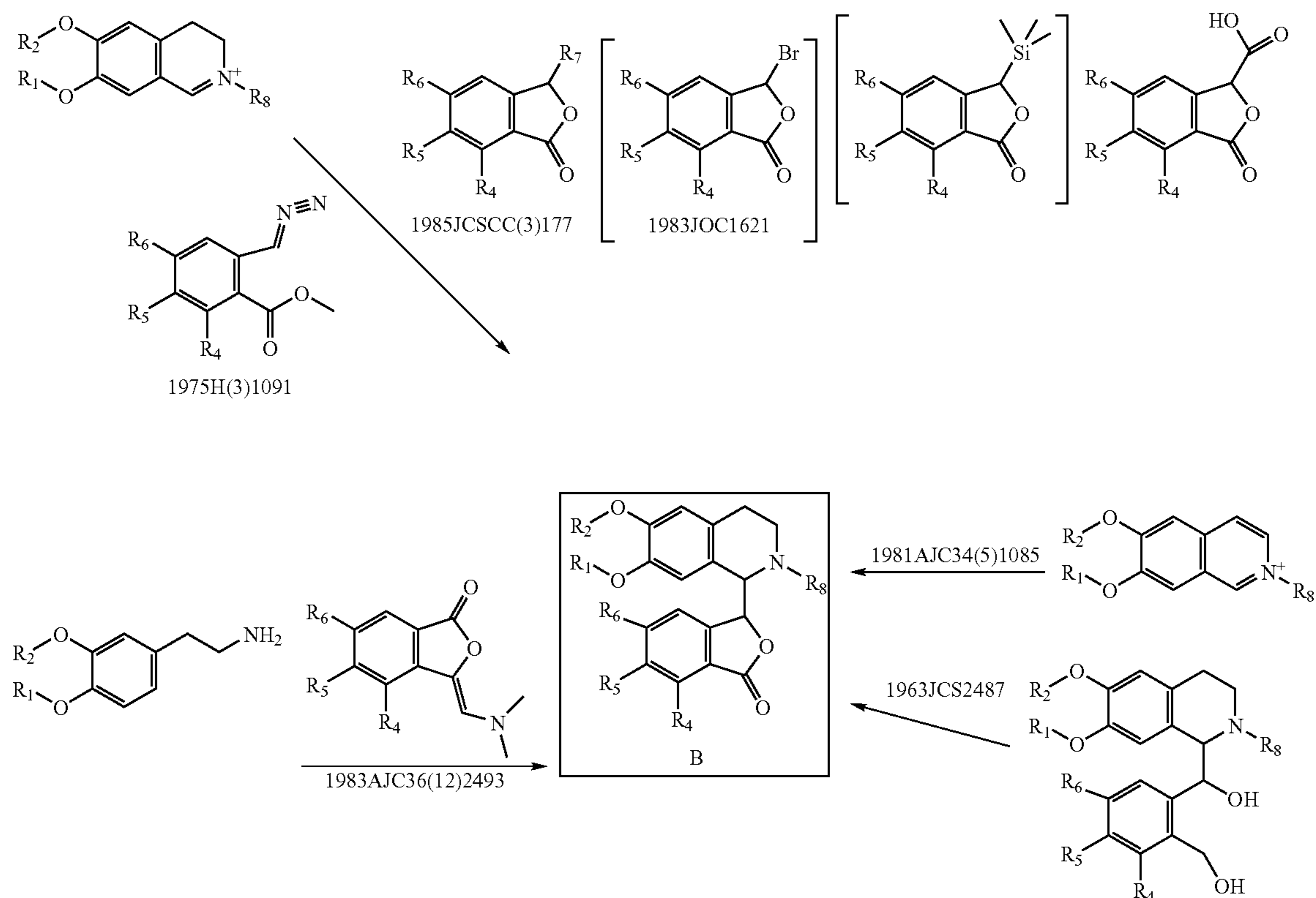
Scheme 12
