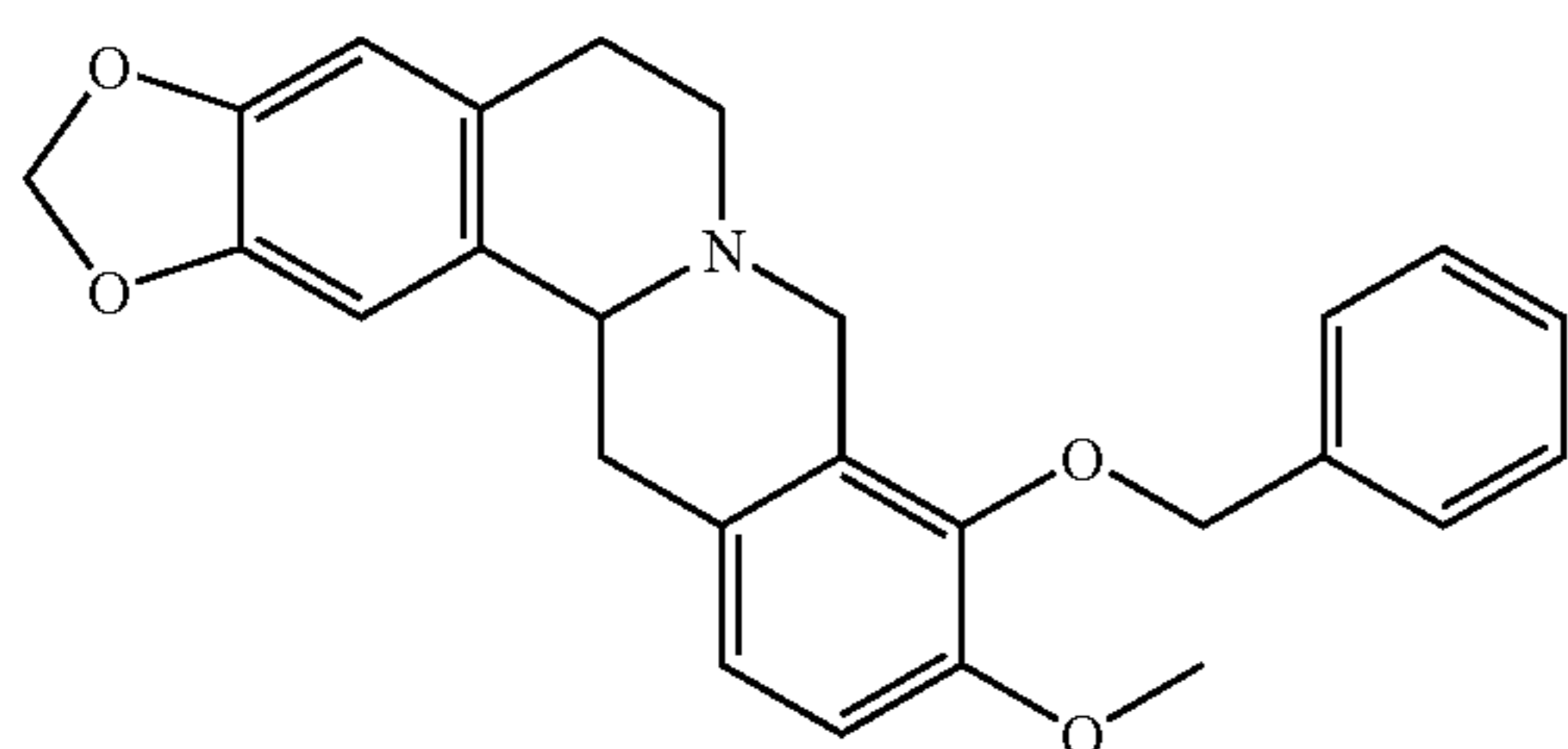
Compound 23
