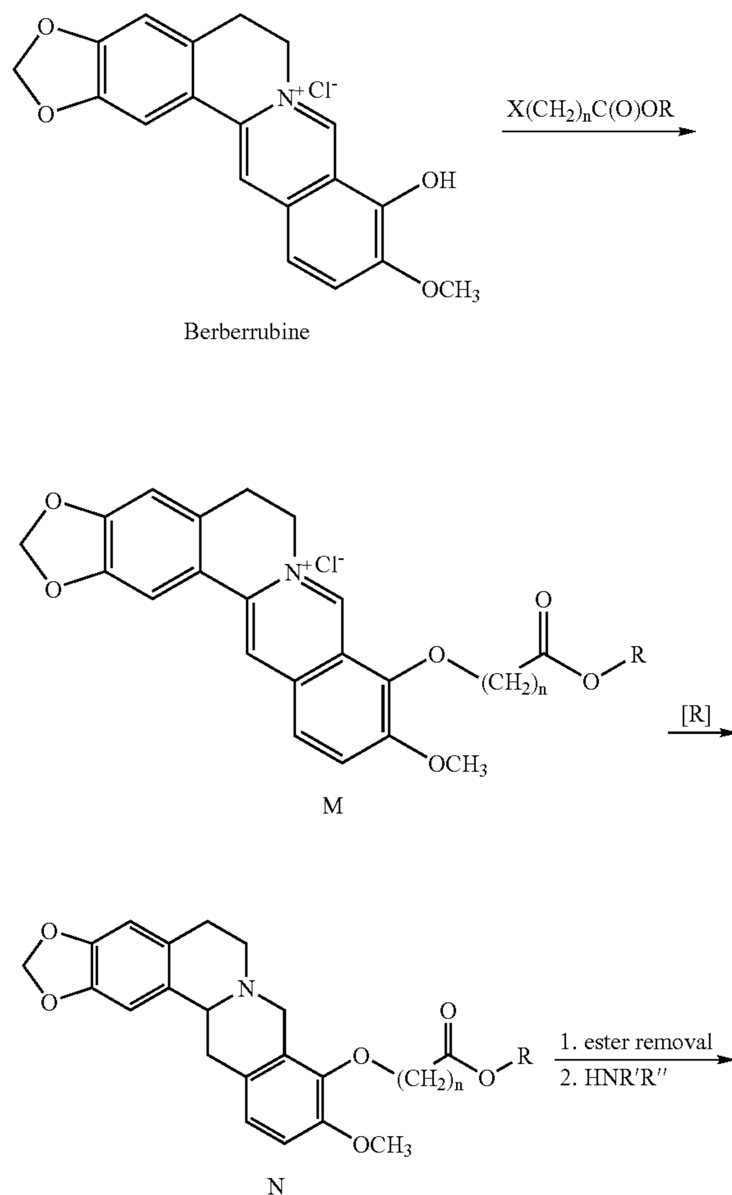
Scheme 5
