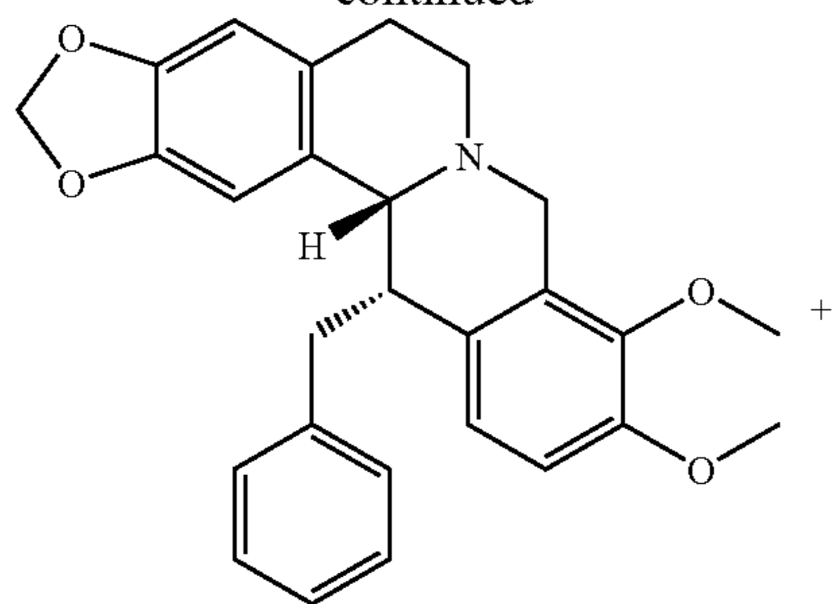
Compound 31
