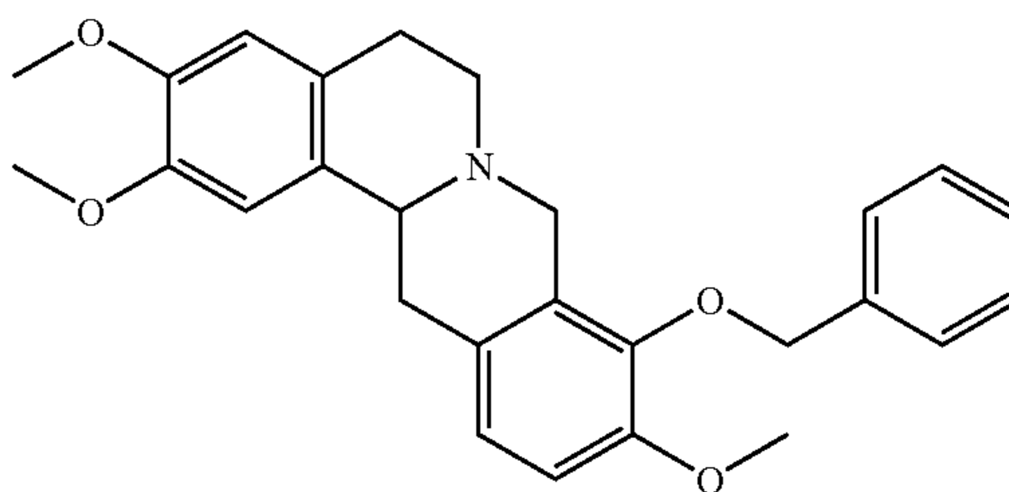
Compound 64
