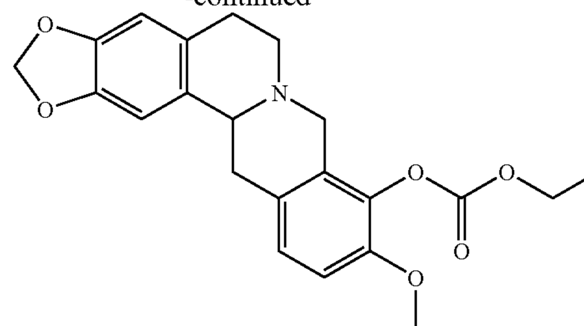
Compound 48
