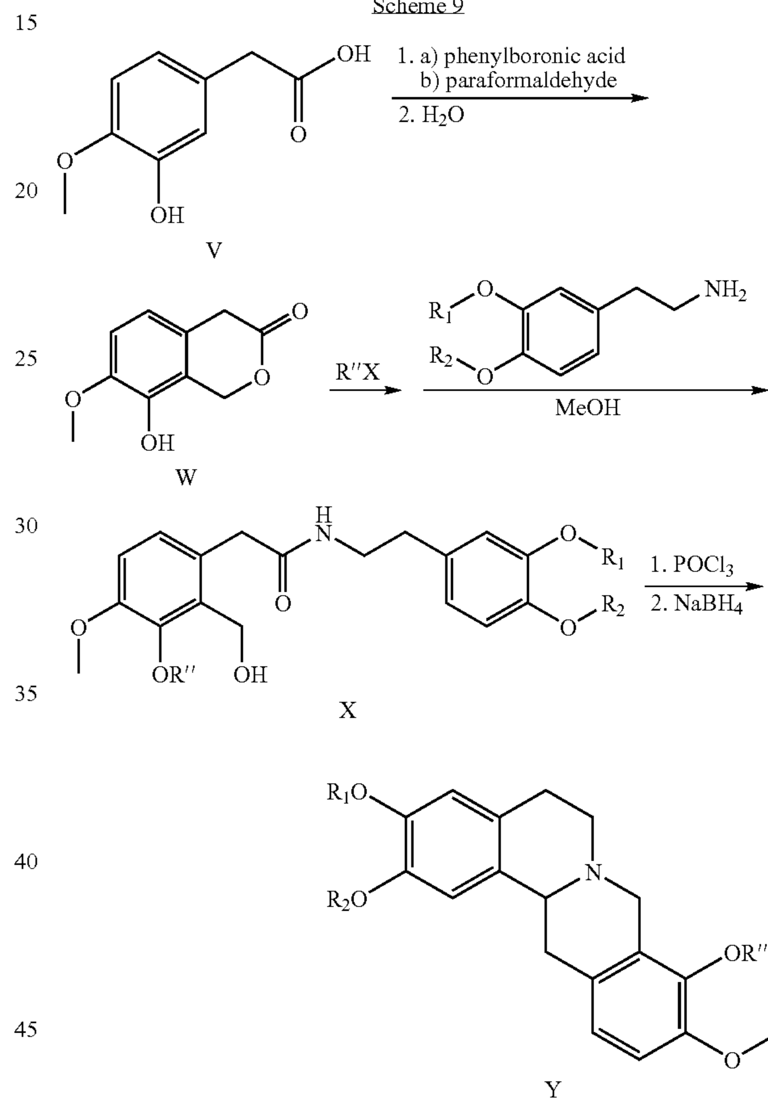
Scheme 9
