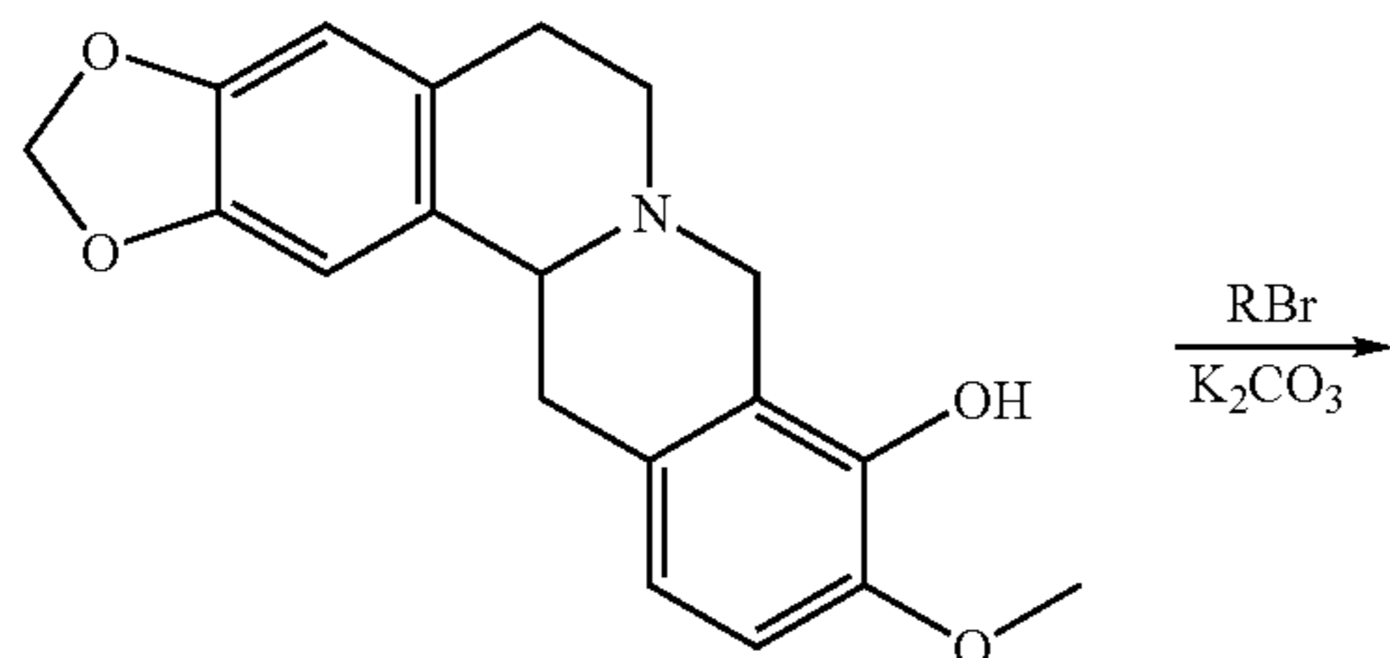
Compound 34
