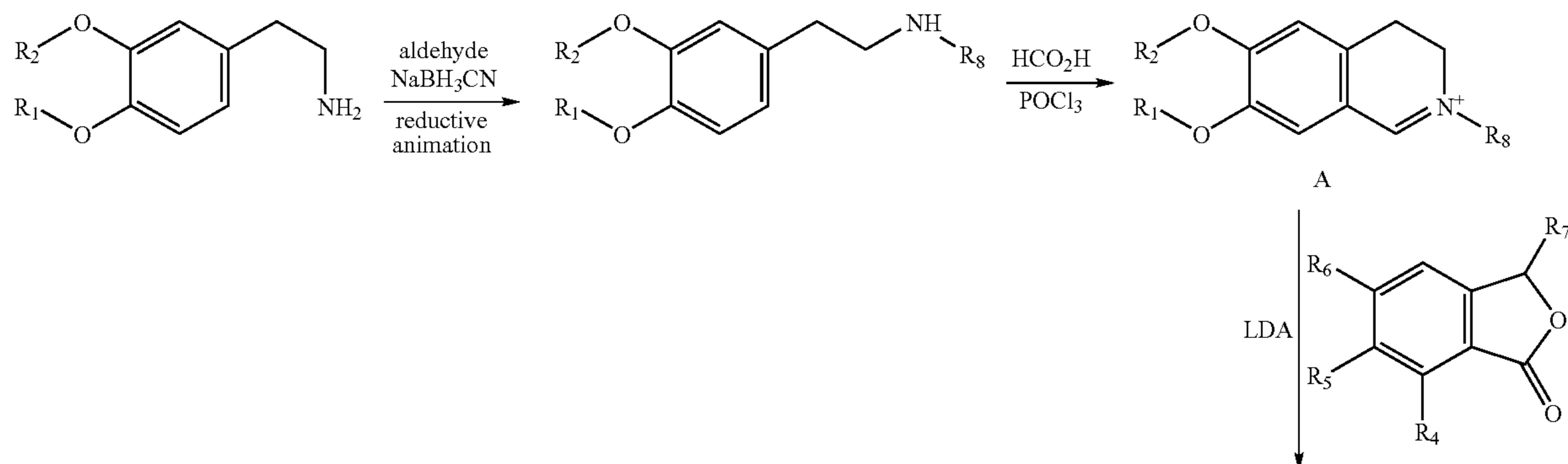
Scheme 11
