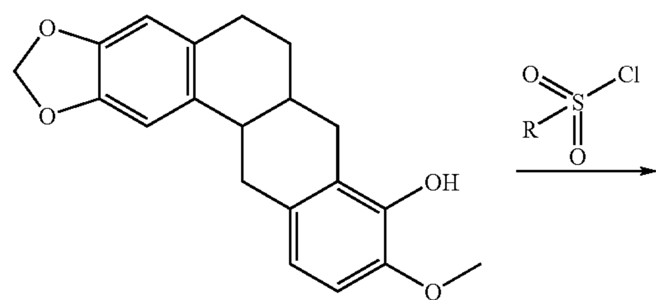
Compound 34
