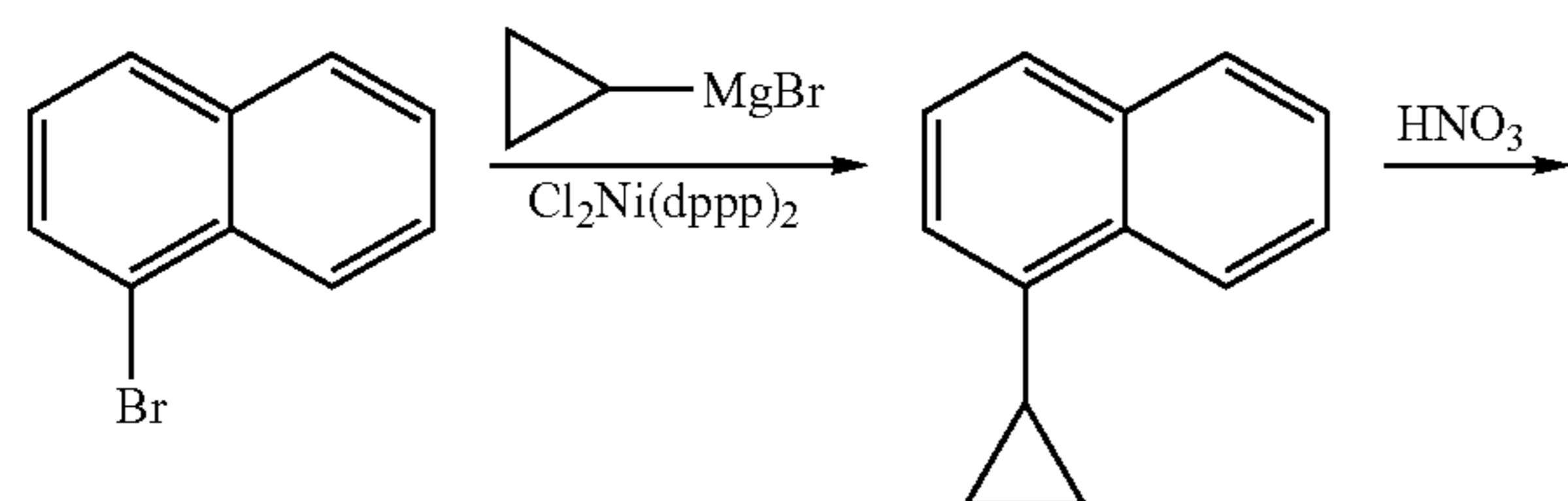
Scheme 3
