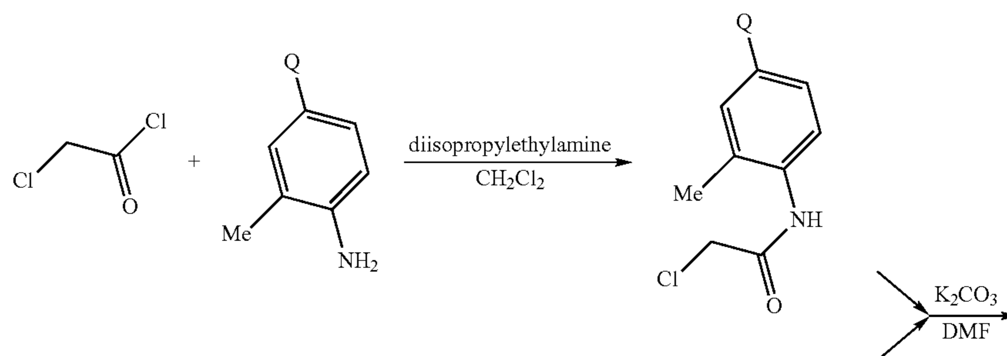
Scheme 6
