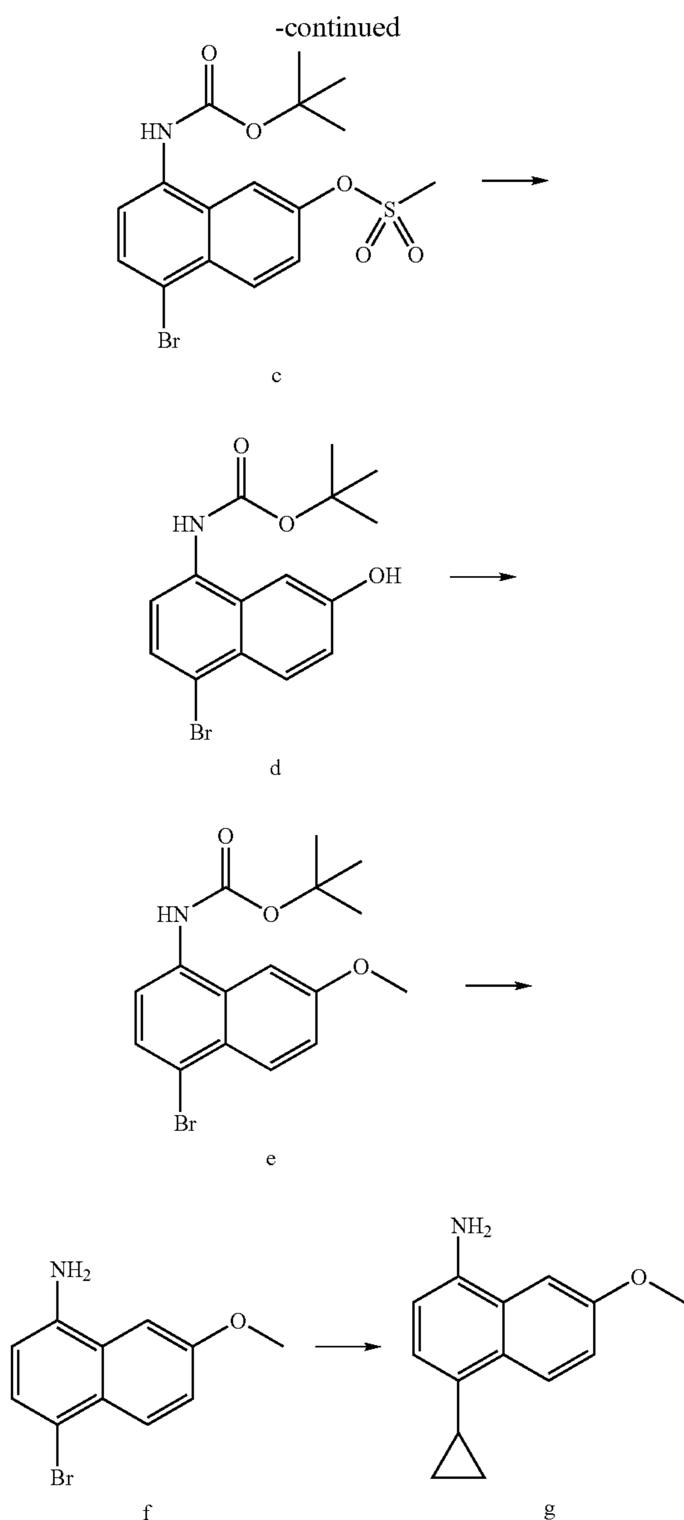
1-amino-4-cyclopropyl-7-methoxynaphthalene
