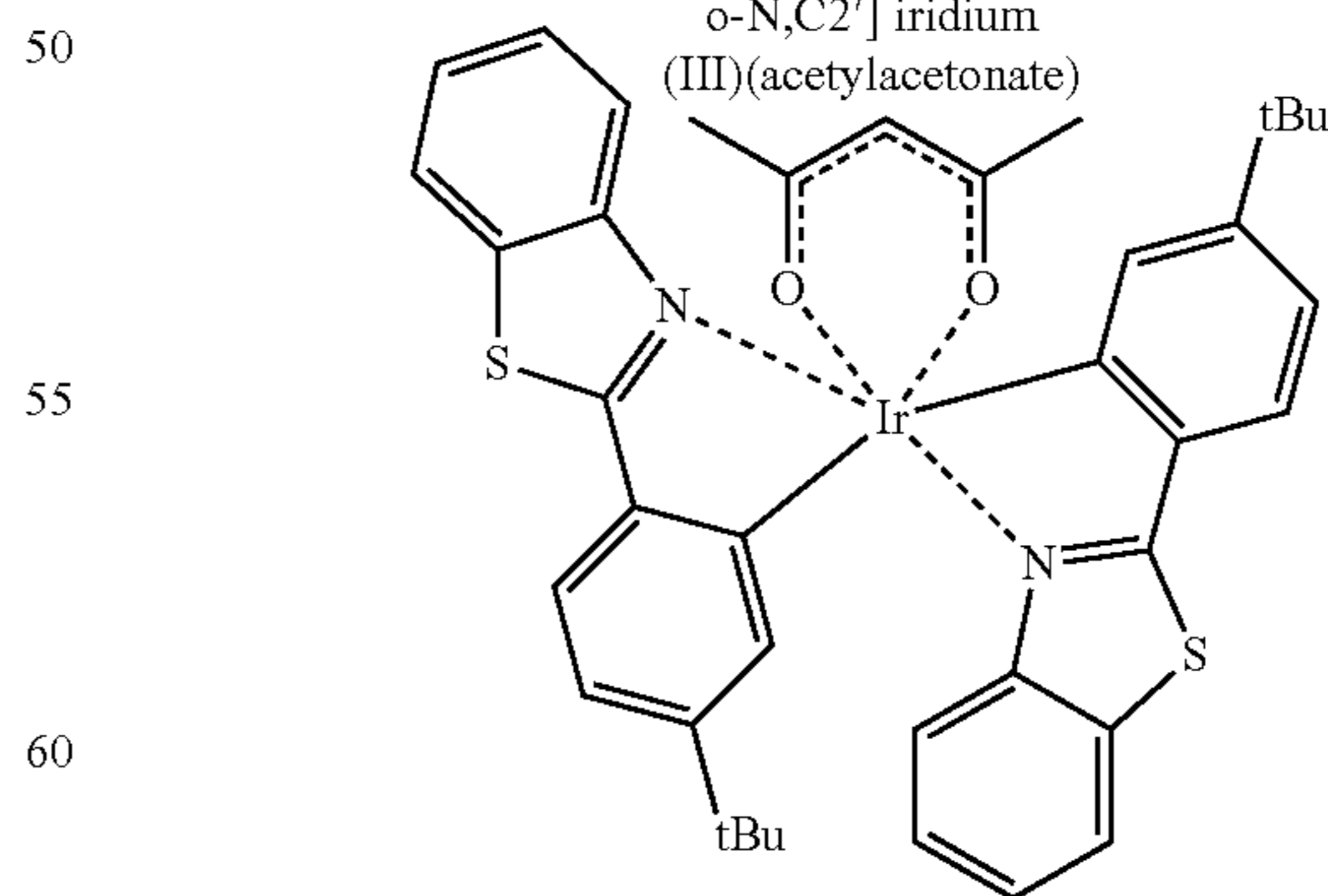
(t-bt) 2 Ir(III)(acac) Bis[2-(4-tert-butylphenyl)benzothiazolato-N,C2']iridium(III)(acetylacetonate)
