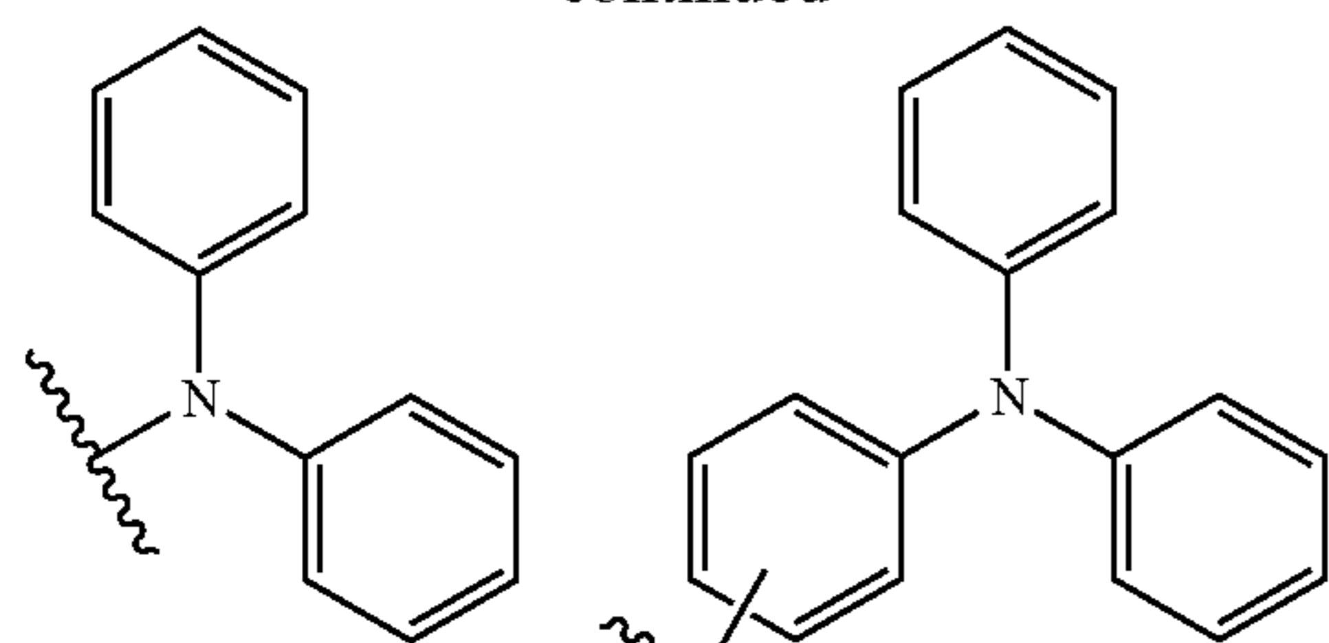
Diphenylamine
