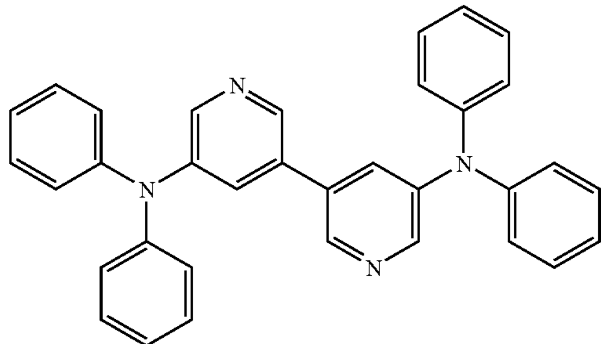
5,5'-bis(diphenylamino)-3,3'-bipyridine
