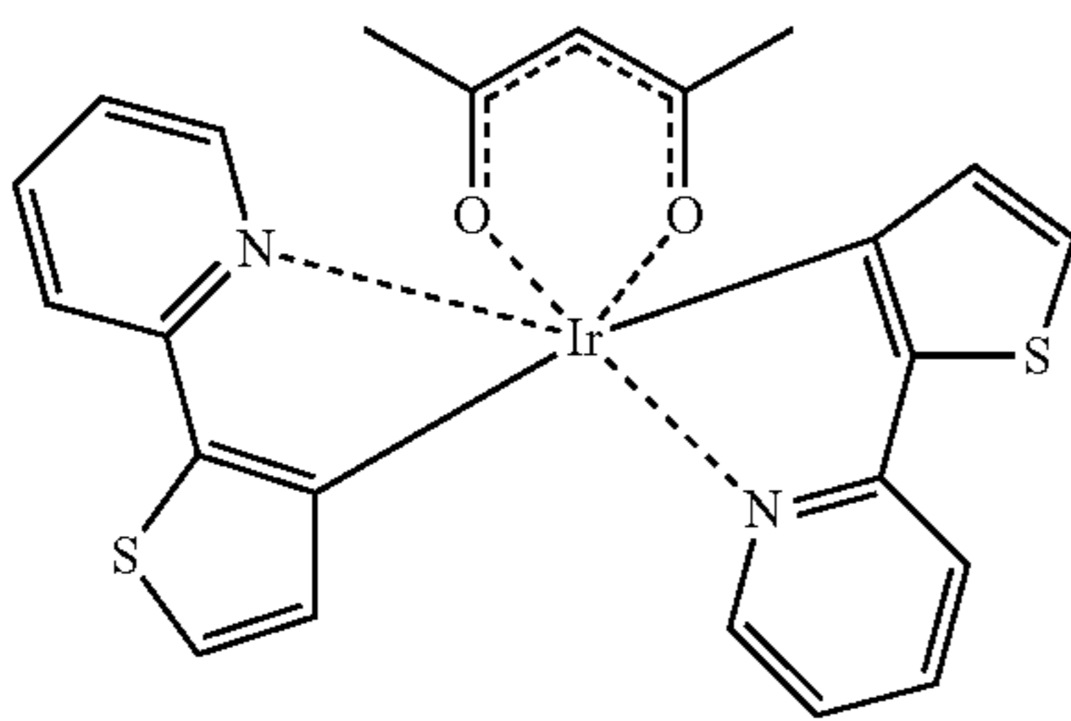
(thp) 2 Ir(III)(acac) Bis[2-(2'- thienyl)pyridinato- N,C3']iridium (III) (acetylacetonate)
