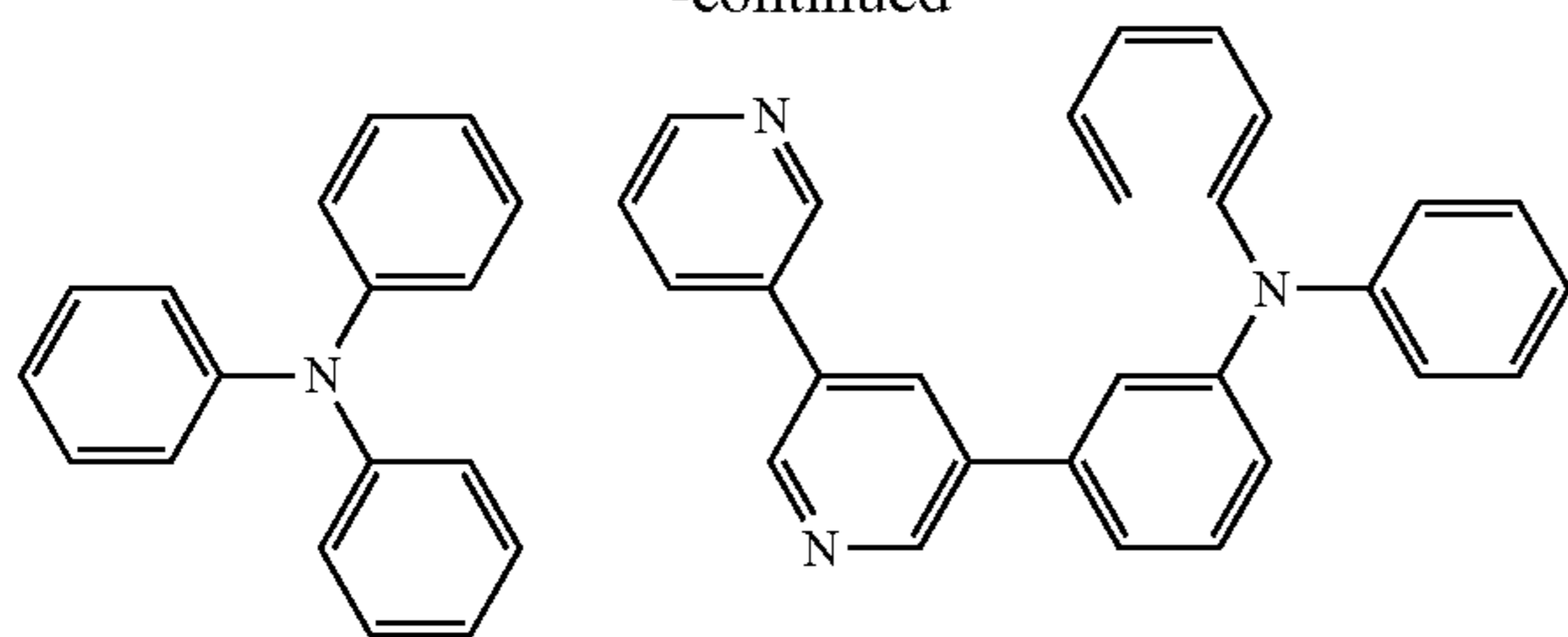
5,5'-bis(3-diphenylaminophenyl)-3,3'-bipyridine
