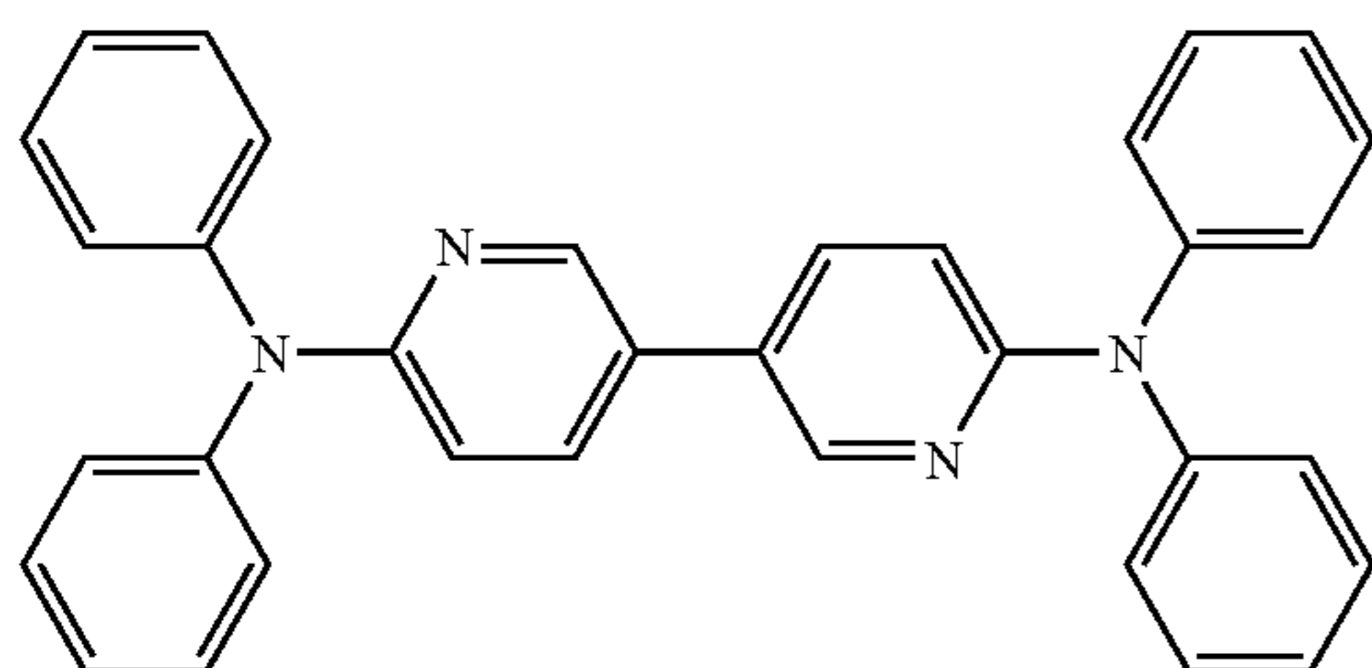
6-6'-bis(diphenylamino)-3,3'-bipyridine
