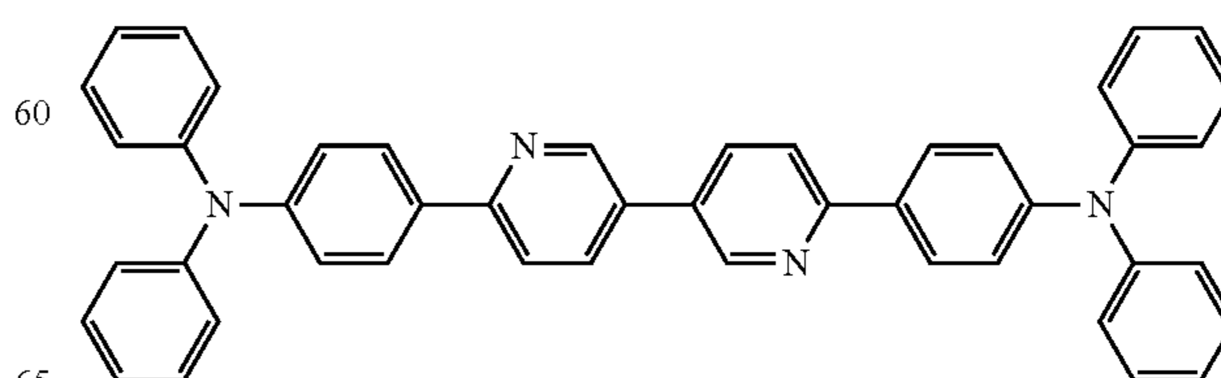
4,4'-(3,3'-bipyridine-6,6'-diyl)bis(N,N-diphenylaniline)
