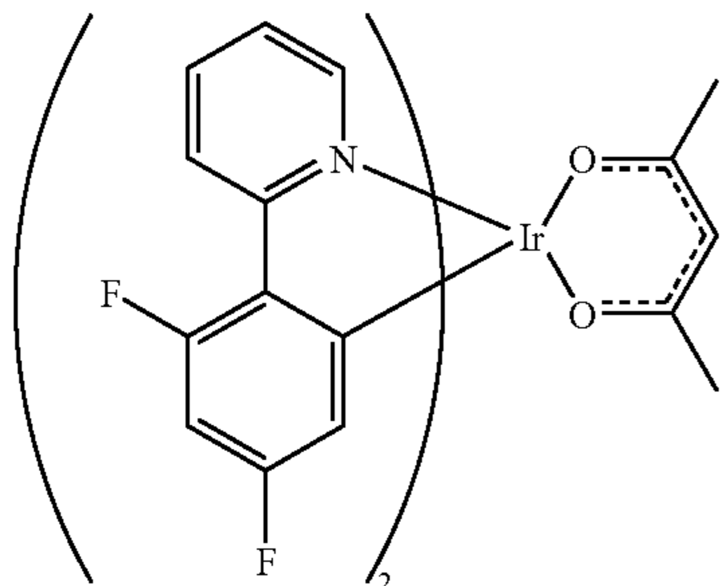
bis(2-[4,6-difluorophenyl]pyridinato-N,C2')iridium(acetylacetonate) [FIr(acac)]
