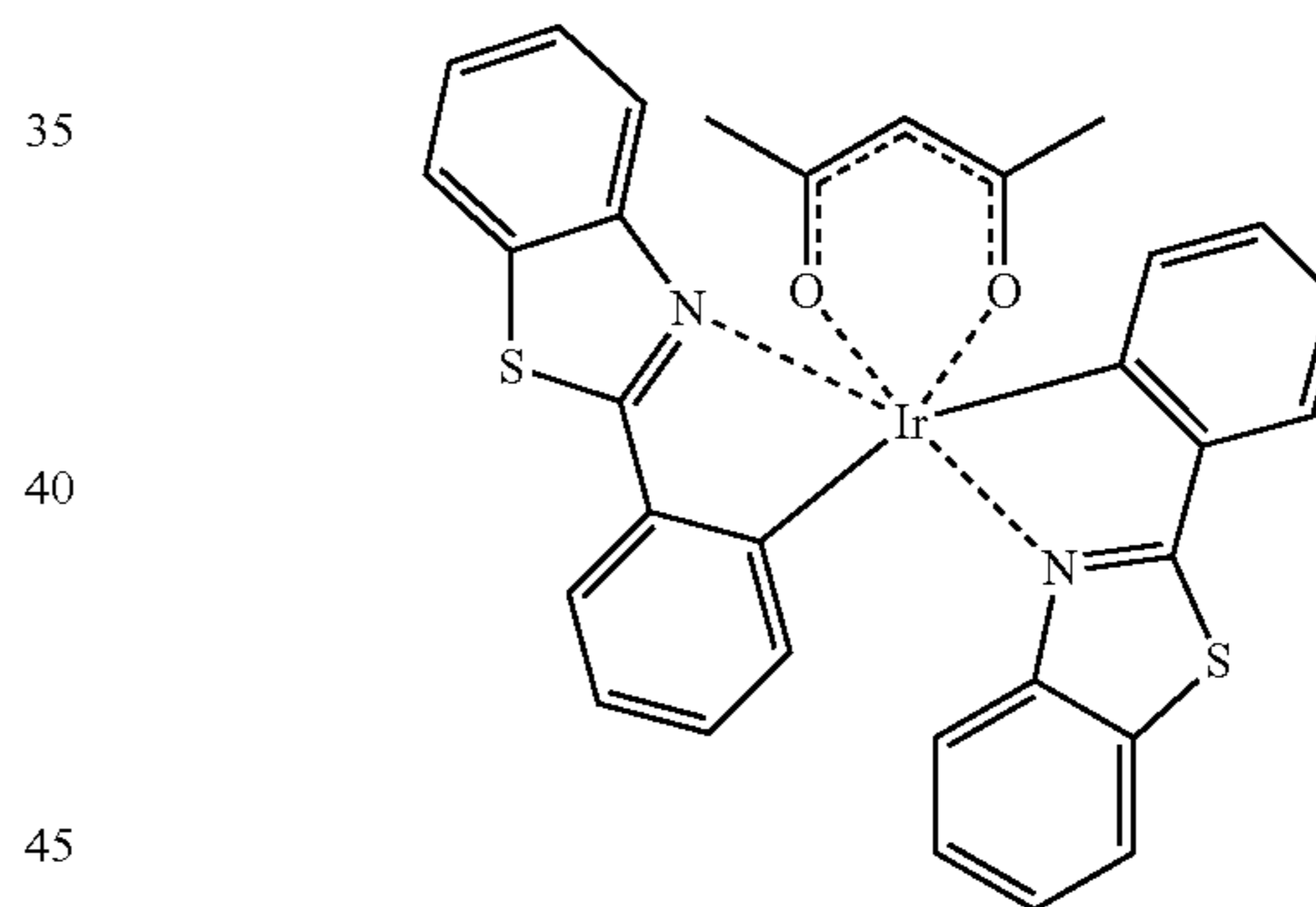
(bt) 2 Ir(III)(acac) Bis[2-phenylbenzothiazolato-N,C2'] iridium (III)(acetylacetonate)
