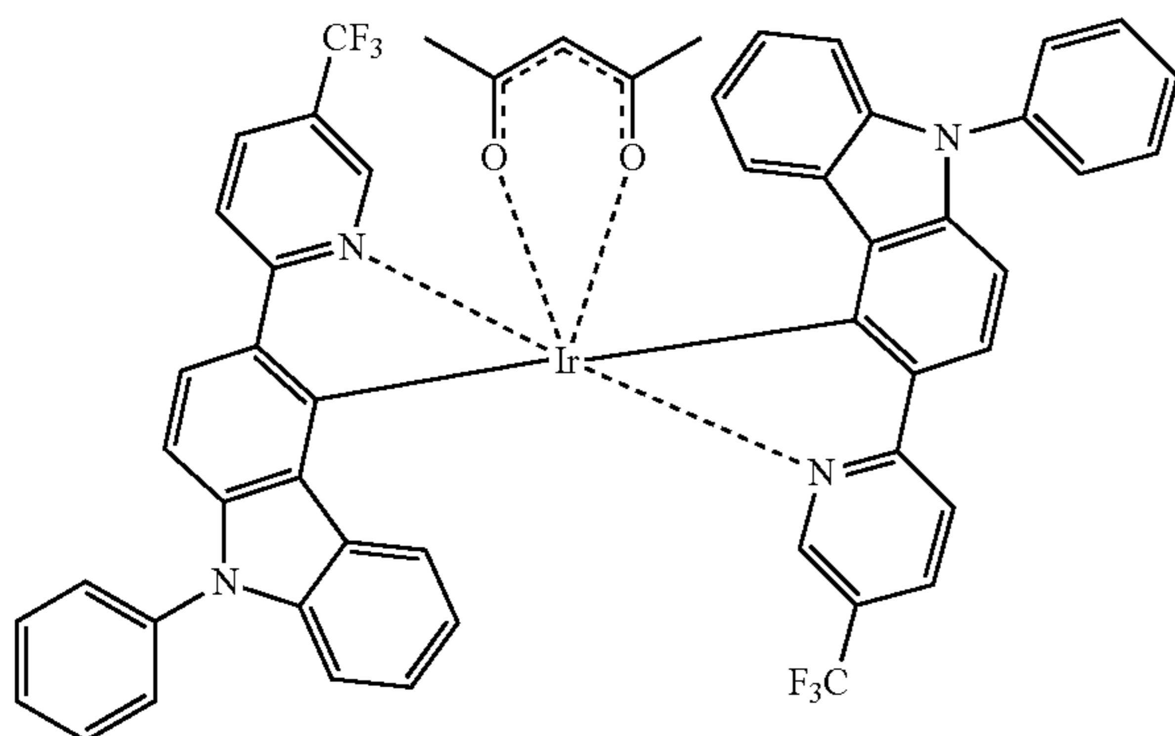
(Cz-CF 3 )Ir(III)(acac) Bis[5-trifluoromethyl-2-[3-(N- phenylcarbazolyl)pyridinato- N,C2']iridium(III)(acetylacetonate)
