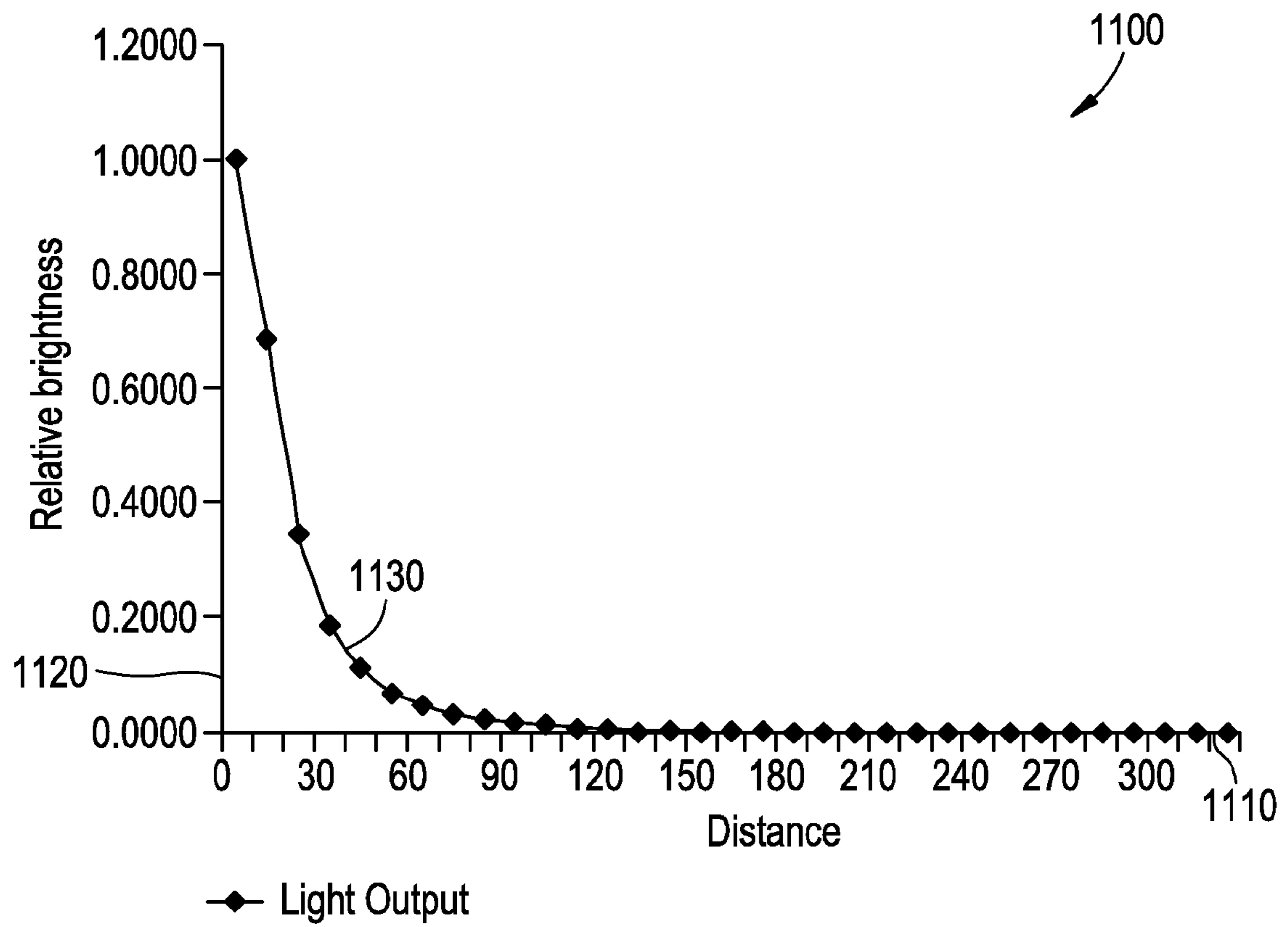
FIG. 11 Light Output at 15mm
