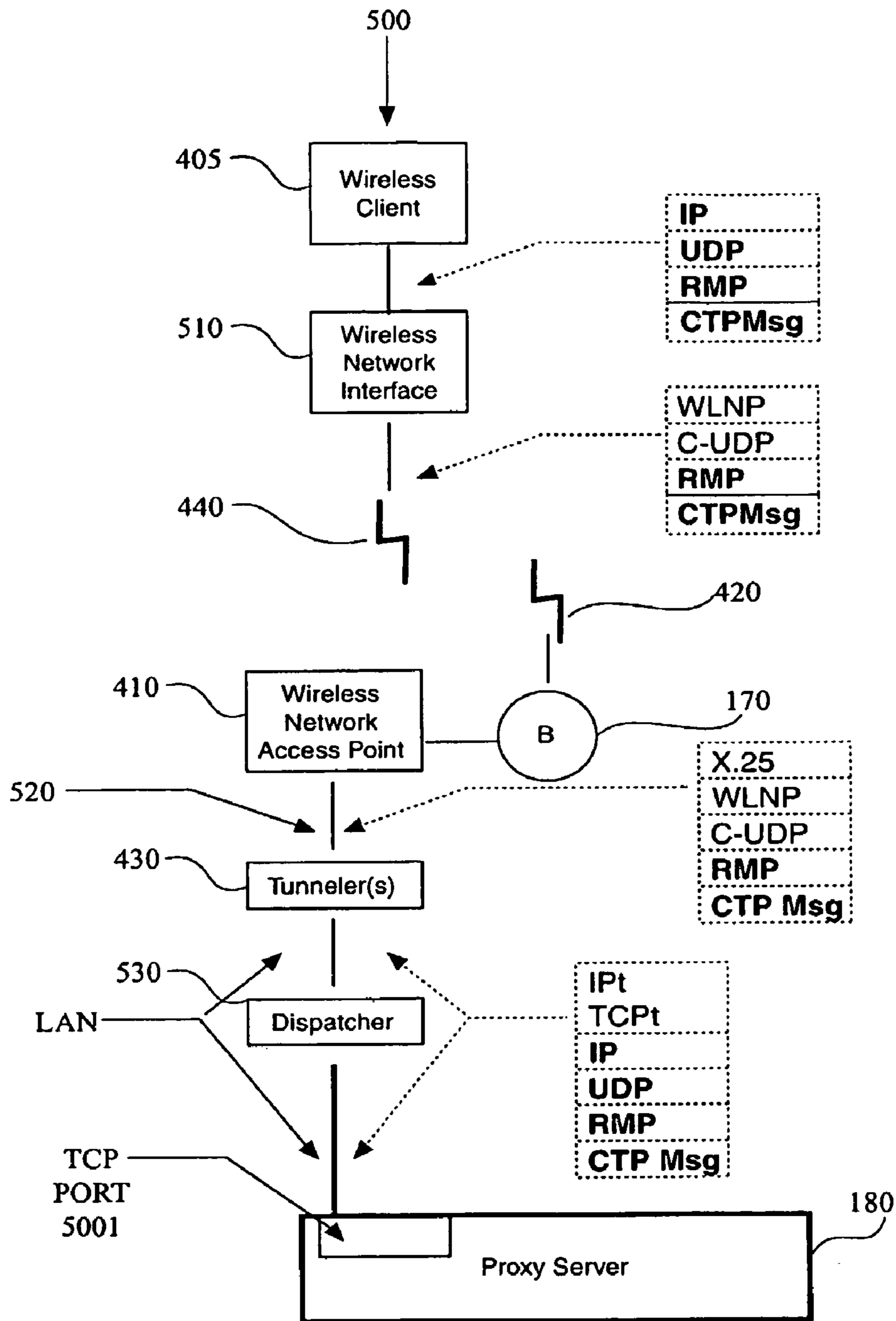
FIG. 5 – WIRELESS NETWORK TOPOLOGY INCLUDING A WIRELESS NETWORK INTERFACE, A LEASED LINE, AND A DISPATCHER
