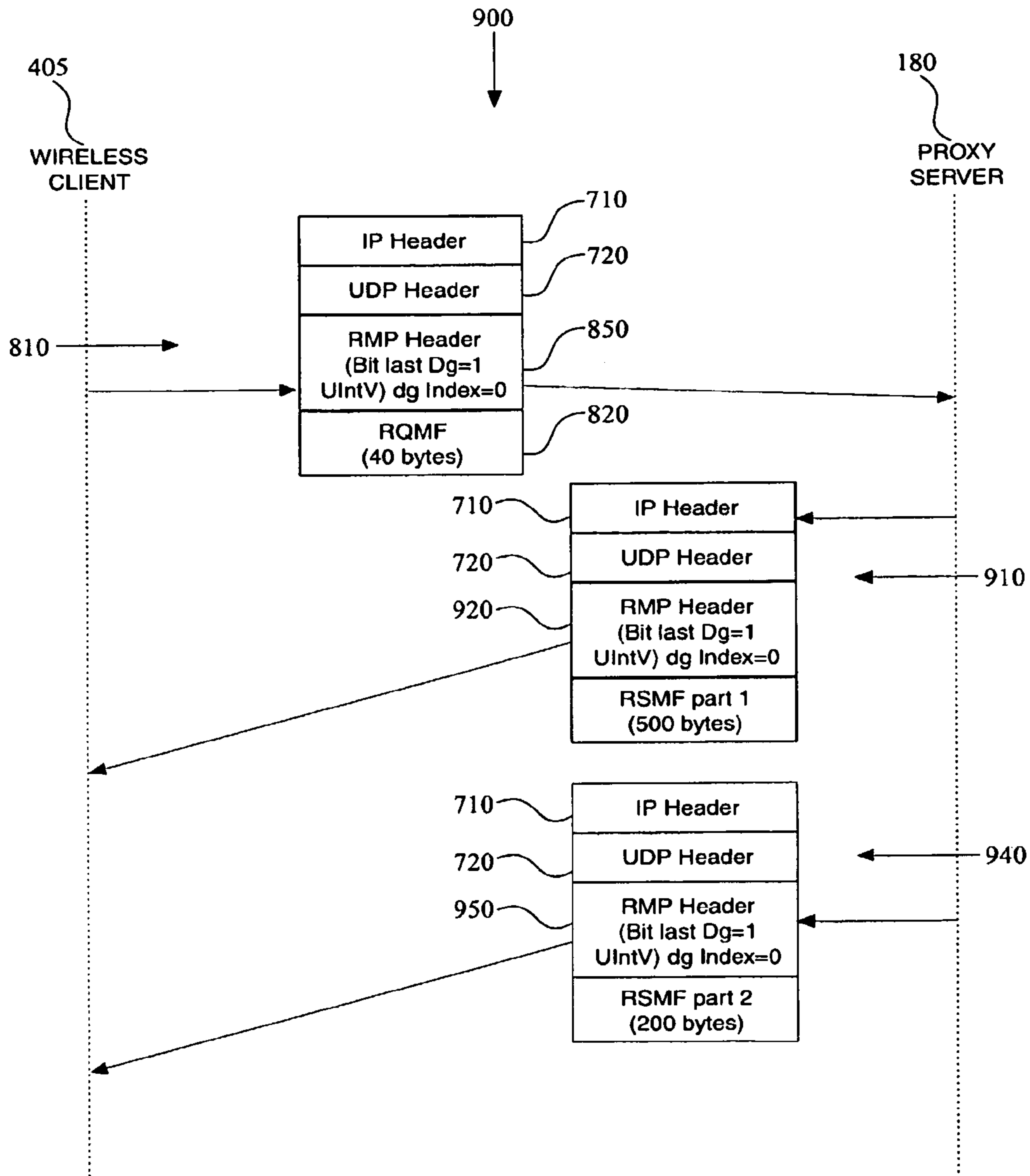
FIG. 9 – EXCHANGE OF MESSAGES COMPRISING A SINGLE REQUEST PACKET AND TWO RESPONSE PACKETS
