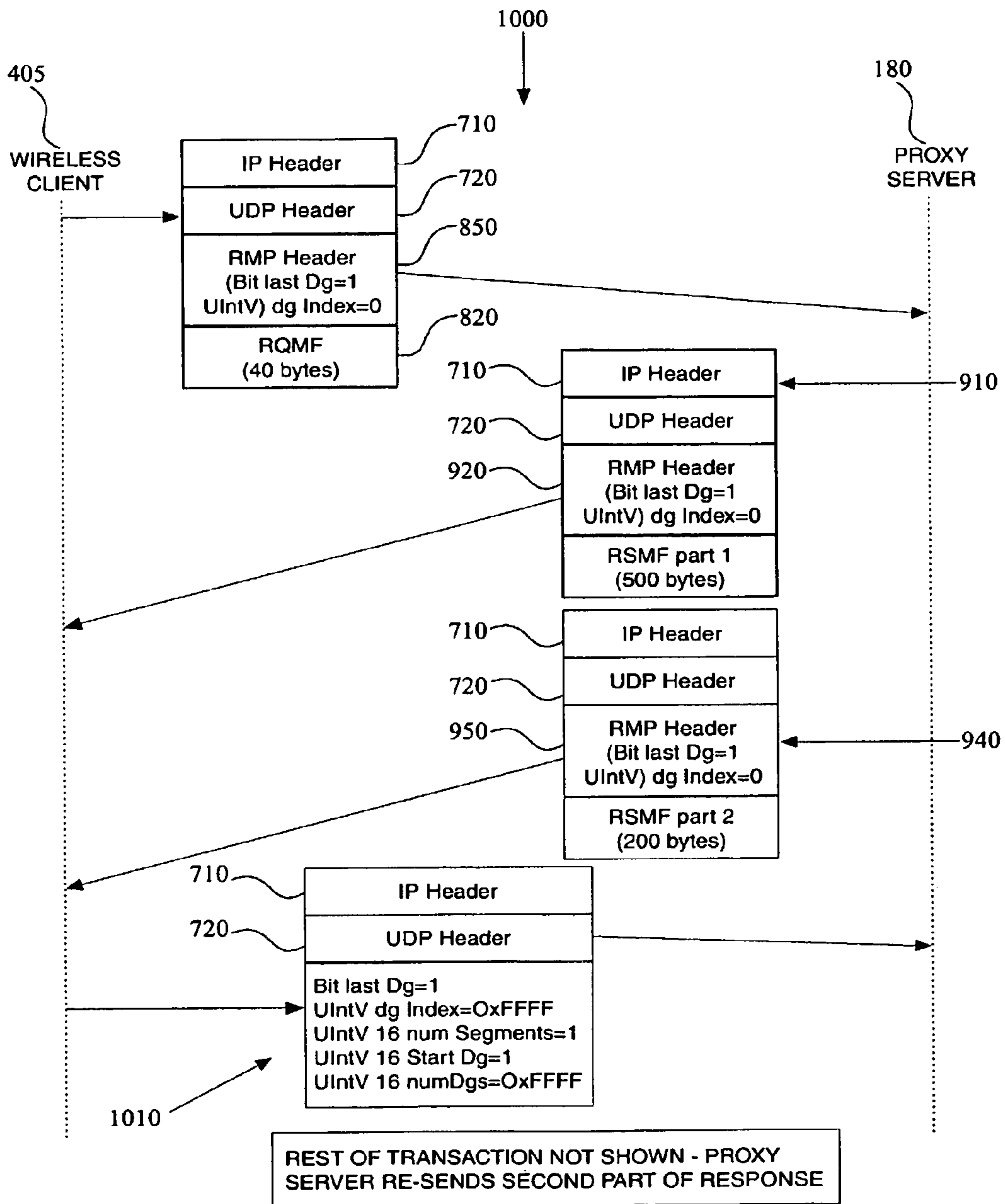
FIG. 10 – EXCHANGE OF MESSAGES INCLUDING A RE-TRANSMIT SEQUENCE
