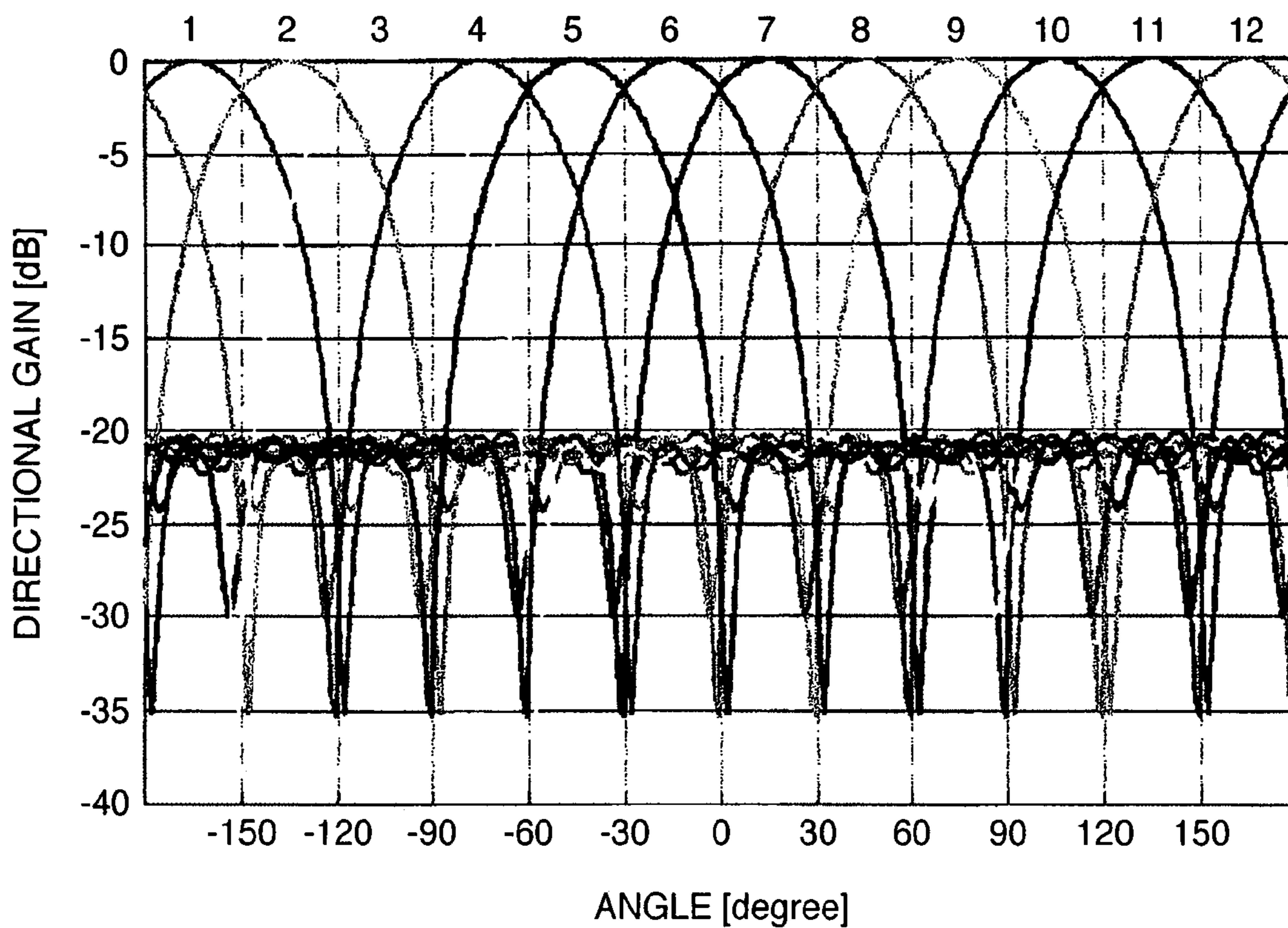
1~12 : BEAM PATTERN
