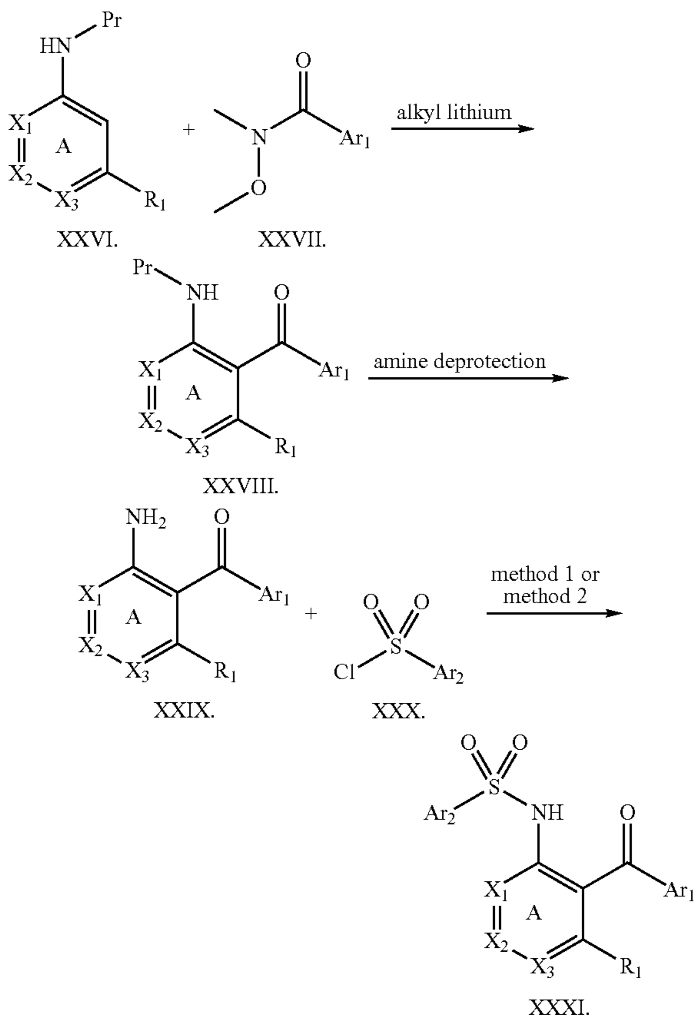
Scheme I: General synthesis of diaryl methanones.
