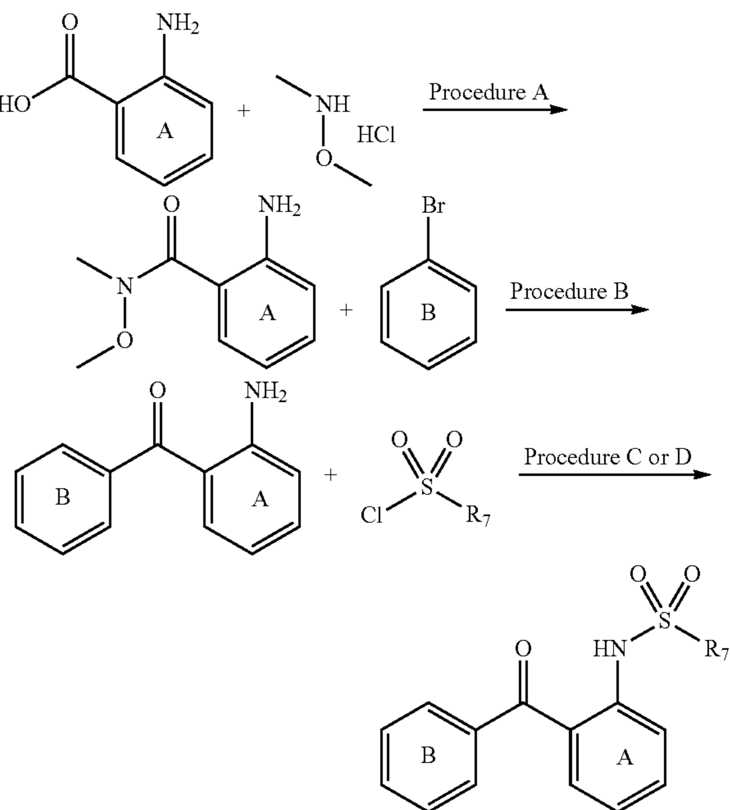
Scheme II: Synthesis of N-(2-Benzoyl-Phenyl)-Benzenesulfonamides and N-(2-Benzoyl-Phenyl)-Heteroarylsulfonamides.
