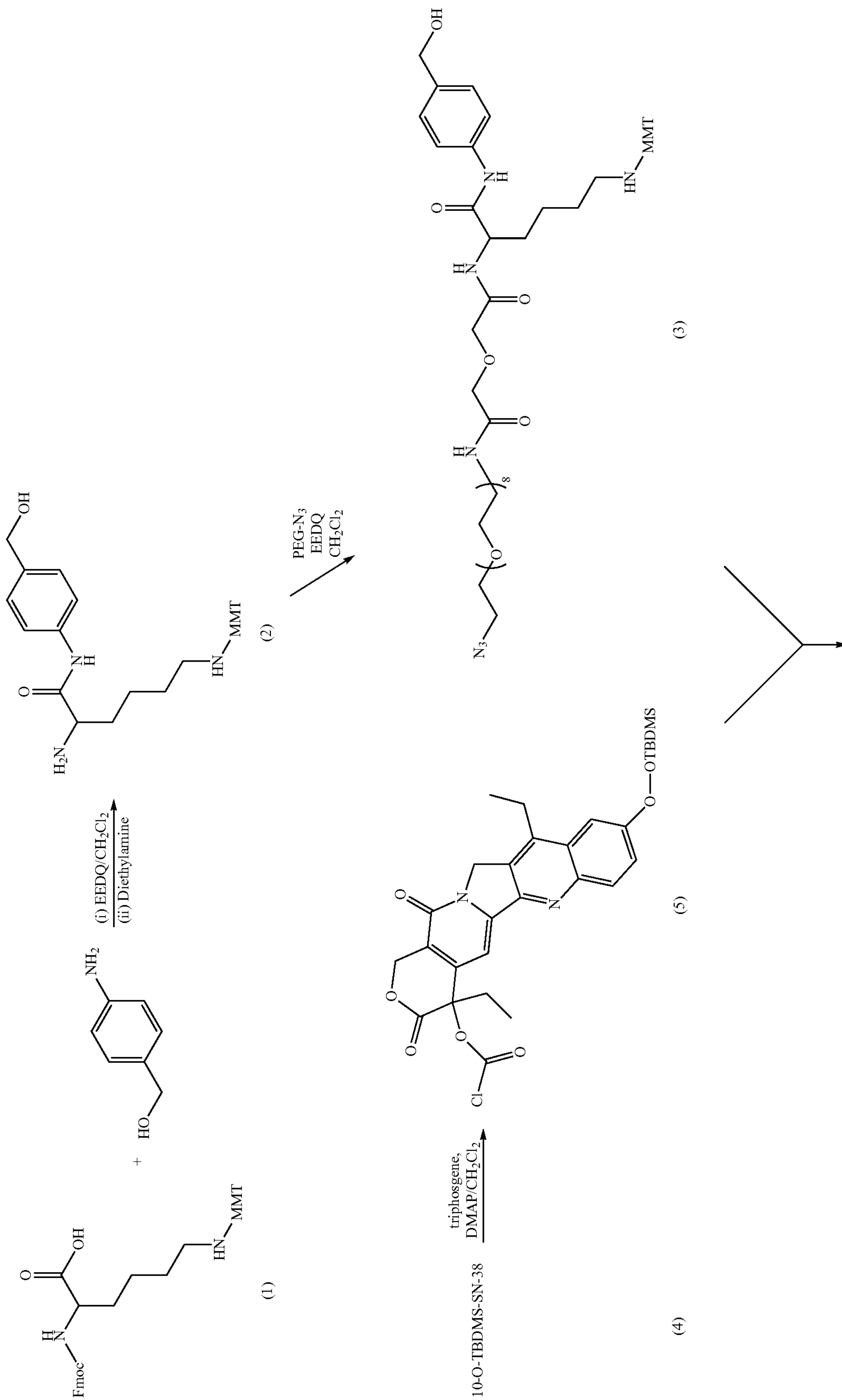
Scheme-3: Preparation of CL2A-SN-38
