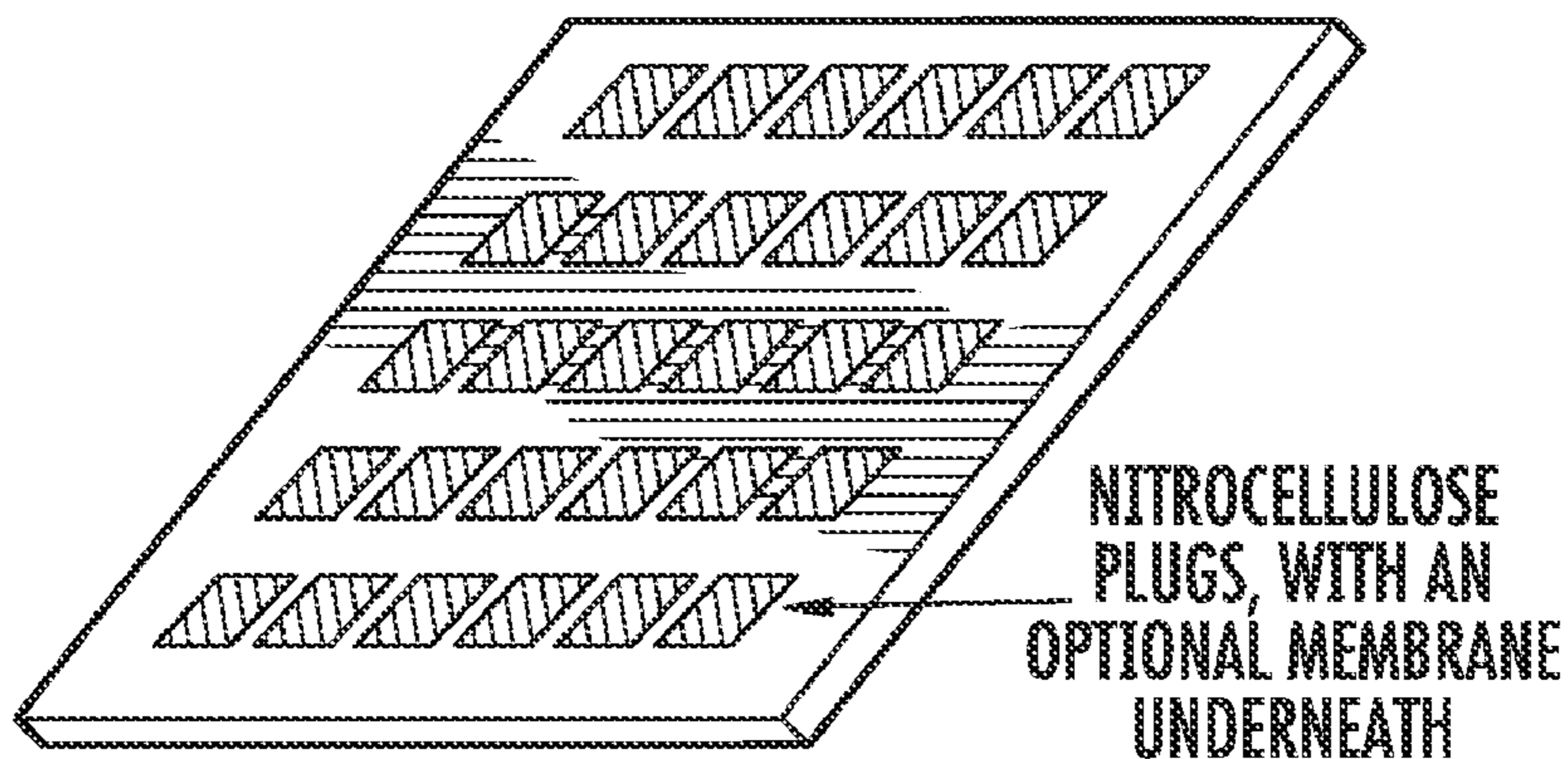
TWO EXAMPLES OF THE TYPES OF MATERIAL THAT CAN BE USED TO MANUFACTURE THE 3D POROUS ARRAY
