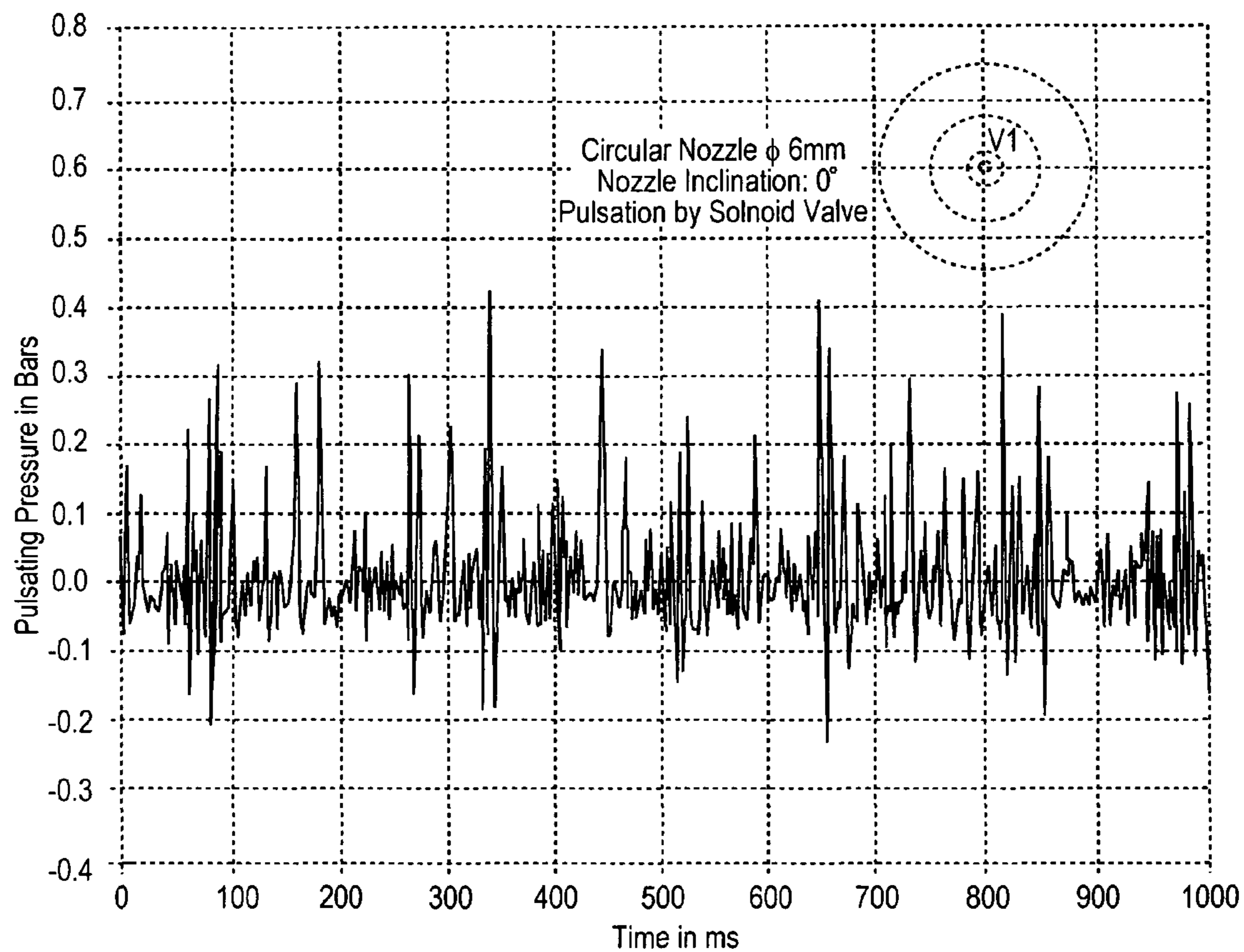
Pulsating Pressures Measured at Measuring Point V1, pulsation frequency adjusted to 7 Hz
