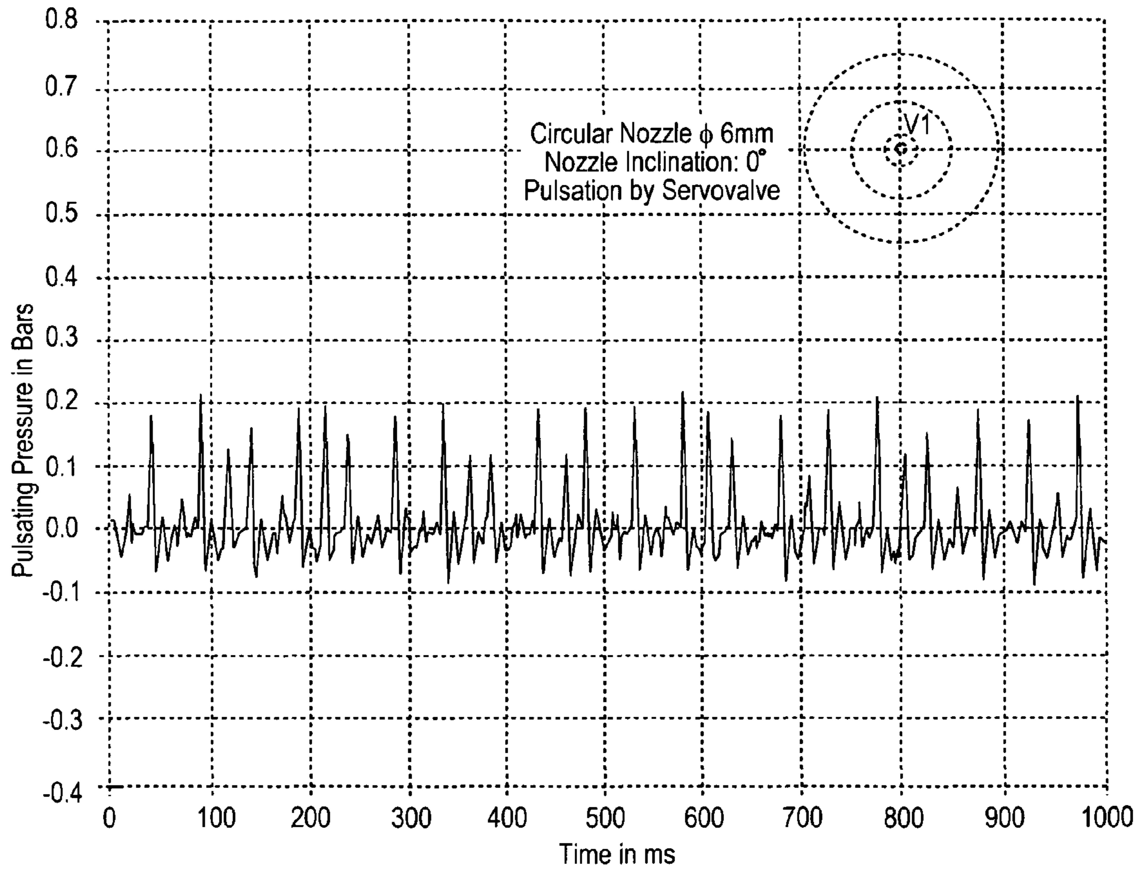
Pulsating Pressures Measured at Measuring Point V1, pulsation frequency adjusted to 20 Hz
