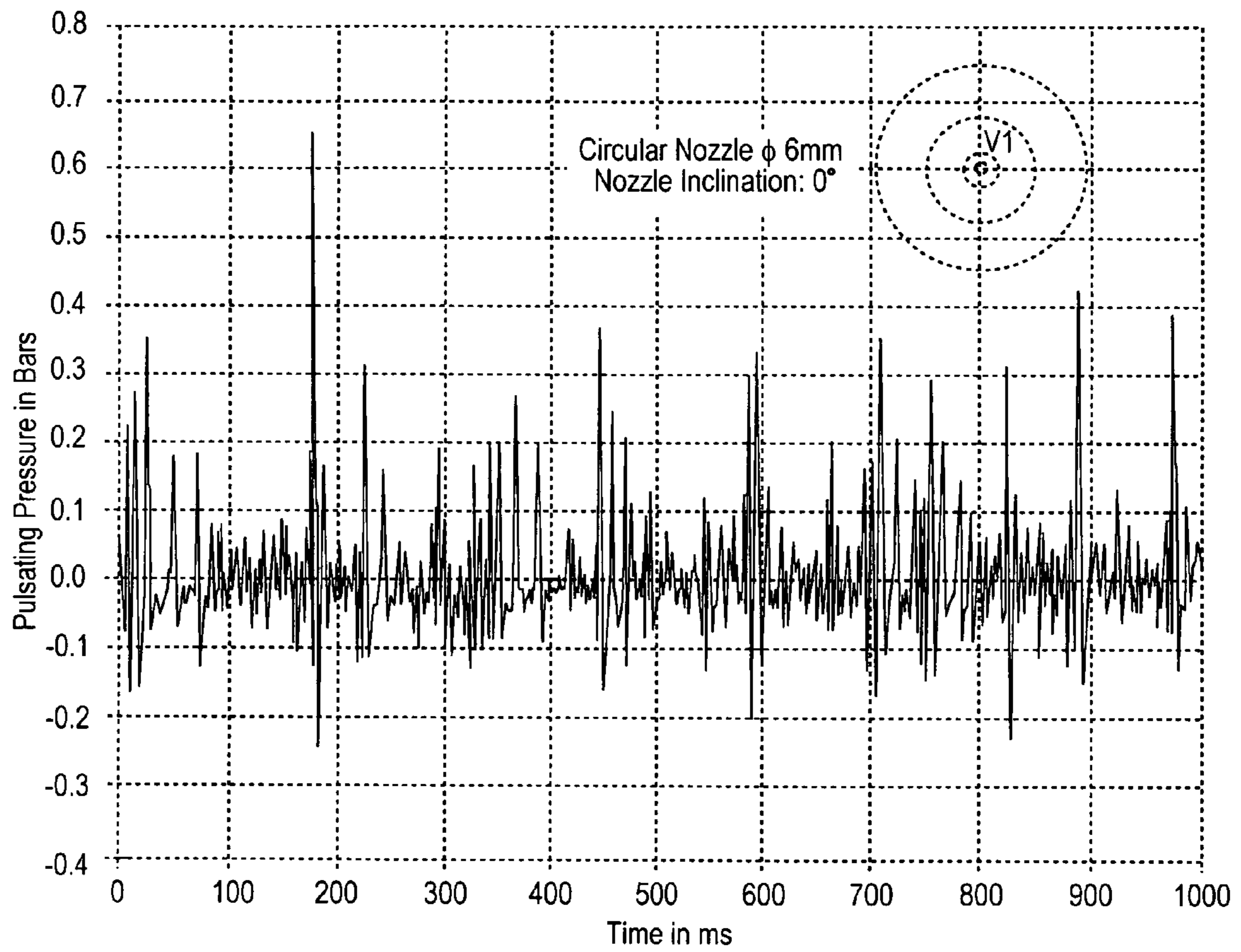
Pulsating Pressures Measured at Measuring Point V1, without value
