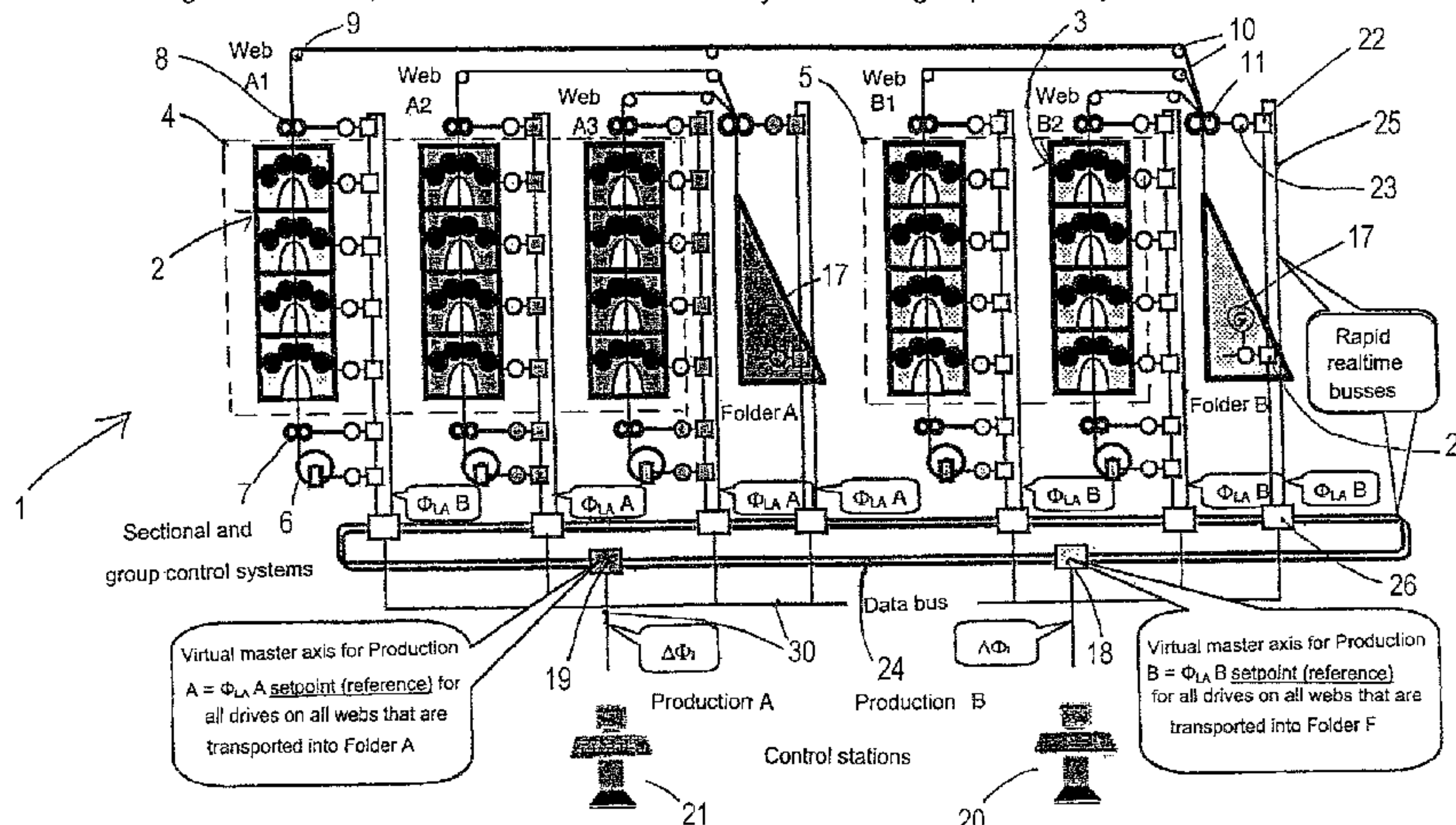
Basic design of a shaftless drive system for two sub-machines A+B (sections), each having several webs, with sectional motion control systems and group control systems
