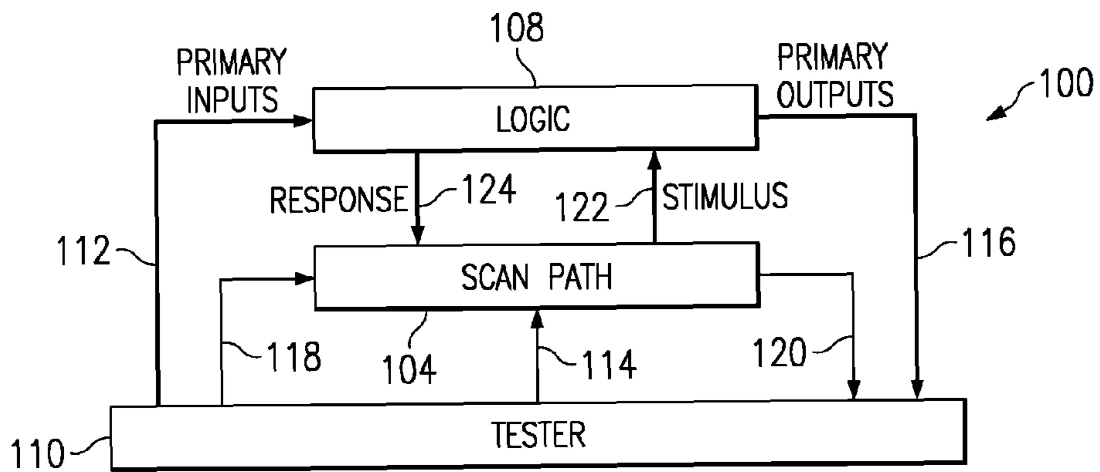
FIG. 1 (PRIOR ART)
