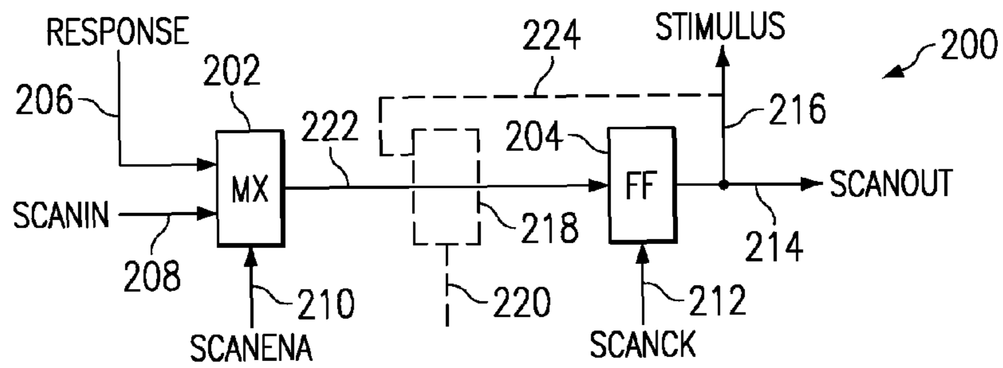
FIG. 2 (PRIOR ART)
