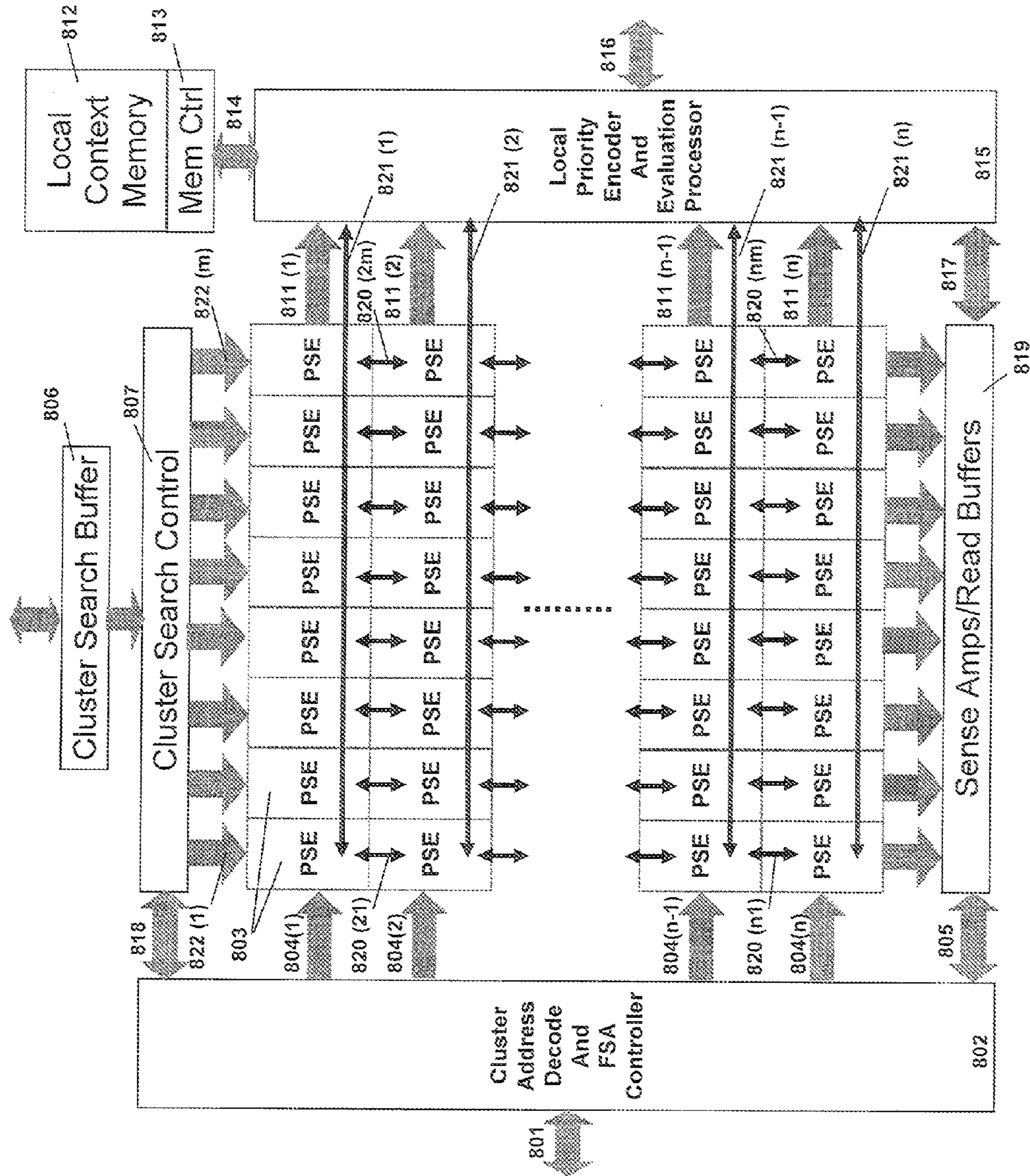
Fig. 8b PRISM Memory Cluster Detailed Block Diagram
