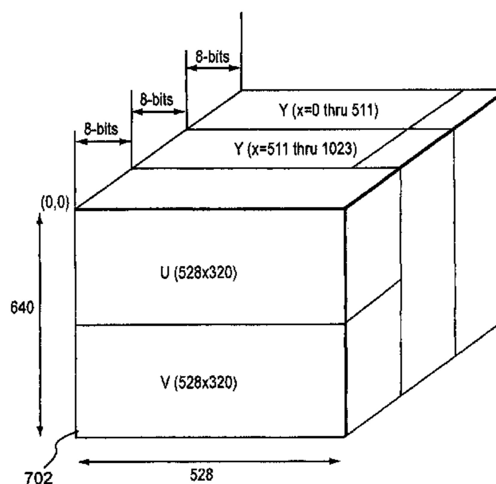
(Embedded Frame Buffer Organization)
