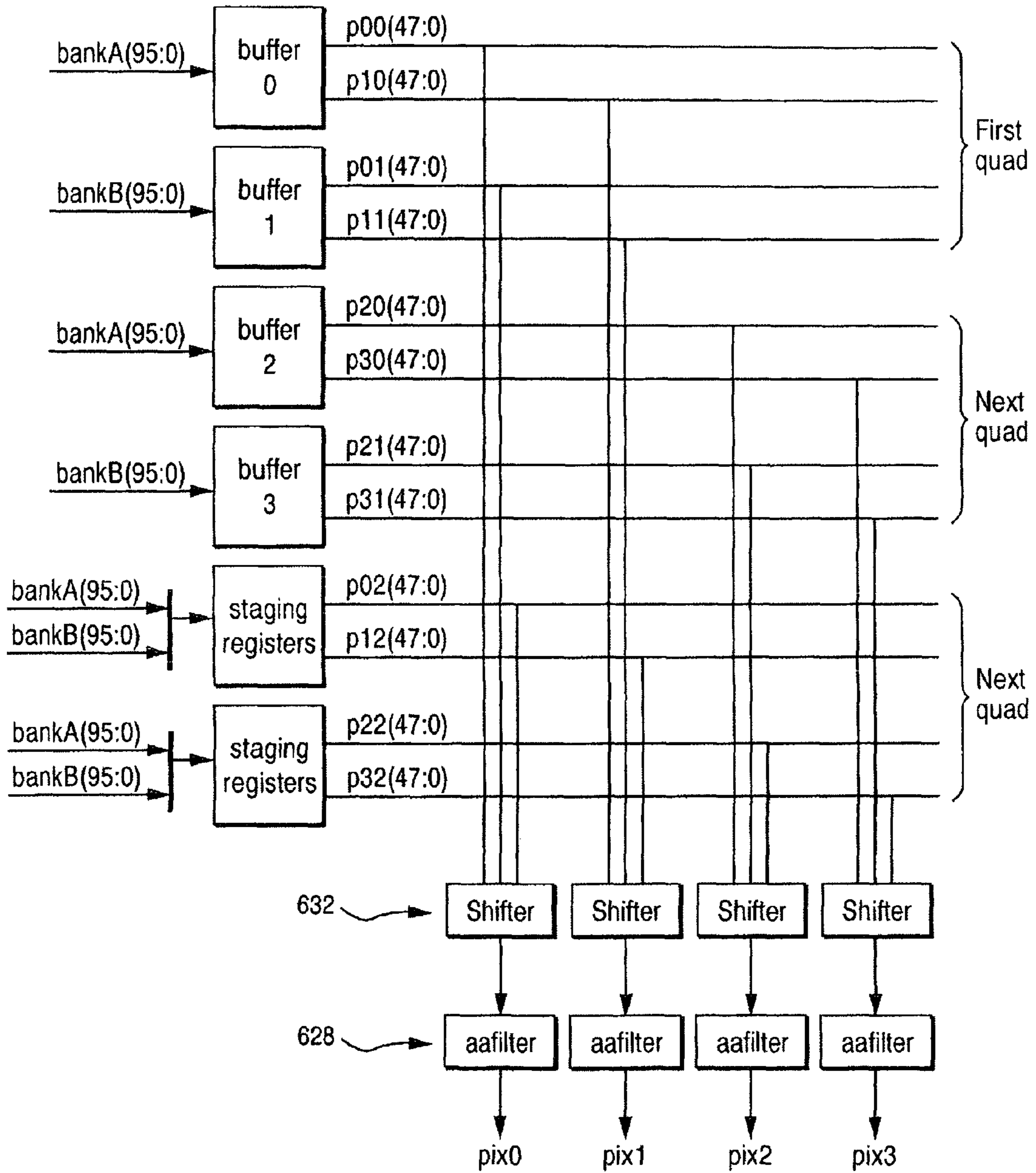
Fig. 12B (AA buffering)
