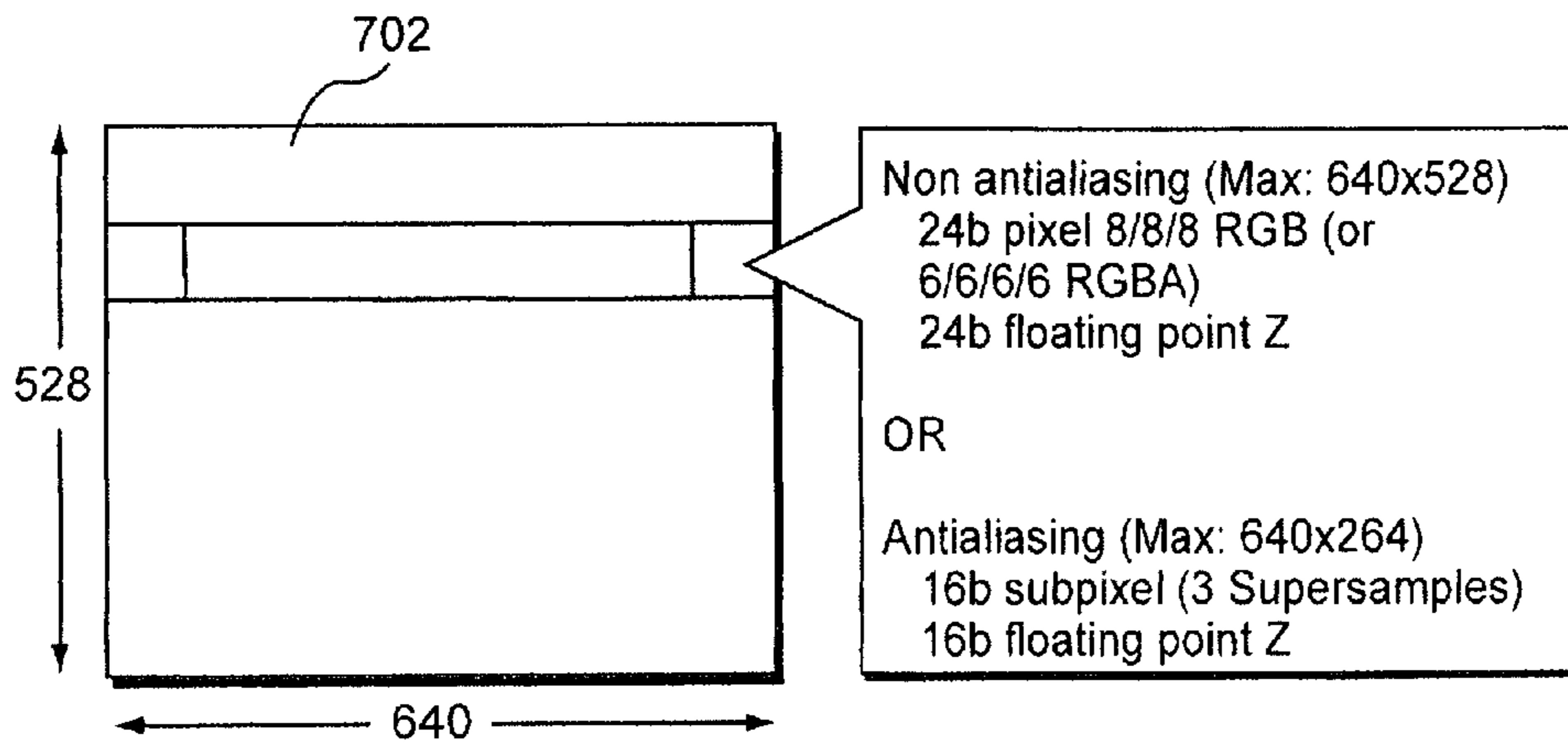
Fig. 6 (Embedded Frame Buffer (EFB))
