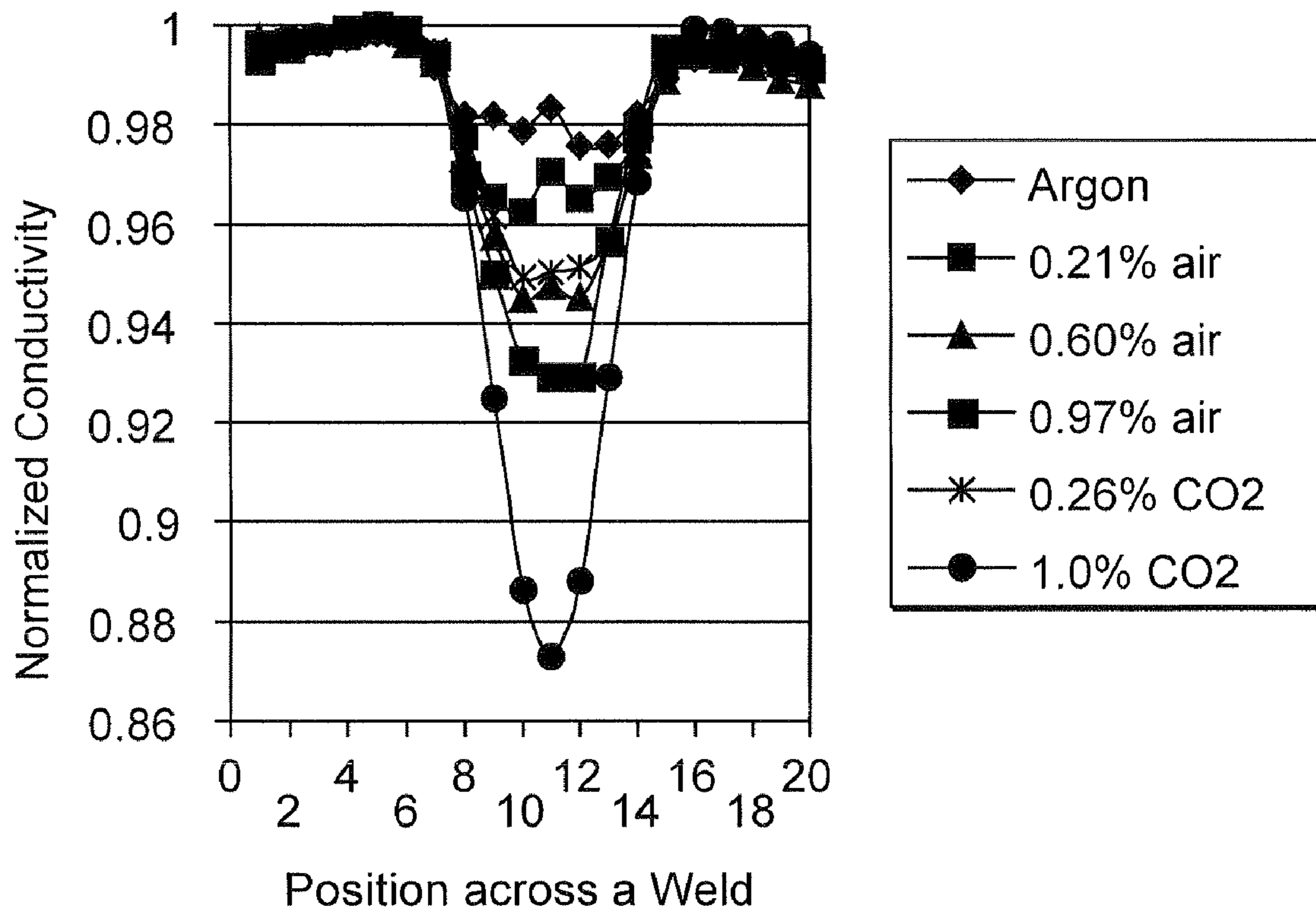
MWM Monitoring of Weld Quality in GTAW Ti-2 Welds at 400 kHz
