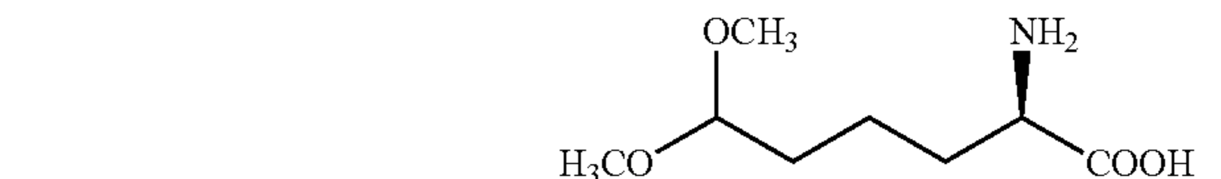
(R)-2-amino-6,6-dimethoxy hexanoic acid
