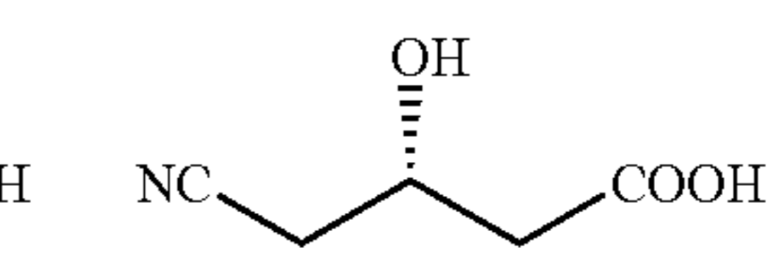
3-hydroxy-cyano gluteric acid side chain for Lescol
