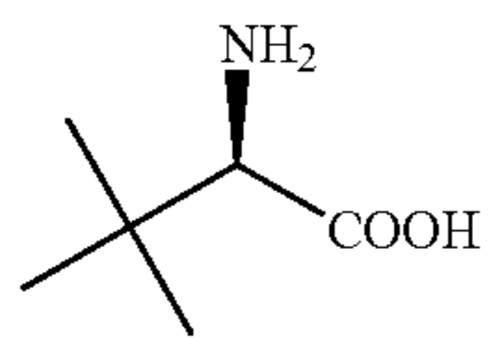
D-tertiary leucine
