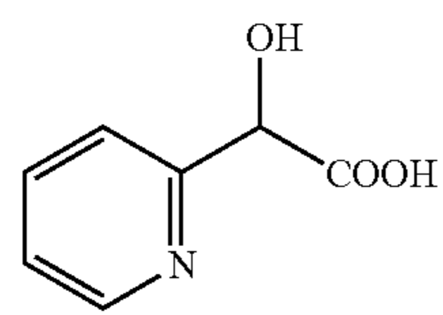
2-pyridyl glycolic acid
