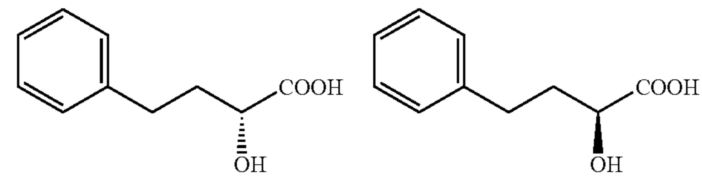
(R)-2-hydroxy-4-phenyl butyric acid
