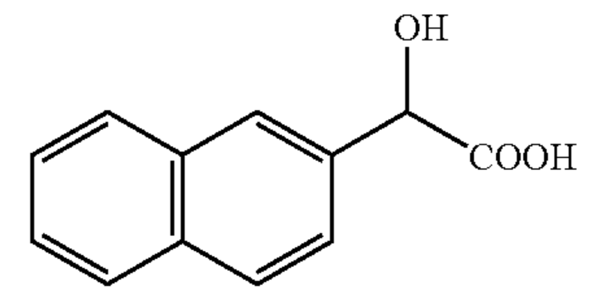
2-naphthyl glycolic acid
