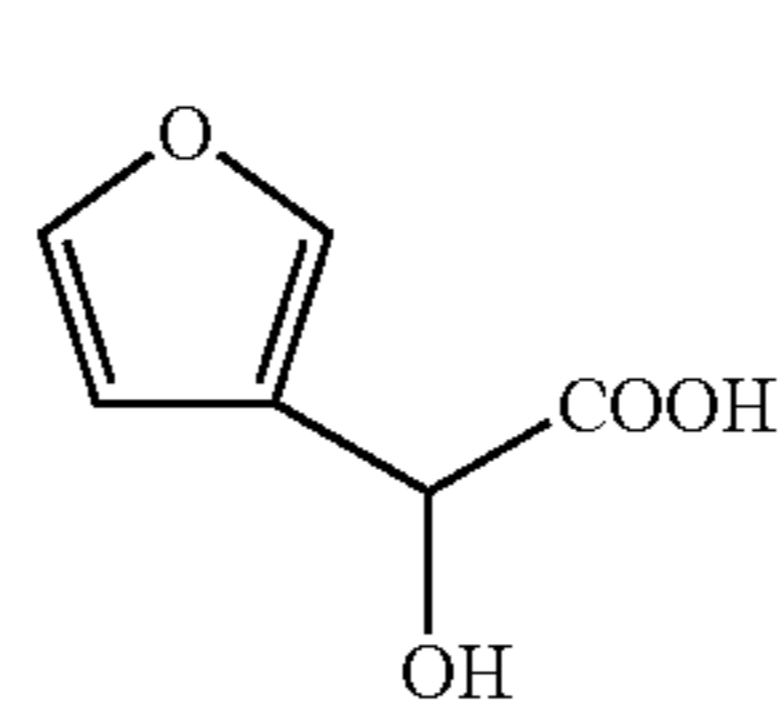
3-furanyl glycolic acid
