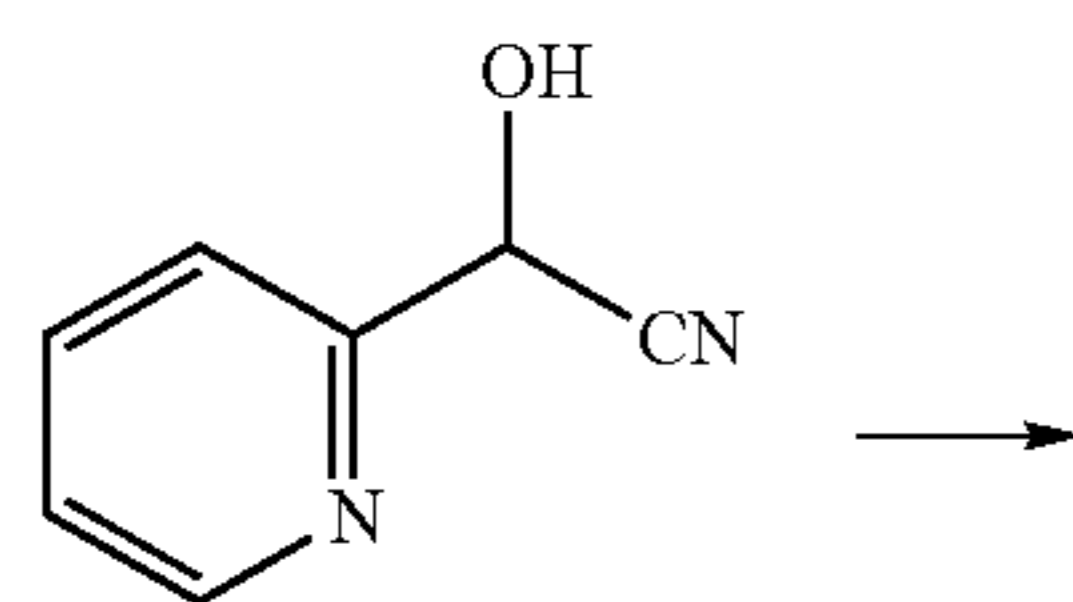
2-pyridyl formaldehyde cyanohydrin
