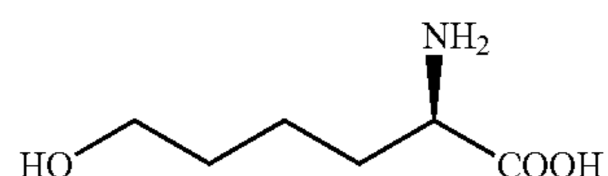
(R)-2-amino-6-hydroxy hexanoic acid
