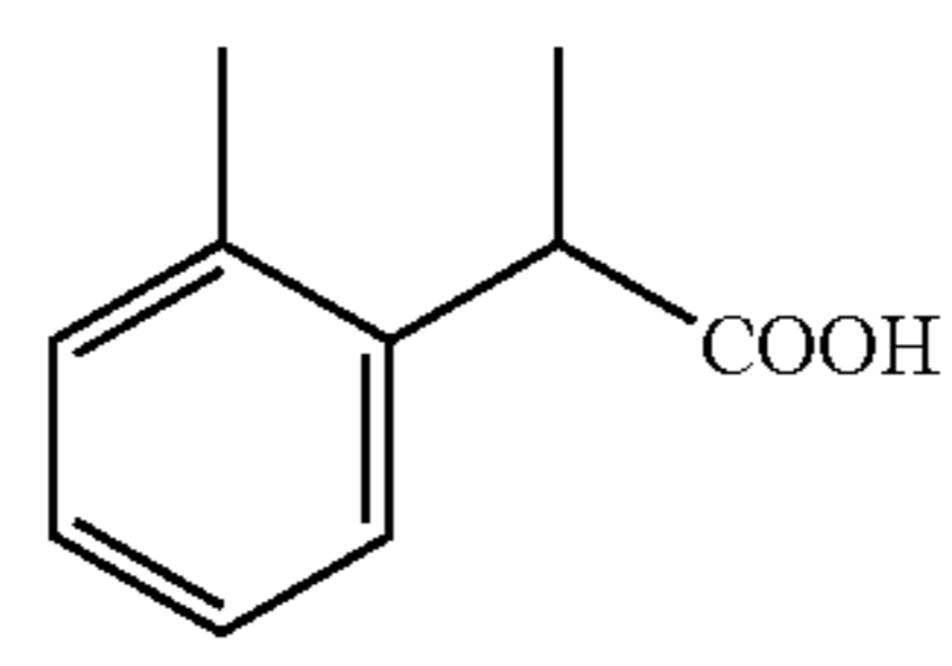
methyl-mandelic acid
