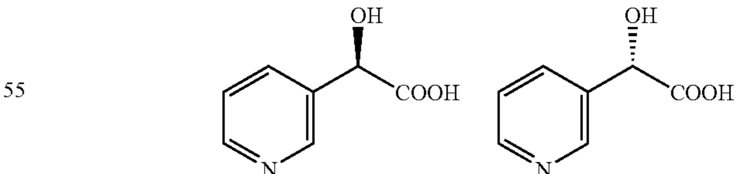
(R)-3-pyridyl glycolic acid (S)-3-pyridyl glycolic acid
