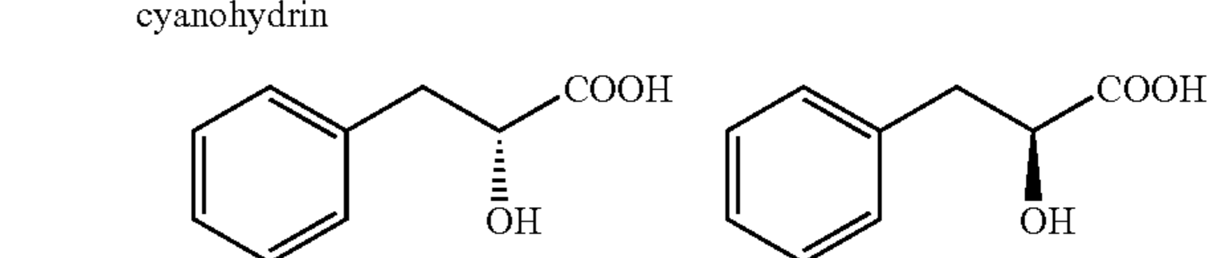
(R)-phenyl lactic acid
