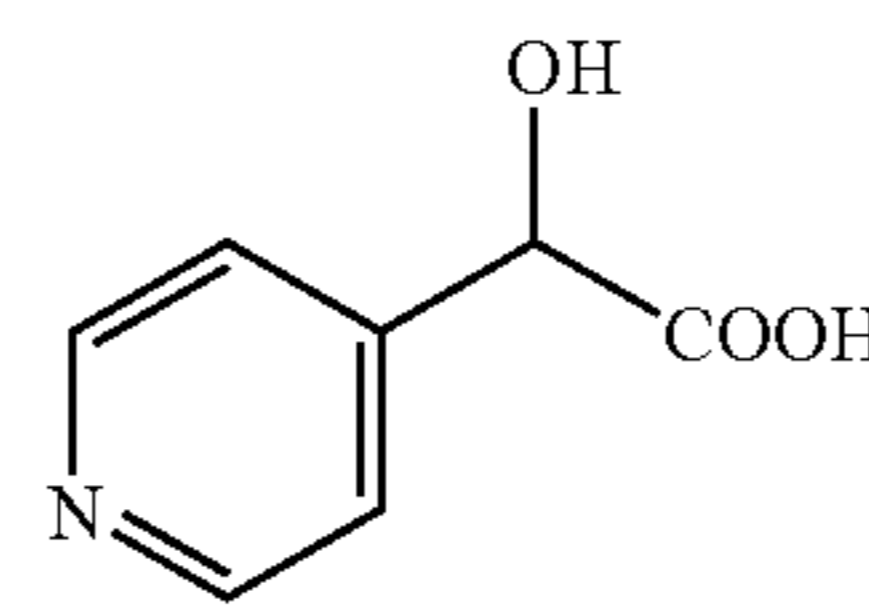
4-pyridyl glycolic acid
