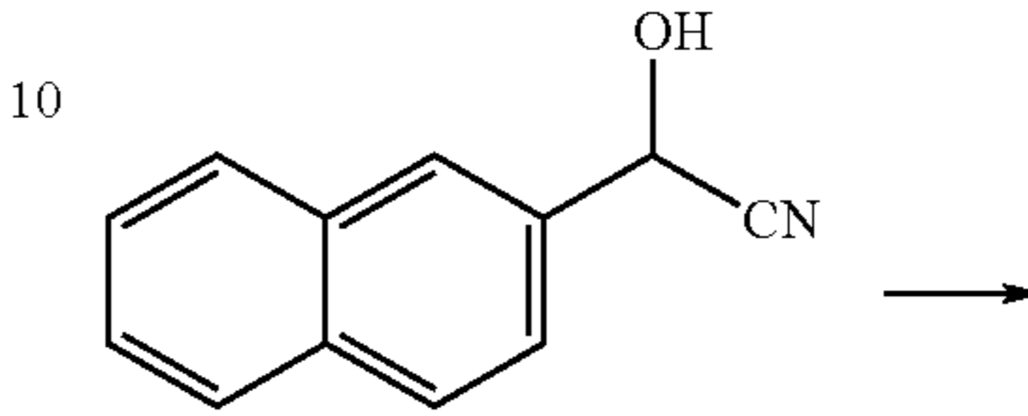
2-naphthyl formaldehyde cyanohydrin
