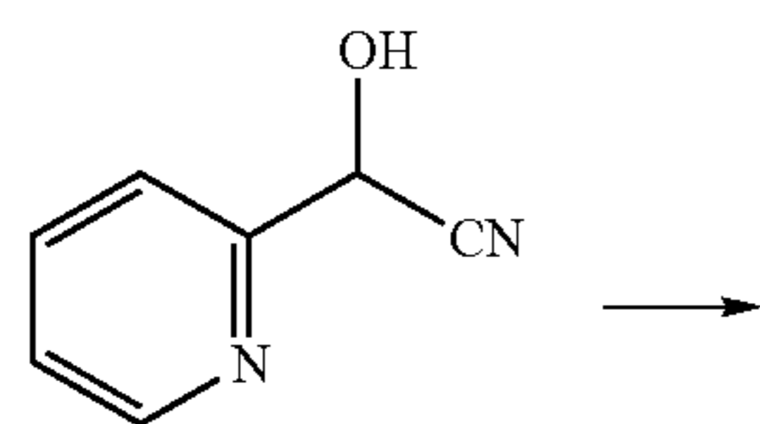
2-pyridyl formaldehyde cyanohydrin
