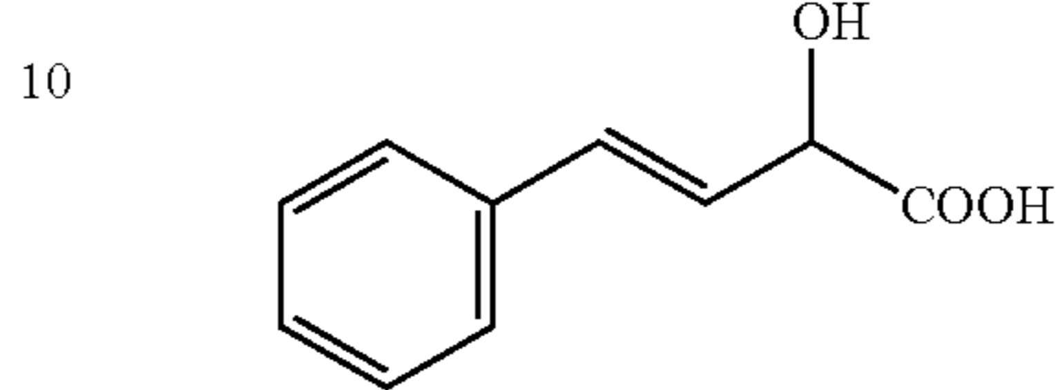
4-phenyl-2-hydroxy-3,4-butenoic acid
