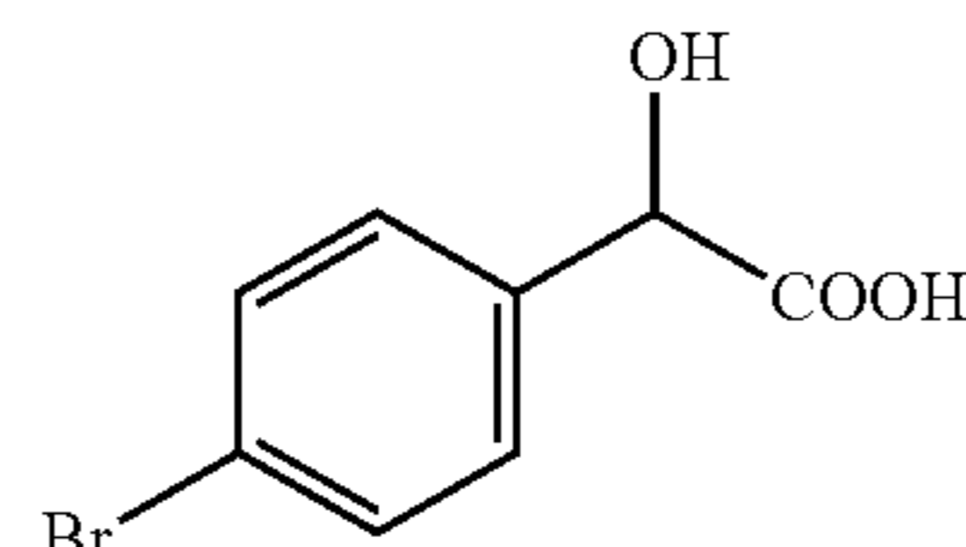
bromo-mandelic acid
