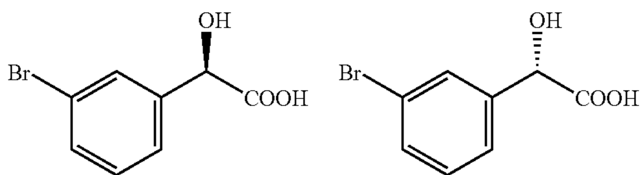
(R)-3-bromo mandelic acid (S)-3-bromo mandelic acid
