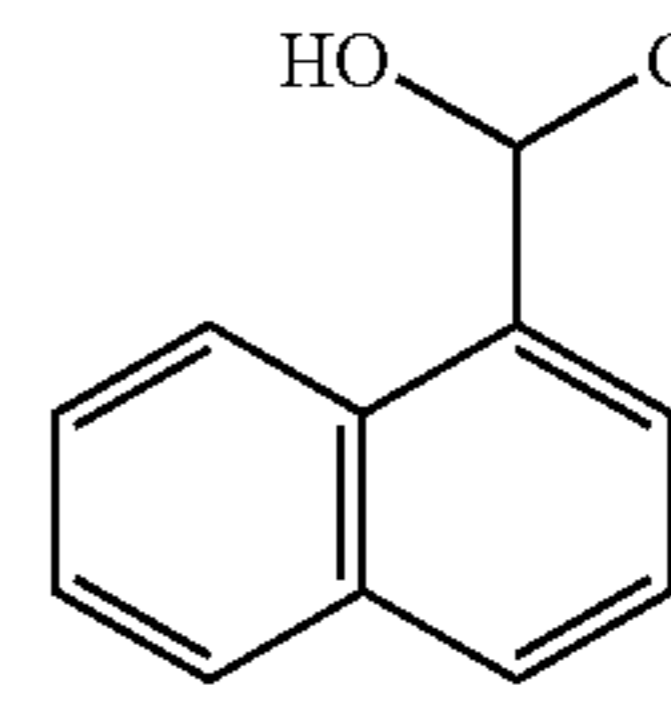
1-naphthyl glycolic acid
