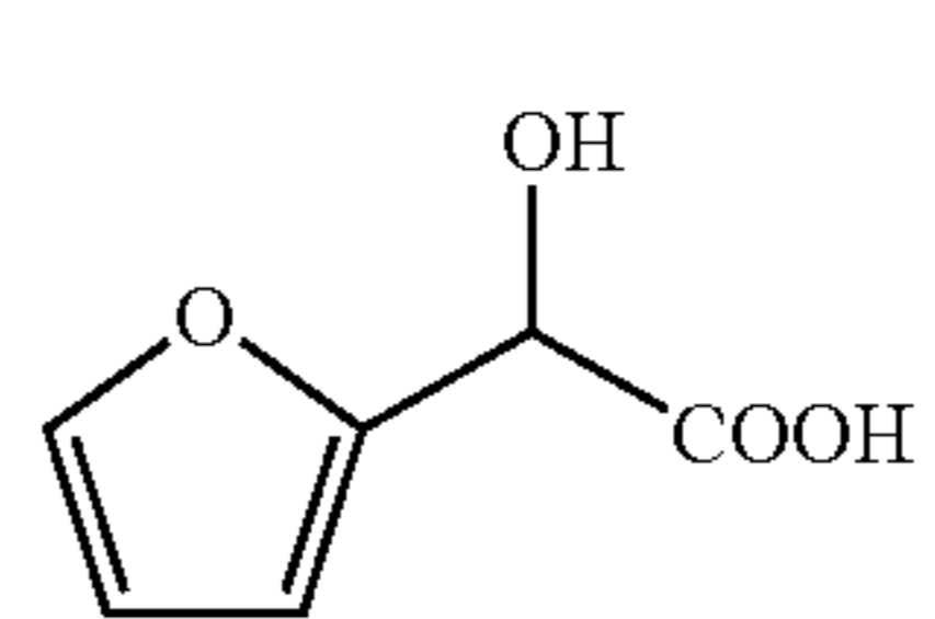
2-furanyl glycolic acid
