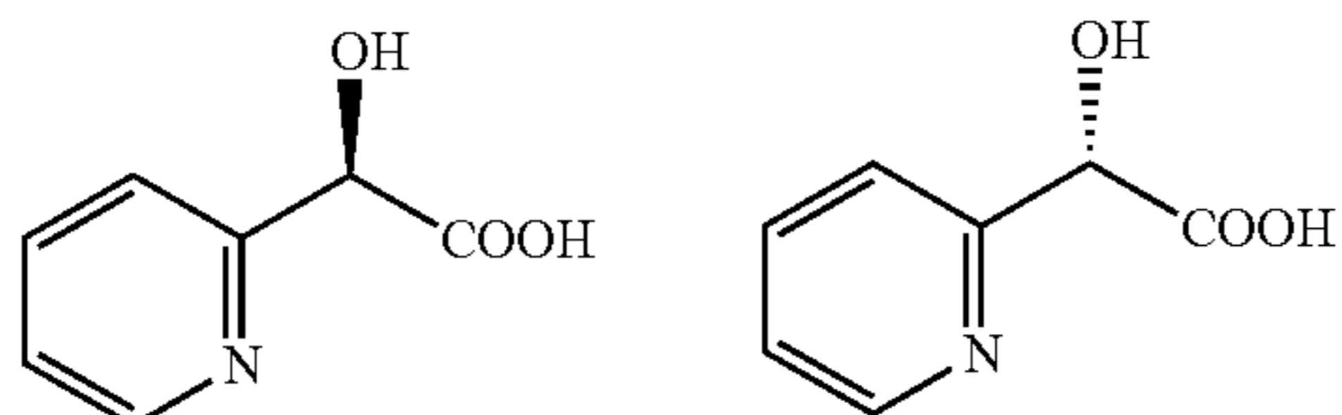
(R)-pyridyl glycolic acid
