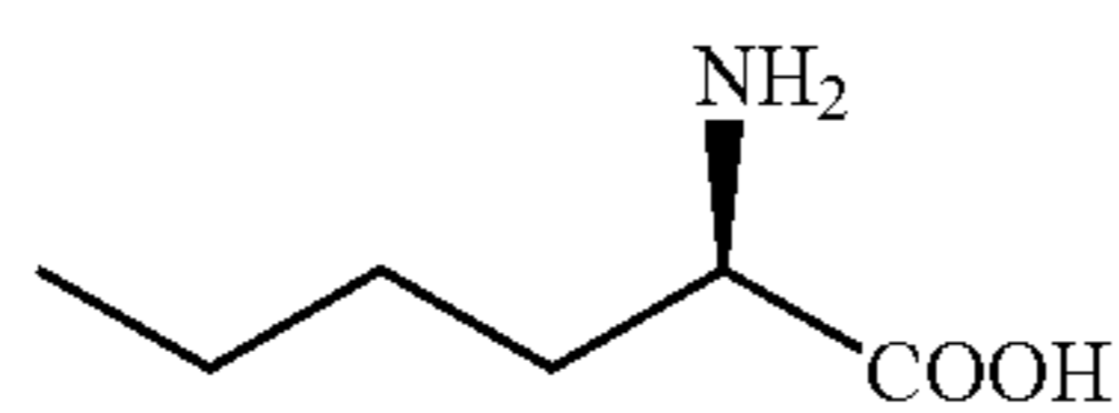
D-norleucine
