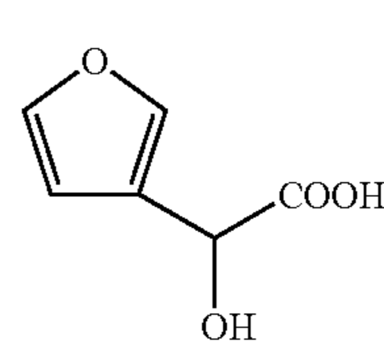
3-furanyl glycolic acid
