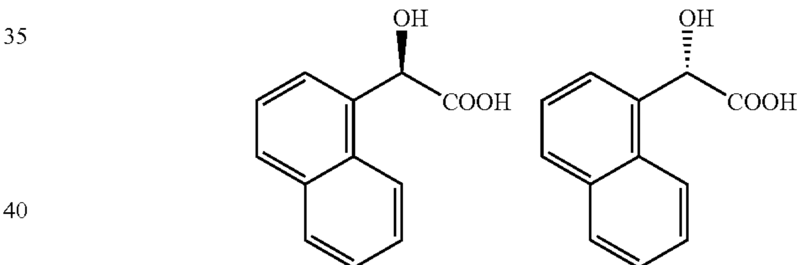
(R)-1-naphthylglycolic acid (S)-1-naphthylglycolic acid
