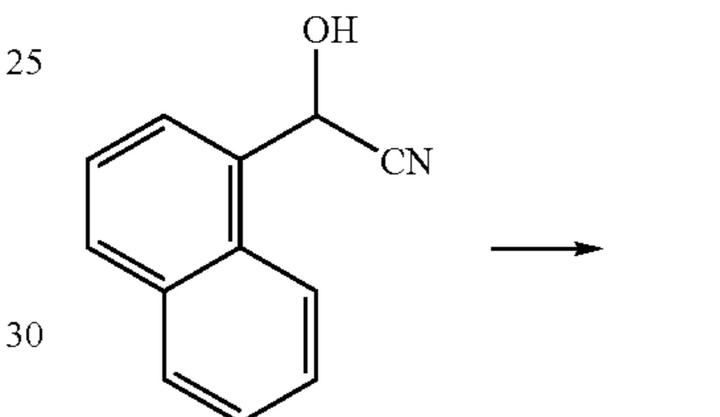
1-naphthyl formaldehyde cyanohydrin
