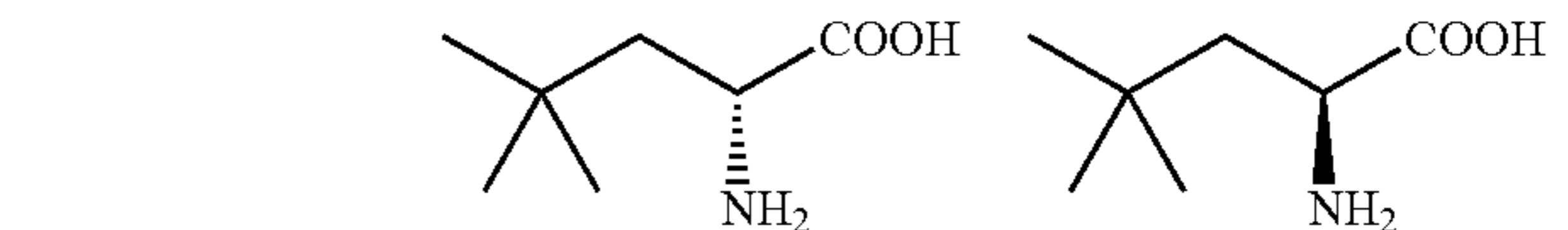
(R)-2-amino-4,4-dimethyl pentanoic acid
