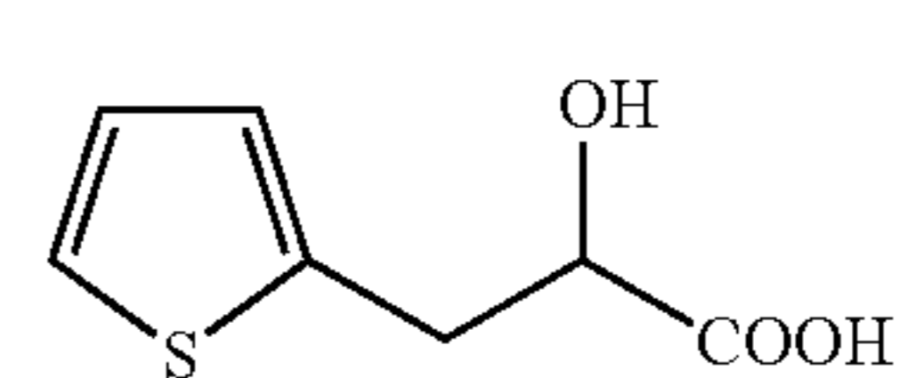
thienyl acetic acid
