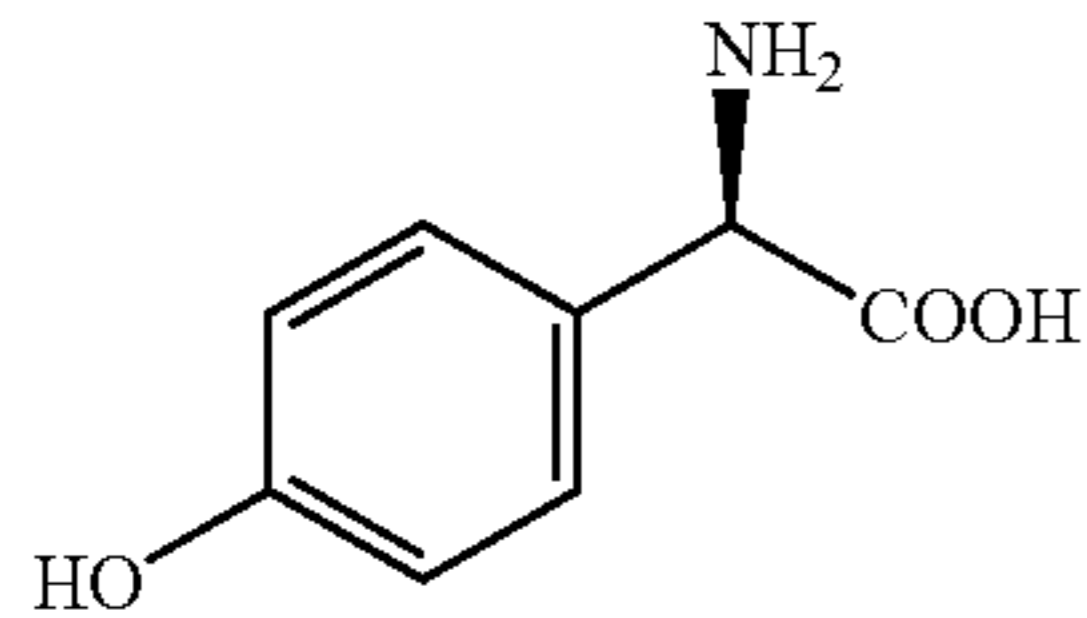
D-4-hydroxyl phenylglycine
