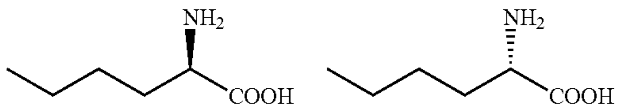
(R)-2-amino-hexanoic acid
