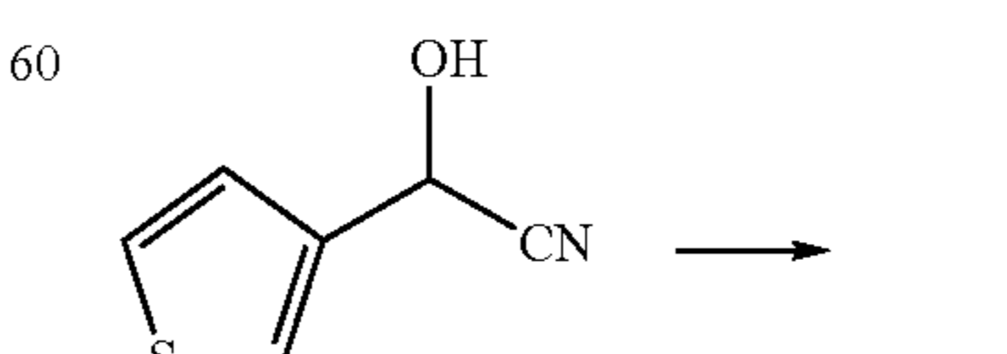
3-thienyl formaldehyde cyanohydrin
