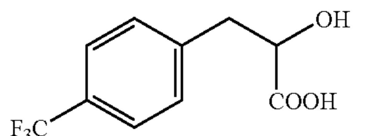
trifluoromethylphenyl lactic acid
