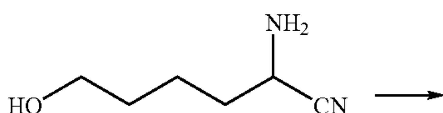
2-amino-6-hydroxy hexanenitrile
