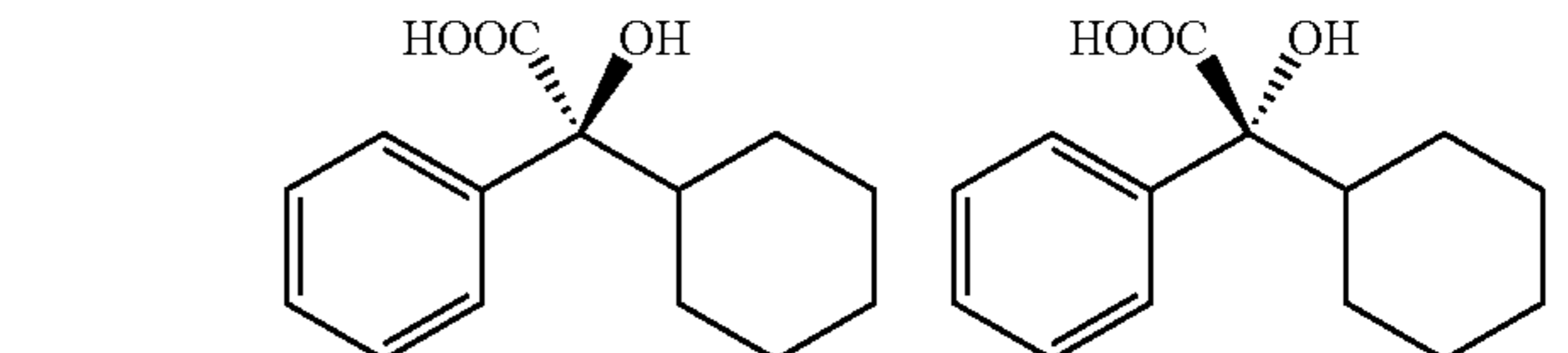
(S)-cyclohexyl mandelic acid
