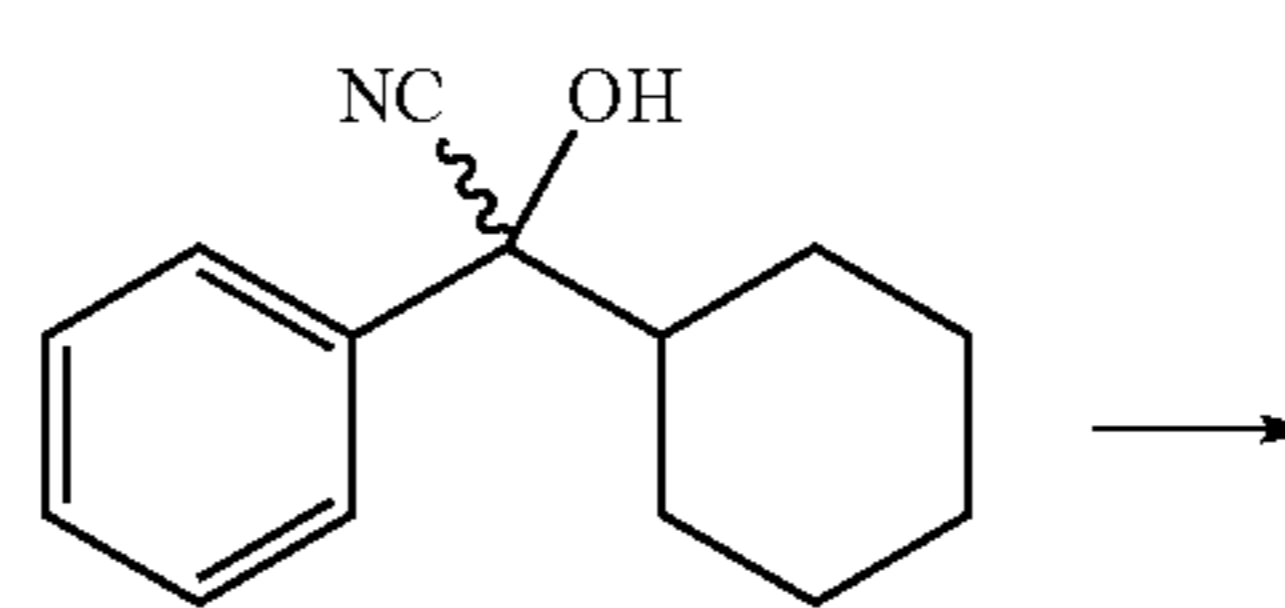
cyclohexyl mandelonitrile
