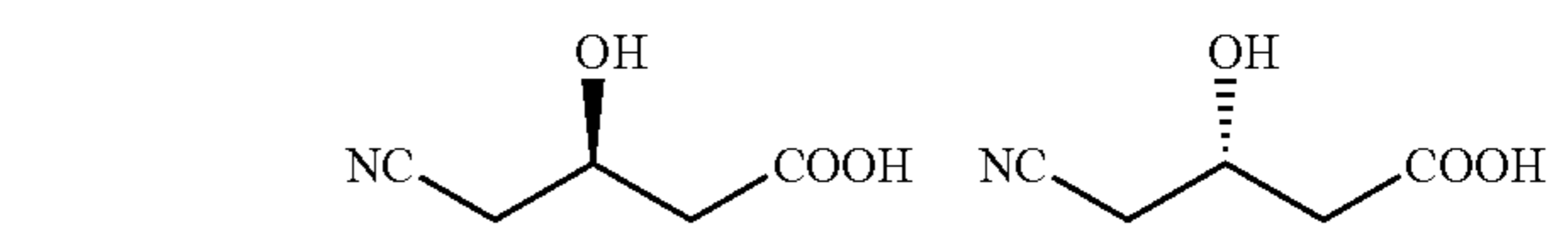
(R)-(3)-hydroxy-4-cyano-butrylic acid
