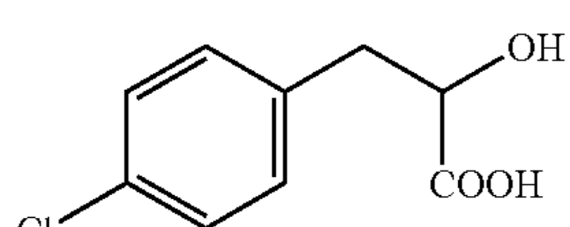
chlorophenyl lactic acid
