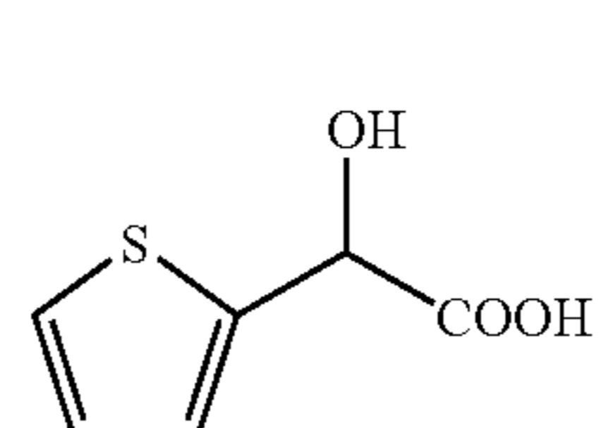
2-thienyl glycolic acid
