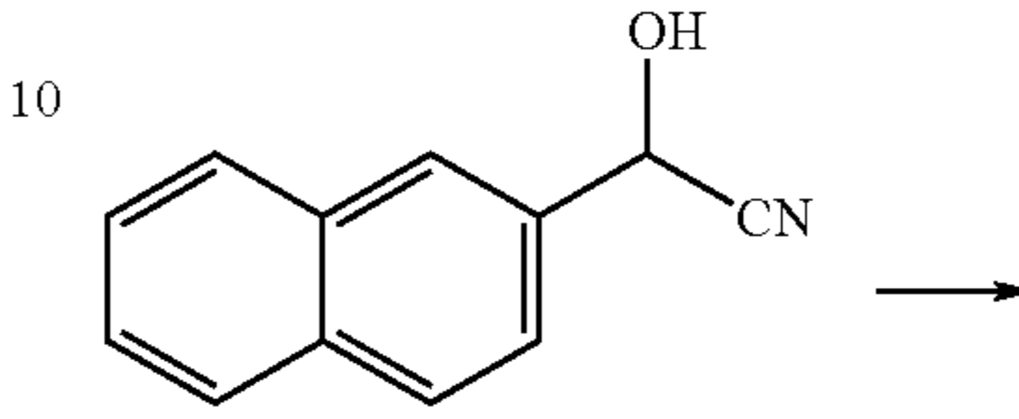
2-naphthyl formaldehyde cyanohydrin
