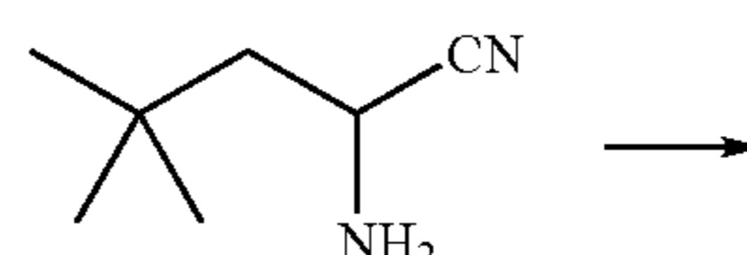
2-amino-4,4-dimethyl pentanenitrile
