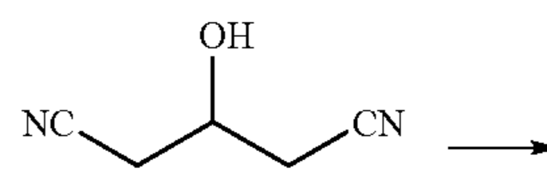
hydroxyglutarylnitrile
