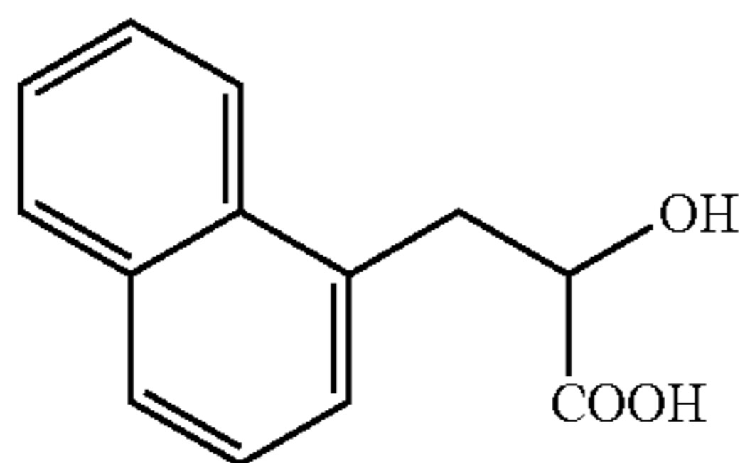
naphthyl acetic acid
