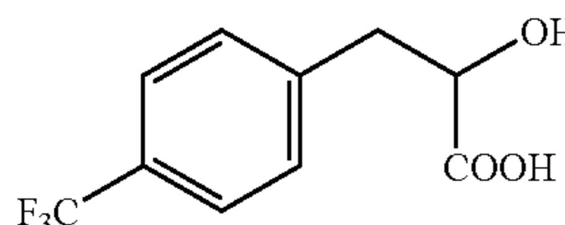
trifluoromethylphenyl lactic acid
