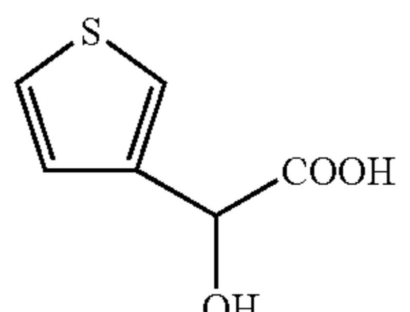
3-thienyl glycolic acid
