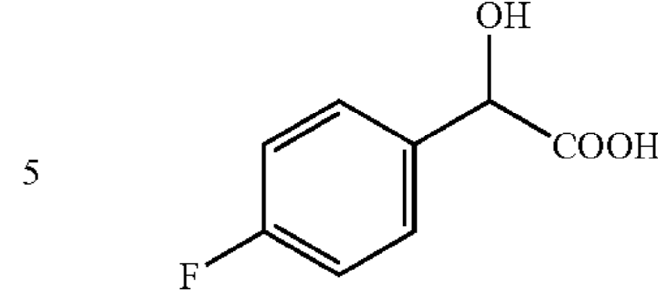
fluoro-mandelic acid
