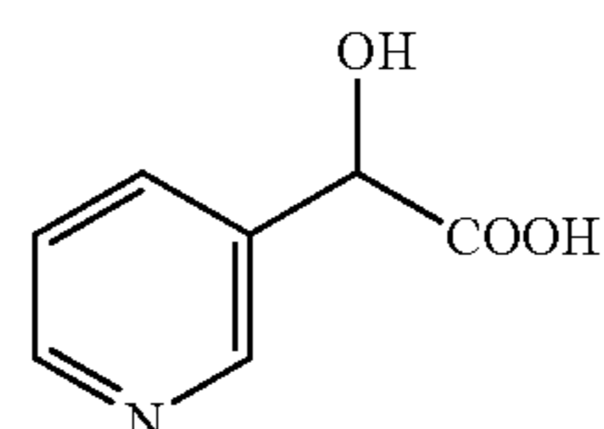
3-pyridyl glycolic acid
