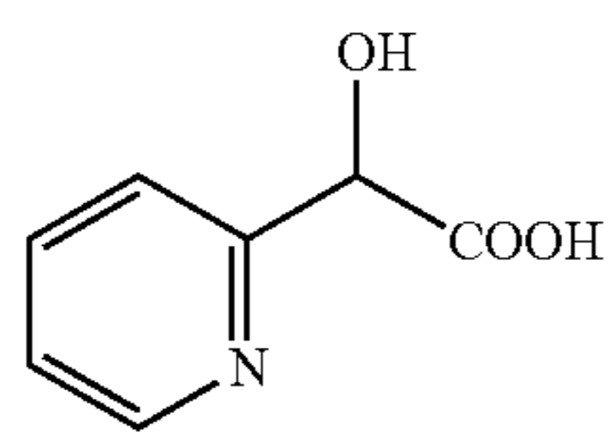
2-pyridyl glycolic acid
