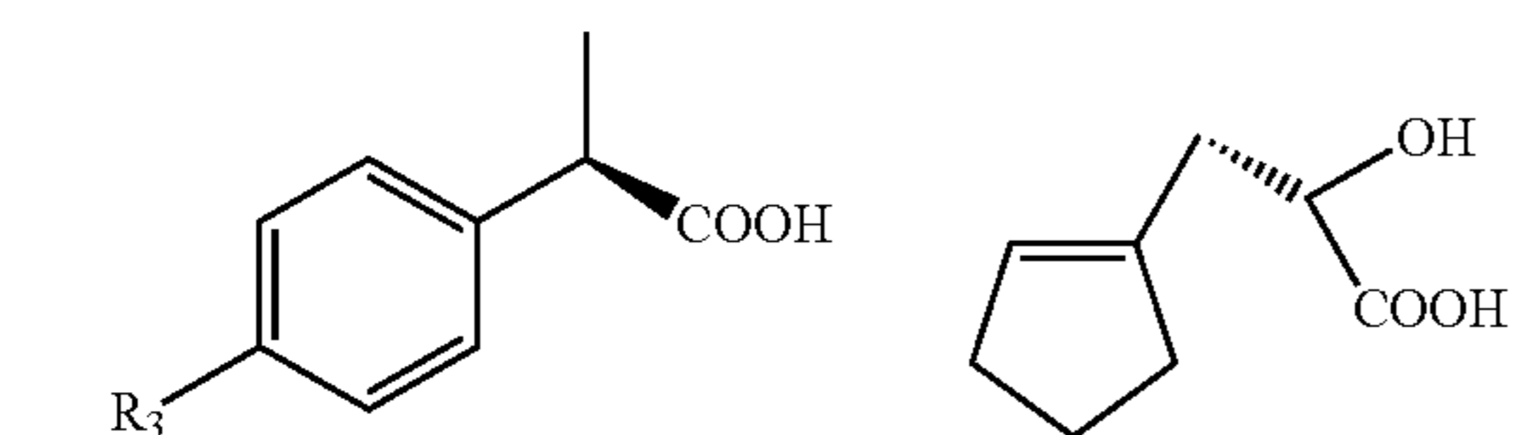
alpha-methyl benzyl cyanide derivatives intermediate for Trocade
