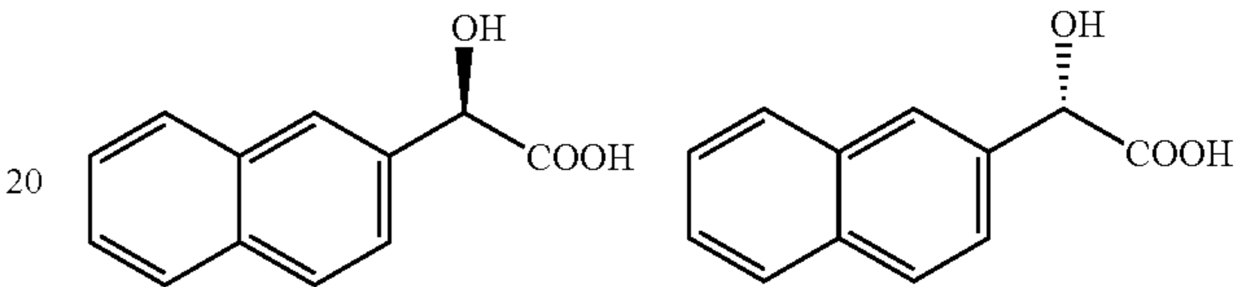
(R)-2-naphthylglycolic acid (S)-2-naphthylglycolic acid
