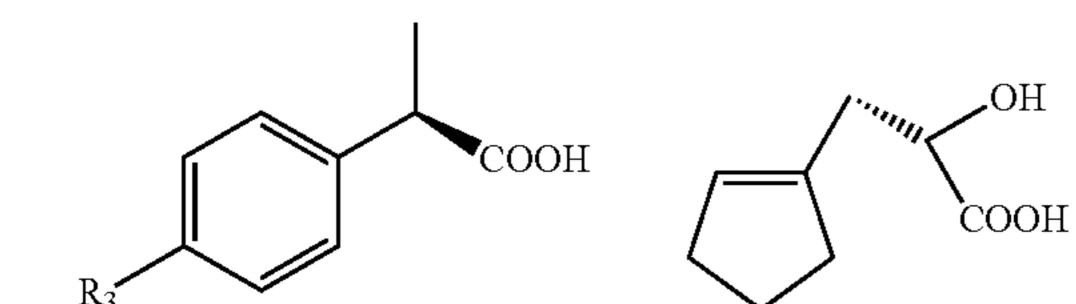
alpha-methyl benzyl cyanide derivatives intermediate for Trocade
