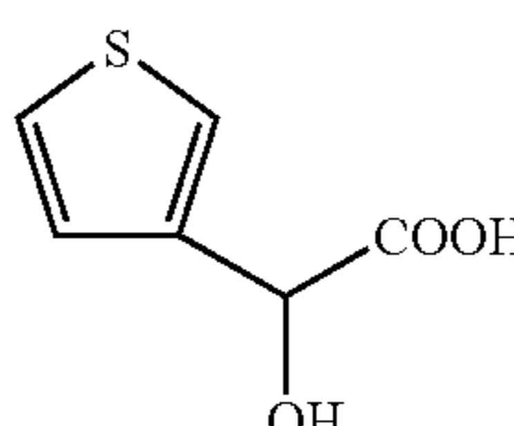
3-thienyl glycolic acid
