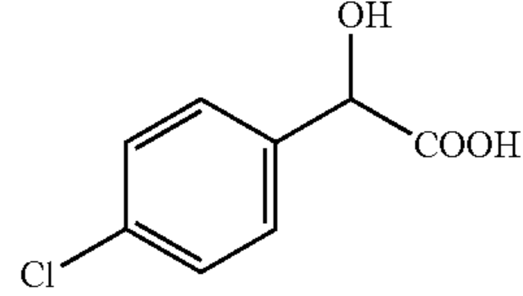
chloro-mandelic acid
