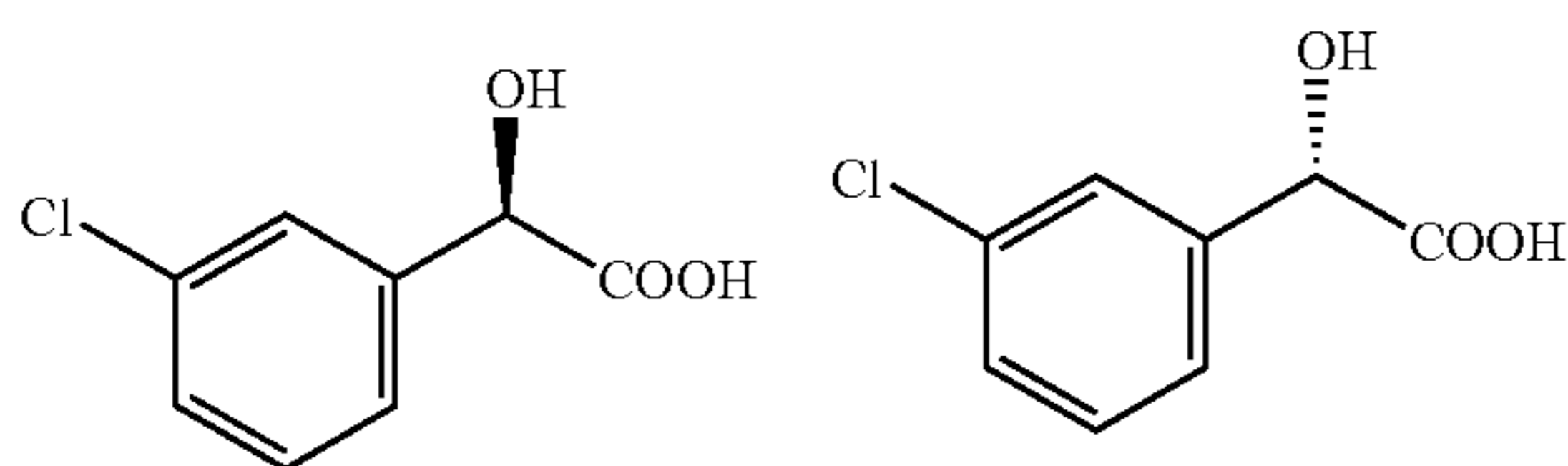
(R)-3-chloro mandelic acid (S)-3-chloro mandelic acid
