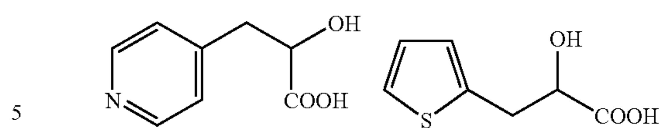
pyridyl acetic acid
