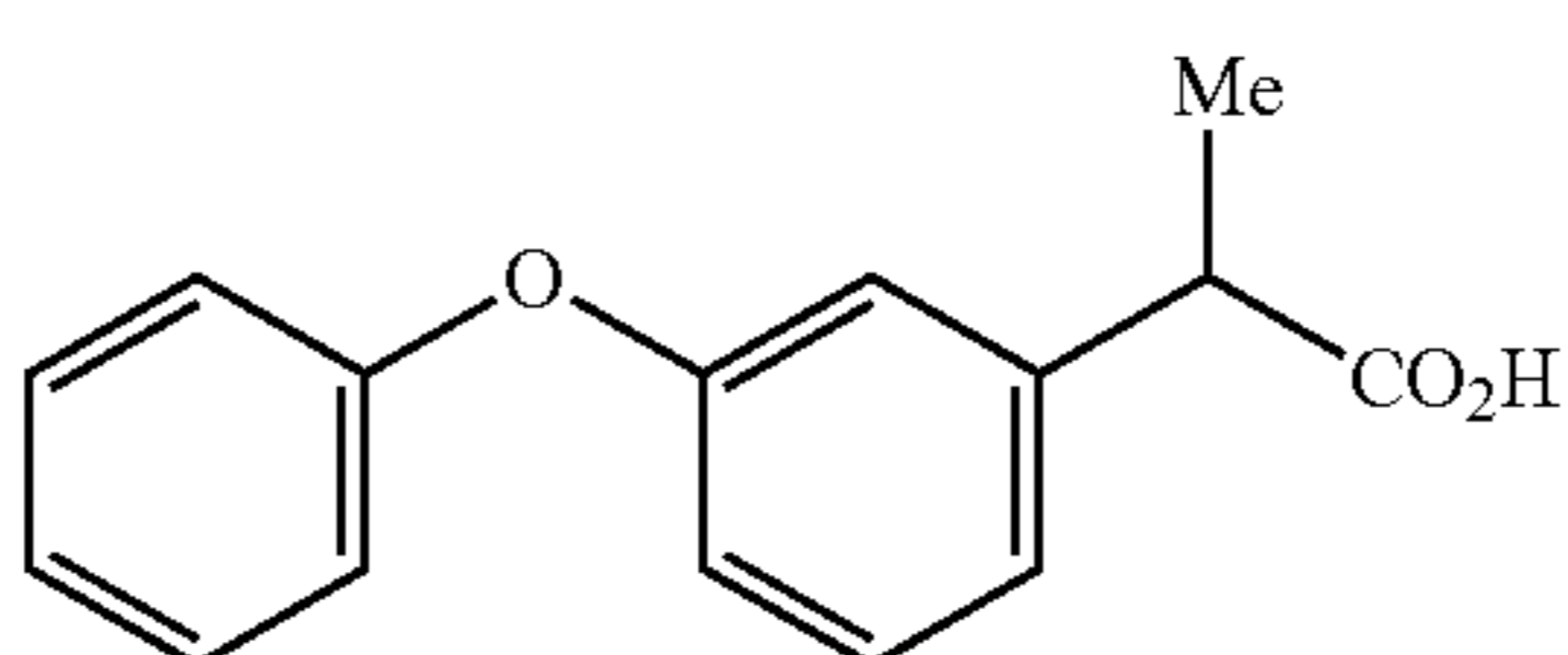
Fenoprofen
