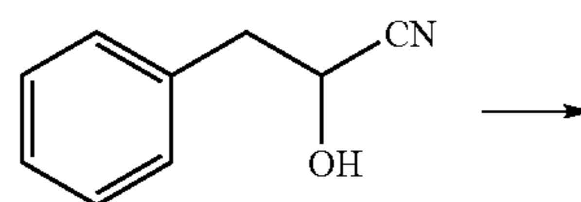
phenyl acetaldehyde cyanohydrin
