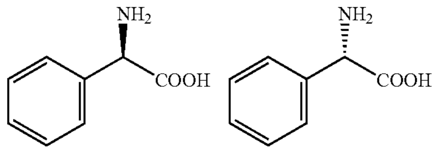
D-phenylglycine
