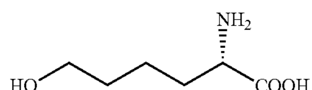
(S)-2-amino-6-hydroxy hexanoic acid
