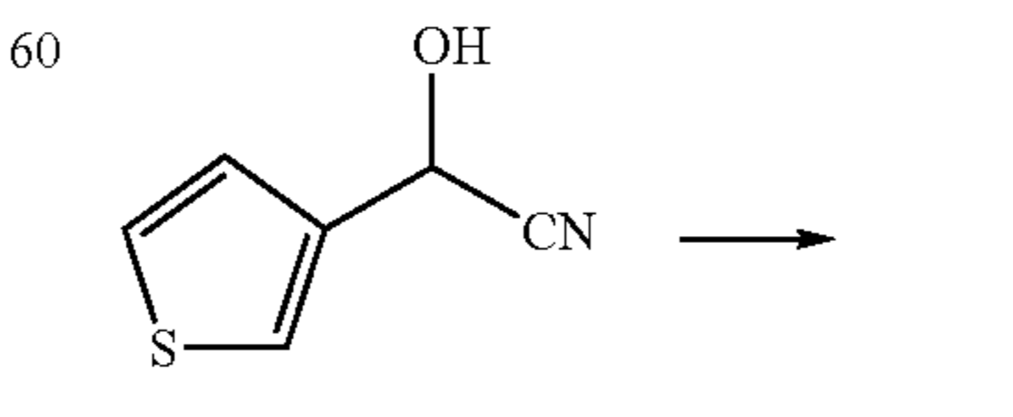
3-thienyl formaldehyde cyanohydrin
