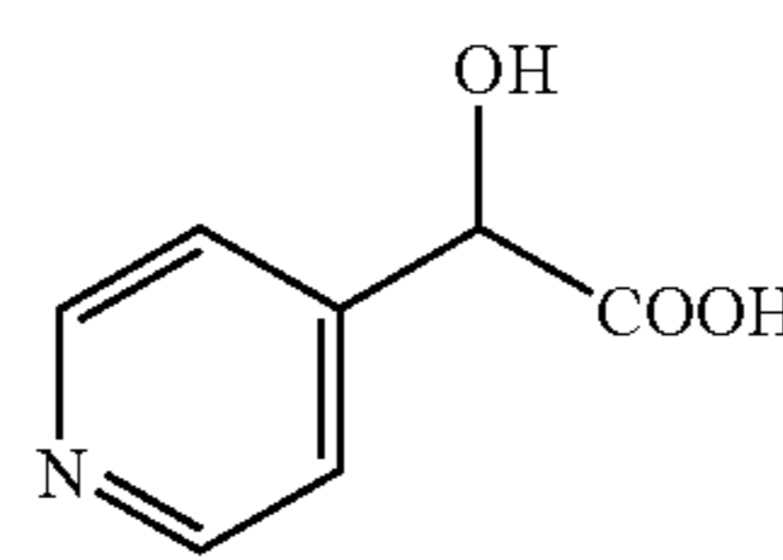
4-pyridyl glycolic acid
