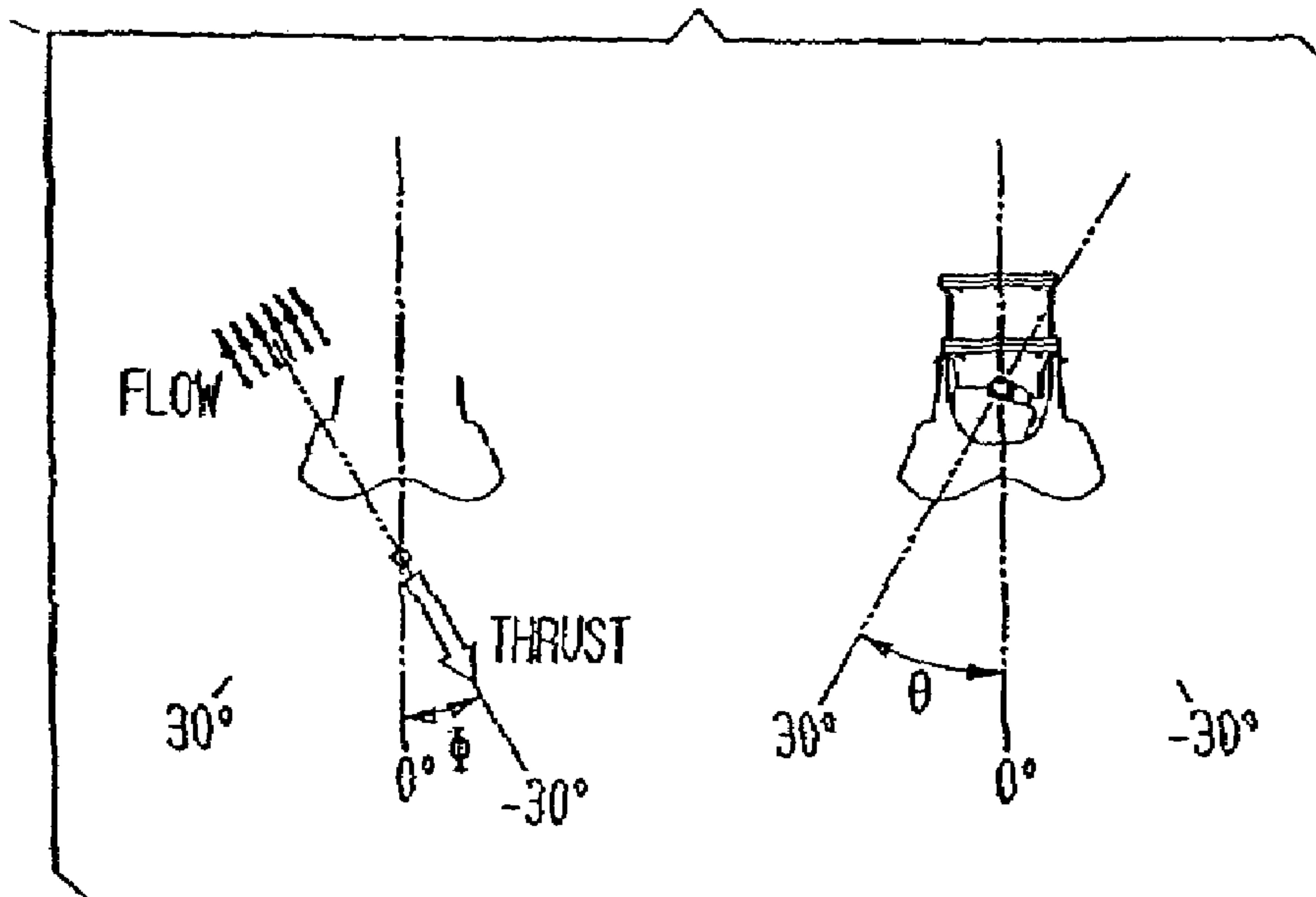
FIG. 25B FULL REVERSE BUCKET
