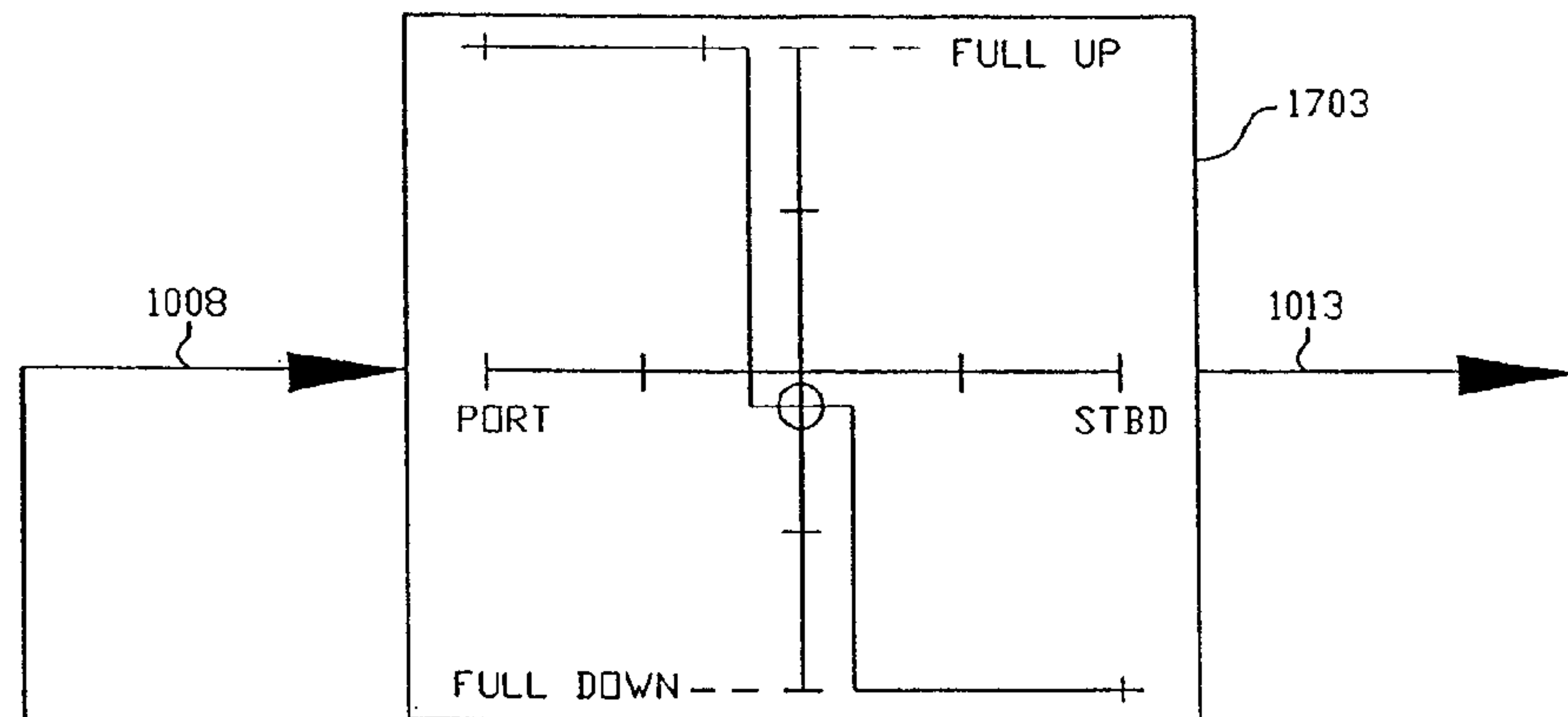
FIG 15D STBD BUCKET POSITION
