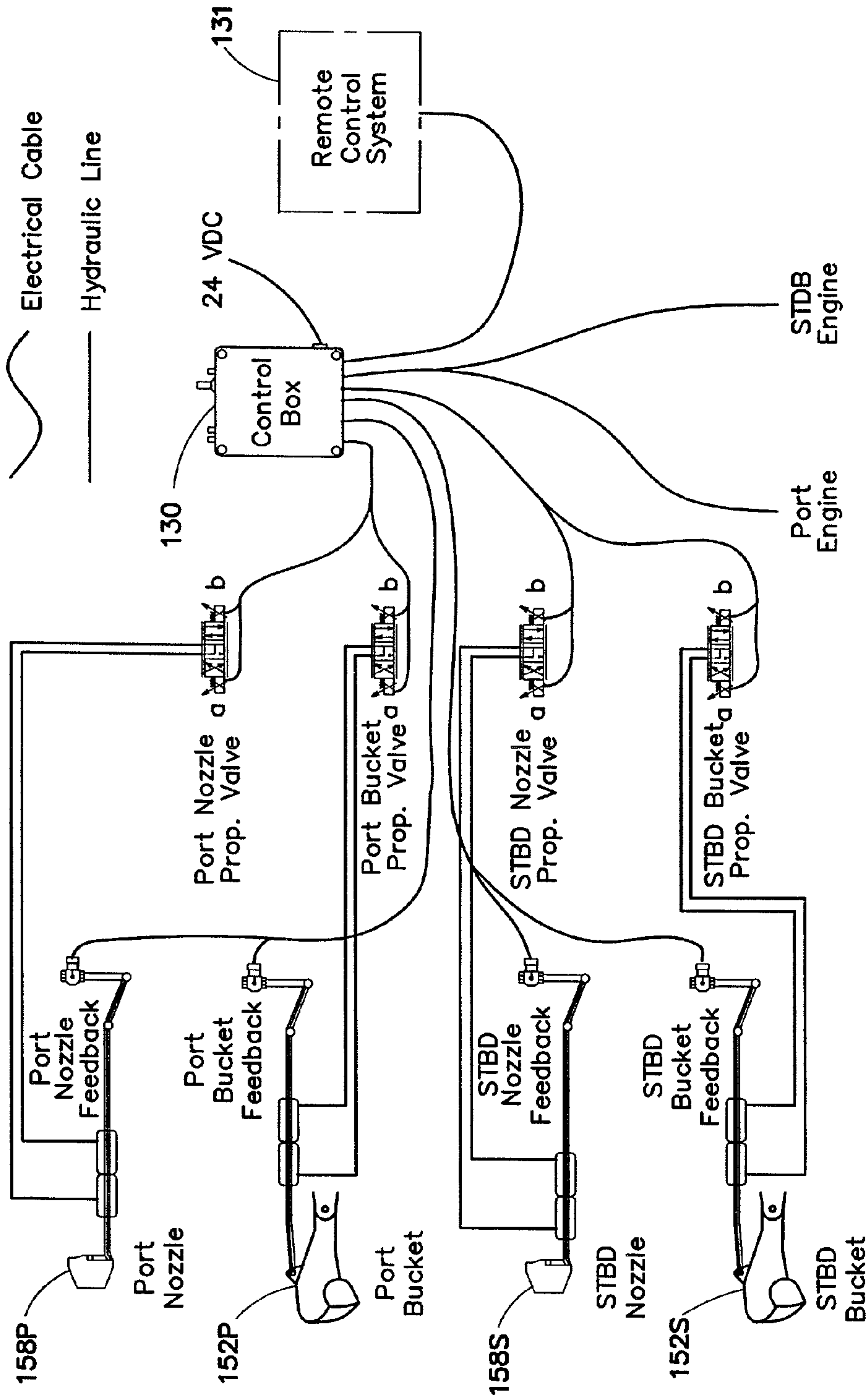
TWIN JET REMOTELY CONTROLLED SYSTEM DIAGRAM
