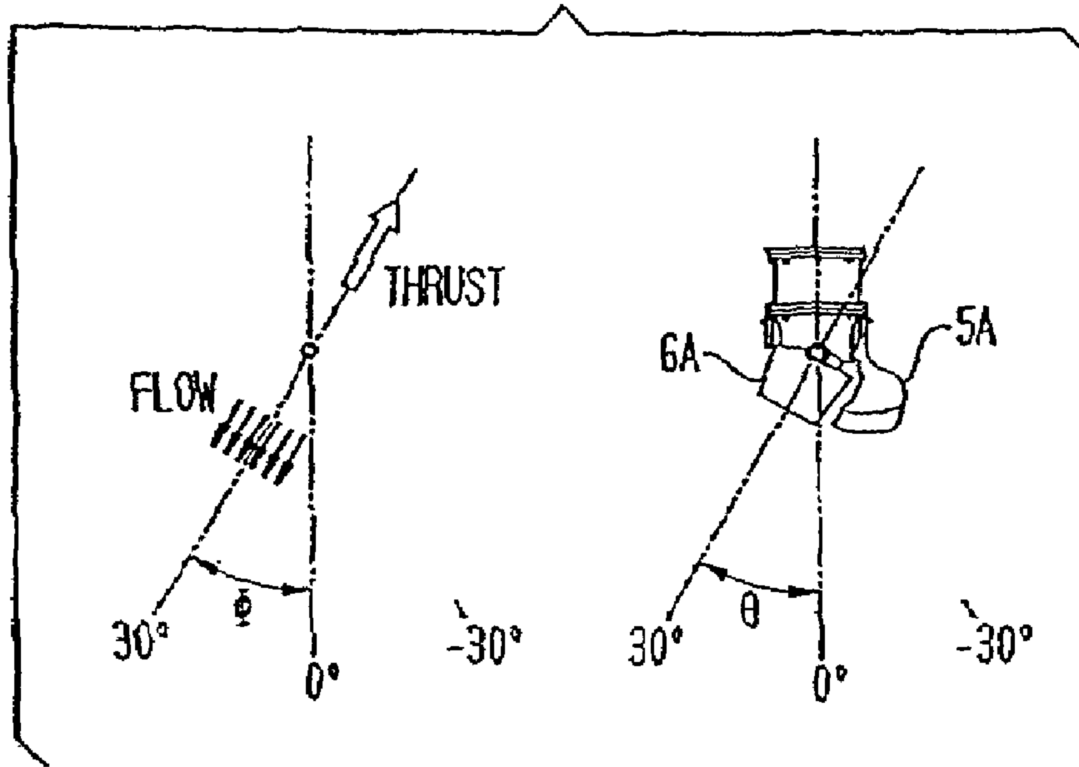
FIG. 25A FULL AHEAD BUCKET
