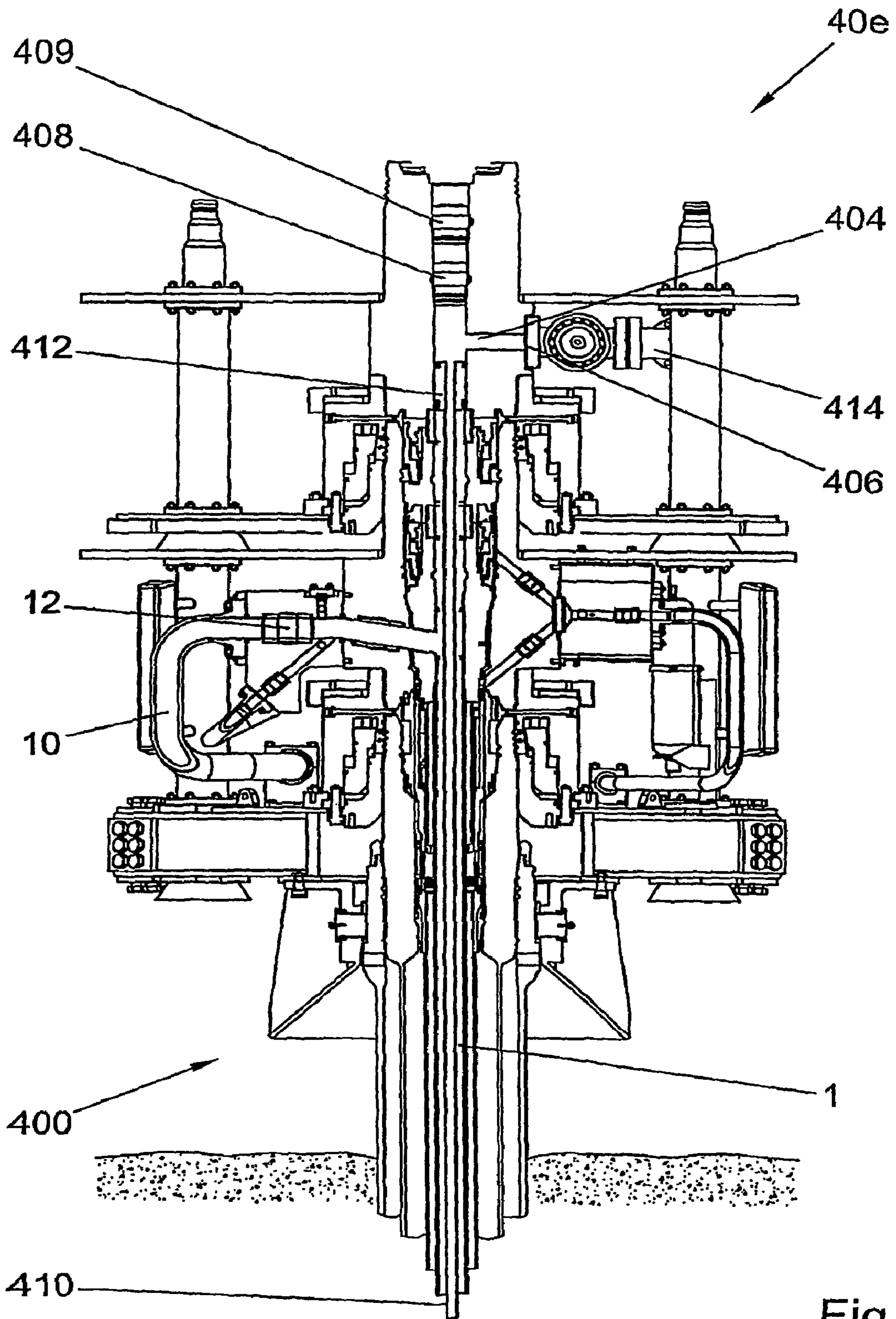
TYPICAL SECTION
