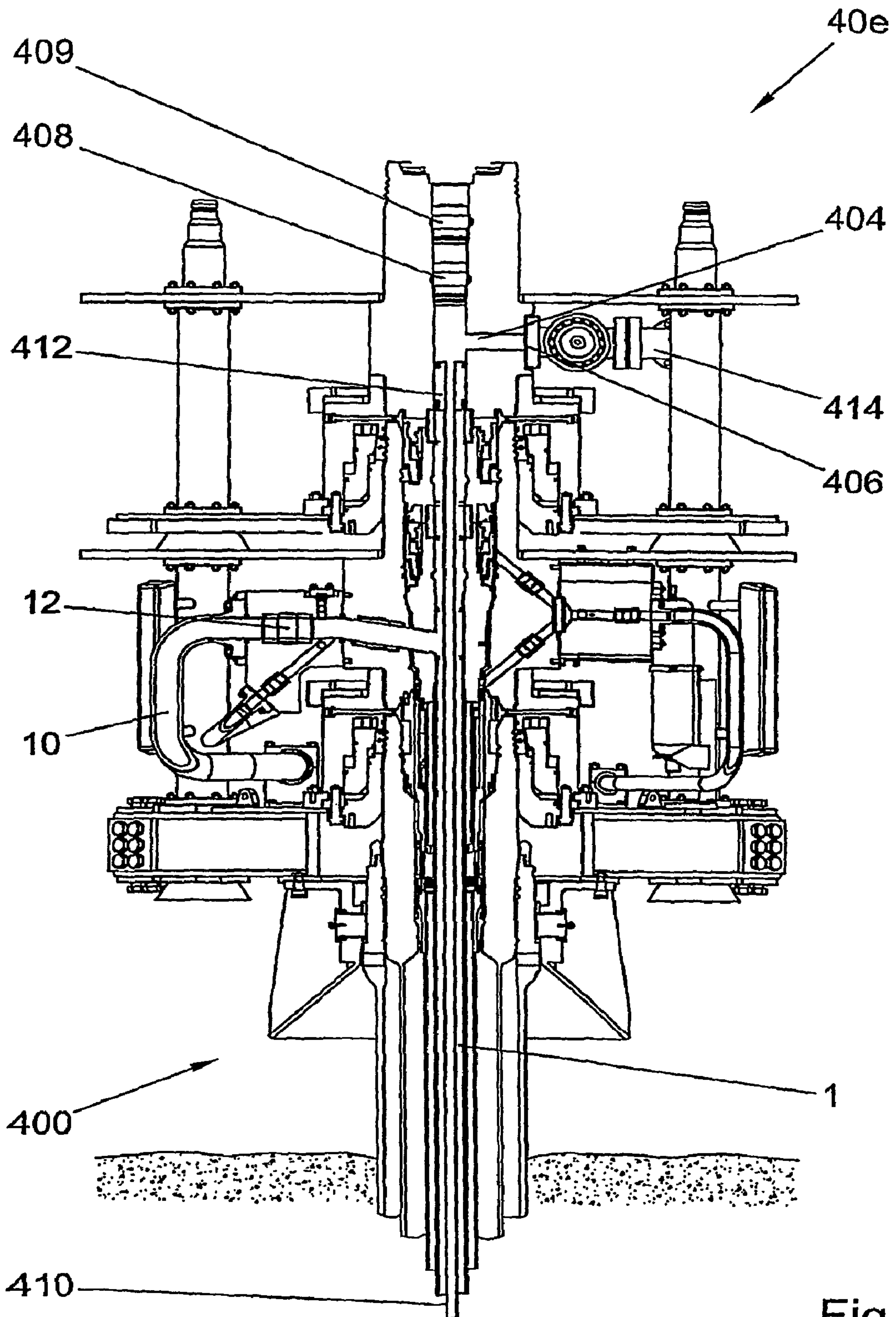
TYPICAL SECTION
