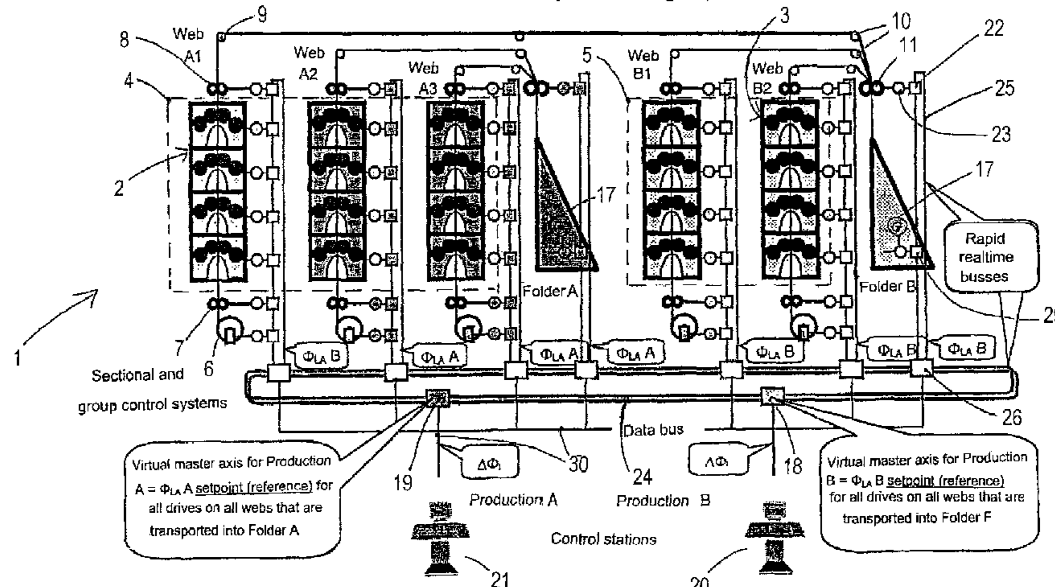
Basic design of a shaftless drive system for two sub-machines A+B (sections), each having several webs, with sectional motion control systems and group control systems
