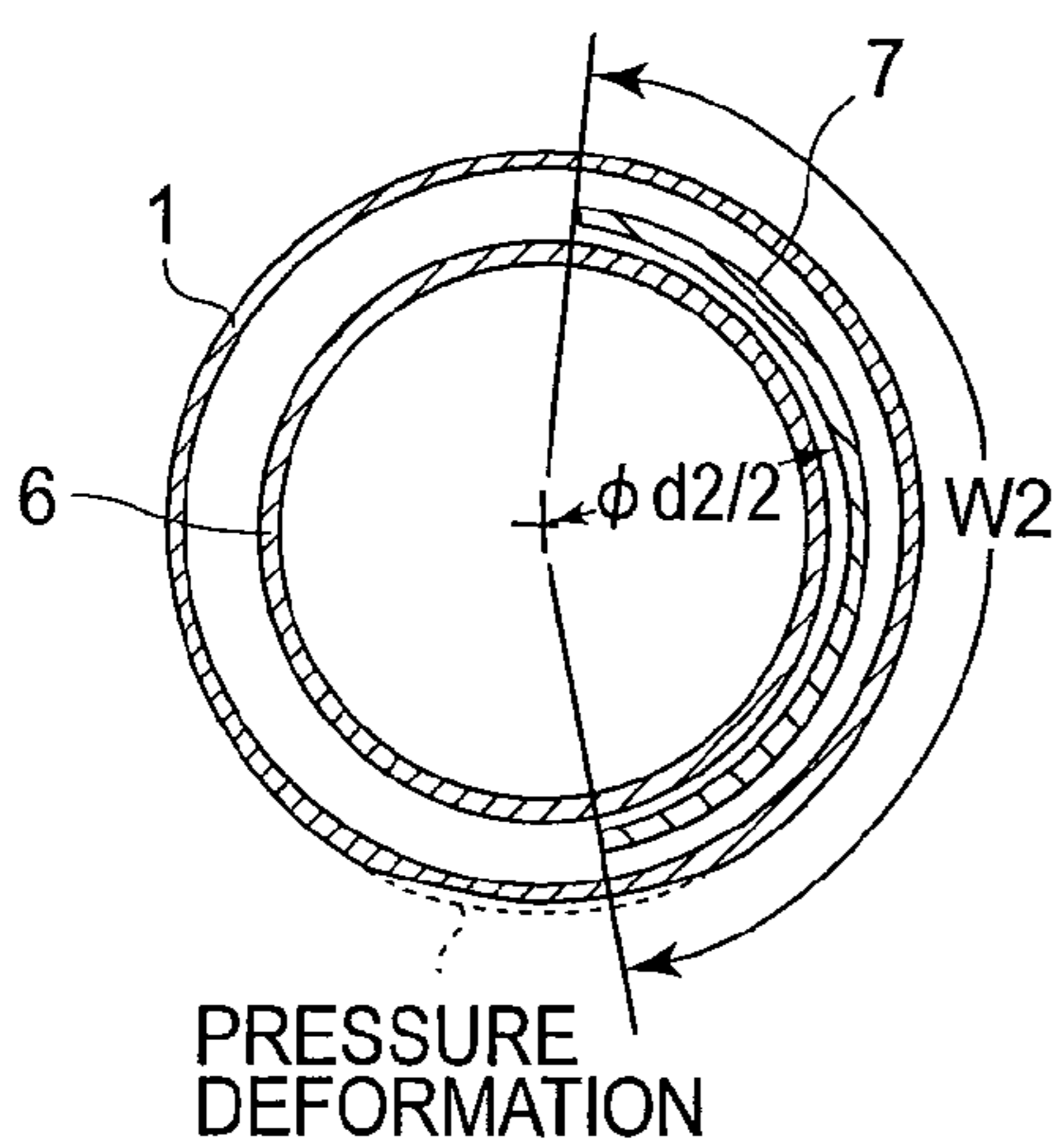
(b) END CROSS-SECTION
