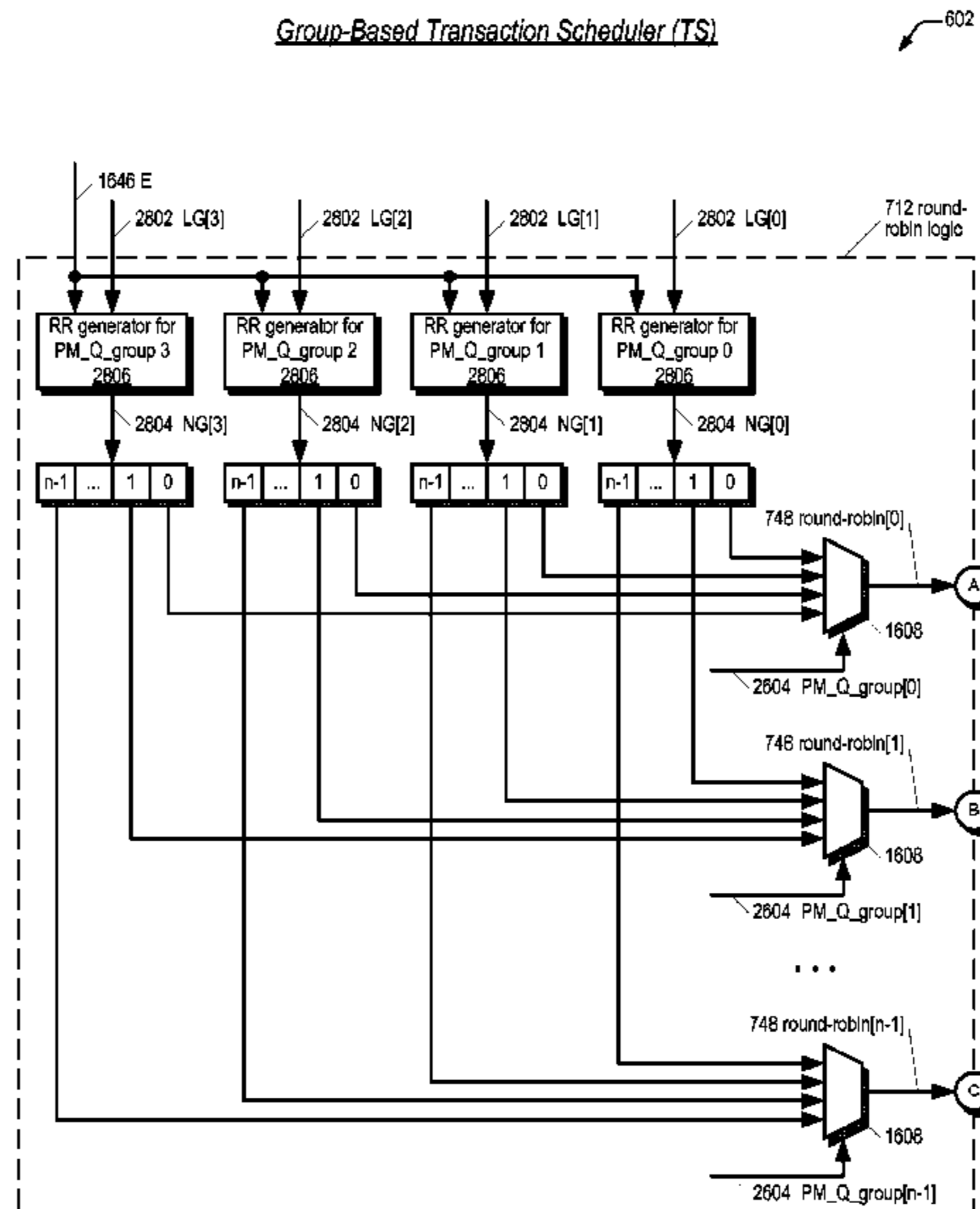
Group-Based Transaction Scheduler (TS)
