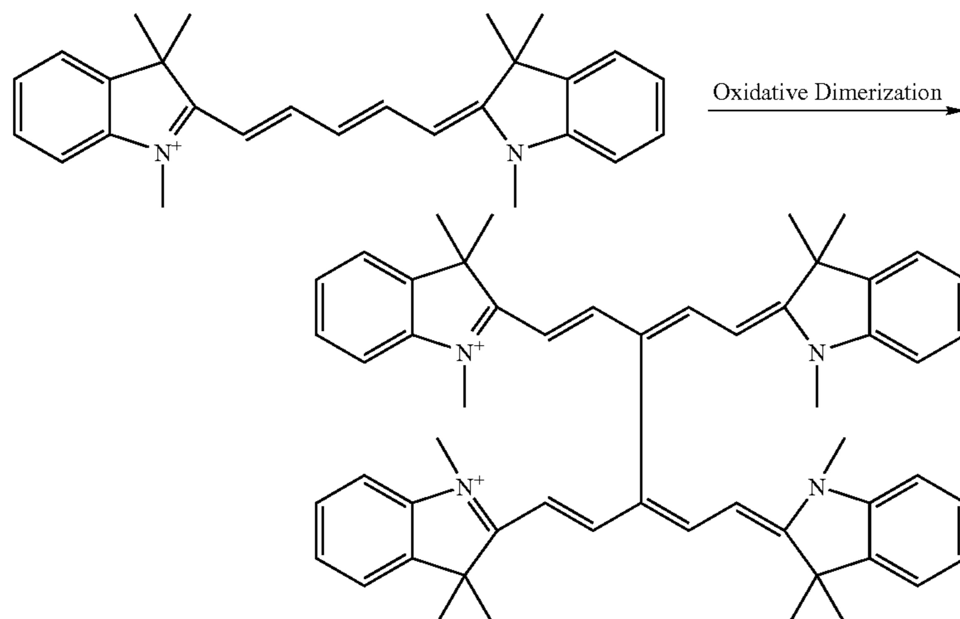
Scheme 2. Oxidative dimerization of carbocyanines
