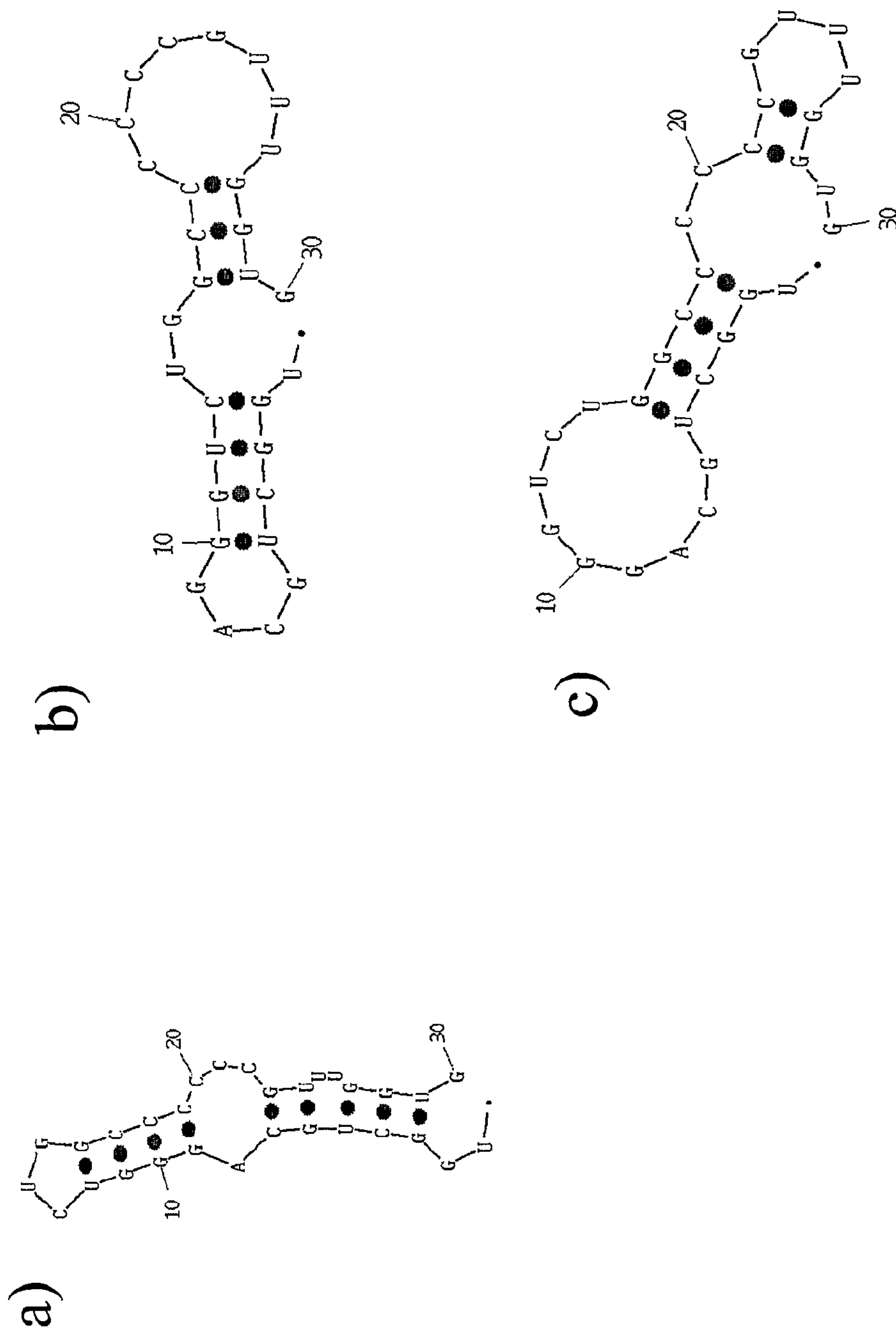
Predicted structures of the 30-mer RNA calculated by MFold program
